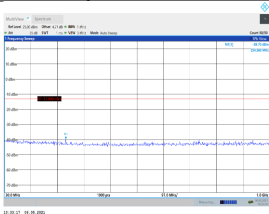
Band66-20MHz-QPSK-132322-1RB#0- Range1:30~1000MHz
