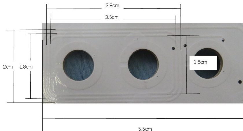
Antenna dimension design
