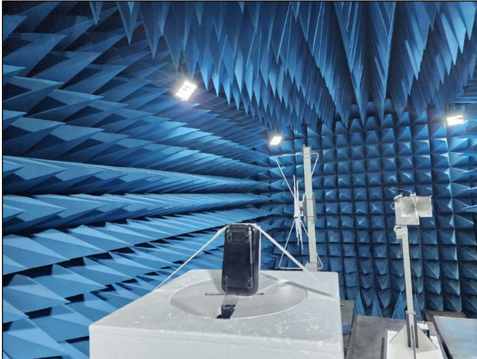
Photo of Test Set up for RSE (30 MHz ~ 12.75 GHz)
