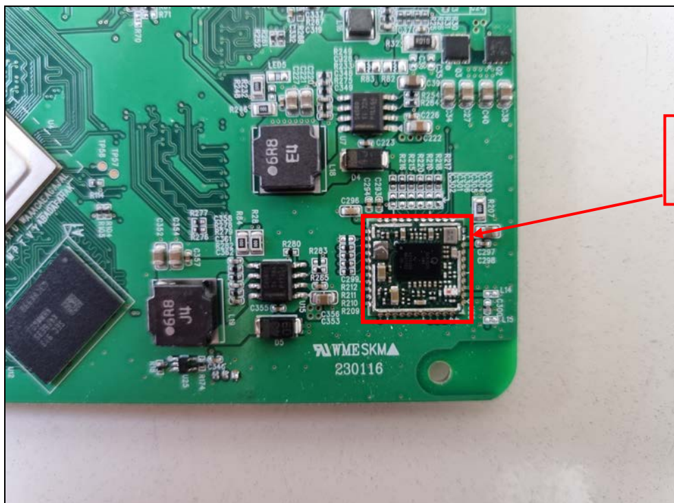
View of Bluetooth & WIFI Module (without Shielding)
