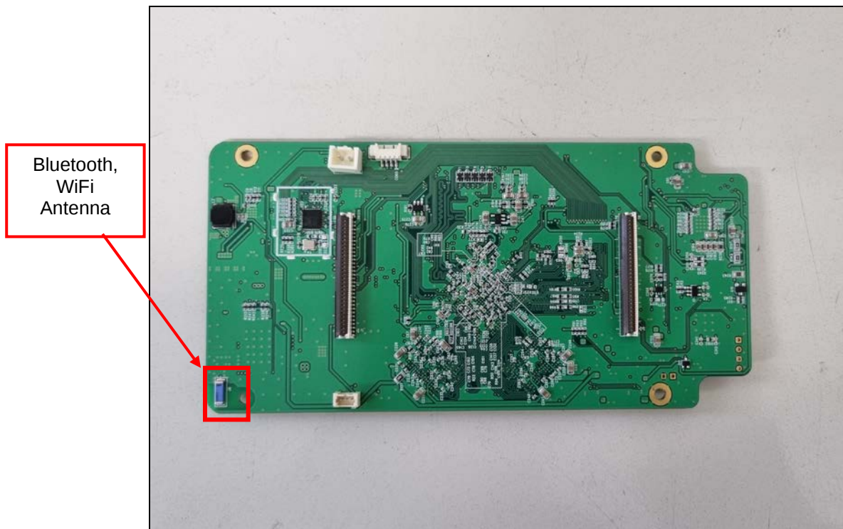
Bottom view of Main PCB
