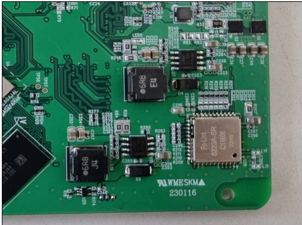
View of Bluetooth & WIFI Module (with Shielding)
