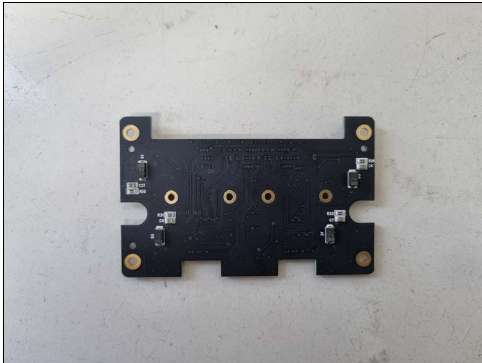
Bottom view of SUB2 PCB
