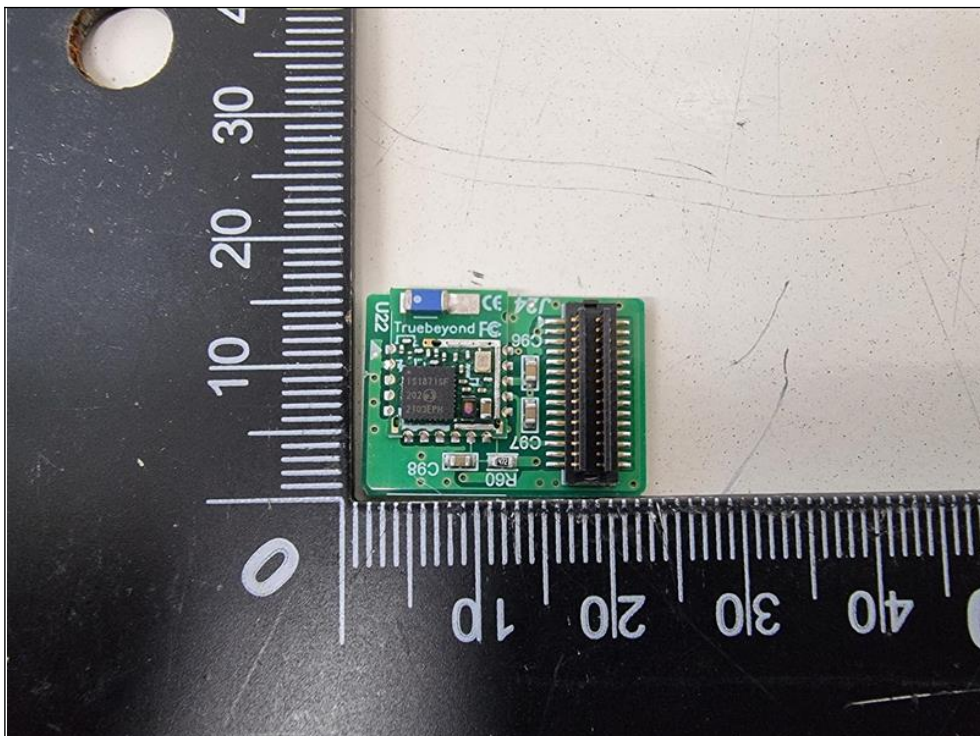
Top view of Module without shielding
