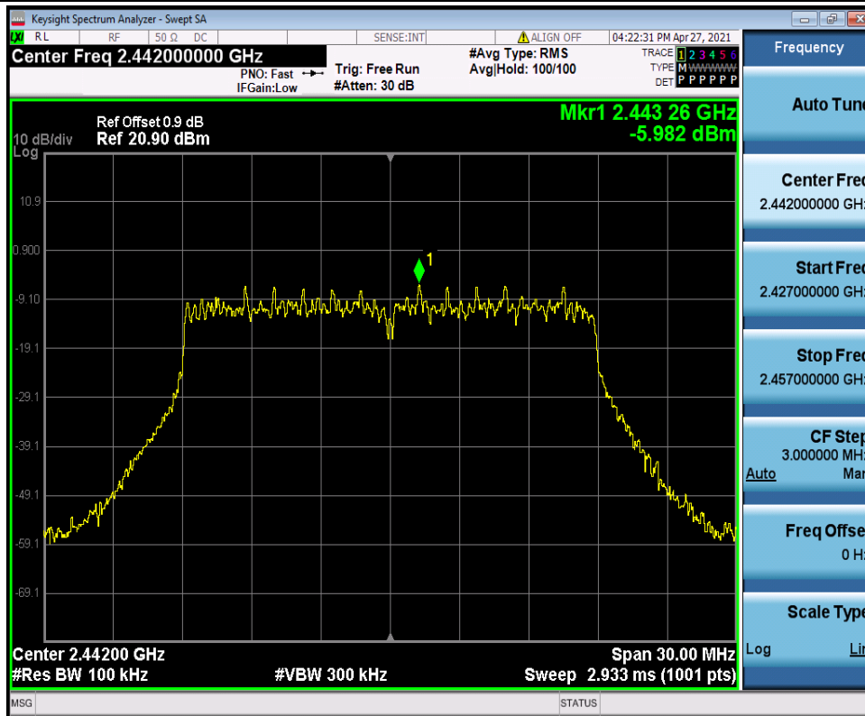
11N20SISO_Ant1_2442_0~Reference
