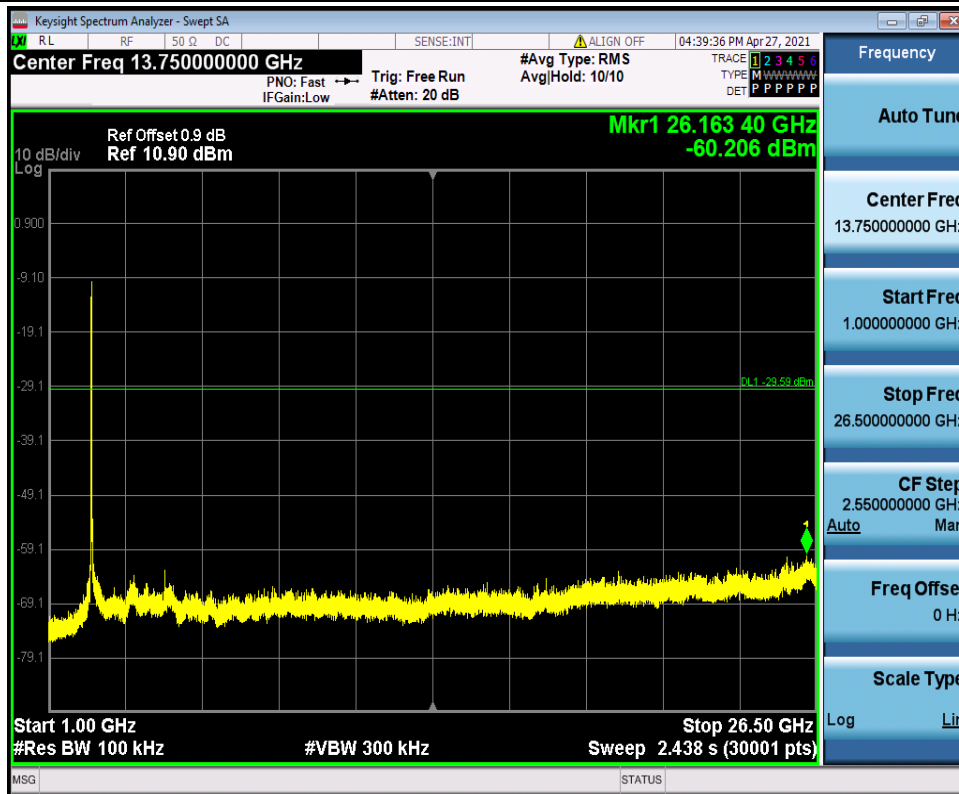
11N40SISO_Ant1_2422_1000~26500
