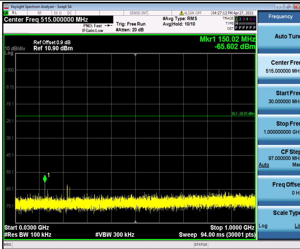
11N20SISO_Ant1_2462_30~1000
