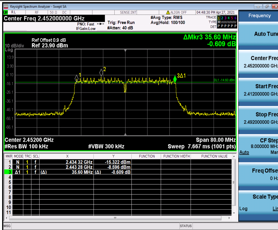
11N40SISO_Ant1_2452
