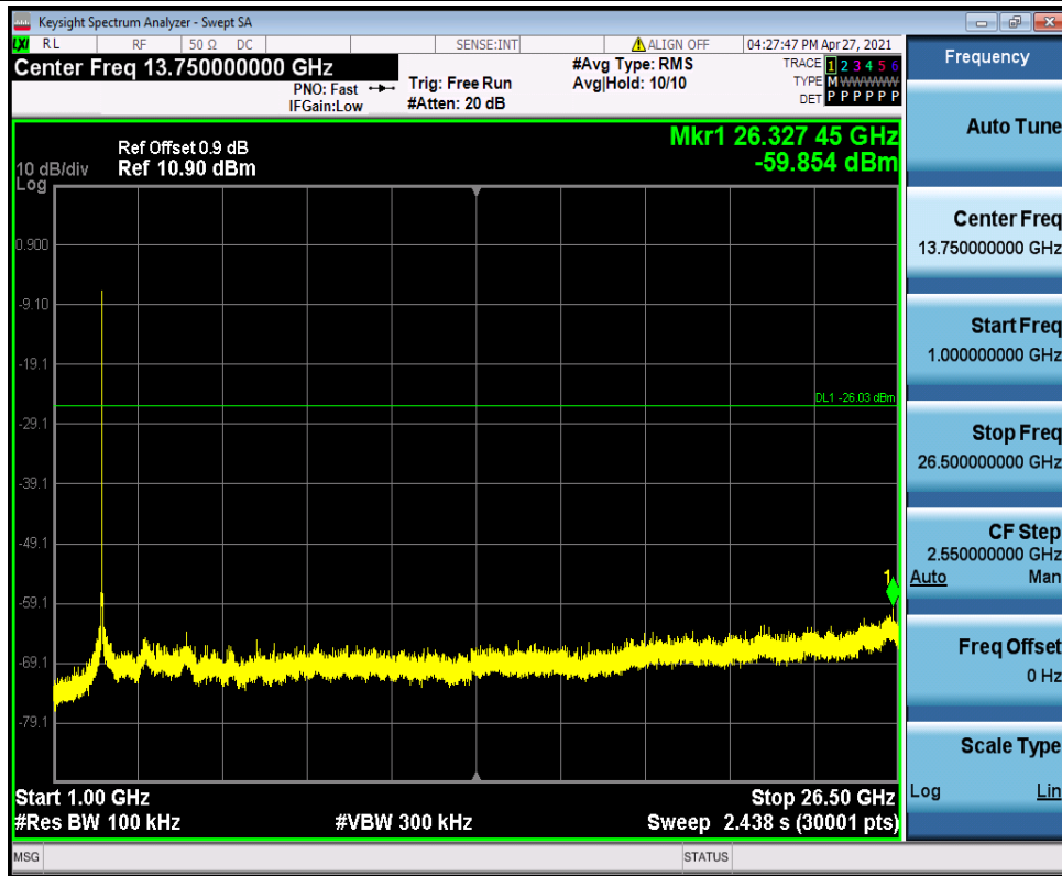
11N40SISO_Ant1_2422_0~Reference
