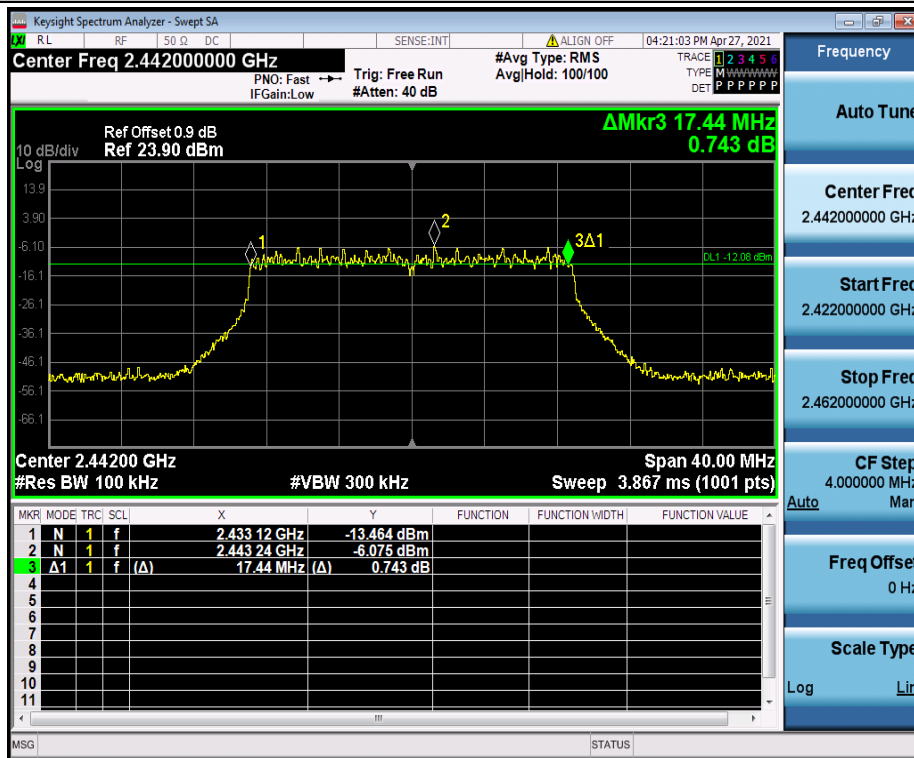
11N20SISO_Ant1_2442
