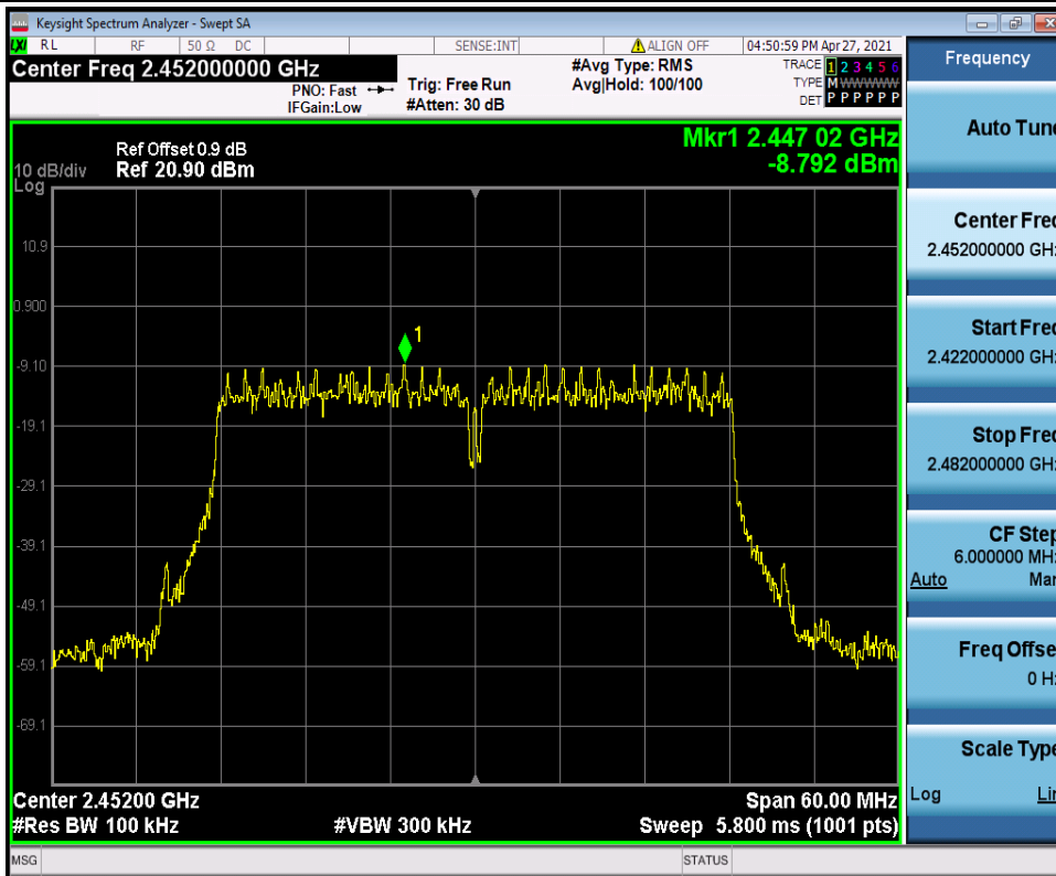
11N40SISO_Ant1_2452_0~Reference
