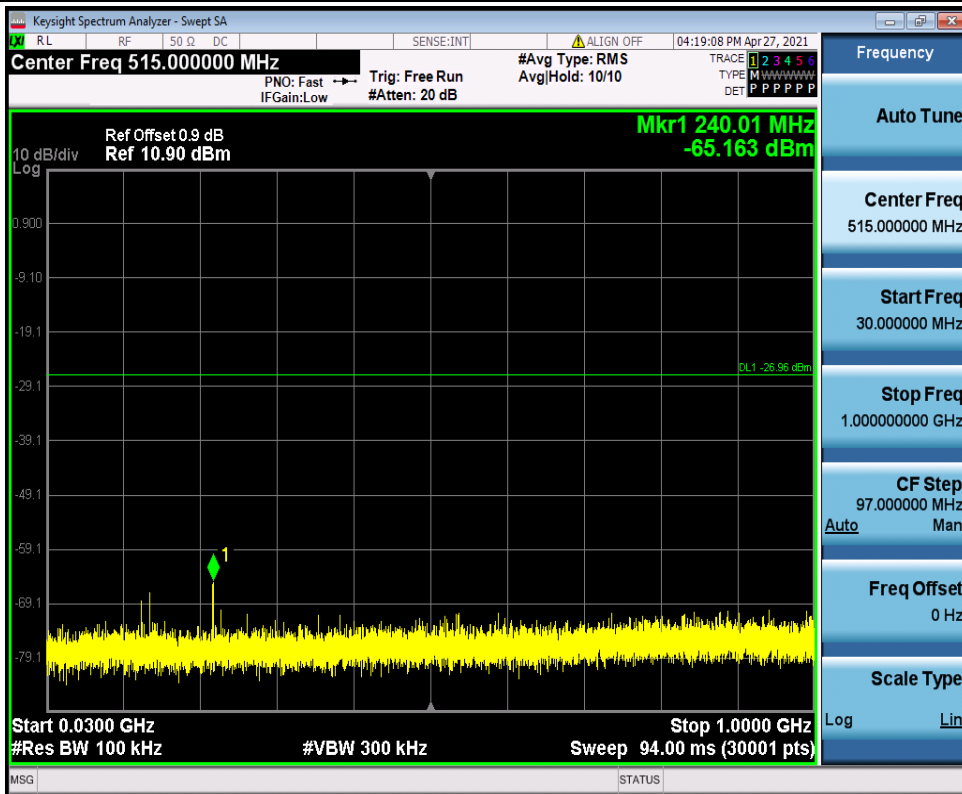
11N20SISO_Ant1_2412_30~1000
