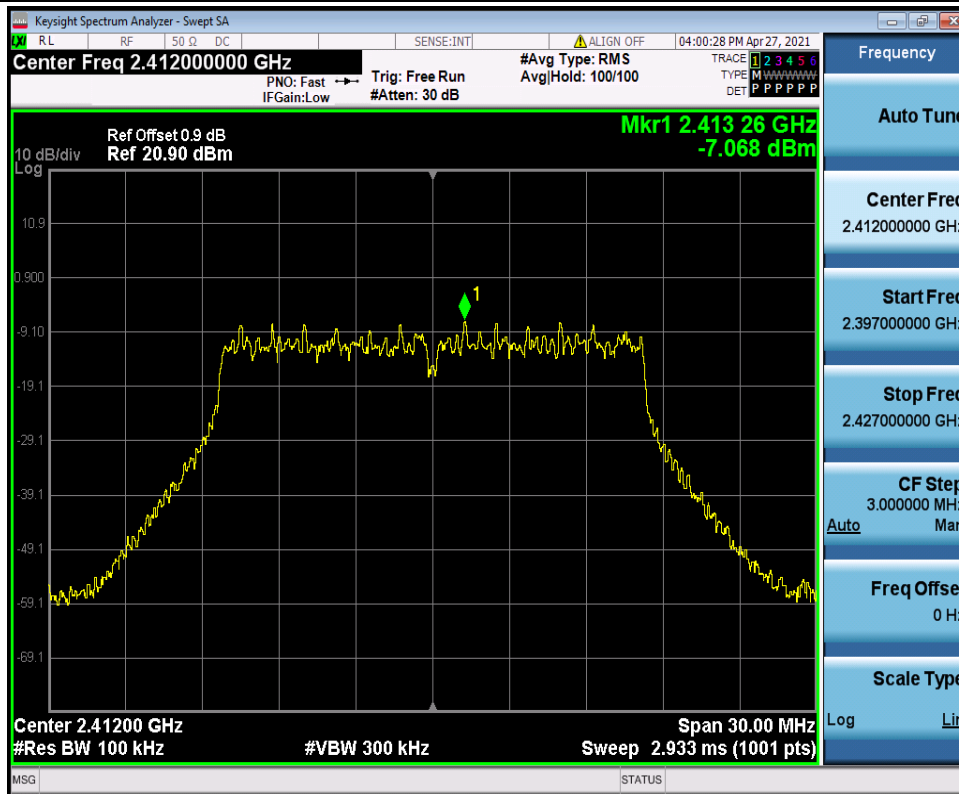
11G_Ant1_2412_0~Reference
