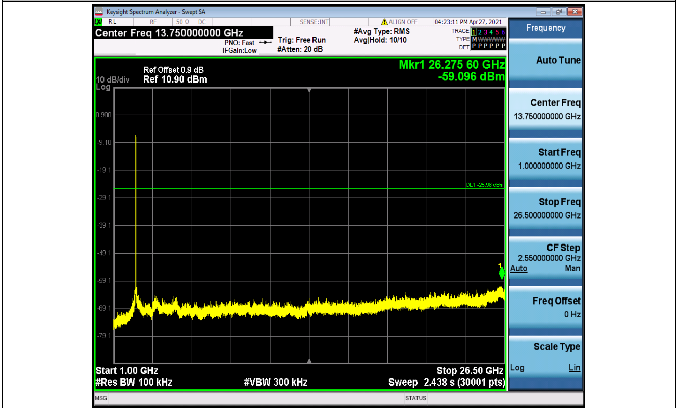
11N20SISO_Ant1_2442_1000~26500
