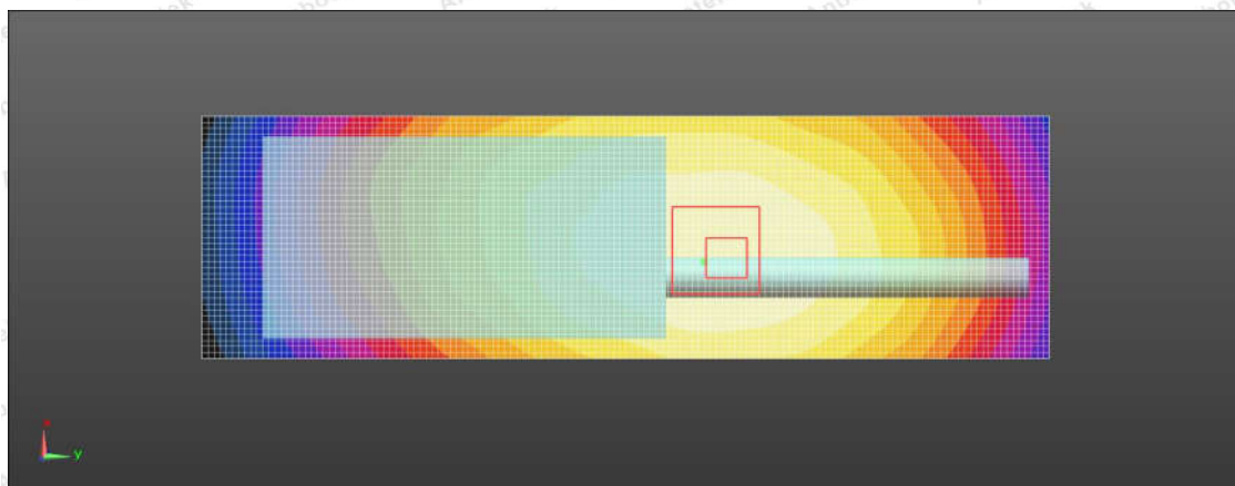
Figure 1: PMR_FM12.5KHz_Face held_25mm
