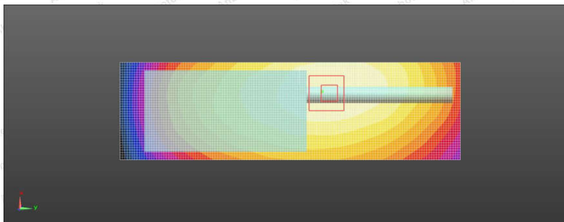
Figure 2: PMR_FM12.5KHz_Body Worn_0mm
