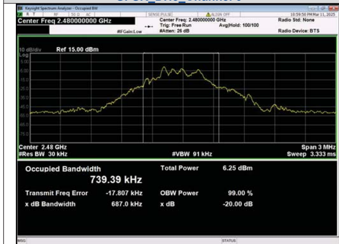
GFSK_DH5_Channel 78
