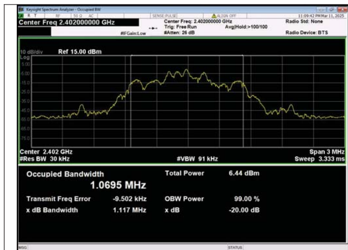
8DPSK_3-DH5_Channel 0
