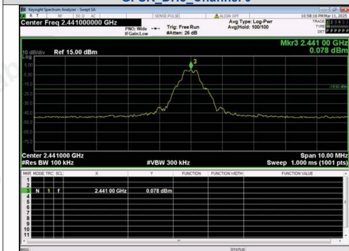
Out Of Band Emission GFSK_DH5_Channel 39
