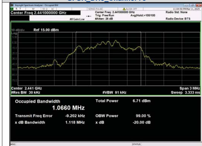
\pi/4 DQPSK_2-DH5_Channel 39
