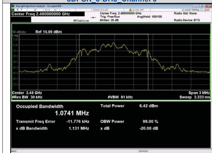
8DPSK_3-DH5_Channel 78
