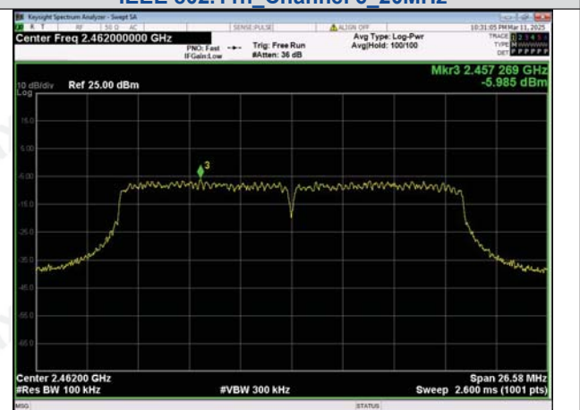
In-Band Reference Level IEEE 802.11n_Channel 11_20MHz
