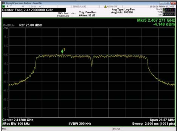
In-Band Reference Level IEEE 802.11n_Channel 1_20MHz
