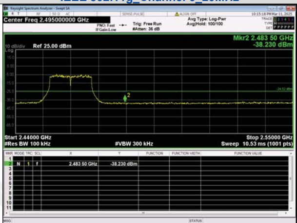
Out Of Band Emission IEEE 802.11g_Channel 11_20MHz
