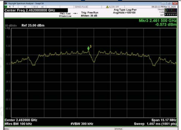
In-Band Reference Level IEEE 802.11b_Channel 11_20MHz
