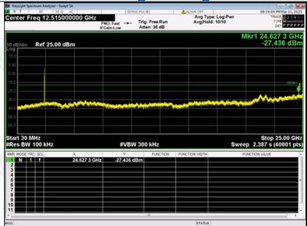
30.0 MHz - 25000.0 MHz IEEE 802.11b_Channel 1_20MHz
