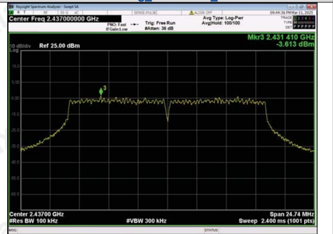
In-Band Reference Level IEEE 802.11g_Channel 6_20MHz
