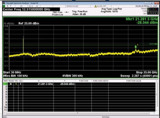
30.0 MHz - 25000.0 MHz IEEE 802.11b_Channel 6_20MHz
