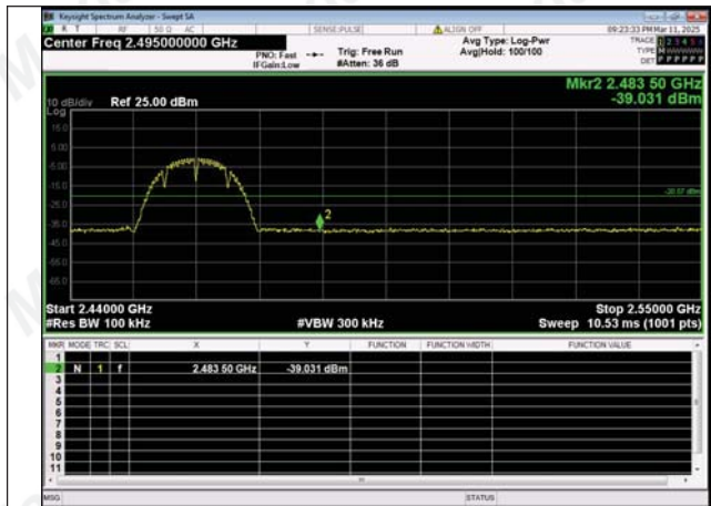
Out Of Band Emission IEEE 802.11b_Channel 11_20MHz
