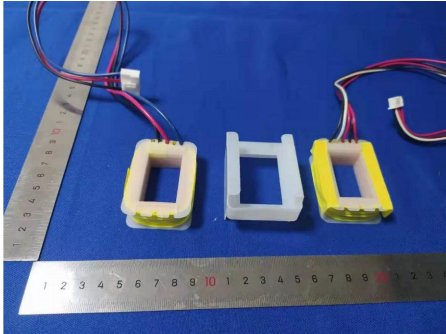
AC transformer
