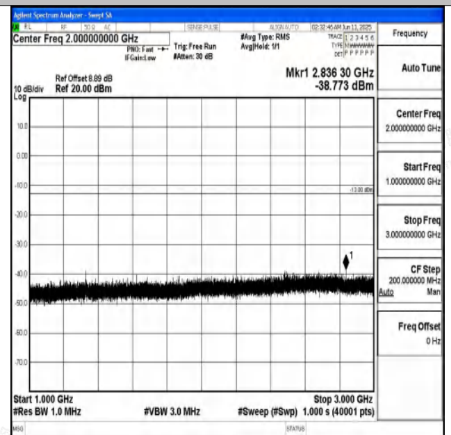
Band71_10MHz_QPSK_133172_1RB#0_1000~3000_1000 ~3000
