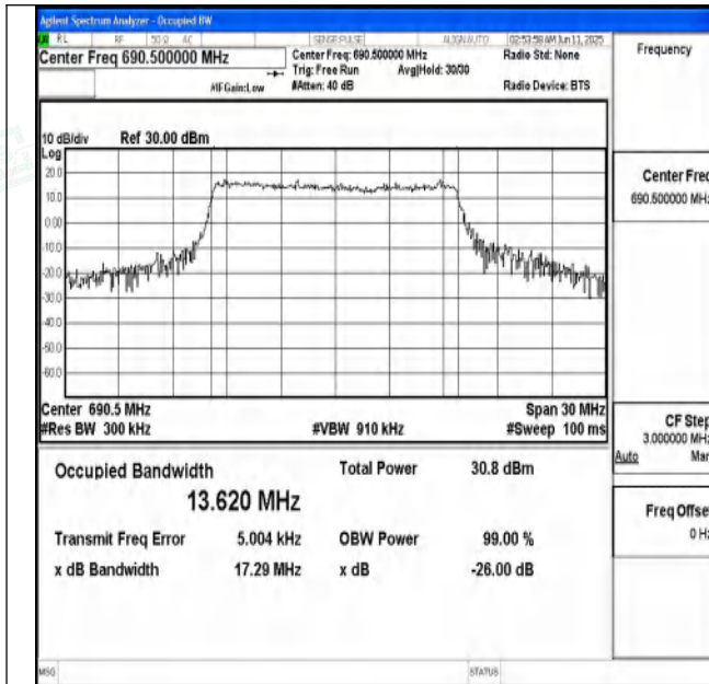
Band71-15MHz-QPSK-133397-75RB#0-PASS
