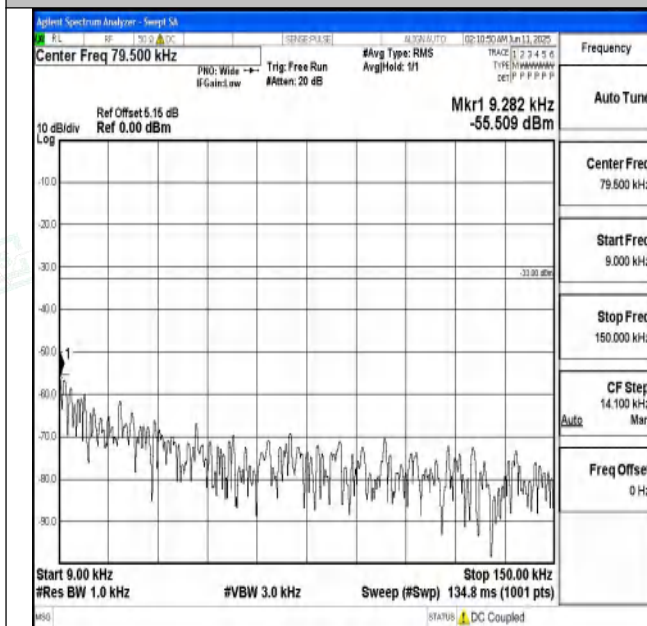
Band71_5MHz_QPSK_133297_1RB#0_0.009~0.15_0.009~ 0.15
