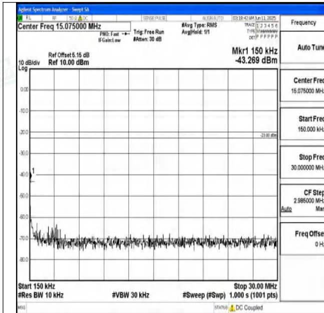
Band71_20MHz_QPSK_133222_1RB#0_0.15~30_0.15~30
