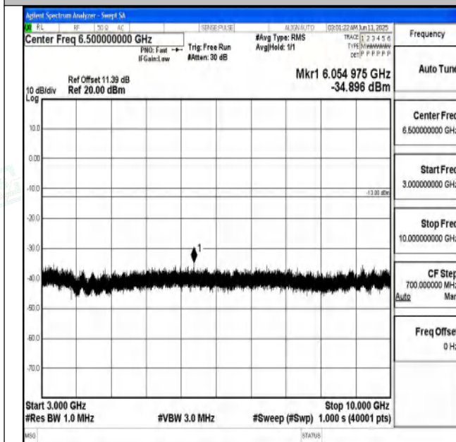
Band71_15MHz_QPSK_133397_1RB#0_3000~10000_3000 ~10000
