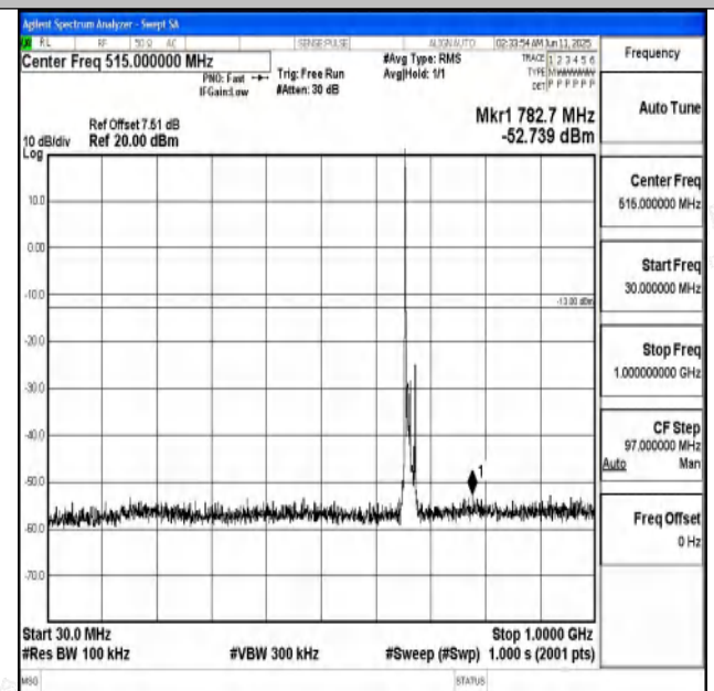
Band71_10MHz_16QAM_133172_1RB#0_30~1000_30~1000
