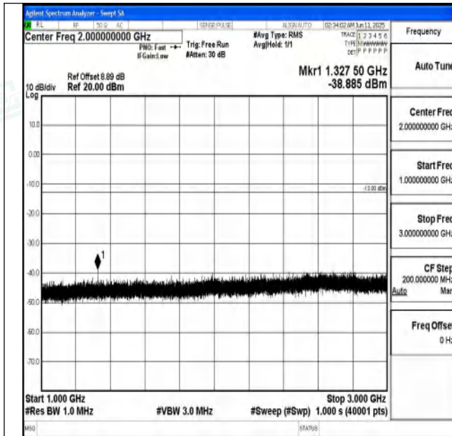
Band71_10MHz_16QAM_133172_1RB#0_1000~3000_100 0~3000
