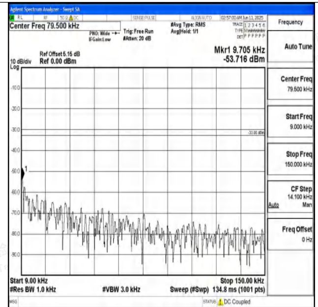
Band71_15MHz_16QAM_133197_1RB#0_0.009~0.15_0.009~0.15
