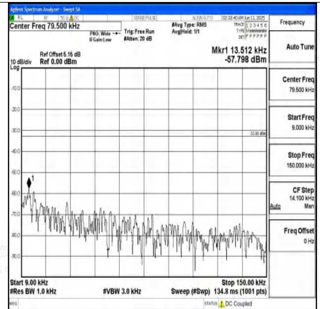
Band71_10MHz_16QAM_133172_1RB#0_0.009~0.15_0.009~0.15
