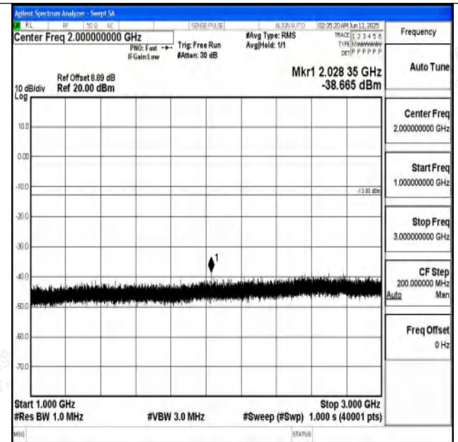
Band71_10MHz_QPSK_133297_1RB#0_1000~3000_1000
