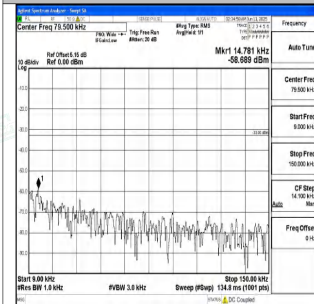
Band71_10MHz_QPSK_133297_1RB#0_0.009~0.15_0.009 ~0.15
