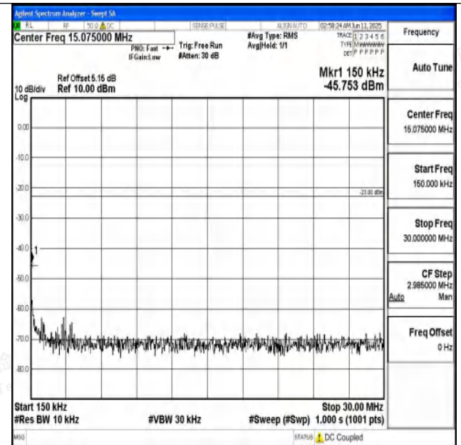
Band71_15MHz_QPSK_133297_1RB#0_0.15~30_0.15~30
