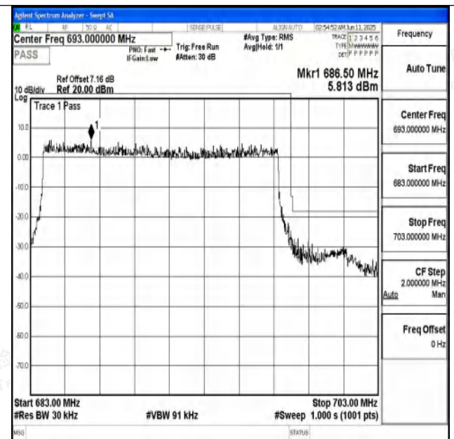
Band71_15MHz_16QAM_133397_75RB#0
