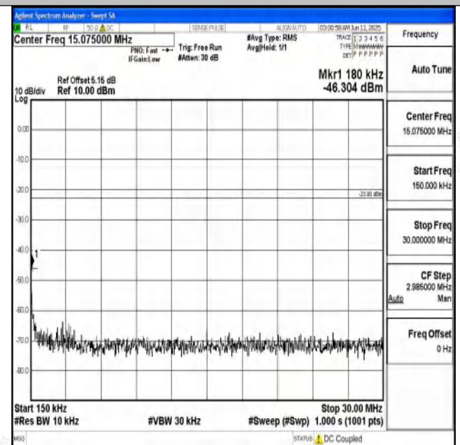
Band71_15MHz_QPSK_133397_1RB#0_0.15~30_0.15~30
