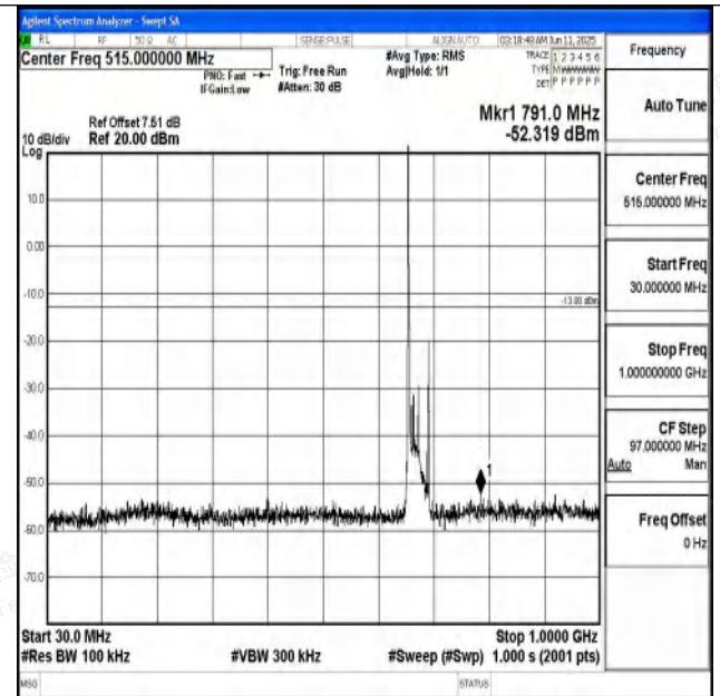
Band71_20MHz_QPSK_133222_1RB#0_30~1000_30~100 0
