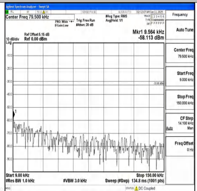
Band71_5MHz_16QAM_133297_1RB#0_0.009~0.15_0.009~0.15
