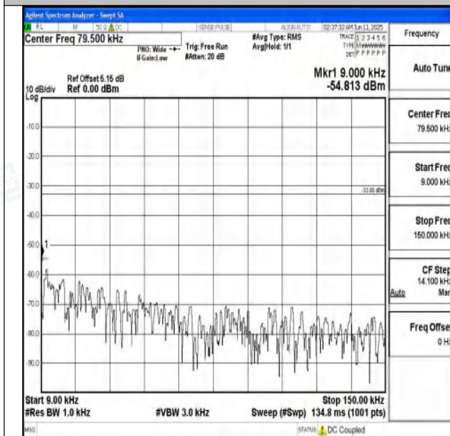
Band71_10MHz_QPSK_133422_1RB#0_0.009~0.15_0.009
