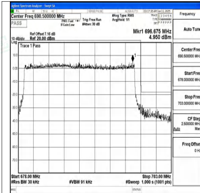
Band71_20MHz_QPSK_133372_100RB#0
