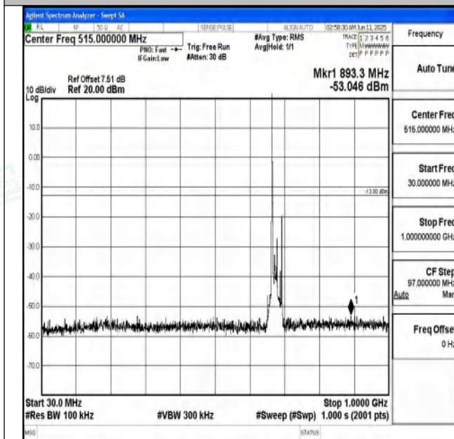
Band71_15MHz_QPSK_133297_1RB#0_30~1000_30~100 0
