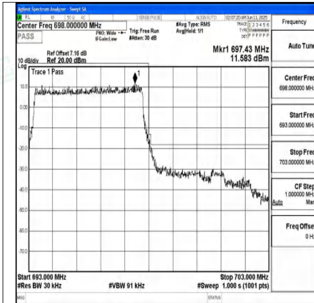
Band71_5MHz_QPSK_133447_25RB#0
