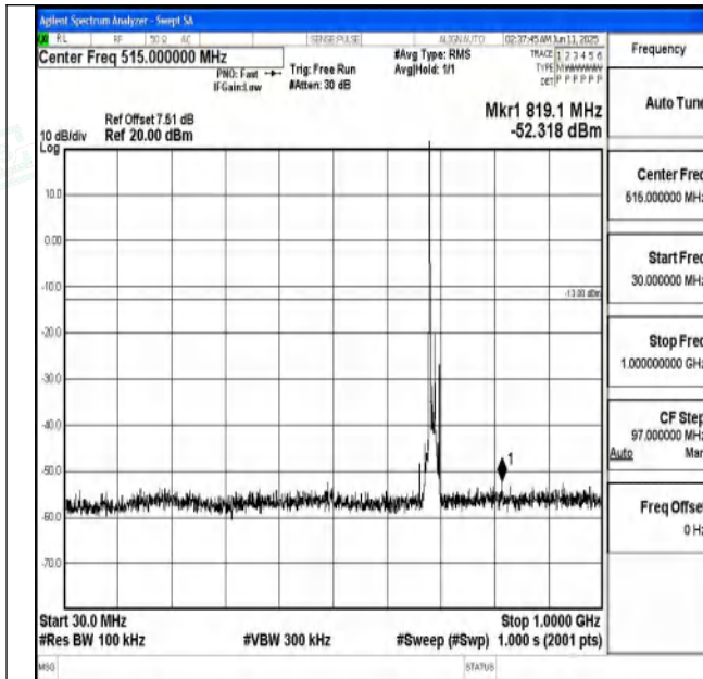
Band71_10MHz_QPSK_133422_1RB#0_30~1000_30~100
