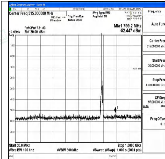
Band71_5MHz_16QAM_133447_1RB#0_30~1000_30~100
