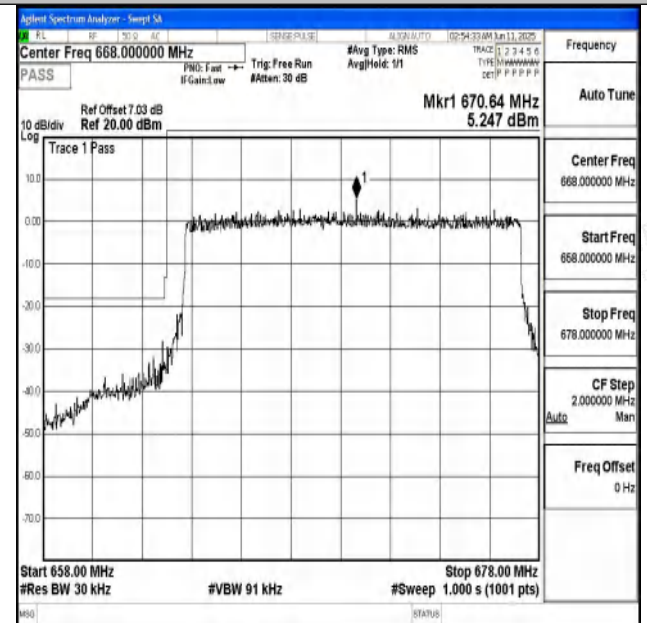
Band71_15MHz_16QAM_133197_75RB#0
