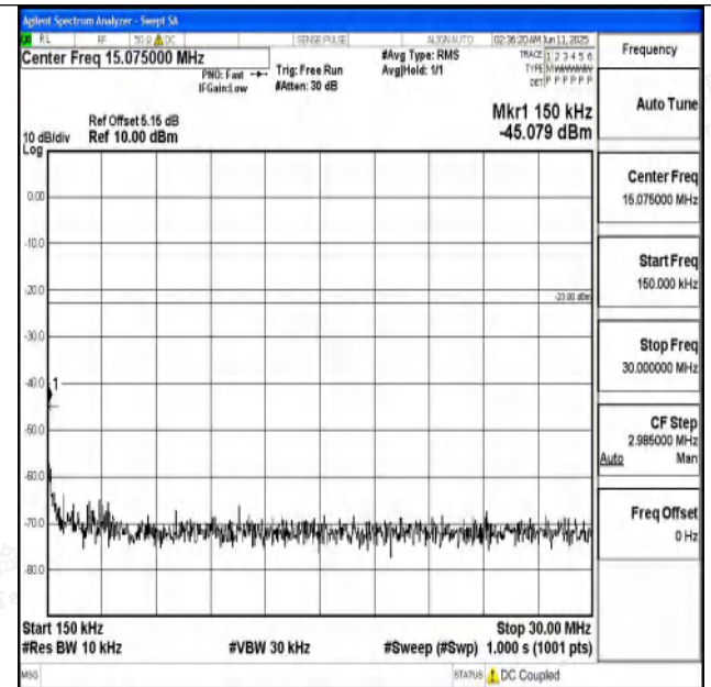
Band71_10MHz_16QAM_133297_1RB#0_0.15~30_0.15~3 0
