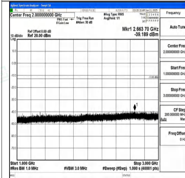
Band71_20MHz_16QAM_133222_1RB#0_1000~3000_1000~3000
