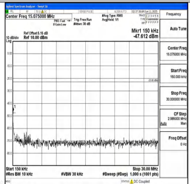
Band71_10MHz_QPSK_133422_1RB#0_0.15~30_0.15~30
