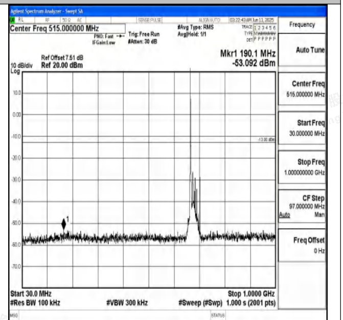
Band71_20MHz_16QAM_133322_1RB#0_30~1000_30~1000
