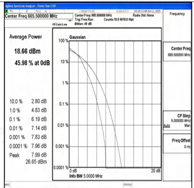
Band71-5MHz-16QAM-133147-25RB#0-PASS
