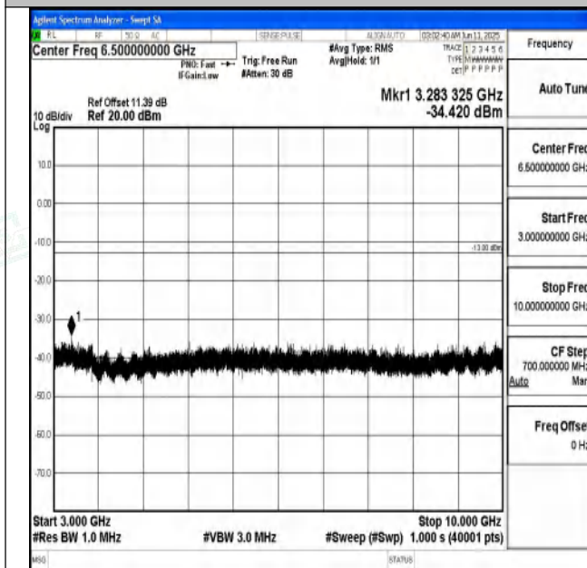
Band71_15MHz_16QAM_133397_1RB#0_3000~10000_30 00~10000
