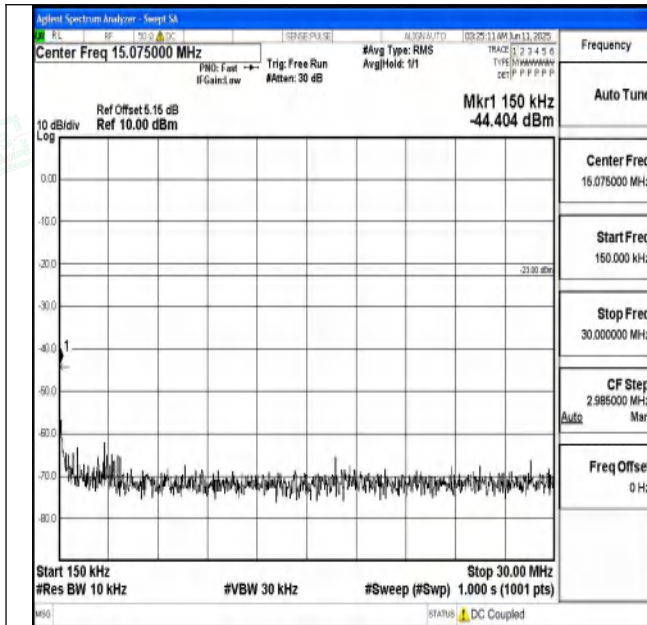
Band71_20MHz_16QAM_133372_1RB#0_0.15~30_0.15~3
