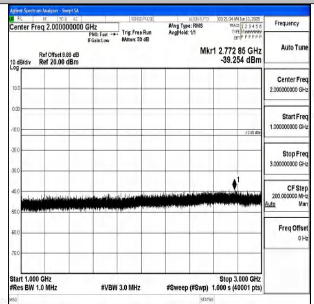
Band71_20MHz_QPSK_133322_1RB#0_1000~3000_1000 ~3000
