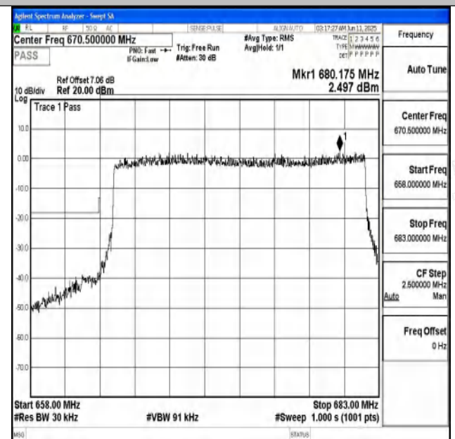
Band71_20MHz_16QAM_133222_100RB#0
