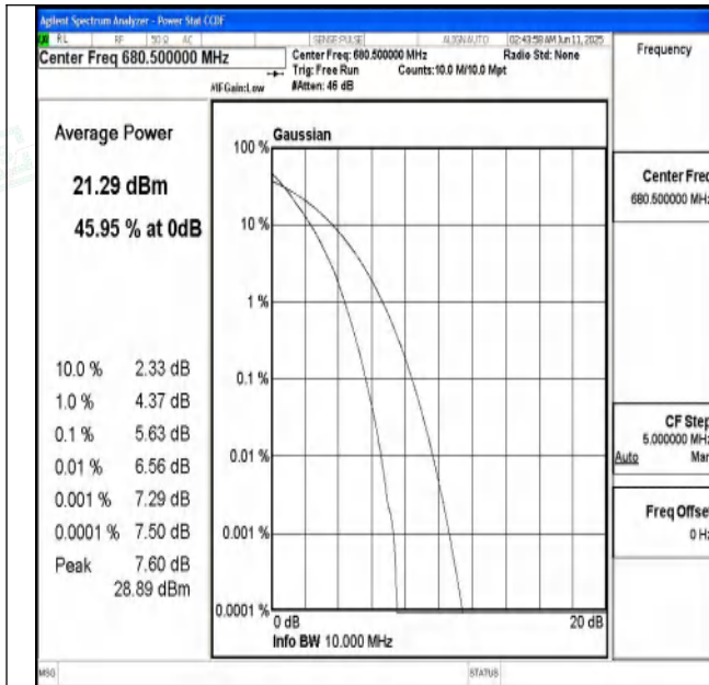
Band71-10MHz-QPSK-133297-50RB#0-PASS
