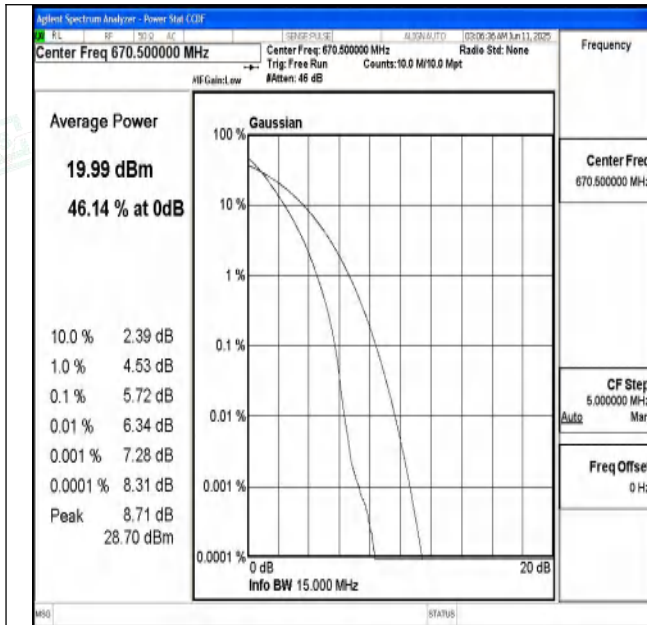
Band71-15MHz-QPSK-133197-75RB#0-PASS
