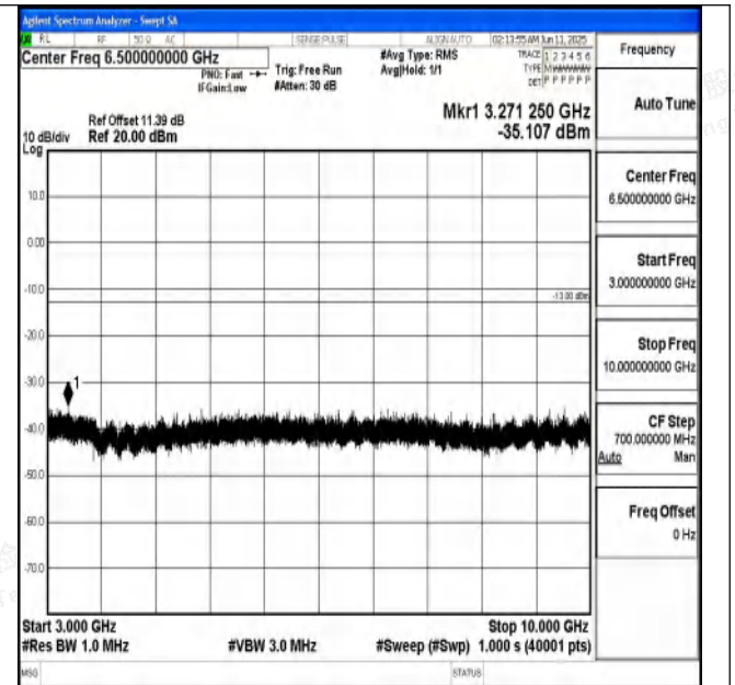
Band71_5MHz_QPSK_133447_1RB#0_3000~10000_3000
