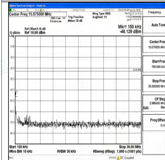
Band71_20MHz_16QAM_133322_1RB#0_0.15~30_0.15~30
