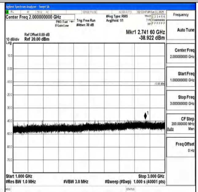
Band71_5MHz_QPSK_133447_1RB#0_1000~3000_1000~3000
