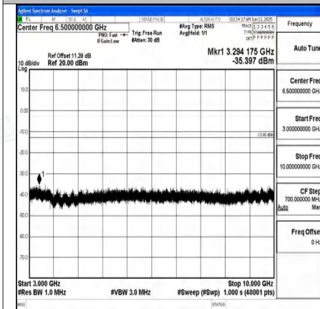
Band71_20MHz_QPSK_133372_1RB#0_3000~10000_3000~10000
