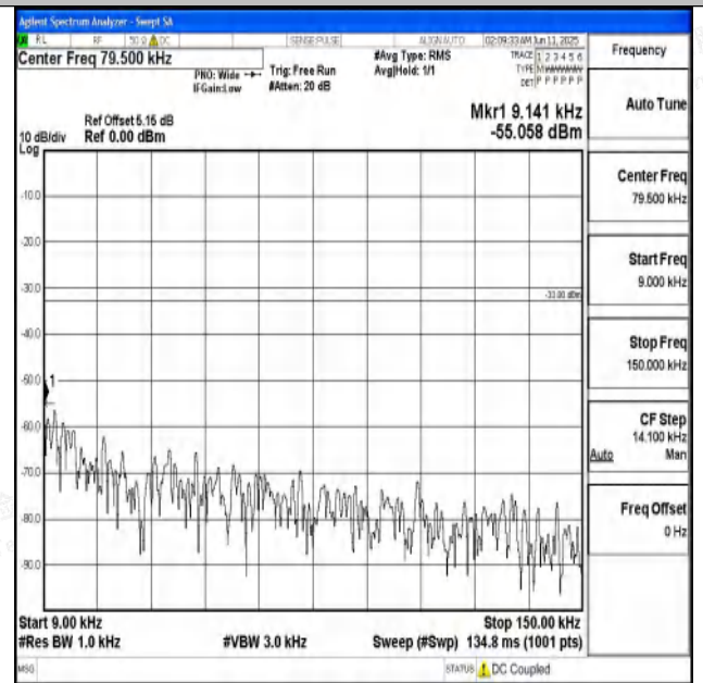
Band71_5MHz_16QAM_133147_1RB#0_0.009~0.15_0.009 ~0.15
