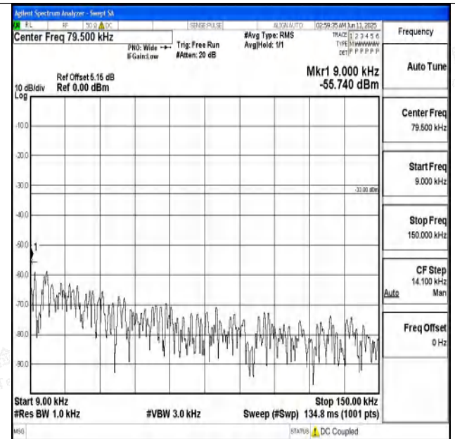
Band71_15MHz_16QAM_133297_1RB#0_0.009~0.15_0.009~0.15
