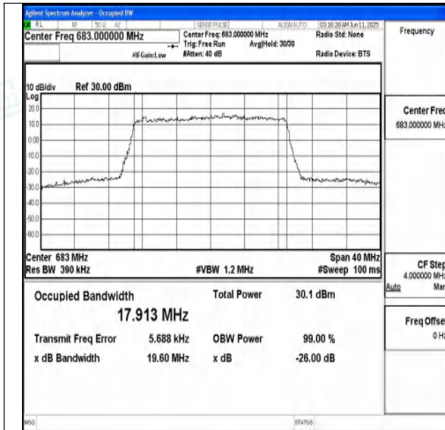
Band71-20MHz-QPSK-133322-100RB#0-PASS
