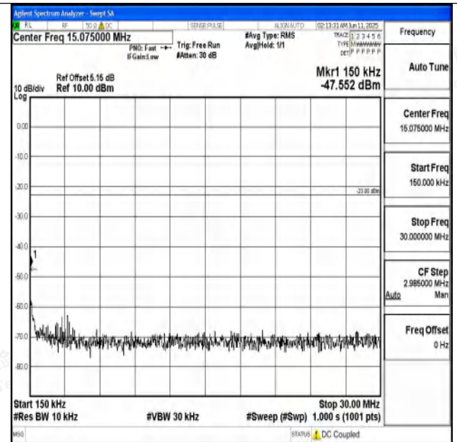
Band71_5MHz_QPSK_133447_1RB#0_0.15~30_0.15~30
