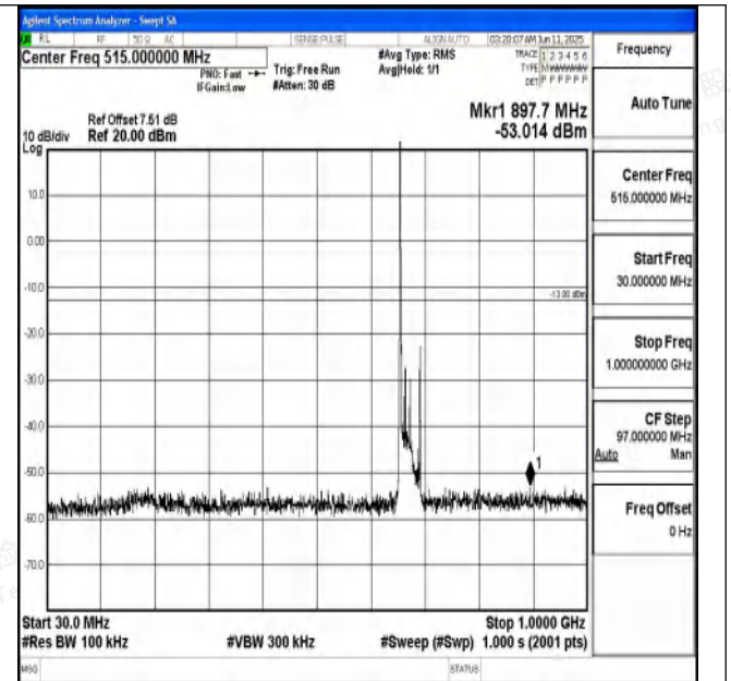
Band71_20MHz_16QAM_133222_1RB#0_30~1000_30~10
