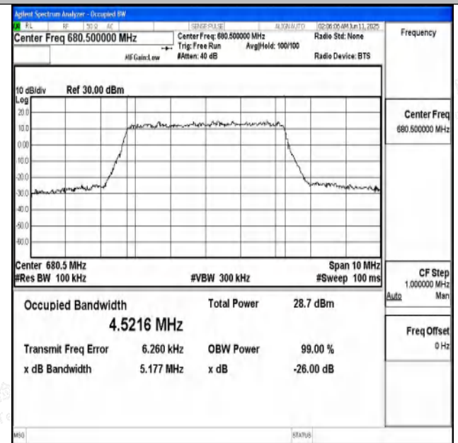
Band71-5MHz-16QAM-133297-25RB#0-PASS
