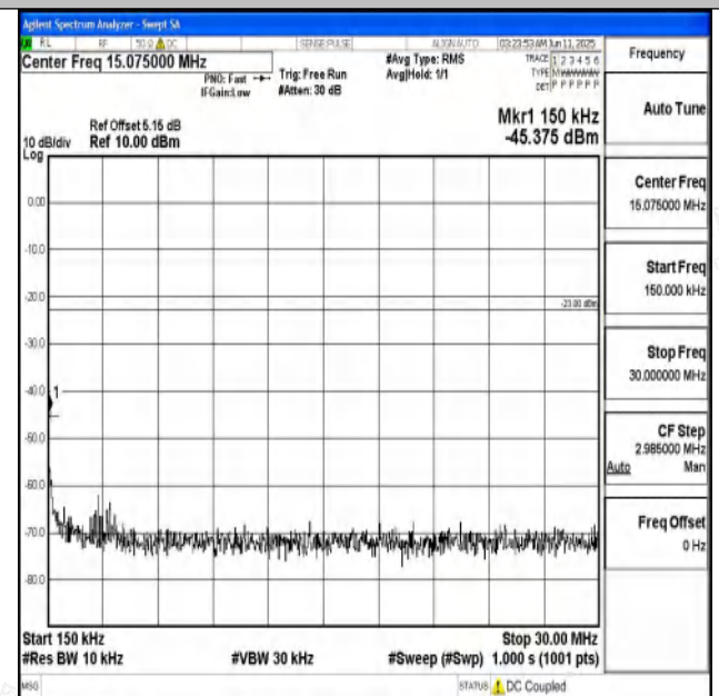
Band71_20MHz_QPSK_133372_1RB#0_0.15~30_0.15~30
