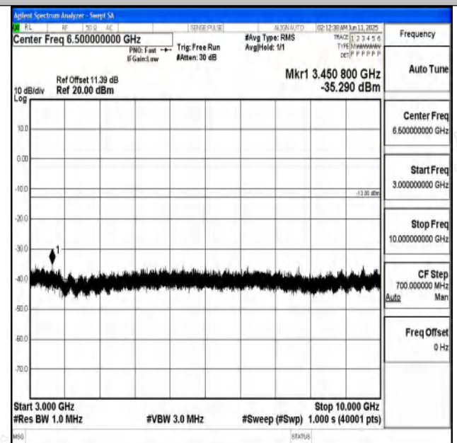
Band71_5MHz_16QAM_133297_1RB#0_3000~10000_3000~10000
