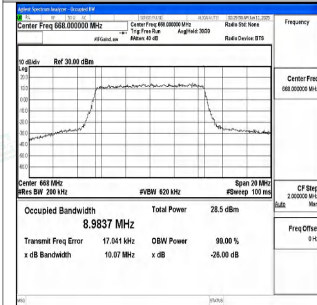
Band71-10MHz-QPSK-133172-50RB#0-PASS
