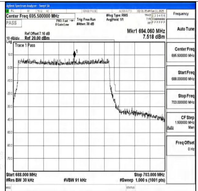
Band71_10MHz_16QAM_133422_50RB#0
