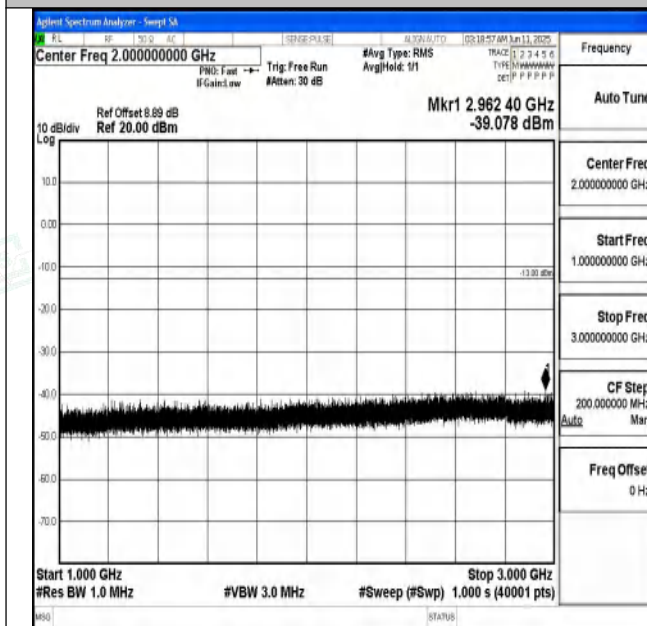
Band71_20MHz_QPSK_133222_1RB#0_1000~3000_1000 ~3000
