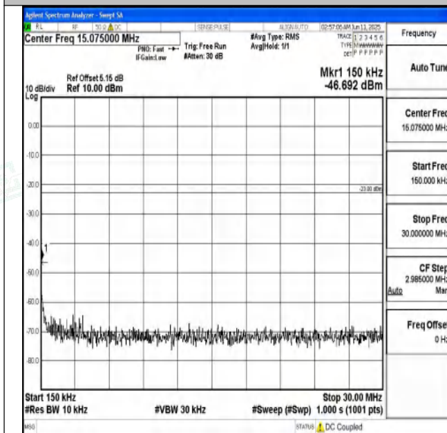
Band71_15MHz_16QAM_133197_1RB#0_0.15~30_0.15~30
