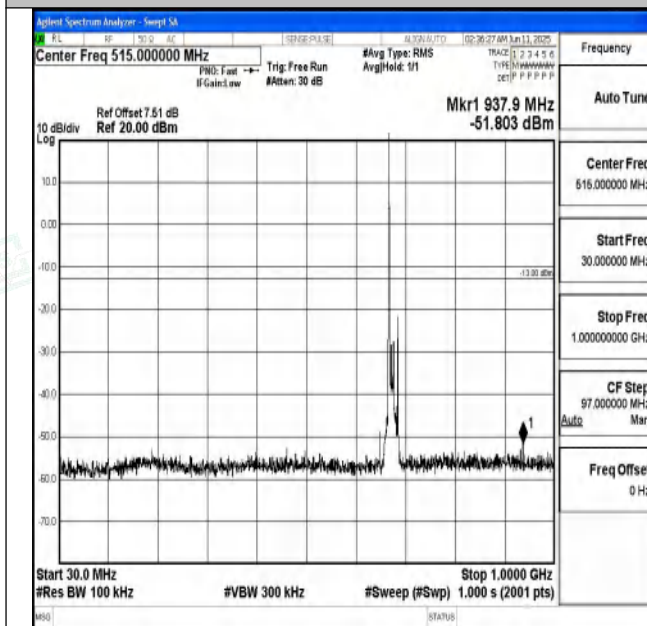
Band71_10MHz_16QAM_133297_1RB#0_30~1000_30~10 00
