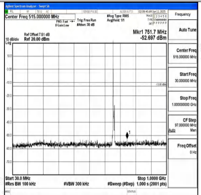
Band71_5MHz_16QAM_133147_1RB#0_30~1000_30~100 0
