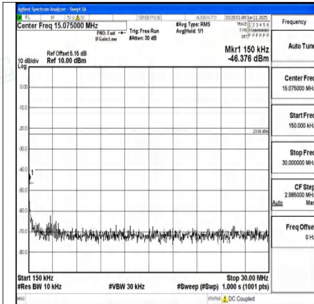
Band71_20MHz_16QAM_133222_1RB#0_0.15~30_0.15~3
