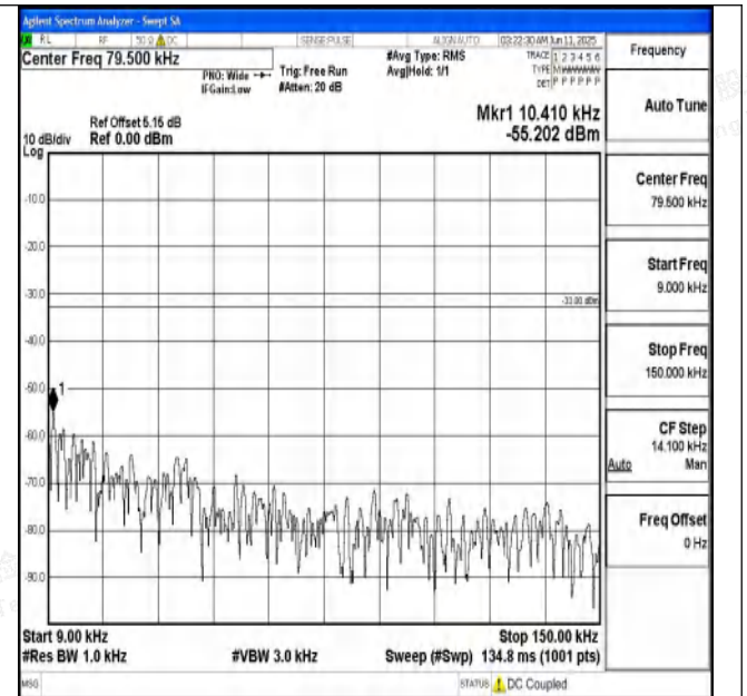
Band71_20MHz_16QAM_133322_1RB#0_0.009~0.15_0.009~0.15
