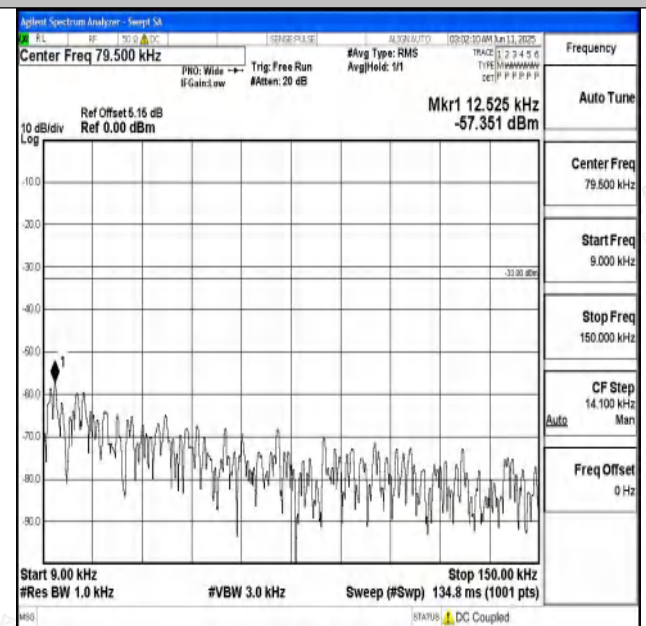
Band71_15MHz_16QAM_133397_1RB#0_0.009~0.15_0.00 9~0.15
