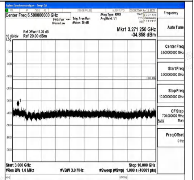
Band71_20MHz_16QAM_133222_1RB#0_3000~10000_3000~10000
