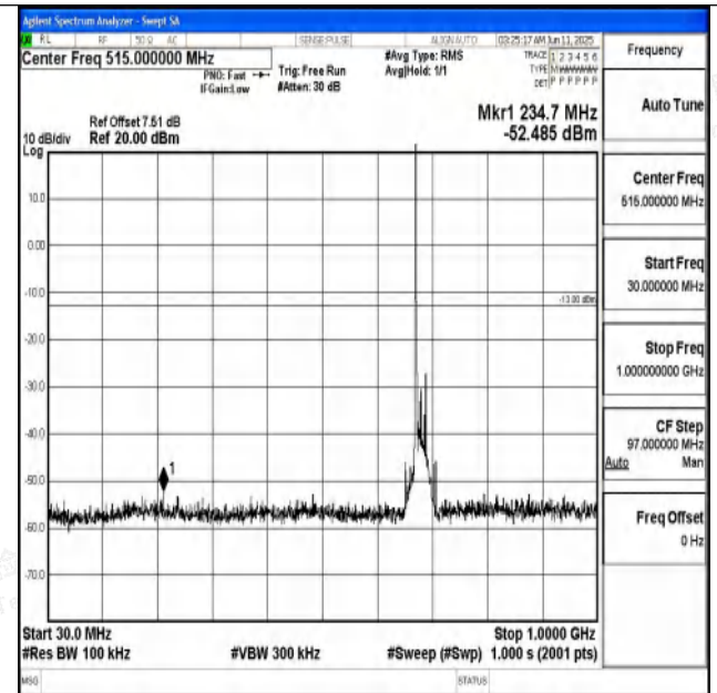
Band71_20MHz_16QAM_133372_1RB#0_30~1000_30~10
