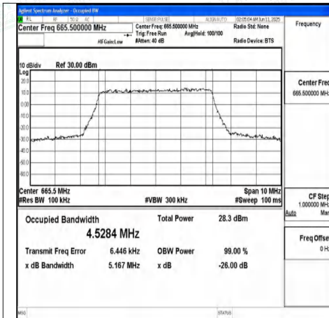
Band71-5MHz-QPSK-133147-25RB#0-PASS
