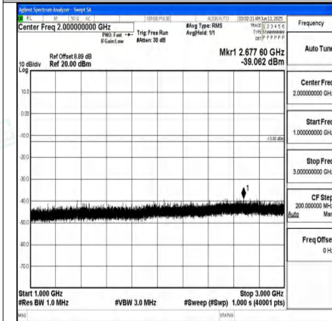
Band71_15MHz_16QAM_133397_1RB#0_1000~3000_1000~3000
