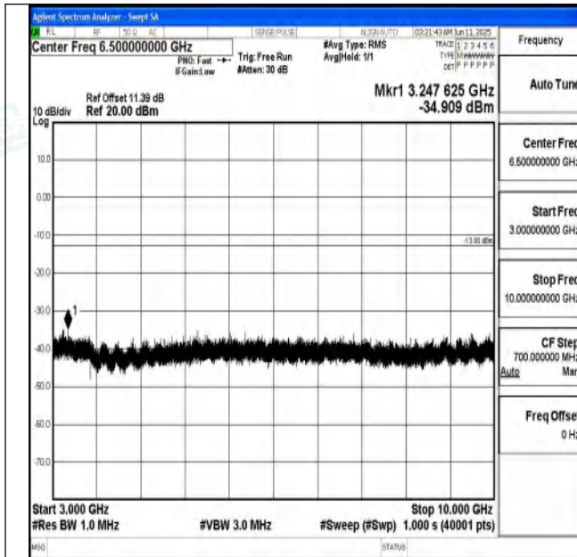
Band71_20MHz_QPSK_133322_1RB#0_3000~10000_3000~10000
