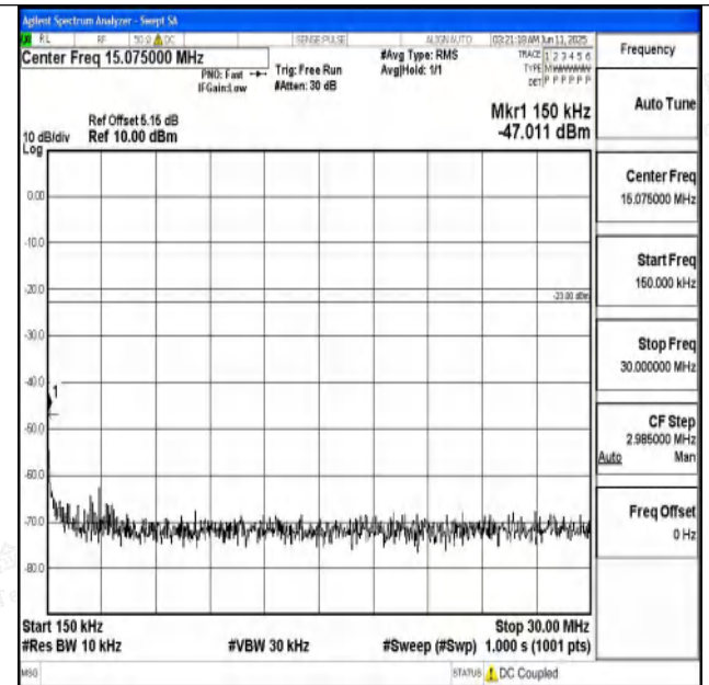
Band71_20MHz_QPSK_133322_1RB#0_0.15~30_0.15~30
