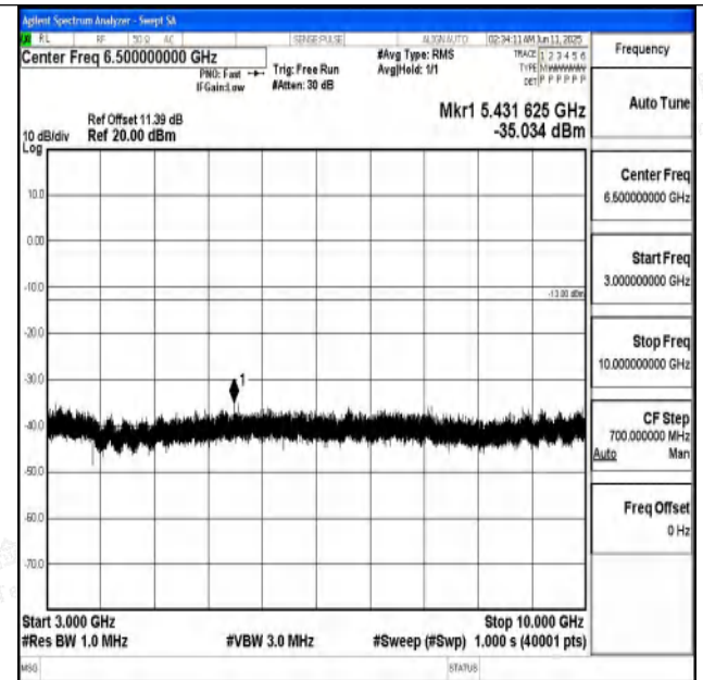
Band71_10MHz_16QAM_133172_1RB#0_3000~10000_30 00~10000
