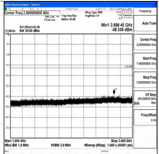
Band71_5MHz_QPSK_133297_1RB#0_1000~3000_1000~3000
