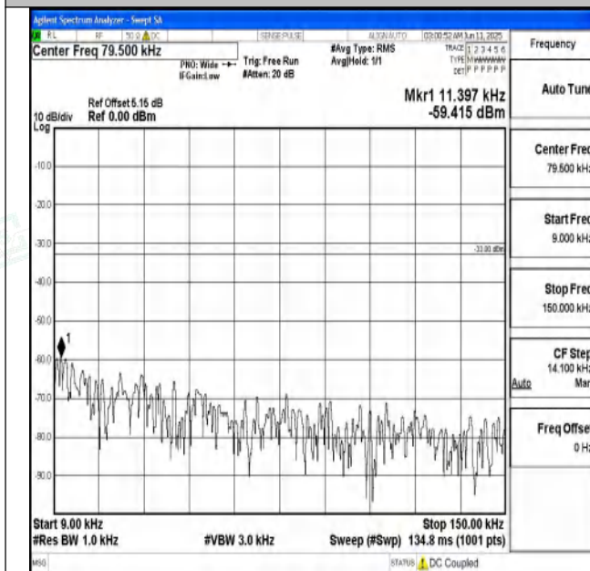
Band71_15MHz_QPSK_133397_1RB#0_0.009~0.15_0.009 ~0.15
