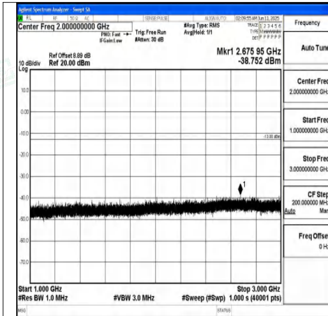
Band71_5MHz_16QAM_133147_1RB#0_1000~3000_1000 ~3000
