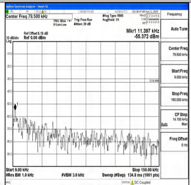
Band71_10MHz_16QAM_133422_1RB#0_0.009~0.15_0.009
