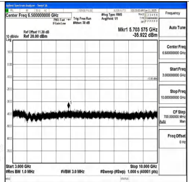
Band71_20MHz_16QAM_133322_1RB#0_3000~10000_30 00~10000
