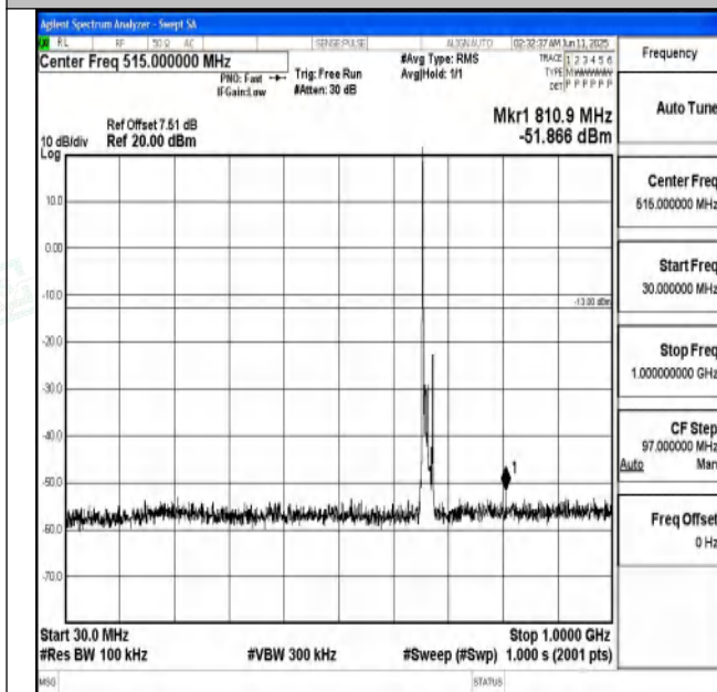
Band71_10MHz_QPSK_133172_1RB#0_30~1000_30~100 0
