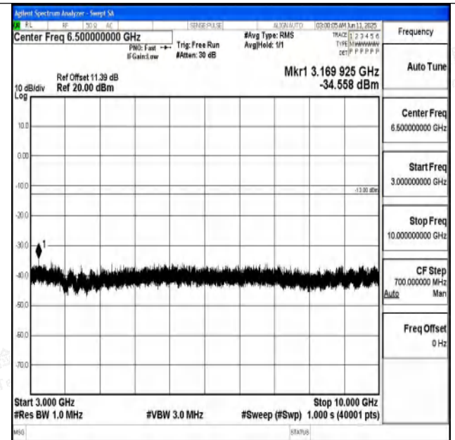
Band71_15MHz_16QAM_133297_1RB#0_3000~10000_30 00~10000
