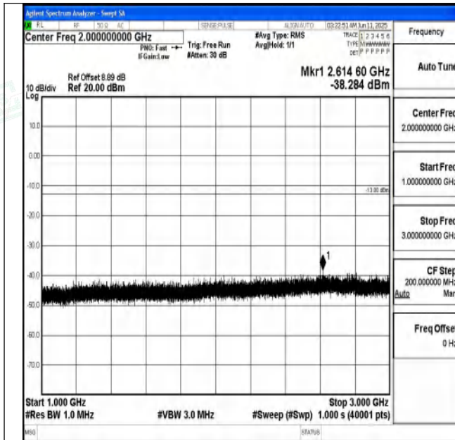
Band71_20MHz_16QAM_133322_1RB#0_1000~3000_100 0~3000
