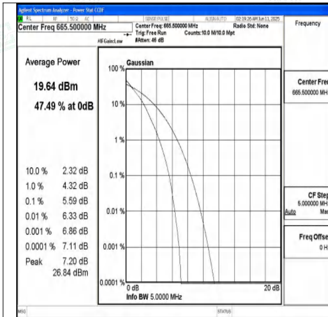
Band71-5MHz-QPSK-133147-25RB#0-PASS
