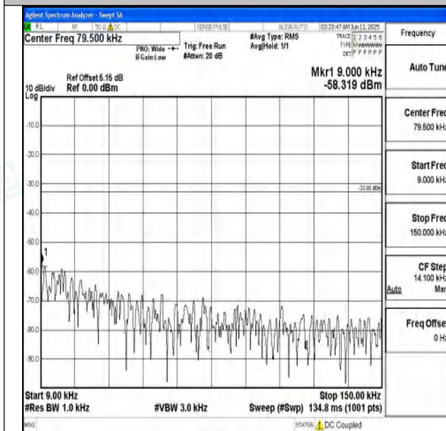
Band71_20MHz_QPSK_133372_1RB#0_0.009~0.15_0.009 ~0.15
