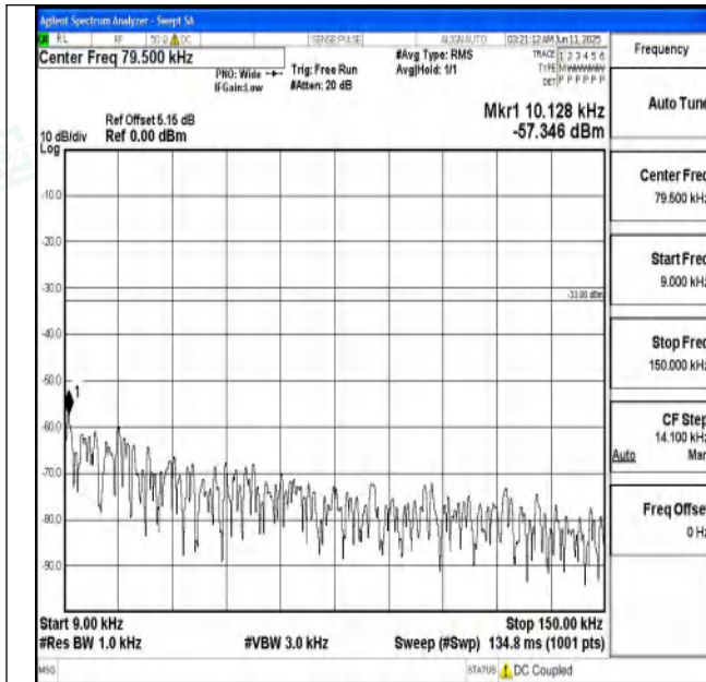
Band71_20MHz_QPSK_133322_1RB#0_0.009~0.15_0.009 ~0.15
