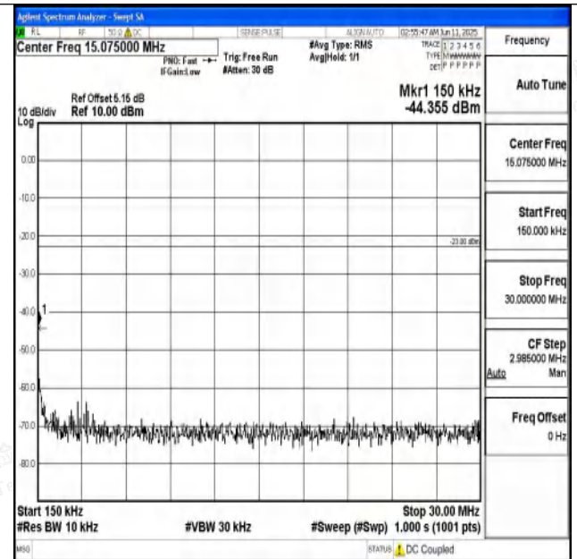
Band71_15MHz_QPSK_133197_1RB#0_0.15~30_0.15~30
