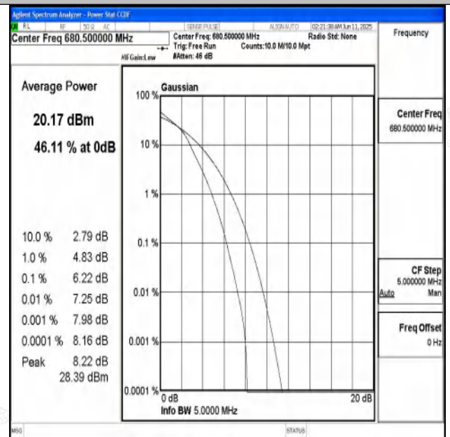
Band71-5MHz-16QAM-133297-25RB#0-PASS
