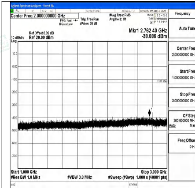
Band71_15MHz_16QAM_133297_1RB#0_1000~3000_100 0~3000
