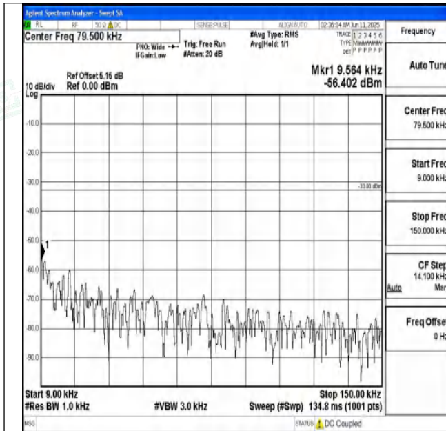
Band71_10MHz_16QAM_133297_1RB#0_0.009~0.15_0.00 9~0.15
