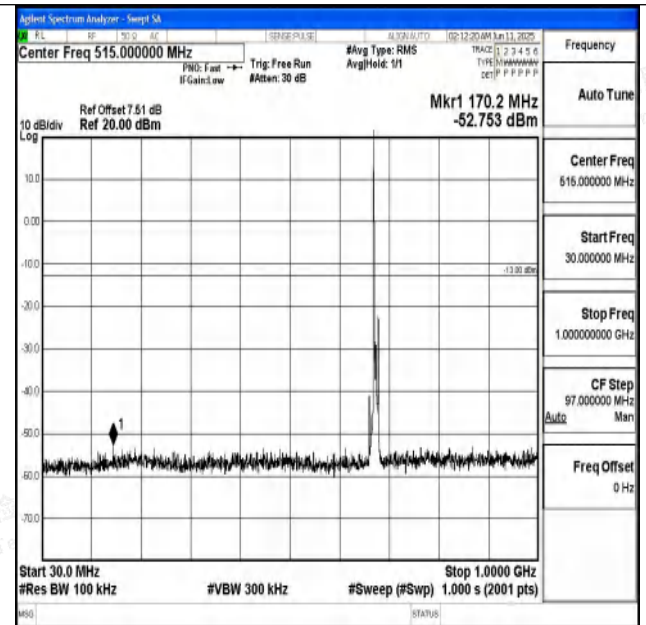
Band71_5MHz_16QAM_133297_1RB#0_30~1000_30~100
