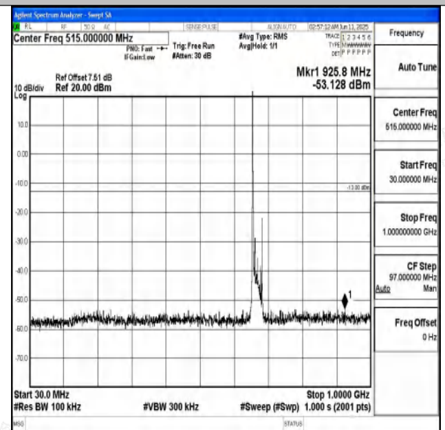
Band71_15MHz_16QAM_133197_1RB#0_30~1000_30~1000
