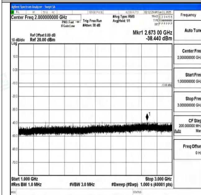
Band71_5MHz_16QAM_133297_1RB#0_1000~3000_1000~3000
