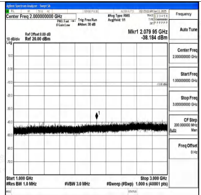
Band71_5MHz_16QAM_133447_1RB#0_1000~3000_1000~3000
