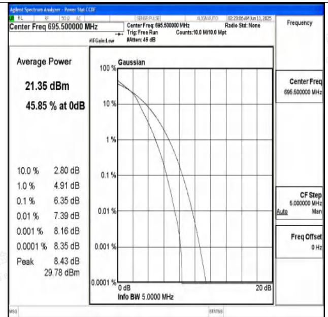
Band71-5MHz-16QAM-133447-25RB#0-PASS
