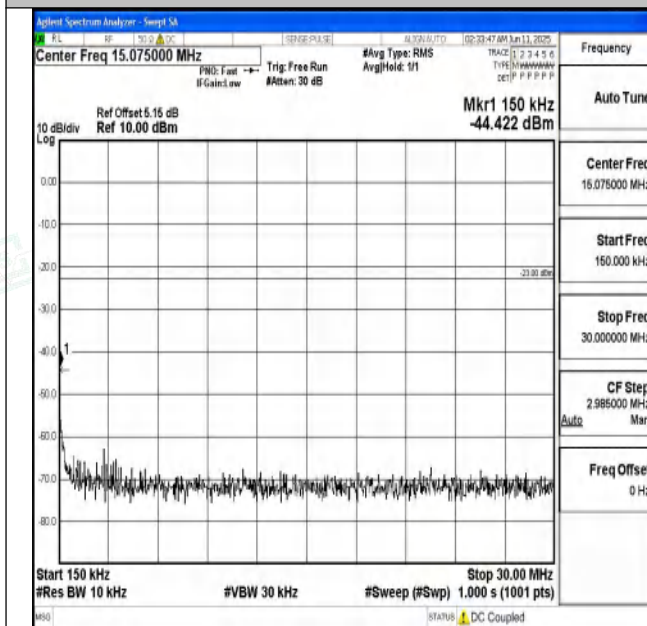
Band71_10MHz_16QAM_133172_1RB#0_0.15~30_0.15~30
