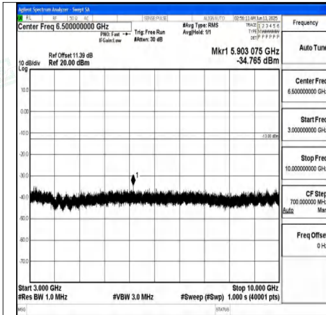
Band71_15MHz_QPSK_133197_1RB#0_3000~10000_3000~10000
