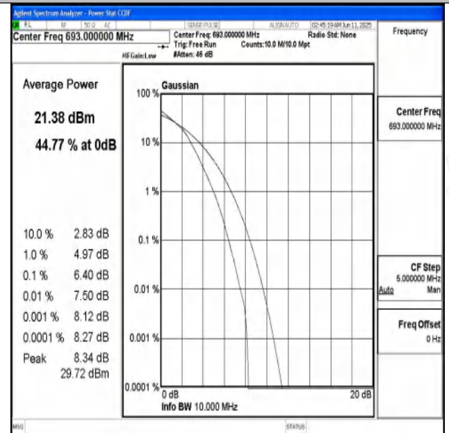
Band71-10MHz-16QAM-133422-50RB#0-PASS
