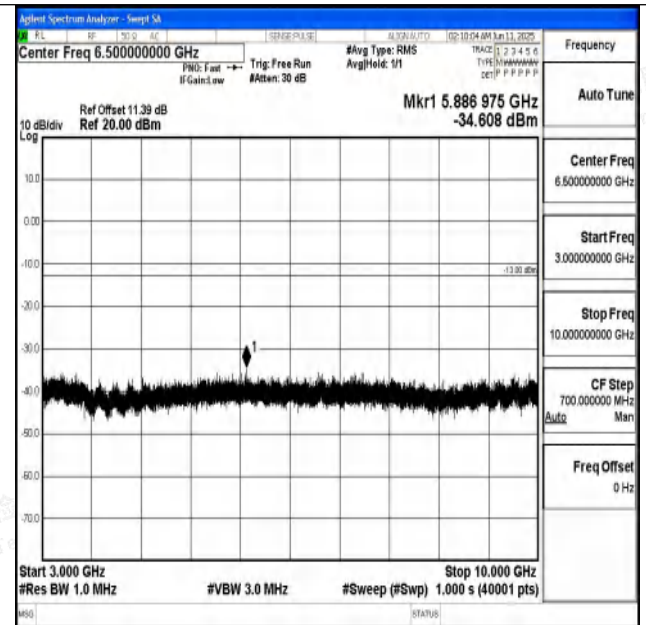
Band71_5MHz_16QAM_133147_1RB#0_3000~10000_300 0~10000
