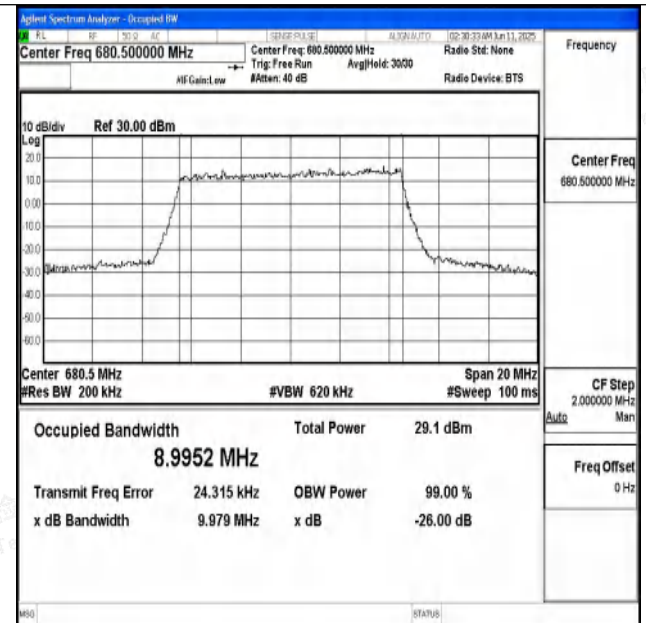
Band71-10MHz-16QAM-133297-50RB#0-PASS
