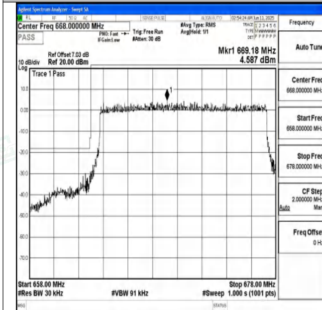
Band71_15MHz_QPSK_133197_75RB#0
