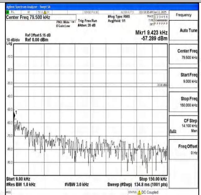
Band71_20MHz_QPSK_133222_1RB#0_0.009~0.15_0.009 ~0.15
