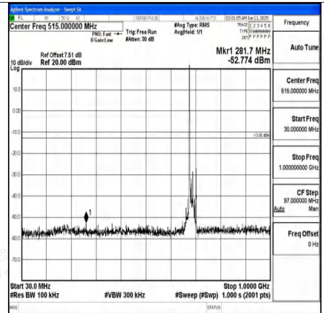
Band71_15MHz_QPSK_133397_1RB#0_30~1000_30~100 0
