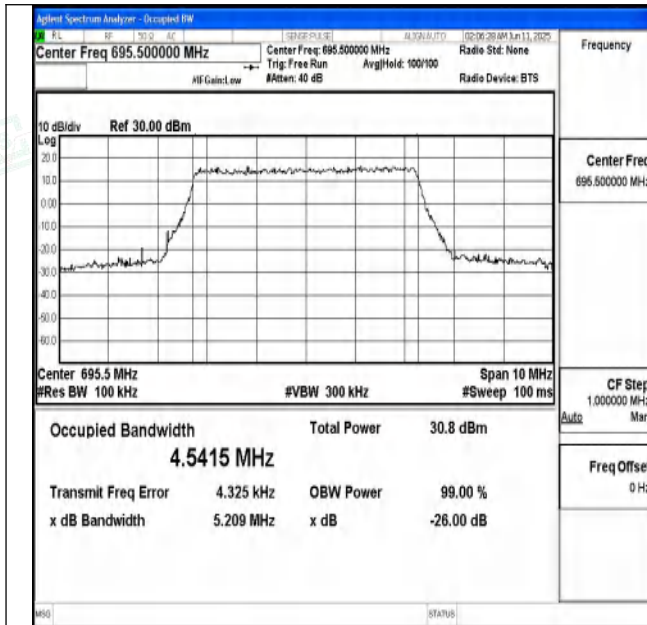
Band71-5MHz-QPSK-133447-25RB#0-PASS
