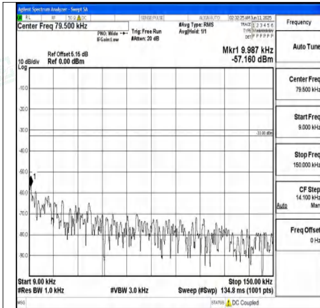
Band71_10MHz_QPSK_133172_1RB#0_0.009~0.15_0.009 ~0.15
