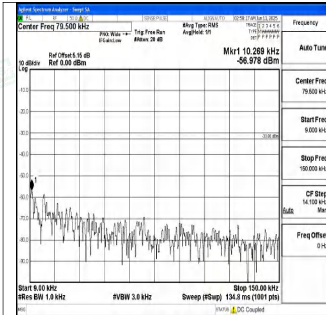
Band71_15MHz_QPSK_133297_1RB#0_0.009~0.15_0.009 ~0.15
