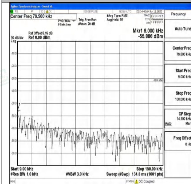
Band71_5MHz_16QAM_133447_1RB#0_0.009~0.15_0.009
