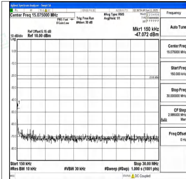
Band71_10MHz_16QAM_133422_1RB#0_0.15~30_0.15~3
