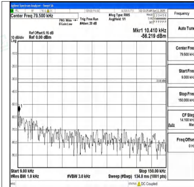
Band71_5MHz_QPSK_133447_1RB#0_0.009~0.15_0.009~0.15
