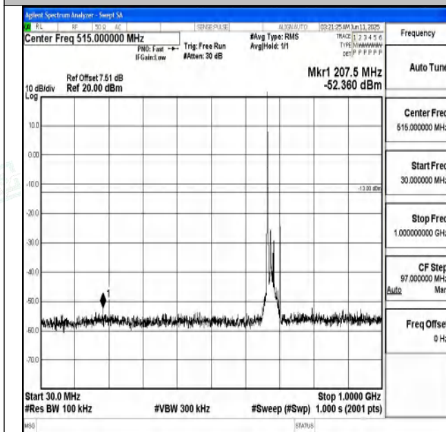
Band71_20MHz_QPSK_133322_1RB#0_30~1000_30~100 0
