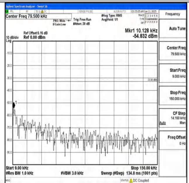
Band71_20MHz_16QAM_133372_1RB#0_0.009~0.15_0.009~0.15
