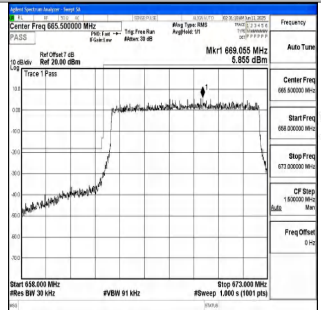
Band71_10MHz_16QAM_133172_50RB#0
