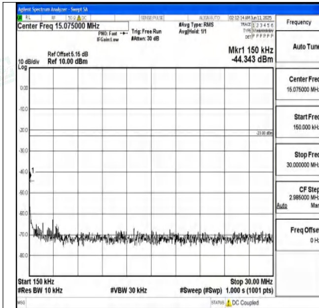
Band71_5MHz_16QAM_133297_1RB#0_0.15~30_0.15~30
