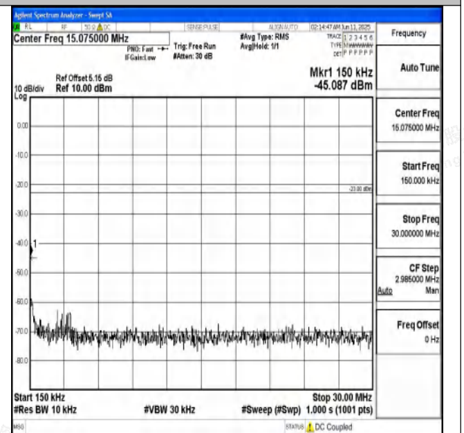
Band71_5MHz_16QAM_133447_1RB#0_0.15~30_0.15~30
