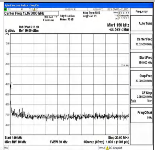
Band71_5MHz_QPSK_133297_1RB#0_0.15~30_0.15~30
