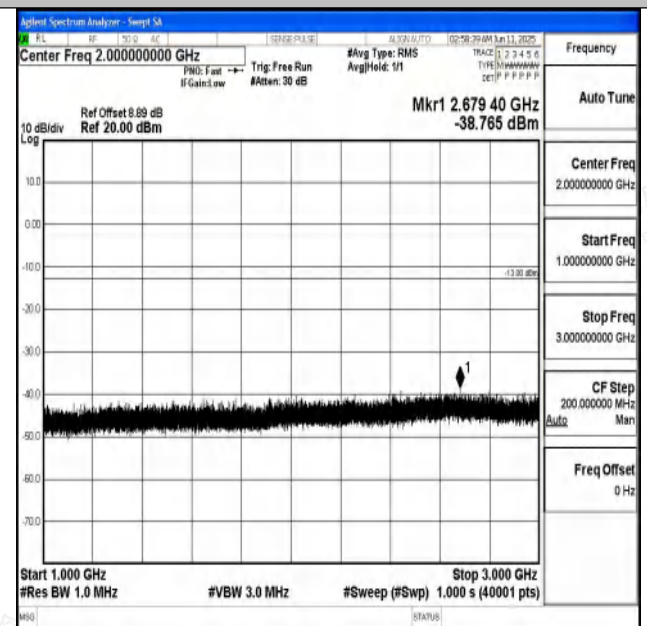
Band71_15MHz_QPSK_133297_1RB#0_1000~3000_1000 ~3000
