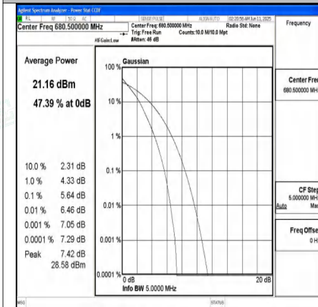
Band71-5MHz-QPSK-133297-25RB#0-PASS
