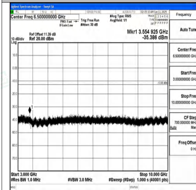
Band71_5MHz_16QAM_133447_1RB#0_3000~10000_3000~10000
