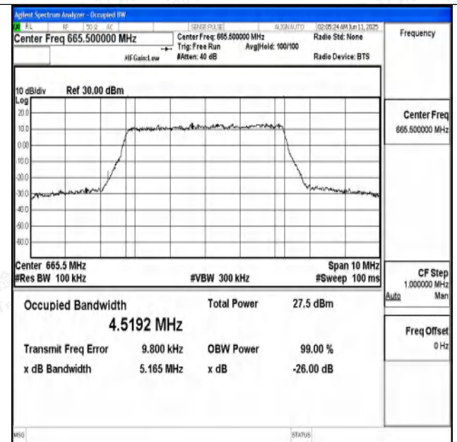
Band71-5MHz-16QAM-133147-25RB#0-PASS
