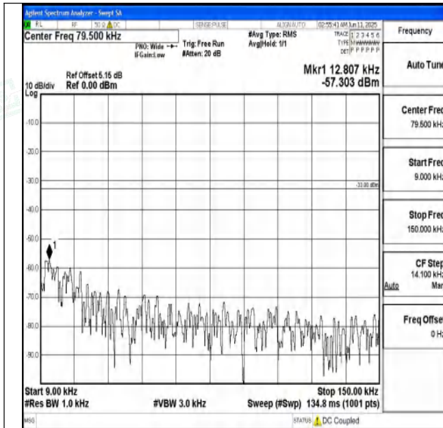
Band71_15MHz_QPSK_133197_1RB#0_0.009~0.15_0.009 ~0.15
