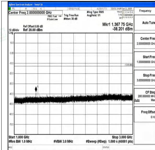
Band71_15MHz_QPSK_133397_1RB#0_1000~3000_1000 ~3000
