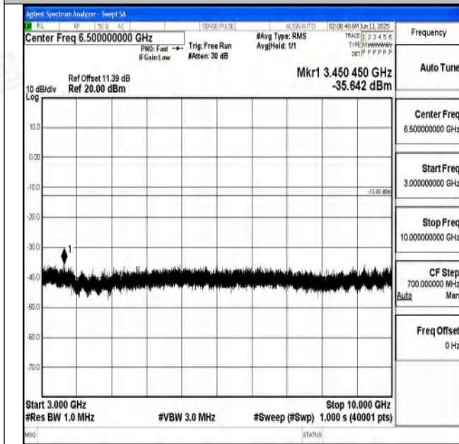
Band71_5MHz_QPSK_133147_1RB#0_3000~10000_3000 ~10000
