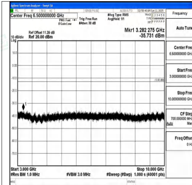
Band71_15MHz_QPSK_133297_1RB#0_3000~10000_3000~10000
