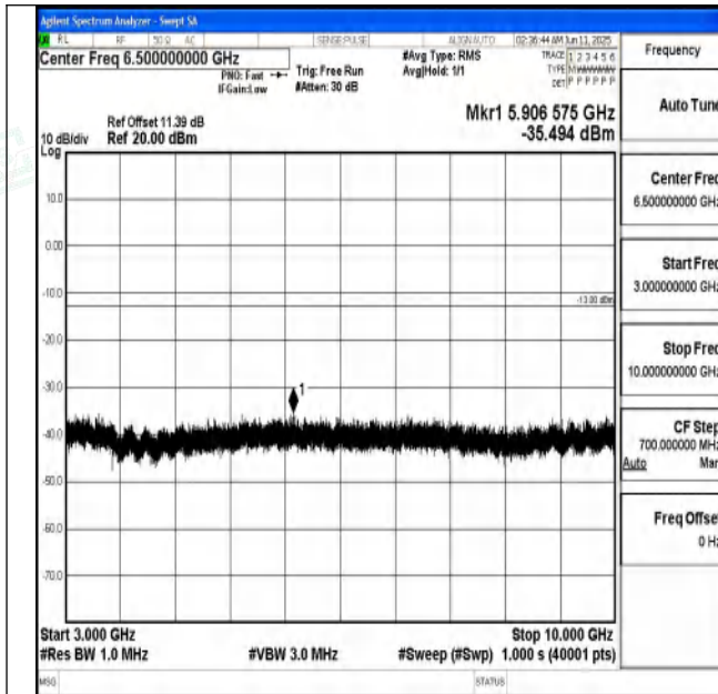
Band71_10MHz_16QAM_133297_1RB#0_3000~10000_30 00~10000
