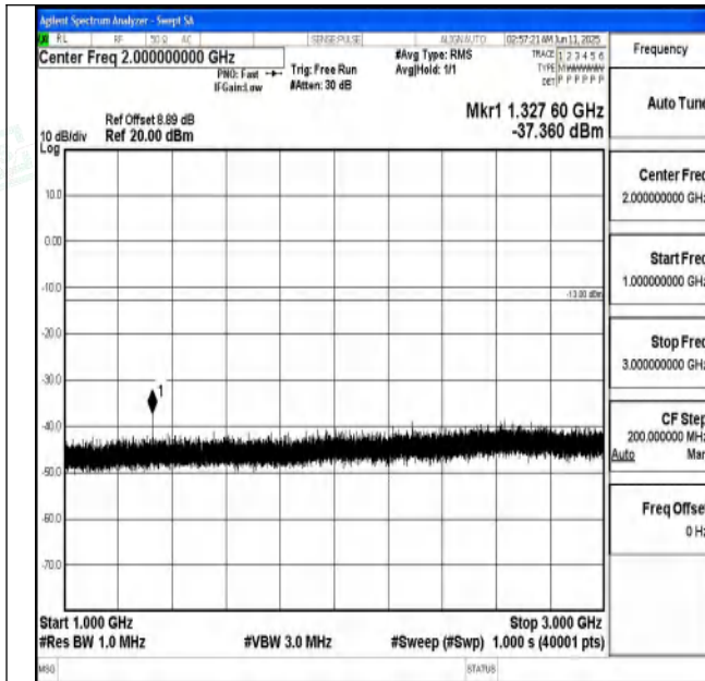
Band71_15MHz_16QAM_133197_1RB#0_1000~3000_100 0~3000
