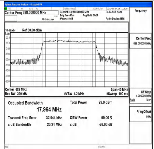
Band71-20MHz-16QAM-133372-100RB#0-PASS
