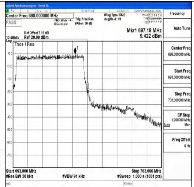
Band71_5MHz_16QAM_133447_25RB#0
