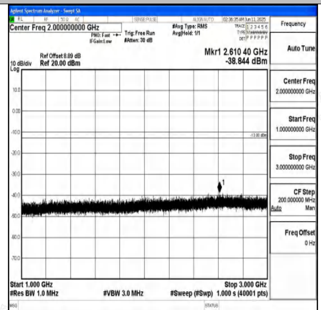
Band71_10MHz_16QAM_133297_1RB#0_1000~3000_100 0~3000
