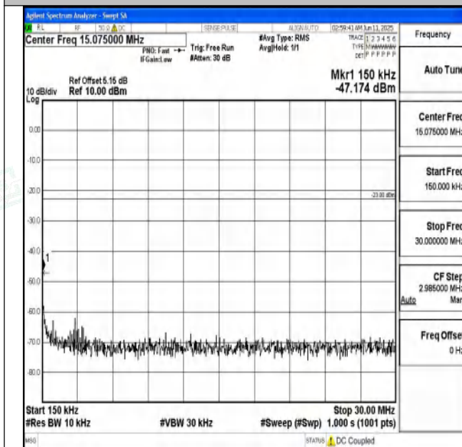
Band71_15MHz_16QAM_133297_1RB#0_0.15~30_0.15~30 0
