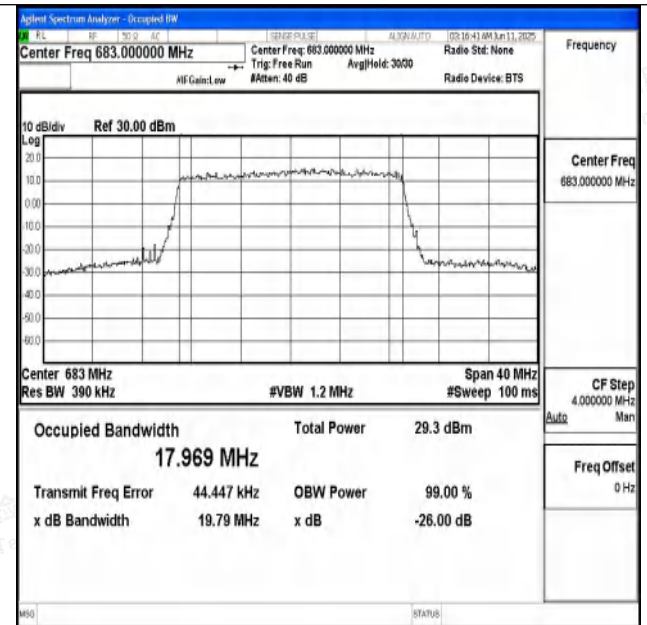
Band71-20MHz-16QAM-133322-100RB#0-PASS
