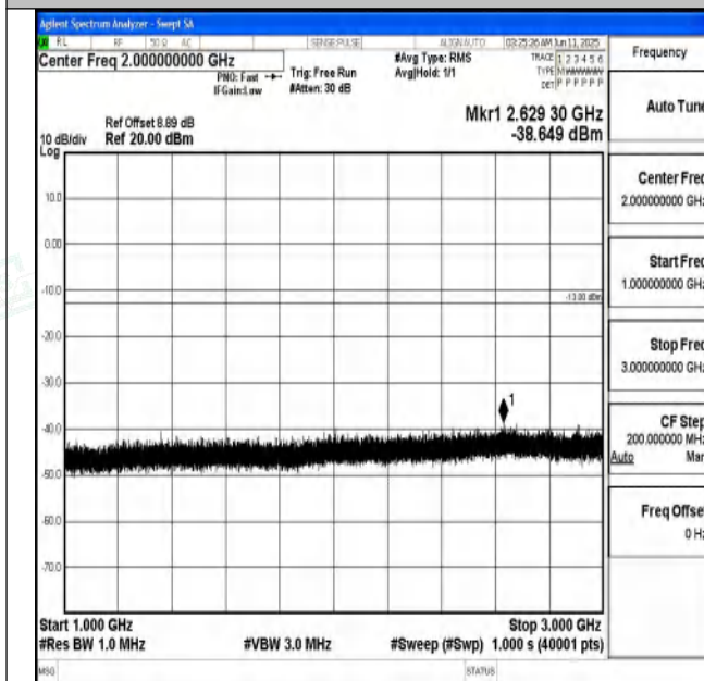
Band71_20MHz_16QAM_133372_1RB#0_1000~3000_1000~3000
