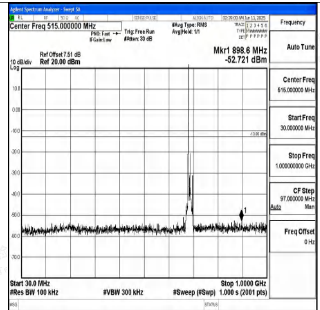
Band71_10MHz_16QAM_133422_1RB#0_30~1000_30~10 00
