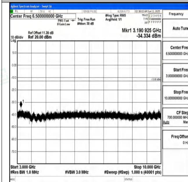
Band71_10MHz_QPSK_133422_1RB#0_3000~10000_3000
