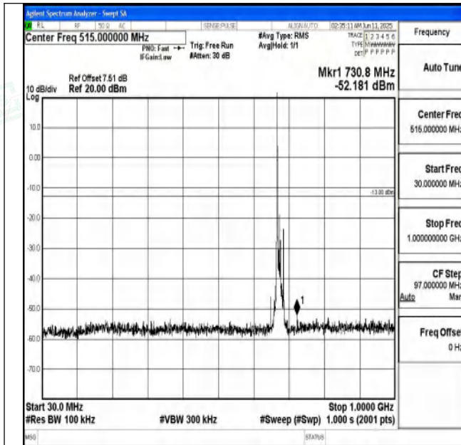
Band71_10MHz_QPSK_133297_1RB#0_30~1000_30~100
