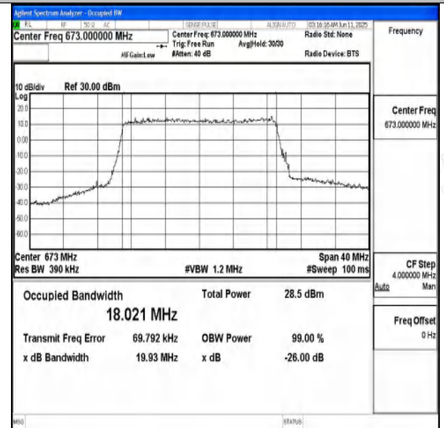
Band71-20MHz-16QAM-133222-100RB#0-PASS
