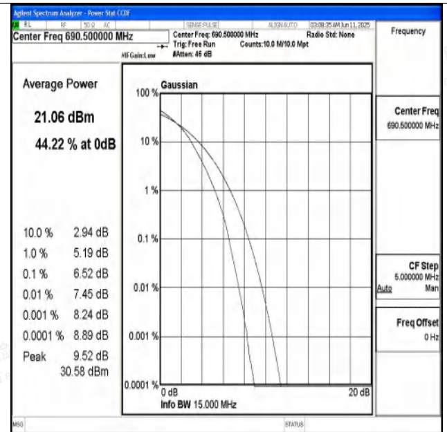
Band71-15MHz-16QAM-133397-75RB#0-PASS
