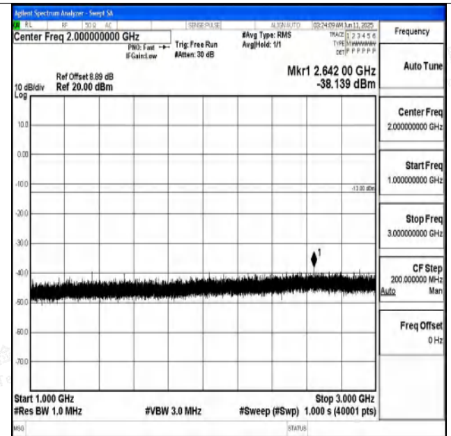
Band71_20MHz_QPSK_133372_1RB#0_1000~3000_1000~3000
