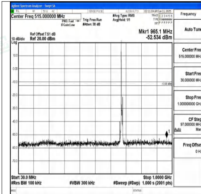
Band71_5MHz_QPSK_133297_1RB#0_30~1000_30~1000
