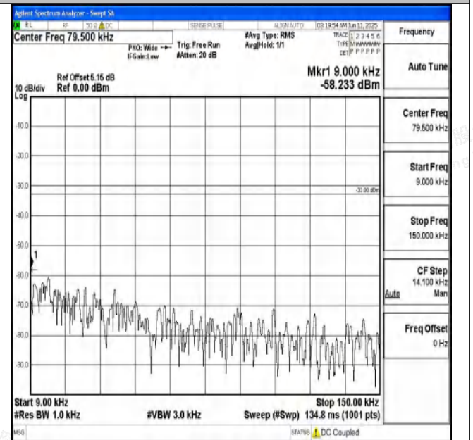
Band71_20MHz_16QAM_133222_1RB#0_0.009~0.15_0.009~0.15
