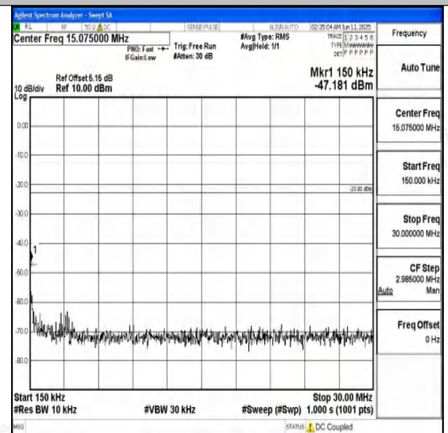
Band71_10MHz_QPSK_133297_1RB#0_0.15~30_0.15~30
