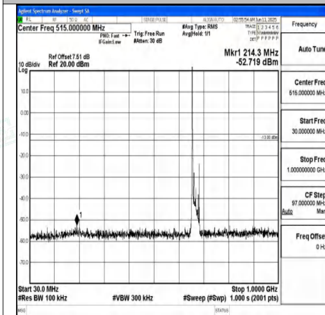
Band71_15MHz_QPSK_133197_1RB#0_30~1000_30~100 0
