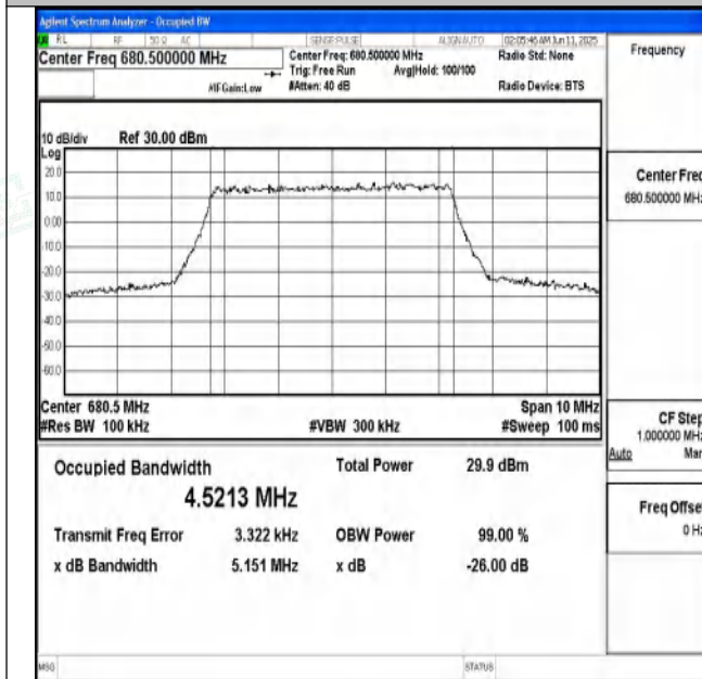
Band71-5MHz-QPSK-133297-25RB#0-PASS
