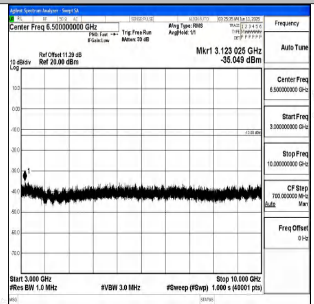
Band71_20MHz_16QAM_133372_1RB#0_3000~10000_3000~10000
