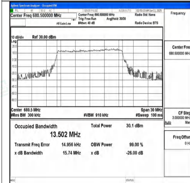
Band71-15MHz-QPSK-133297-75RB#0-PASS
