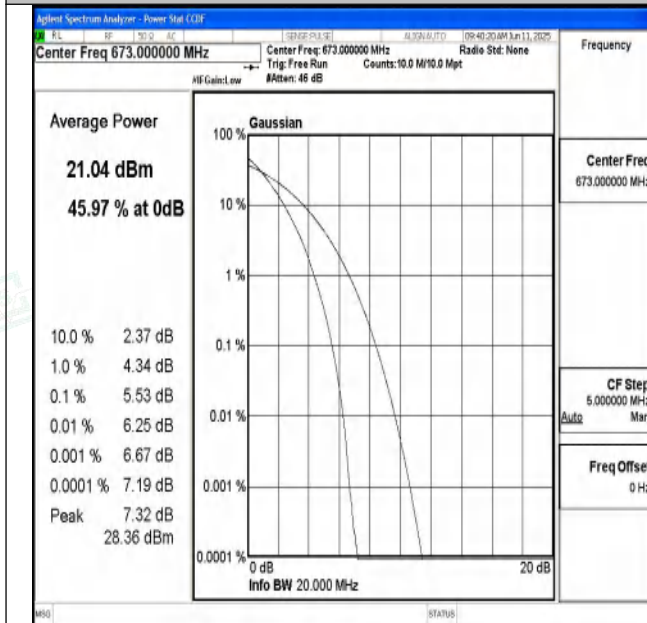
Band71-20MHz-QPSK-133222-100RB#0-PASS
