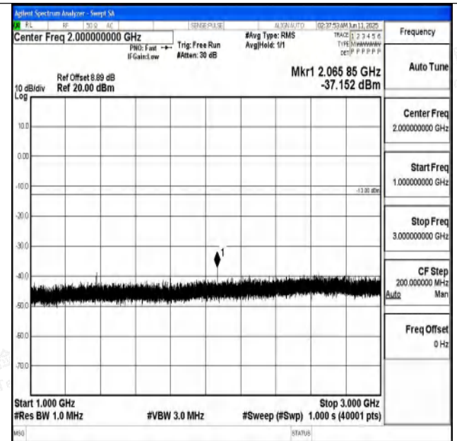
Band71_10MHz_QPSK_133422_1RB#0_1000~3000_1000
