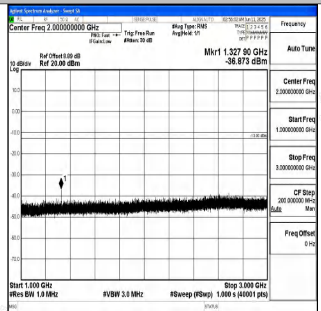
Band71_15MHz_QPSK_133197_1RB#0_1000~3000_1000 ~3000
