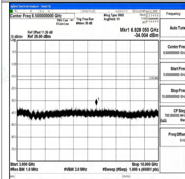
Band71_5MHz_QPSK_133297_1RB#0_3000~10000_3000~10000
