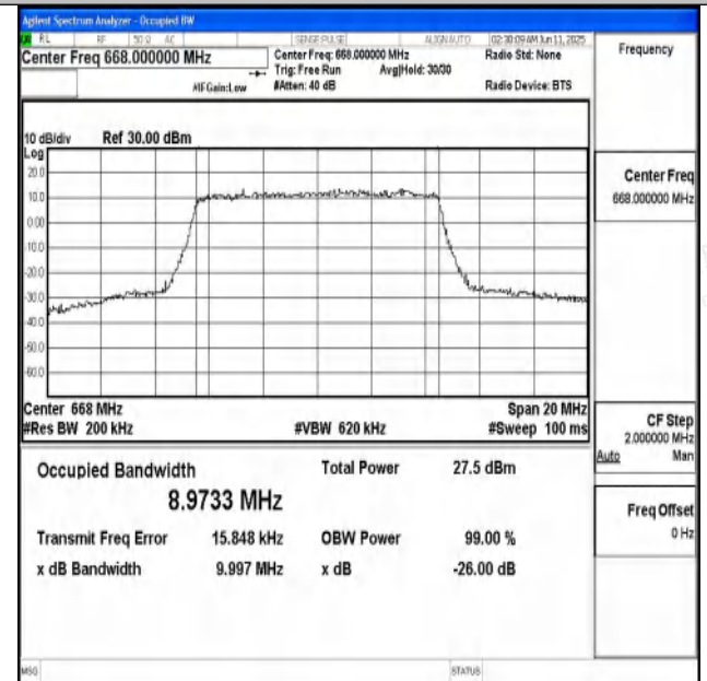
Band71-10MHz-16QAM-133172-50RB#0-PASS
