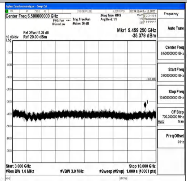
Band71_10MHz_16QAM_133422_1RB#0_3000~10000_30 00~10000
