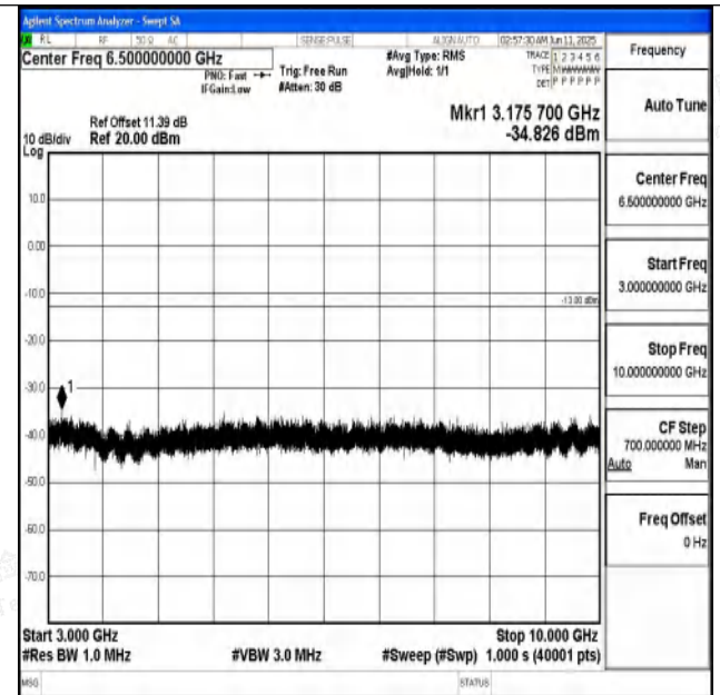
Band71_15MHz_16QAM_133197_1RB#0_3000~10000_30 00~10000
