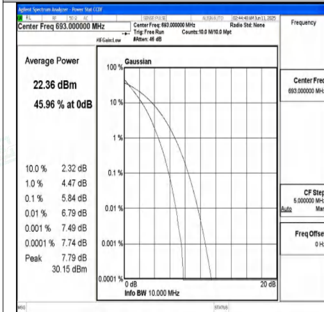
Band71-10MHz-QPSK-133422-50RB#0-PASS
