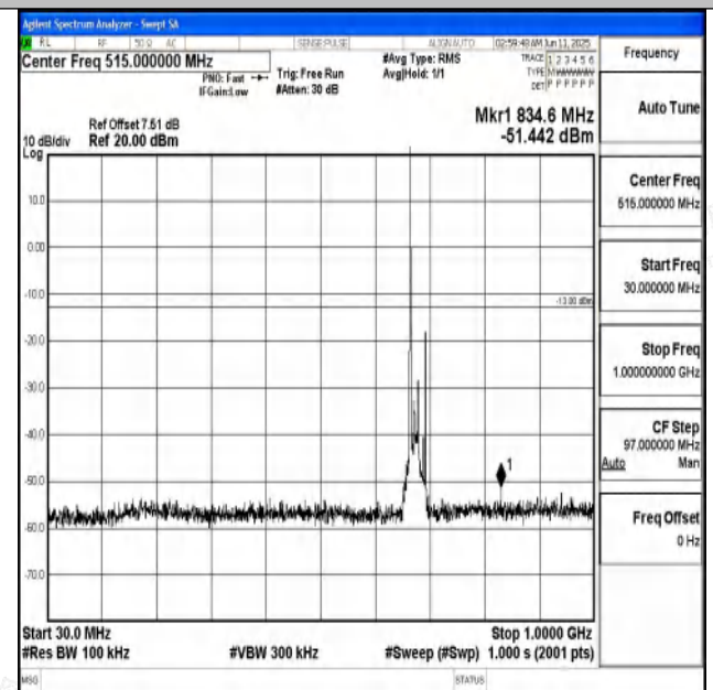
Band71_15MHz_16QAM_133297_1RB#0_30~1000_30~1000 00
