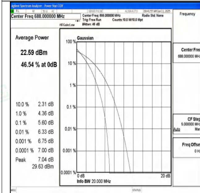
Band71-20MHz-QPSK-133372-100RB#0-PASS
