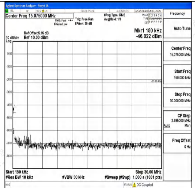
Band71_10MHz_QPSK_133172_1RB#0_0.15~30_0.15~30
