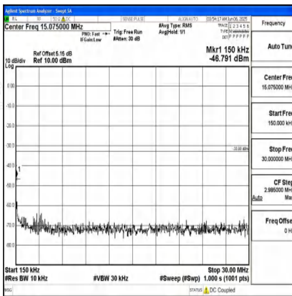
Band66_10MHz_16QAM_132022_1RB#0_0.15~30_0 .15~30
