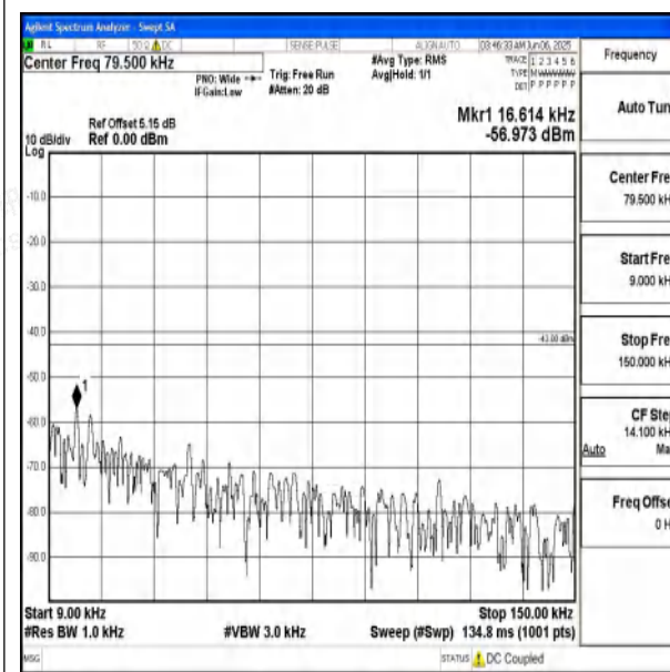
Band66_3MHz_QPSK_132322_1RB#0_0.009~0.15_ 0.009~0.15
