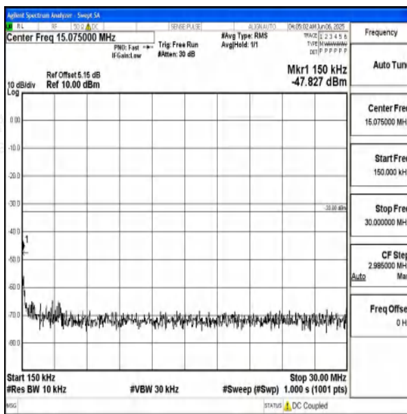
Band66_20MHz_16QAM_132572_1RB#0_0.15~30_0 .15~30
