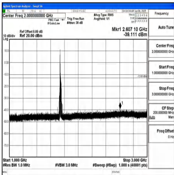
Band66_20MHz_16QAM_132322_1RB#0_1000~3000 0_1000~3000
