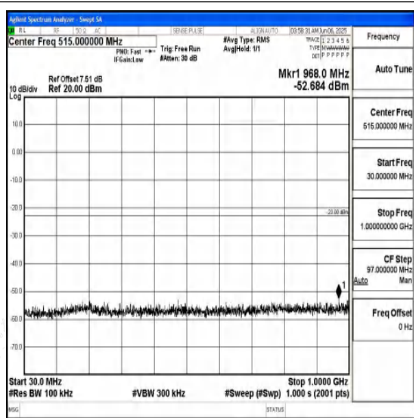
Band66_15MHz_16QAM_132047_1RB#0_30~1000_3 0~1000
