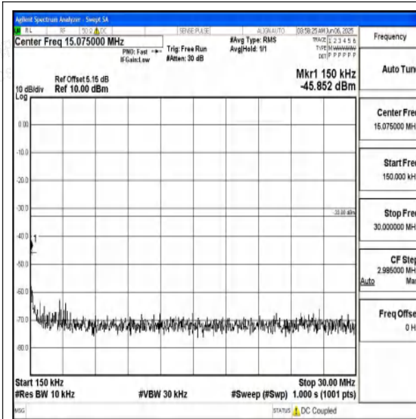
Band66_15MHz_16QAM_132047_1RB#0_0.15~30_0 .15~30
