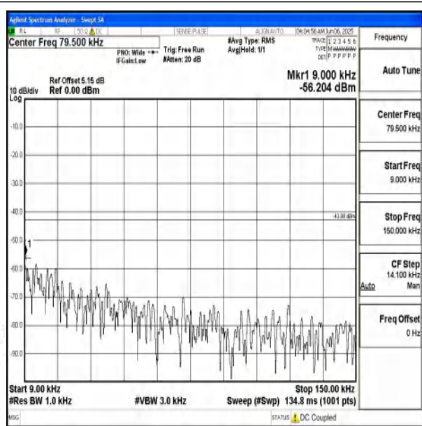
Band66_20MHz_16QAM_132572_1RB#0_0.009~0.15 _0.009~0.15
