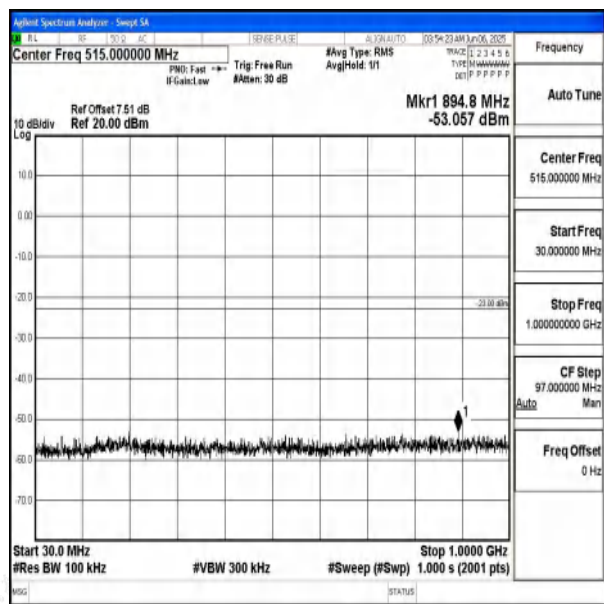
Band66_10MHz_16QAM_132022_1RB#0_30~1000_3 0~1000
