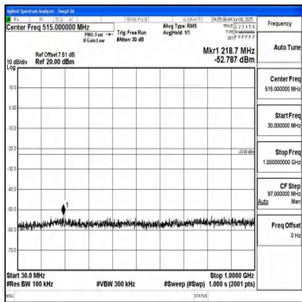
Band66_20MHz_16QAM_132572_1RB#0_30~1000_3 0~1000
