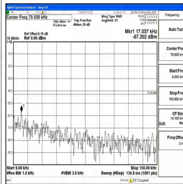
Band66_5MHz_QPSK_131997_1RB#0_0.009~0.15 0.009~0.15
