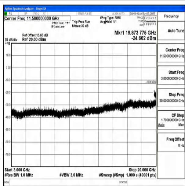
Band66_3MHz_16QAM_132657_1RB#0_3000~20000 _3000~20000
