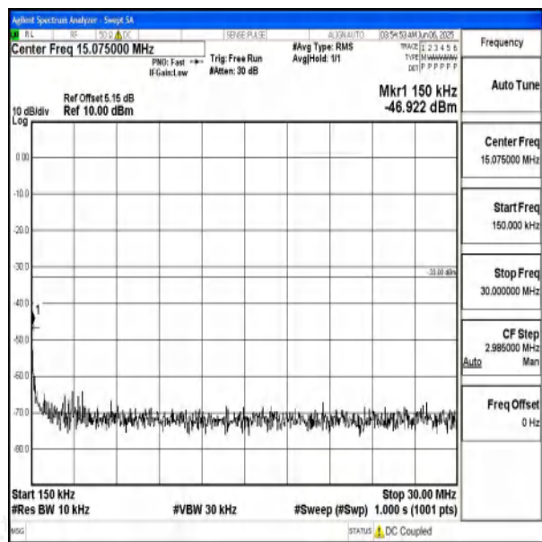
Band66_10MHz_QPSK_132322_1RB#0_0.15~30_0.1 5~30
