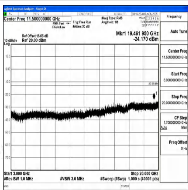
Band66_3MHz_16QAM_131987_1RB#0_3000~20000 _3000~20000
