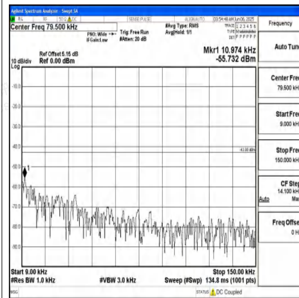
Band66_10MHz_QPSK_132322_1RB#0_0.009~0.15 _0.009~0.15
