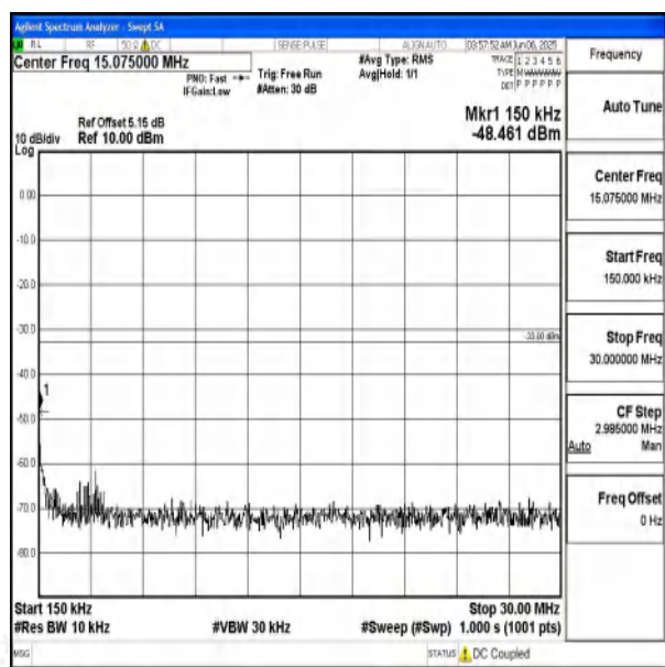
Band66_15MHz_QPSK_132047_1RB#0_0.15~30_0.1 5~30
