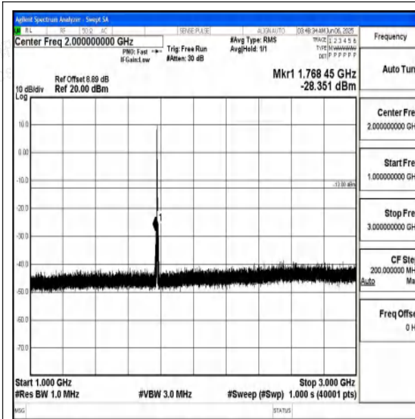
Band66_3MHz_16QAM_132657_1RB#0_1000~3000 _1000~3000
