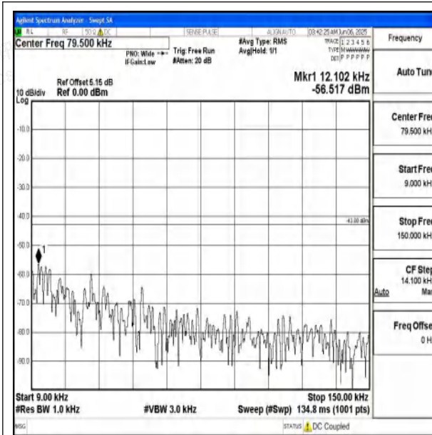
Band66_1.4MHz_QPSK_132322_1RB#0_0.009~0.15 _0.009~0.15
