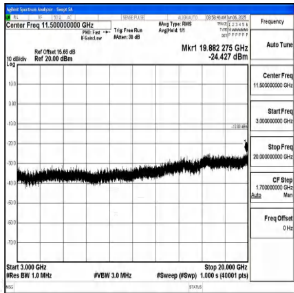
Band66_15MHz_16QAM_132047_1RB#0_3000~2000 0_3000~20000
