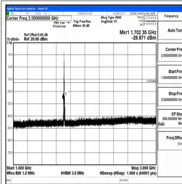
Band66_3MHz_16QAM_131987_1RB#0_1000~3000 _1000~3000
