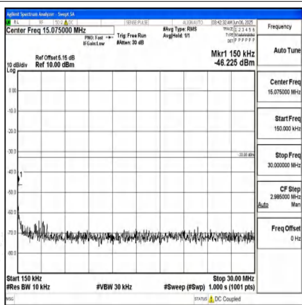
Band66_1.4MHz_QPSK_132322_1RB#0_0.15~30_0.1 5~30
