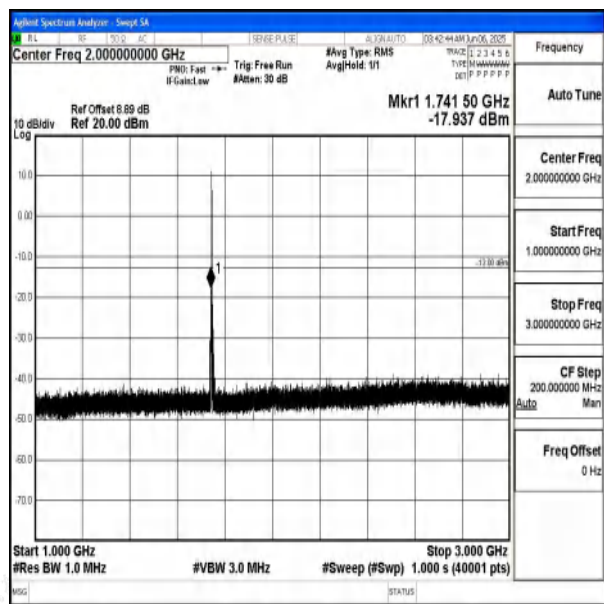
Band66_1.4MHz_QPSK_132322_1RB#0_1000~3000_ 1000~3000
