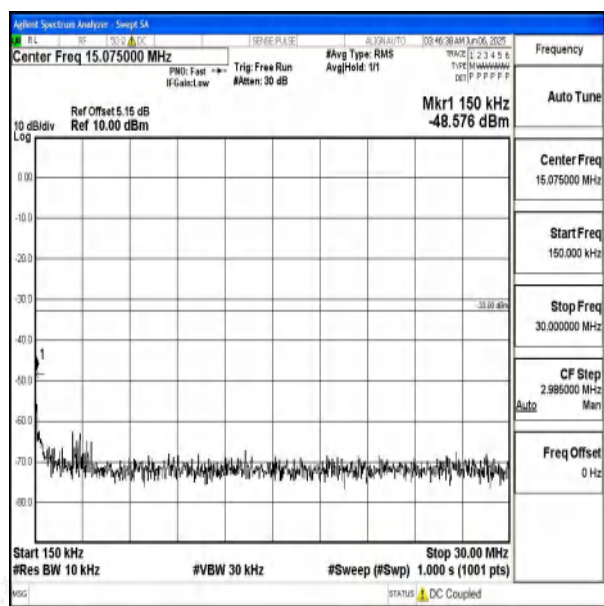
Band66_3MHz_QPSK_132322_1RB#0_0.15~30_0.15 ~30
