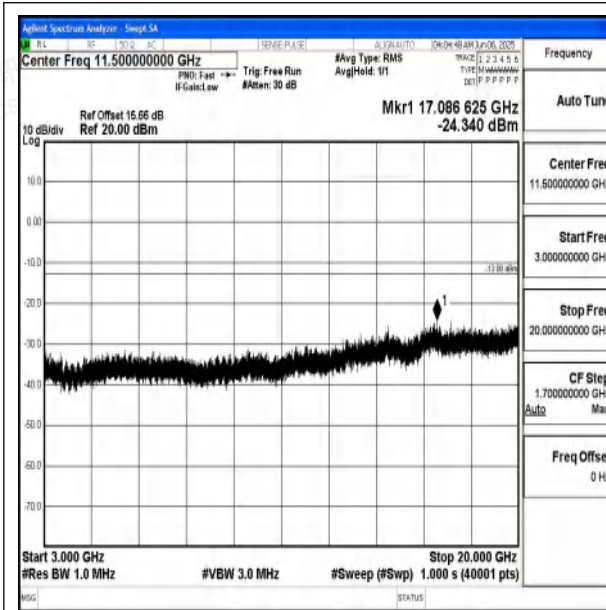
Band66_20MHz_QPSK_132572_1RB#0_3000~2000 0_3000~20000
