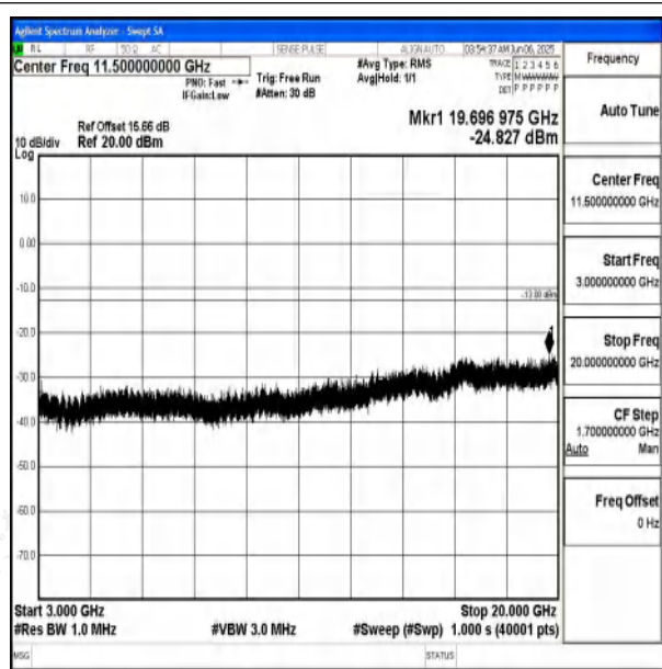
Band66_10MHz_16QAM_132022_1RB#0_3000~2000 0_3000~20000
