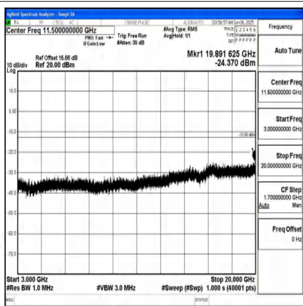
Band66_10MHz_16QAM_132622_1RB#0_3000~2000 0_3000~20000
