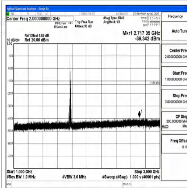
Band66_10MHz_16QAM_132622_1RB#0_1000~3000 0_1000~3000
