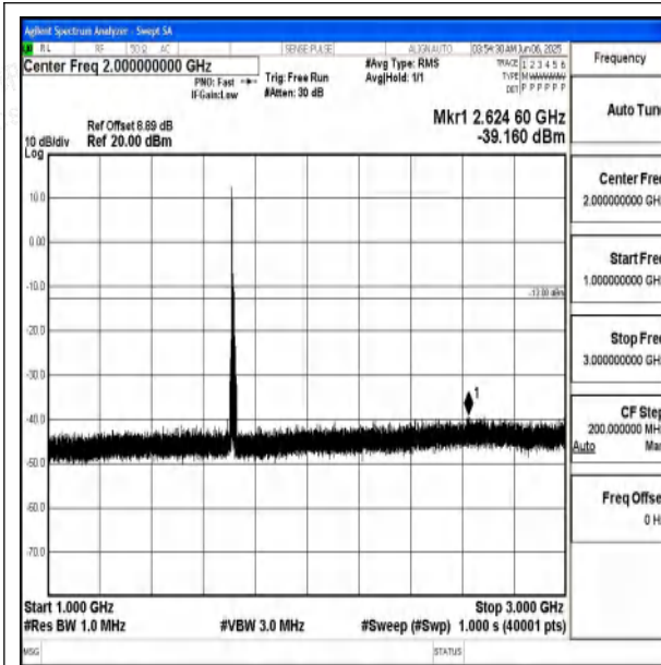
Band66_10MHz_16QAM_132022_1RB#0_1000~3000 0_1000~3000
