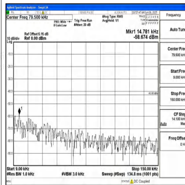
Band66_15MHz_QPSK_132047_1RB#0_0.009~0.15 _0.009~0.15
