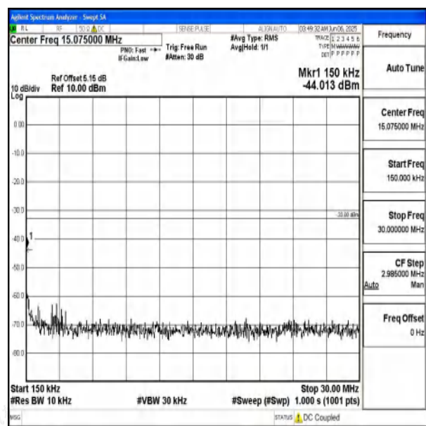
Band66_5MHz_QPSK_131997_1RB#0_0.15~30_0.15 ~30
