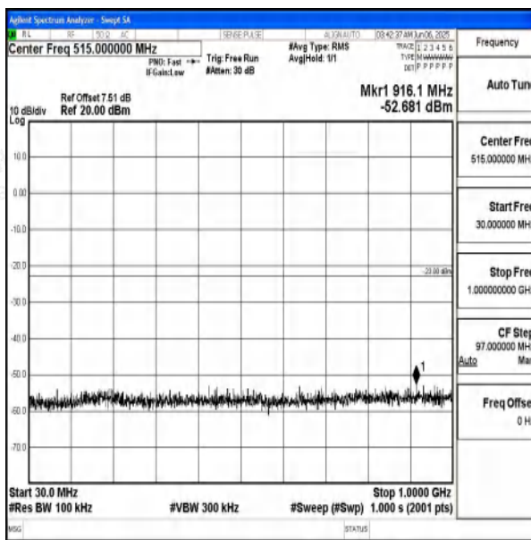
Band66_1.4MHz_QPSK_132322_1RB#0_30~1000_3 0~1000
