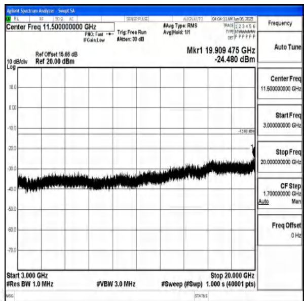
Band66_20MHz_16QAM_132322_1RB#0_3000~2000 0_3000~20000
