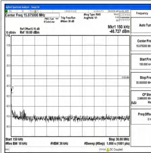
Band66_20MHz_16QAM_132322_1RB#0_0.15~30_0 .15~30
