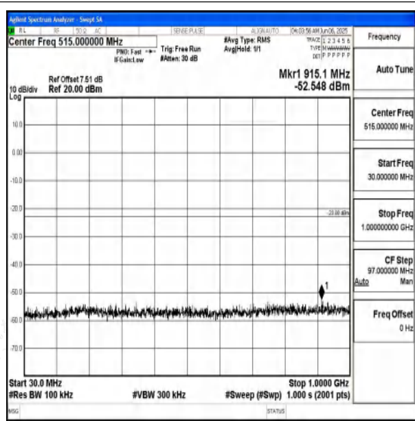
Band66_20MHz_16QAM_132322_1RB#0_30~1000_3 0~1000
