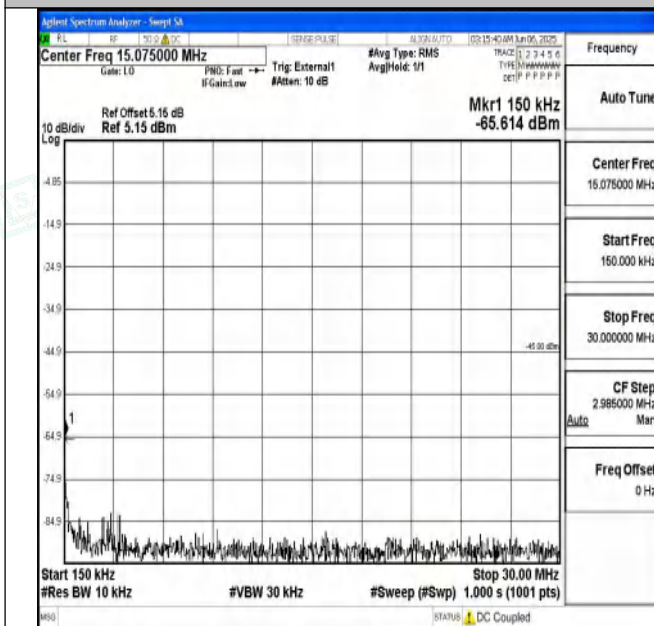
Band41_15MHz_16QAM_39725_1RB#0_0.15~30_0.15~30
