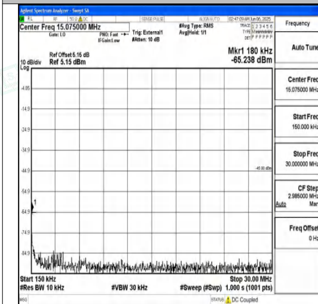
Band41_5MHz_16QAM_39675_1RB#0_0.15~30_0.15~30
