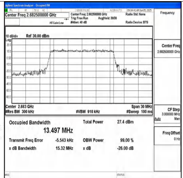
Band41-15MHz-16QAM-41515-75RB#0-PASS
