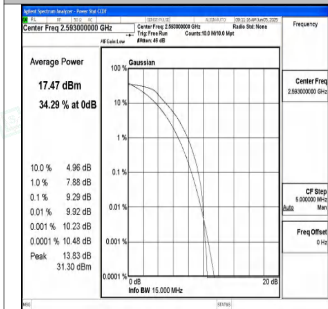
Band41-15MHz-QPSK-40620-75RB#0-PASS
