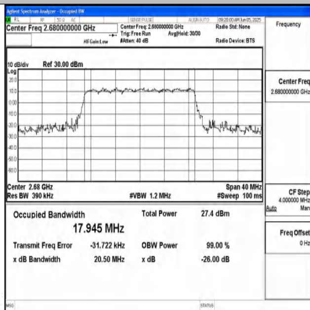
Band41-20MHz-16QAM-41490-100RB#0-PASS
