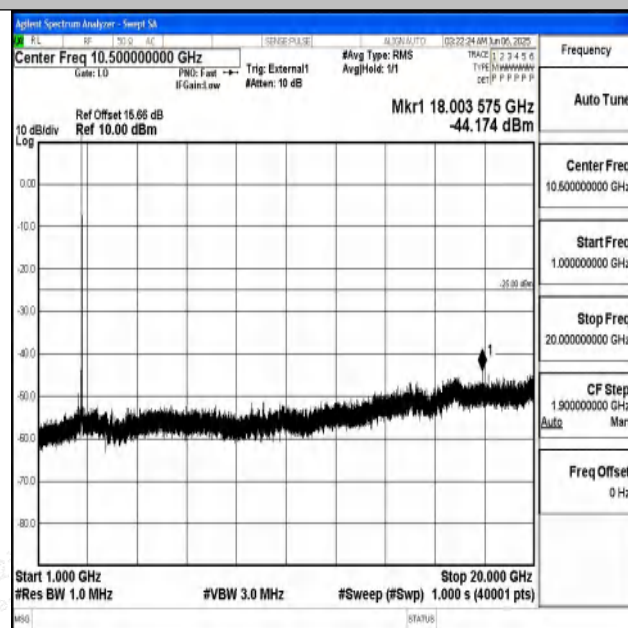
Band41_15MHz_QPSK_41515_1RB#0_1000~20000_1000~20000
