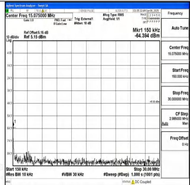
Band41_20MHz_QPSK_41490_1RB#0_0.15~30_0.15~30
