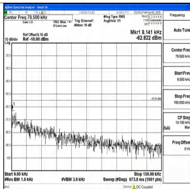
Band41_10MHz_16QAM_40620_1RB#0_0.009~0.15_0.009~0.15
