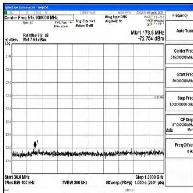
Band41_10MHz_16QAM_39700_1RB#0_30~1000_30~1000
