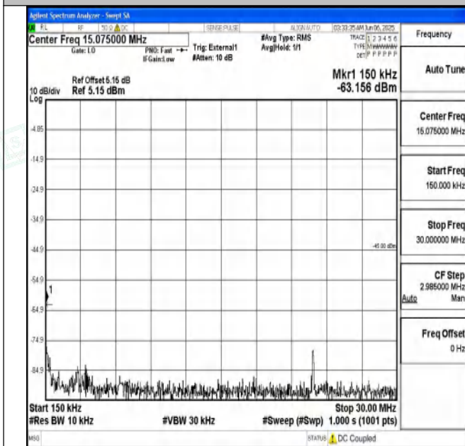
Band41_20MHz_16QAM_40620_1RB#0_0.15~30_0.15~30
