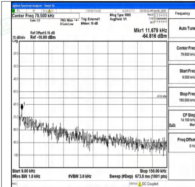
Band41_10MHz_QPSK_40620_1RB#0_0.009~0.15_0.009~0.15
