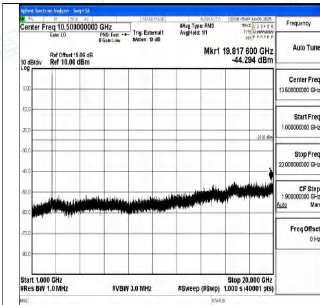
Band41_10MHz_16QAM_40620_1RB#0_1000~20000_1000~20000
