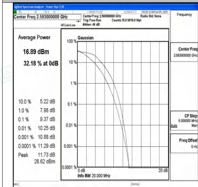
Band41-20MHz-QPSK-40620-100RB#0-PASS
