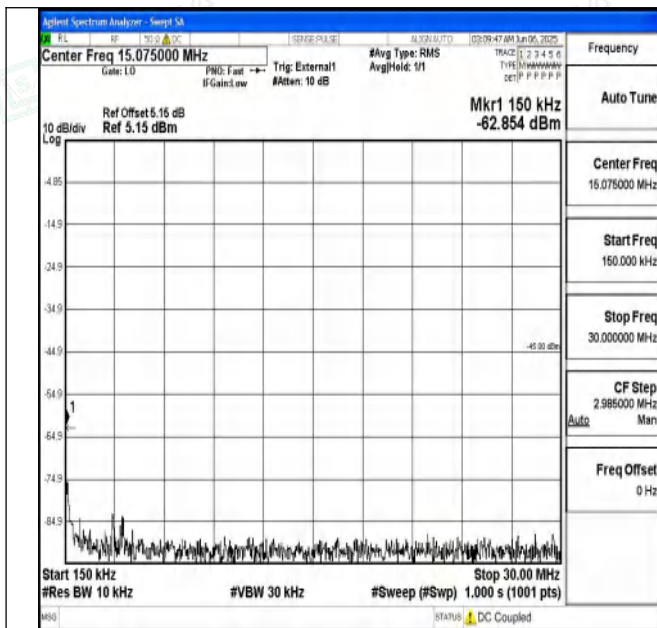
Band41_10MHz_16QAM_41540_1RB#0_0.15~30_0.15~30
