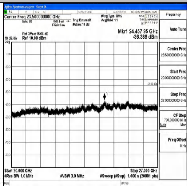
Band41_20MHz_16QAM_39750_1RB#0_20000~27000_2000 0~27000
