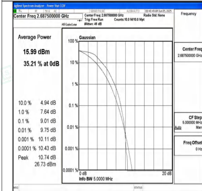
Band41-5MHz-QPSK-41565-25RB#0-PASS
