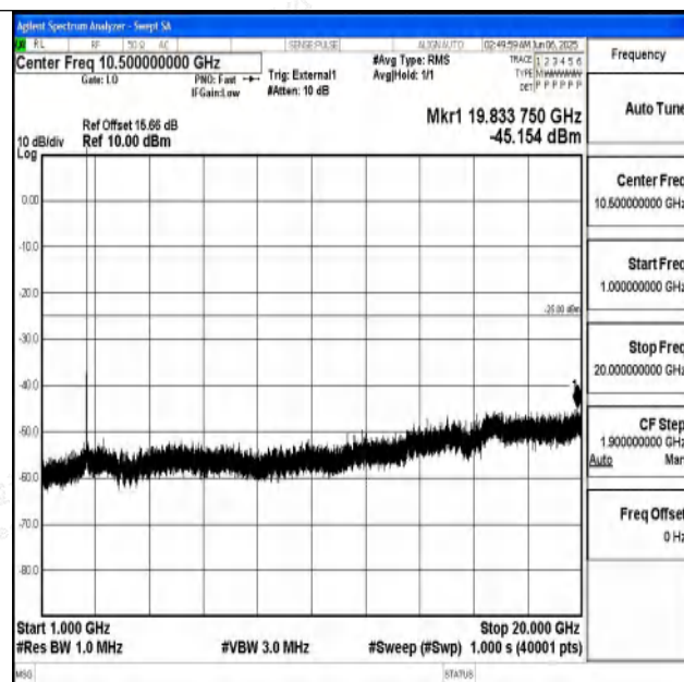
Band41_5MHz_QPSK_40620_1RB#0_1000~20000_1000~20000
