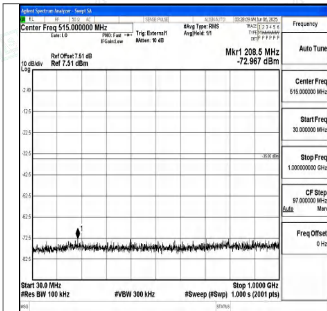
Band41_20MHz_QPSK_39750_1RB#0_30~1000_30~1000
