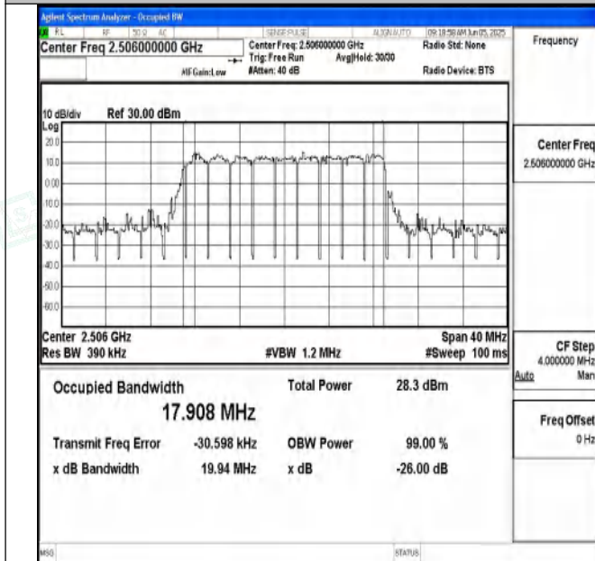
Band41-20MHz-QPSK-39750-100RB#0-PASS
