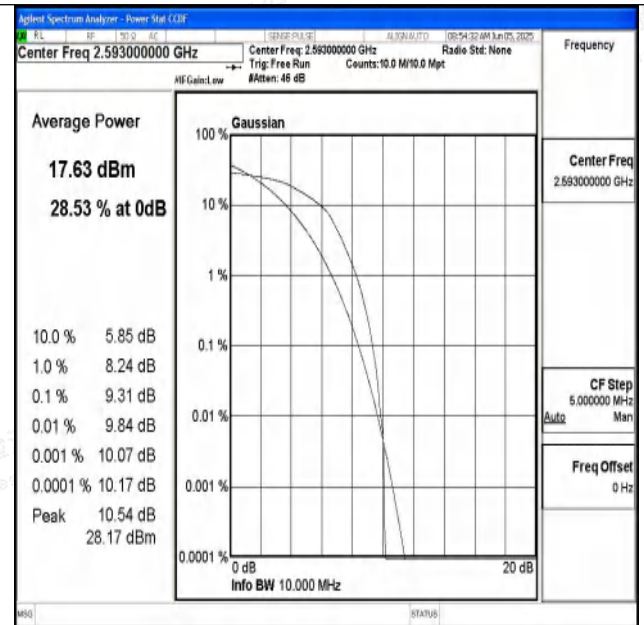
Band41-10MHz-16QAM-40620-1RB#0-PASS
