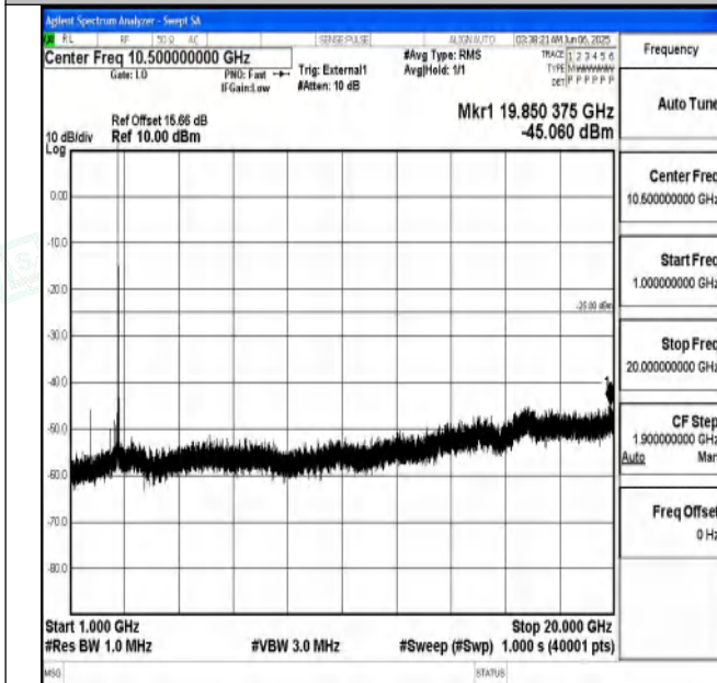
Band41_20MHz_16QAM_41490_1RB#0_1000~20000_1000 ~20000
