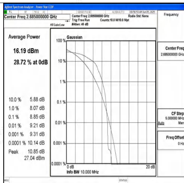
Band41-10MHz-16QAM-41540-1RB#0-PASS
