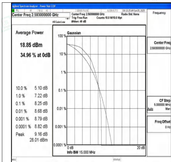
Band41-15MHz-QPSK-40620-1RB#0-PASS
