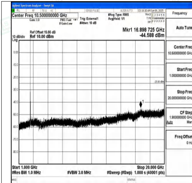
Band41_15MHz_16QAM_39725_1RB#0_1000~20000_1000 ~20000
