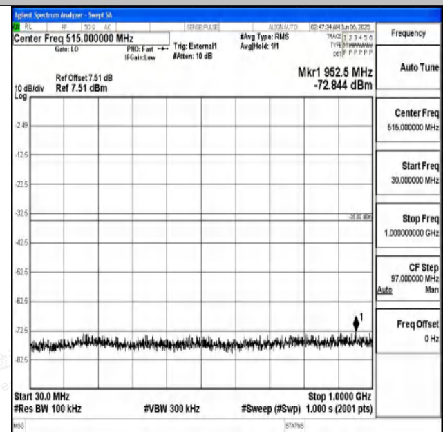
Band41_5MHz_16QAM_39675_1RB#0_30~1000_30~1000
