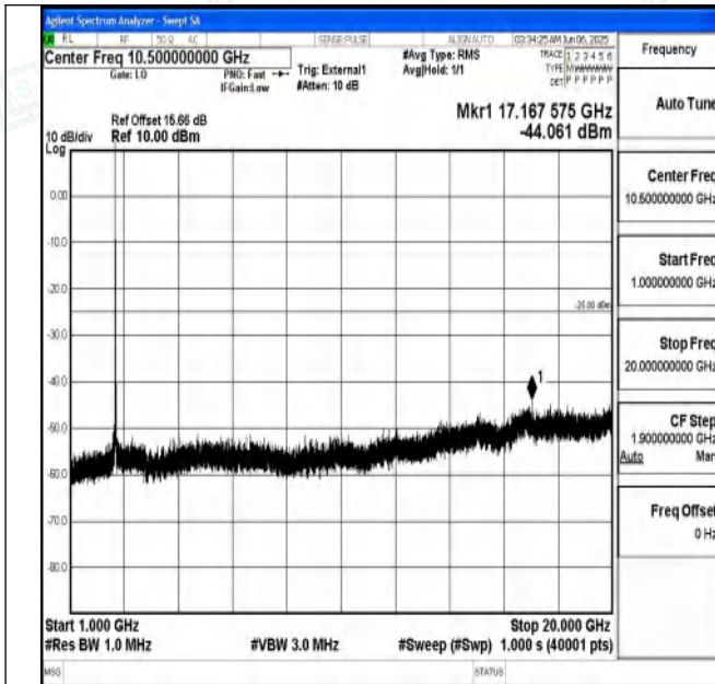
Band41_20MHz_16QAM_40620_1RB#0_1000~20000_1000 ~20000
