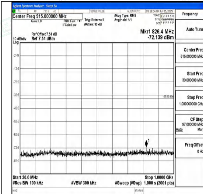
Band41_15MHz_QPSK_40620_1RB#0_30~1000_30~1000
