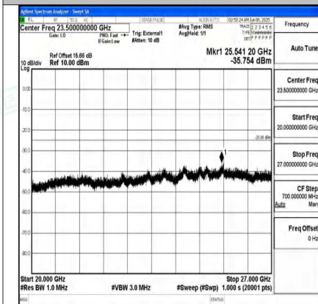
Band41_5MHz_QPSK_40620_1RB#0_20000~27000_20000~27000
