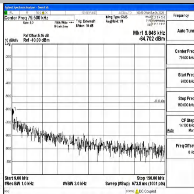
Band41_5MHz_16QAM_40620_1RB#0_0.009~0.15_0.009~0.15
