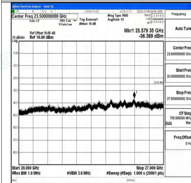
Band41_10MHz_QPSK_39700_1RB#0_20000~27000_20000~27000
