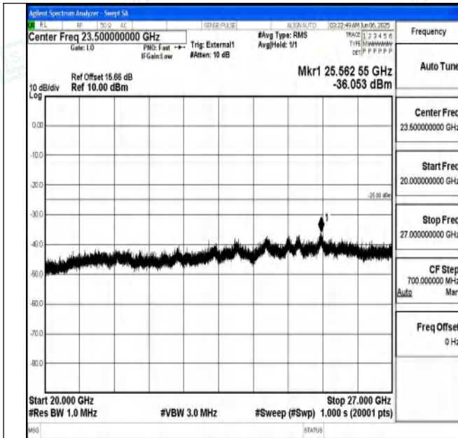
Band41_15MHz_QPSK_41515_1RB#0_20000~27000_2000 0~27000
