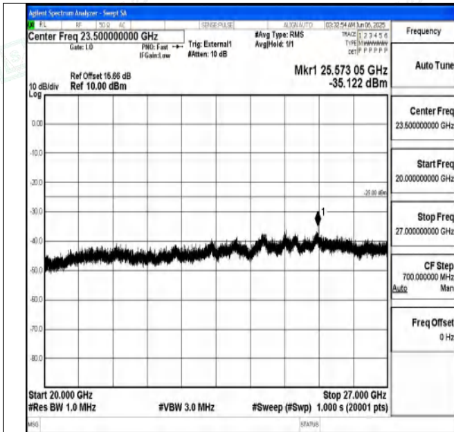
Band41_20MHz_QPSK_40620_1RB#0_20000~27000_2000 0~27000
