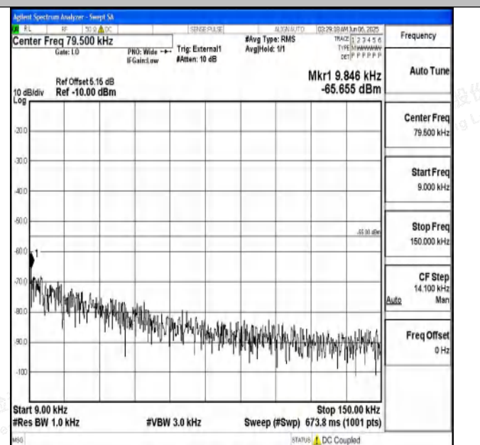
Band41_20MHz_16QAM_39750_1RB#0_0.009~0.15_0.009~0.15
