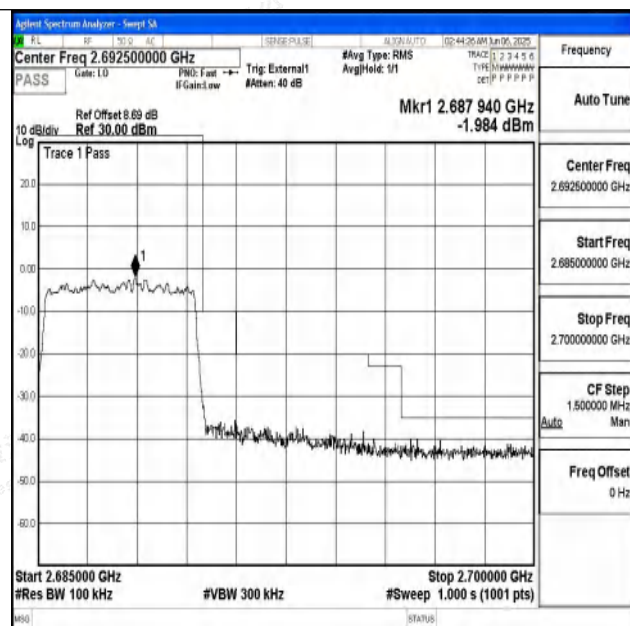
Band41_5MHz_16QAM_41565_25RB#0
