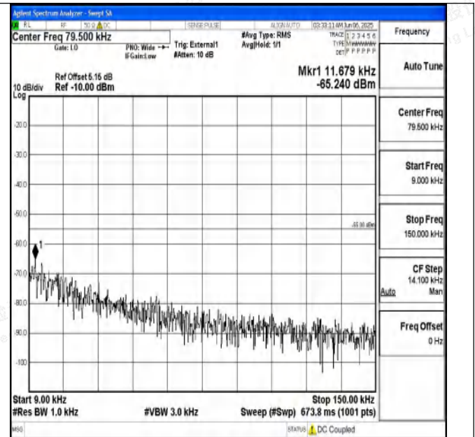
Band41_20MHz_16QAM_40620_1RB#0_0.009~0.15_0.009~0.15
