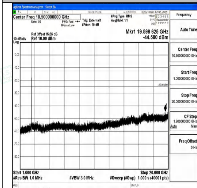
Band41_10MHz_16QAM_39700_1RB#0_1000~20000_1000~20000
