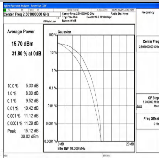
Band41-10MHz-16QAM-39700-50RB#0-PASS
