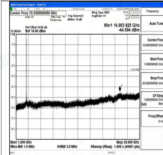
Band41_15MHz_16QAM_40620_1RB#0_1000~20000_1000 ~20000
