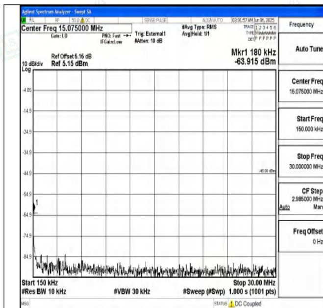
Band41_10MHz_16QAM_39700_1RB#0_0.15~30_0.15~30
