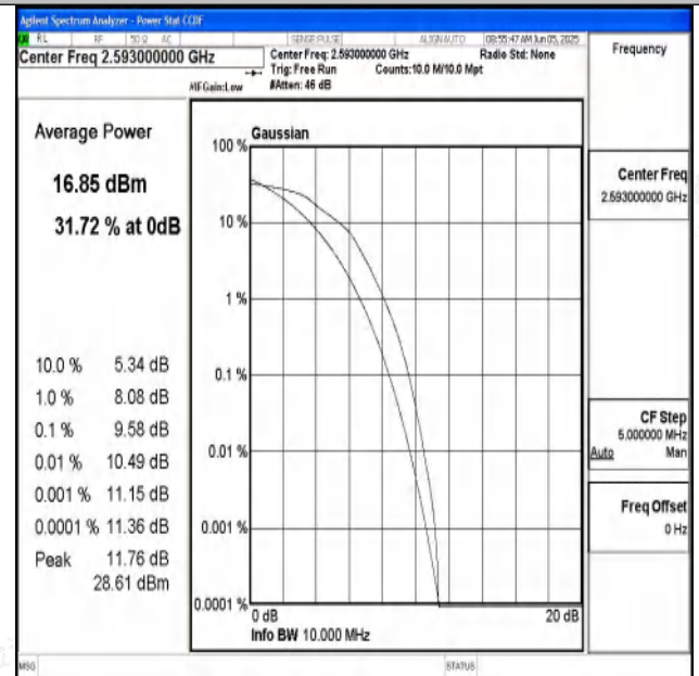
Band41-10MHz-16QAM-40620-50RB#0-PASS
