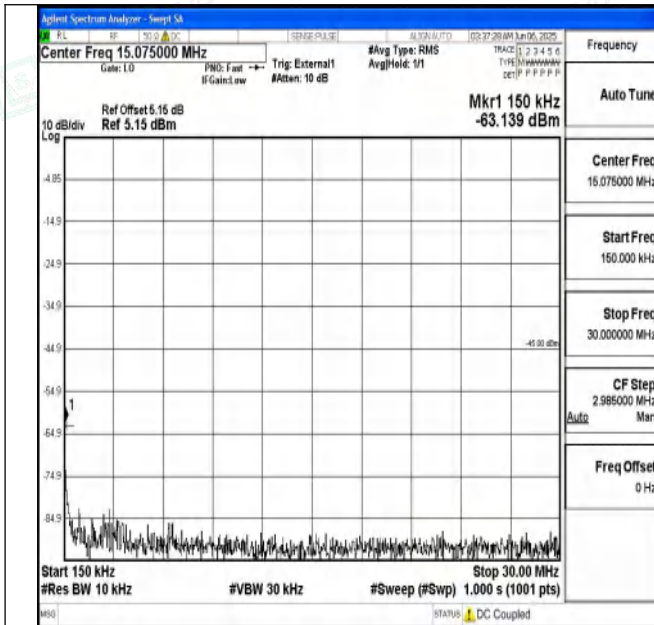
Band41_20MHz_16QAM_41490_1RB#0_0.15~30_0.15~30
