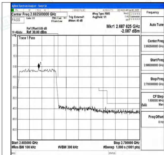
Band41_5MHz_QPSK_41565_25RB#0
