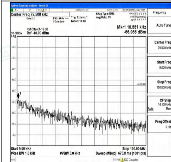
Band41_10MHz_QPSK_41540_1RB#0_0.009~0.15_0.009~0.15
