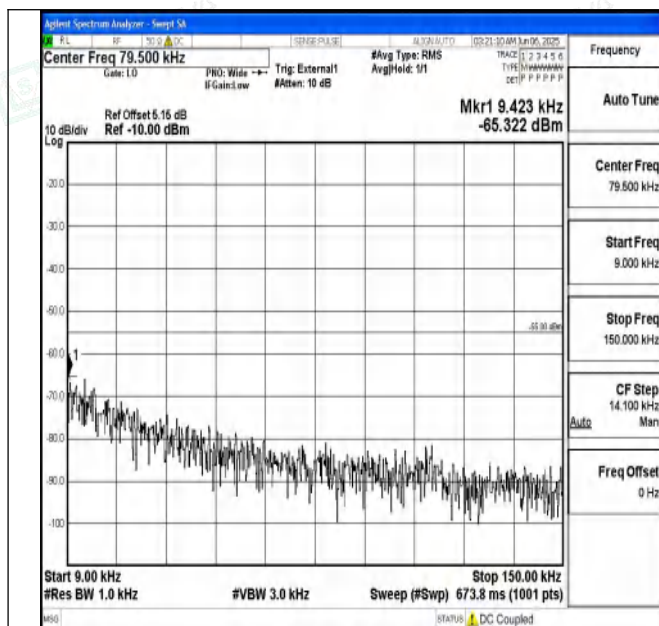
Band41_15MHz_QPSK_41515_1RB#0_0.009~0.15_0.009~0.15
