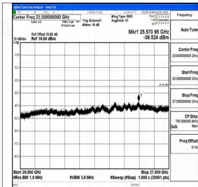
Band41_10MHz_QPSK_40620_1RB#0_20000~27000_2000 0~27000
