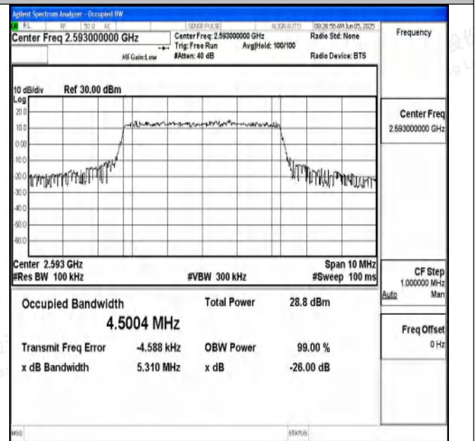
Band41-5MHz-16QAM-40620-25RB#0-PASS
