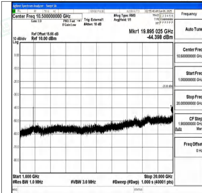
Band41_5MHz_16QAM_41565_1RB#0_1000~20000_1000~20000
