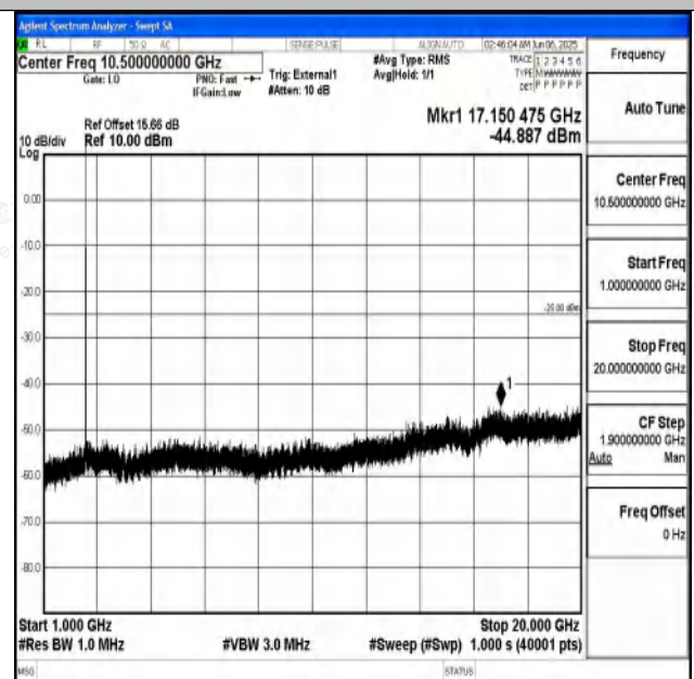
Band41_5MHz_QPSK_39675_1RB#0_1000~20000_1000~20
