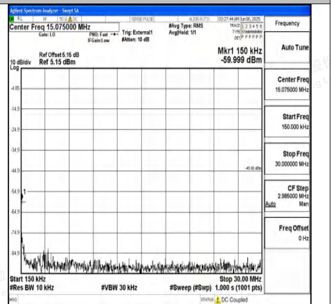
Band41_15MHz_16QAM_41515_1RB#0_20000~27000_2000 0~27000
