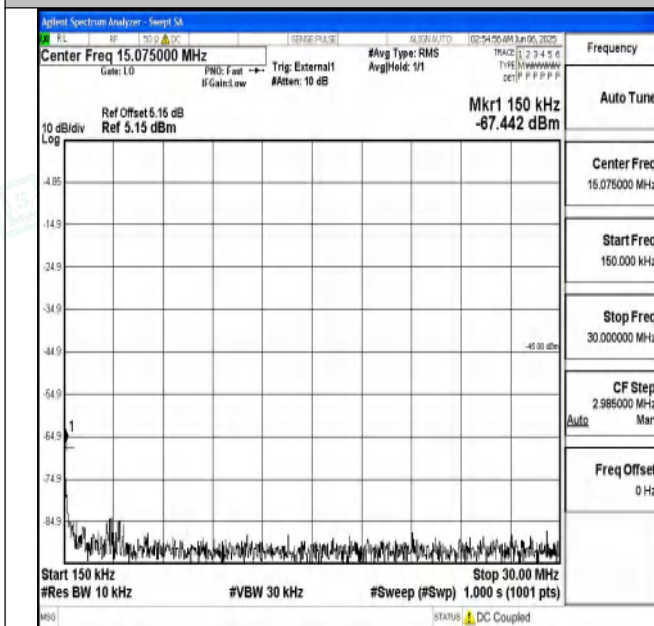
Band41_5MHz_16QAM_41565_1RB#0_0.15~30_0.15~30
