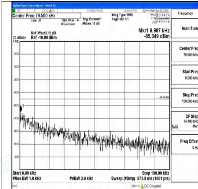
Band41_5MHz_QPSK_39675_1RB#0_0.009~0.15_0.009~0.
