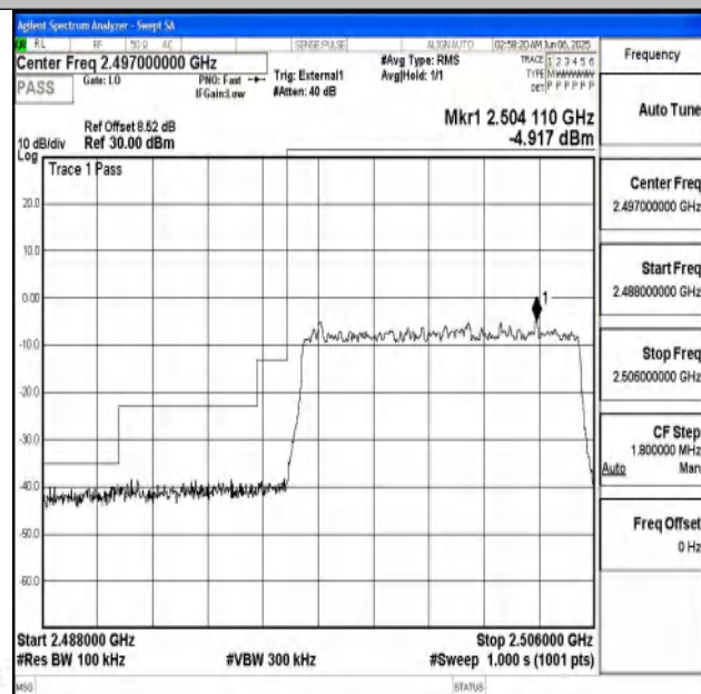
Band41_10MHz_16QAM_39700_50RB#0
