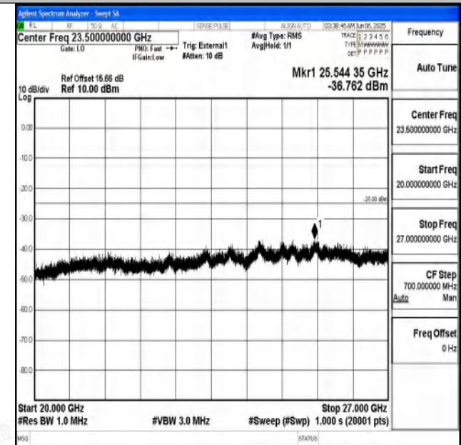
Band41_20MHz_16QAM_41490_1RB#0_20000~27000_2000 0~27000
