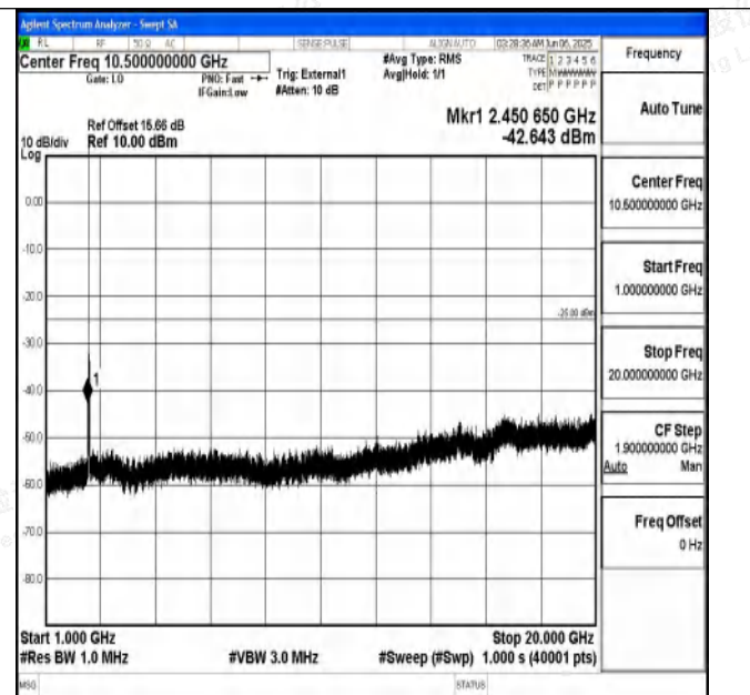
Band41_20MHz_QPSK_39750_1RB#0_1000~20000_1000~20000
