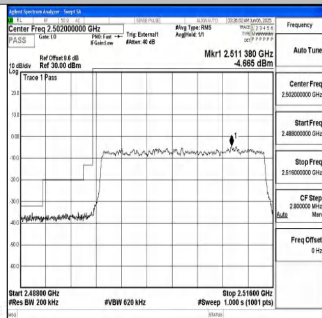
Band41_20MHz_16QAM_39750_100RB#0
