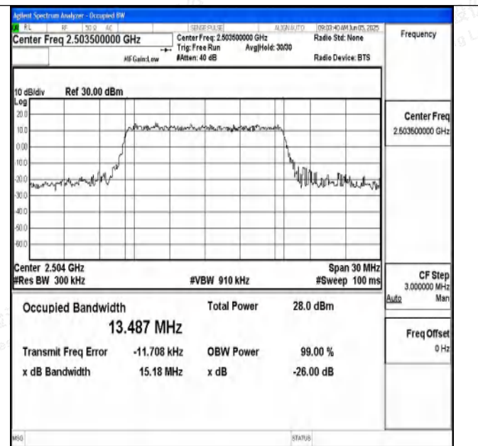
Band41-15MHz-16QAM-39725-75RB#0-PASS
