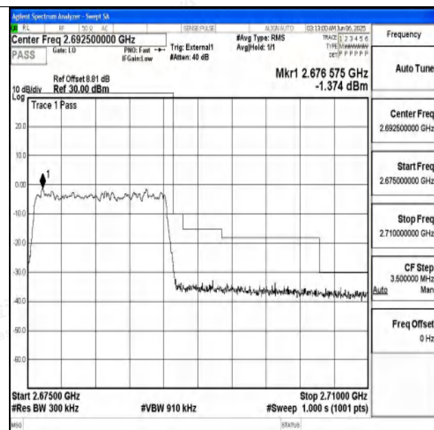
Band41_15MHz_16QAM_41515_75RB#0
