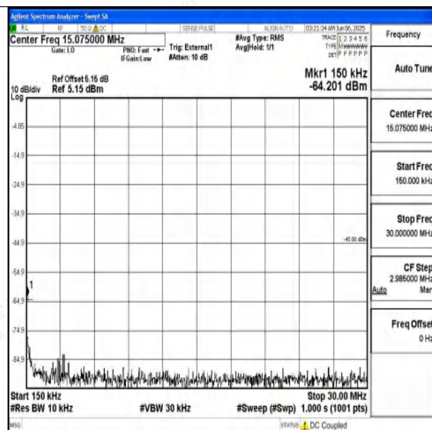
Band41_15MHz_QPSK_41515_1RB#0_0.15~30_0.15~30
