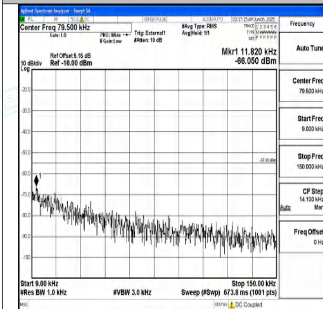
Band41_15MHz_QPSK_40620_1RB#0_0.009~0.15_0.009~0.15
