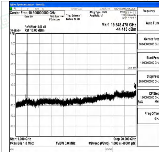
Band41_15MHz_16QAM_41515_1RB#0_1000~20000_1000 ~20000
