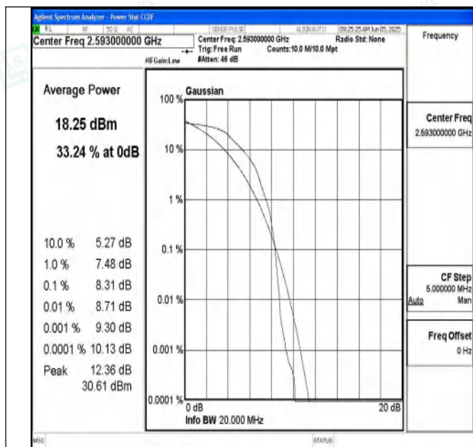
Band41-20MHz-QPSK-40620-1RB#0-PASS
