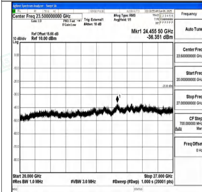
Band41_15MHz_QPSK_40620_1RB#0_20000~27000_20000~27000
