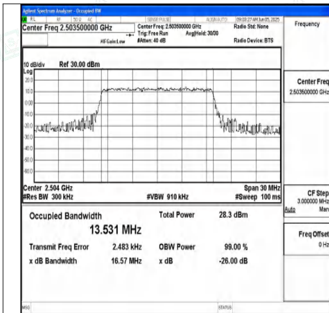
Band41-15MHz-QPSK-39725-75RB#0-PASS
