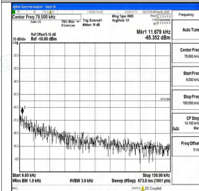
Band41_20MHz_QPSK_39750_1RB#0_0.009~0.15_0.009~0 .15
