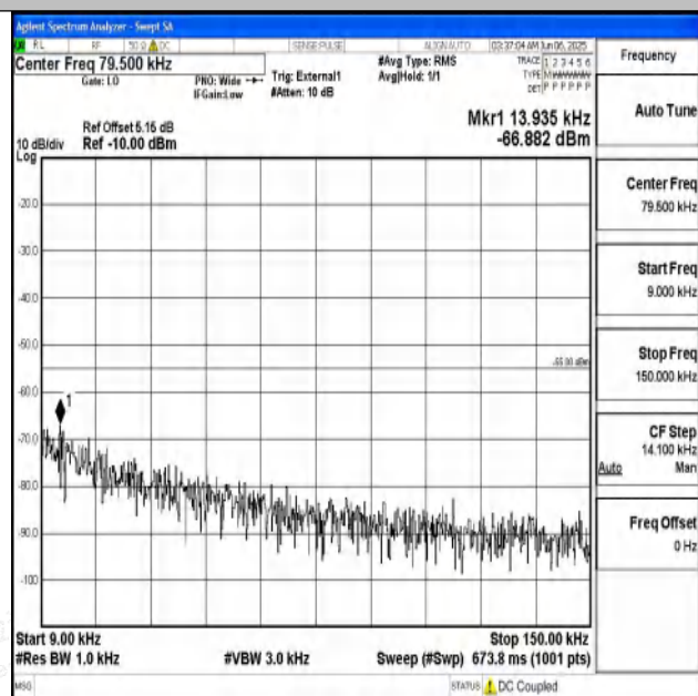
Band41_20MHz_16QAM_41490_1RB#0_0.009~0.15_0.009~0.15
