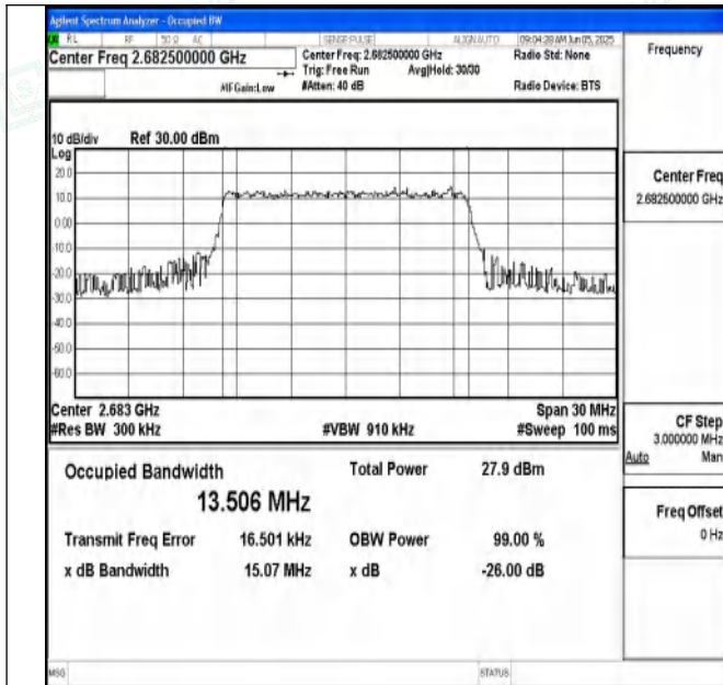
Band41-15MHz-QPSK-41515-75RB#0-PASS
