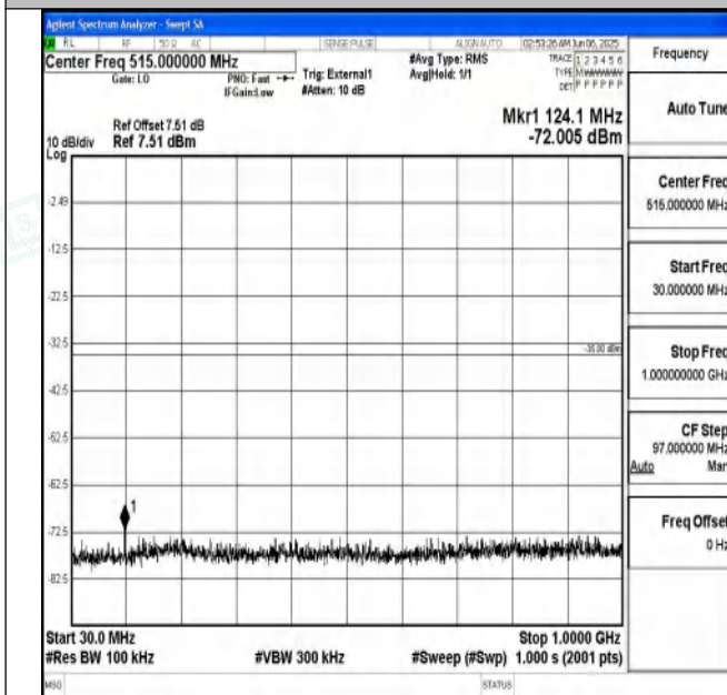
Band41_5MHz_QPSK_41565_1RB#0_30~1000_30~1000
