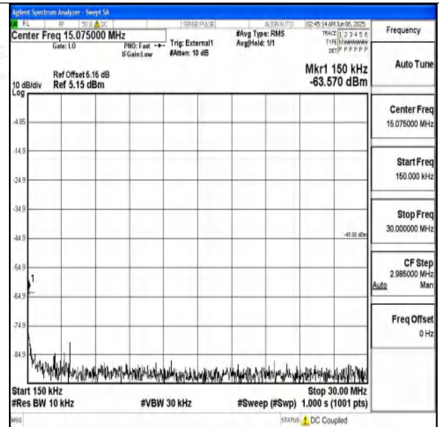
Band41_5MHz_QPSK_39675_1RB#0_0.15~30_0.15~30
