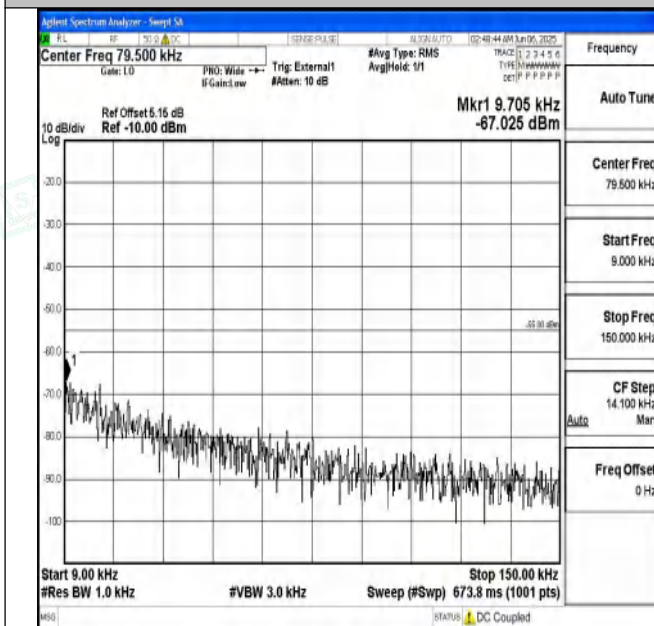
Band41_5MHz_QPSK_40620_1RB#0_0.009~0.15_0.009~0. 15
