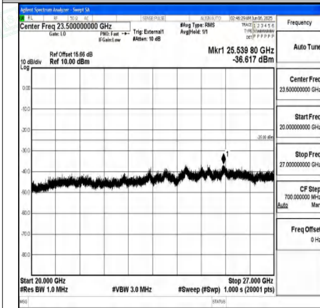
Band41_5MHz_QPSK_39675_1RB#0_20000~27000_20000~27000
