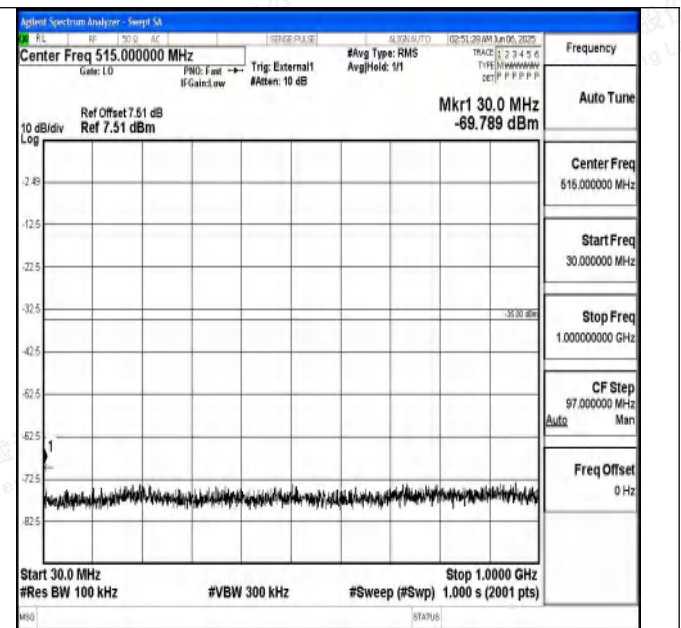
Band41_5MHz_16QAM_40620_1RB#0_30~1000_30~1000
