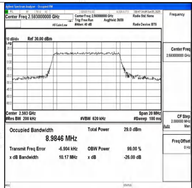
Band41-10MHz-16QAM-40620-50RB#0-PASS
