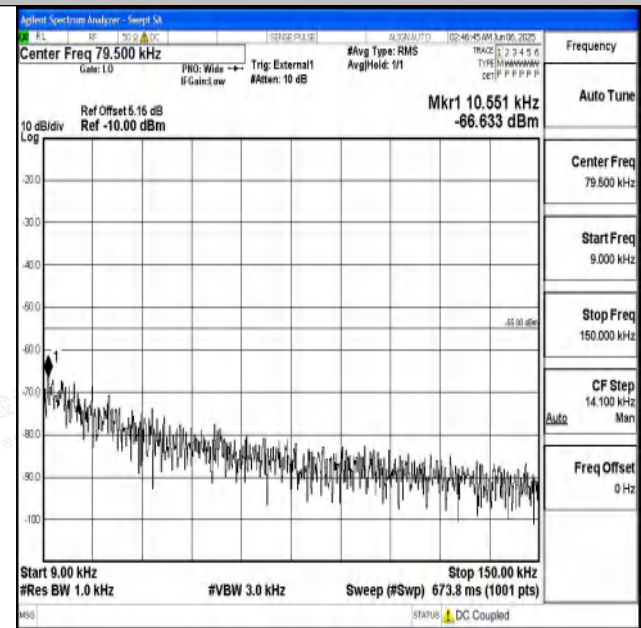
Band41_5MHz_16QAM_39675_1RB#0_0.009~0.15_0.009~0.15
