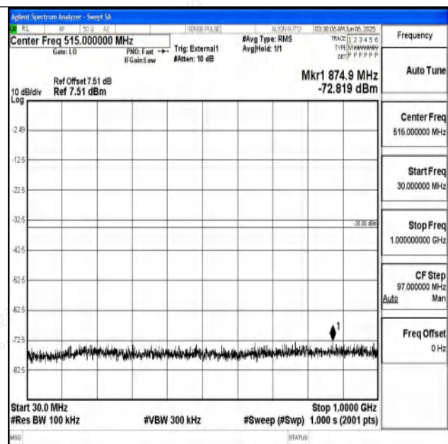
Band41_20MHz_16QAM_39750_1RB#0_30~1000_30~1000
