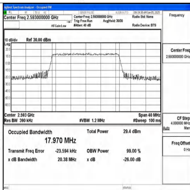
Band41-20MHz-16QAM-40620-100RB#0-PASS
