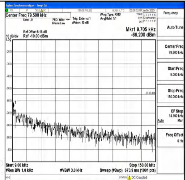
Band41_15MHz_16QAM_40620_1RB#0_0.009~0.15_0.009~0.15
