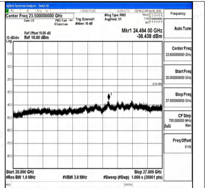
Band41_5MHz_16QAM_41565_1RB#0_20000~27000_20000~27000
