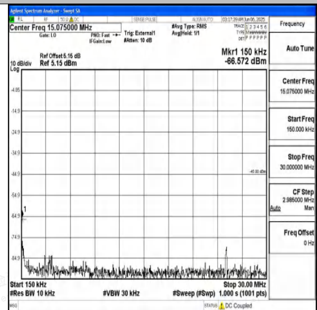
Band41_15MHz_16QAM_39725_1RB#0_20000~27000_2000 0~27000
