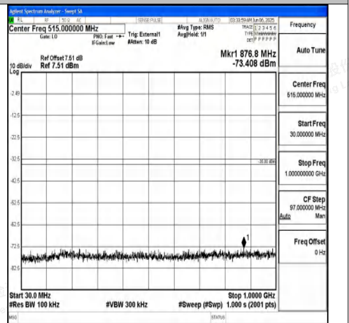
Band41_20MHz_16QAM_40620_1RB#0_30~1000_30~1000
