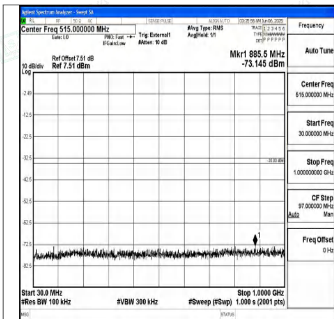
Band41_20MHz_QPSK_41490_1RB#0_30~1000_30~1000
