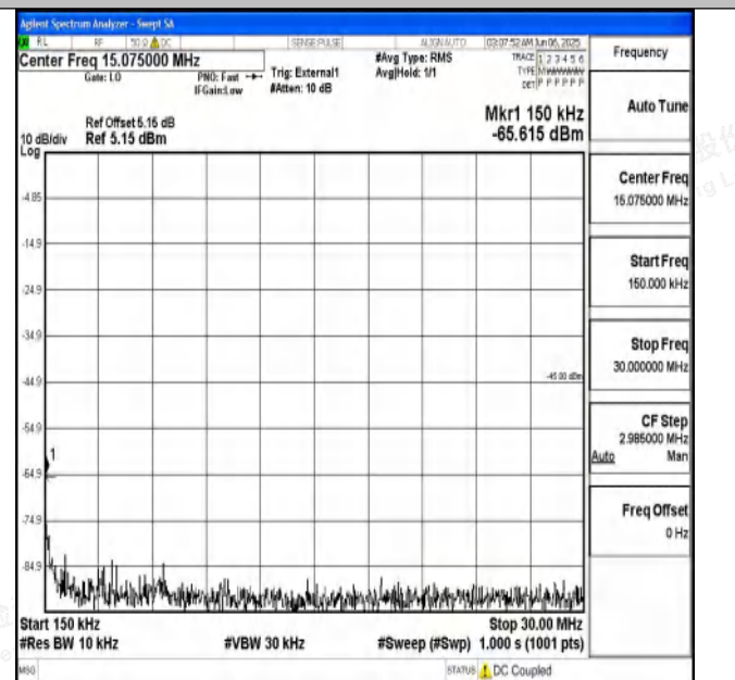
Band41_10MHz_QPSK_41540_1RB#0_0.15~30_0.15~30
