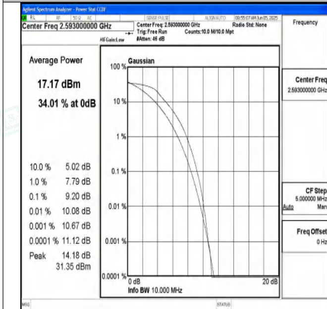
Band41-10MHz-QPSK-40620-50RB#0-PASS
