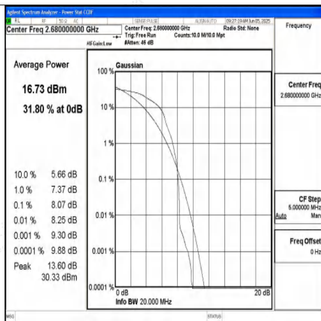
Band41-20MHz-16QAM-41490-1RB#0-PASS
