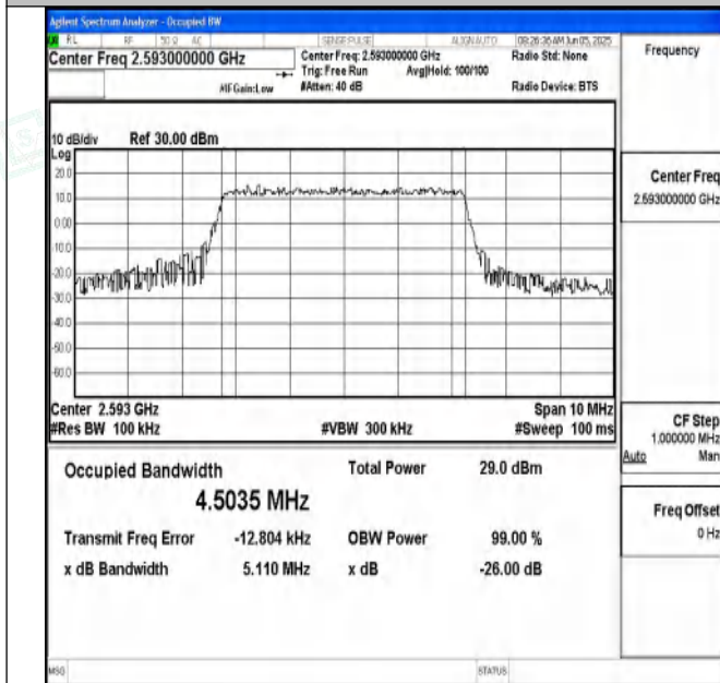
Band41-5MHz-QPSK-40620-25RB#0-PASS
