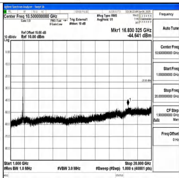
Band41_20MHz_QPSK_41490_1RB#0_1000~20000_1000~20000
