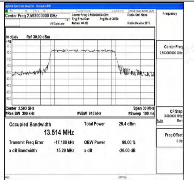
Band41-15MHz-16QAM-40620-75RB#0-PASS
