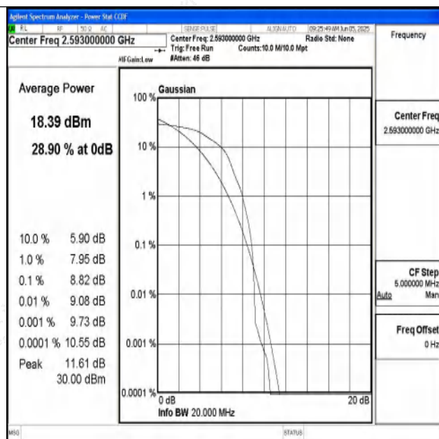
Band41-20MHz-16QAM-40620-1RB#0-PASS
