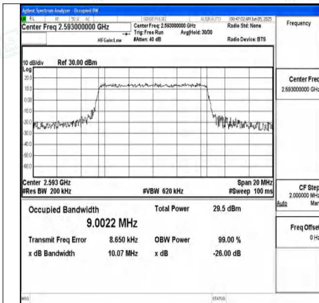
Band41-10MHz-QPSK-40620-50RB#0-PASS
