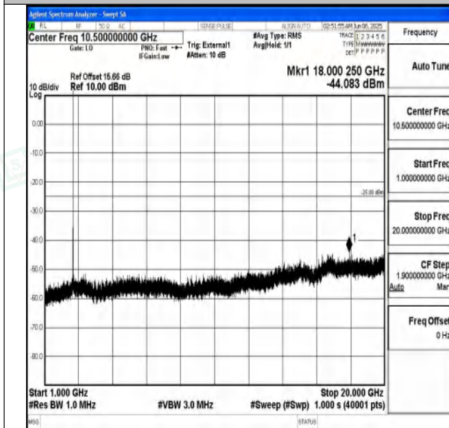
Band41_5MHz_16QAM_40620_1RB#0_1000~20000_1000~20000
