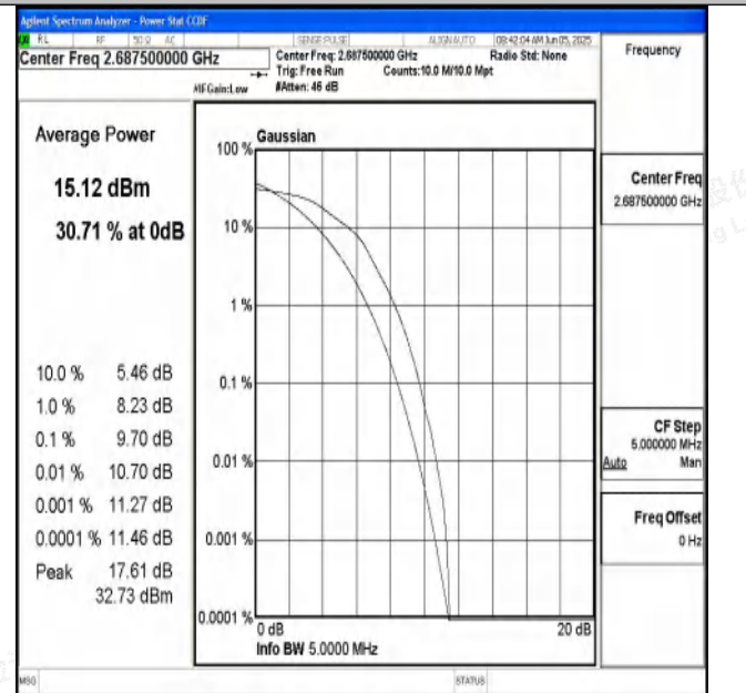
Band41-5MHz-16QAM-41565-25RB#0-PASS
