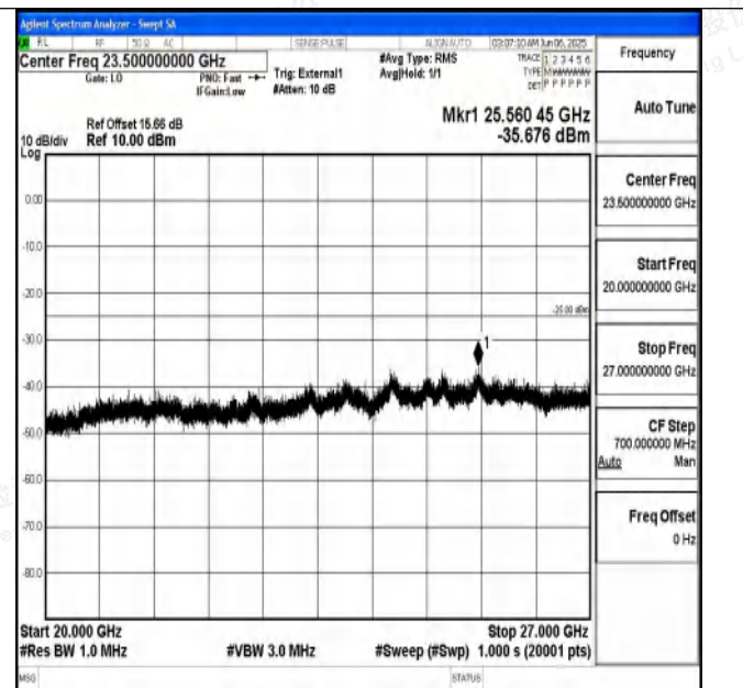
Band41_10MHz_16QAM_40620_1RB#0_20000~27000_20000~27000
