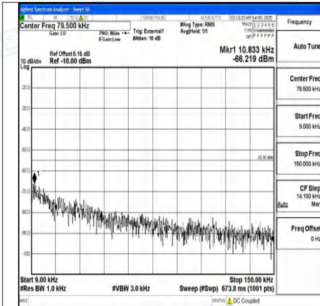
Band41_15MHz_QPSK_39725_1RB#0_0.009~0.15_0.009~0.15
