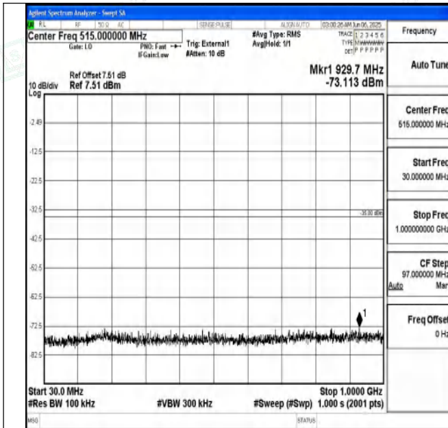
Band41_10MHz_QPSK_39700_1RB#0_30~1000_30~1000
