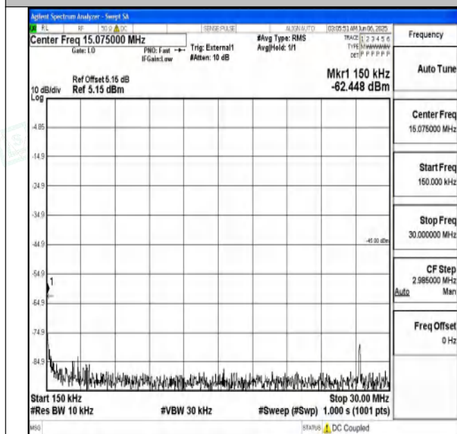
Band41_10MHz_16QAM_40620_1RB#0_0.15~30_0.15~30
