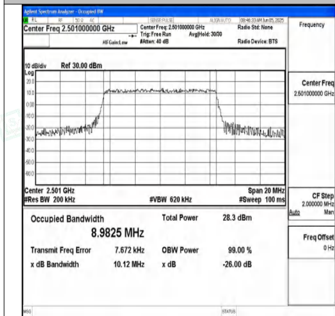
Band41-10MHz-QPSK-39700-50RB#0-PASS
