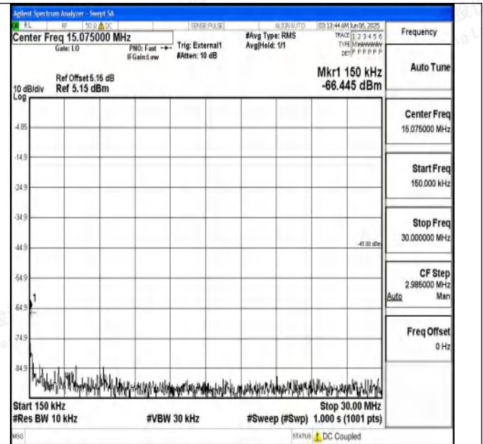
Band41_15MHz_QPSK_39725_1RB#0_0.15~30_0.15~30
