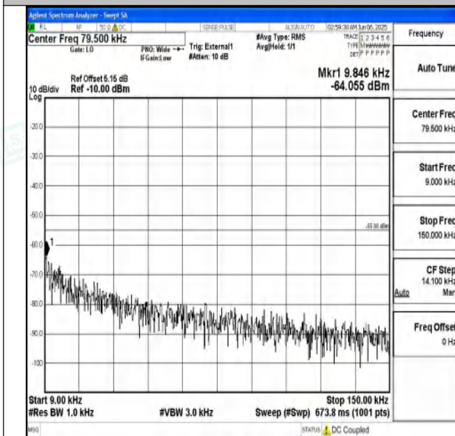
Band41_10MHz_QPSK_39700_1RB#0_0.009~0.15_0.009~0.15
