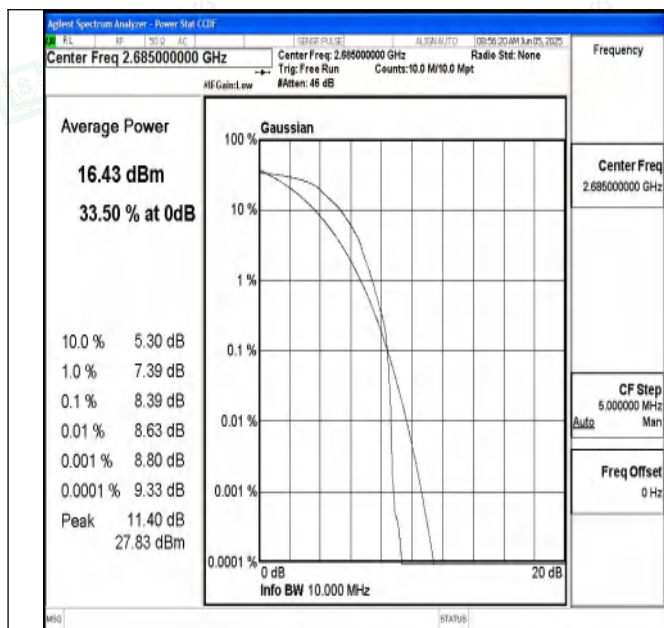
Band41-10MHz-QPSK-41540-1RB#0-PASS
