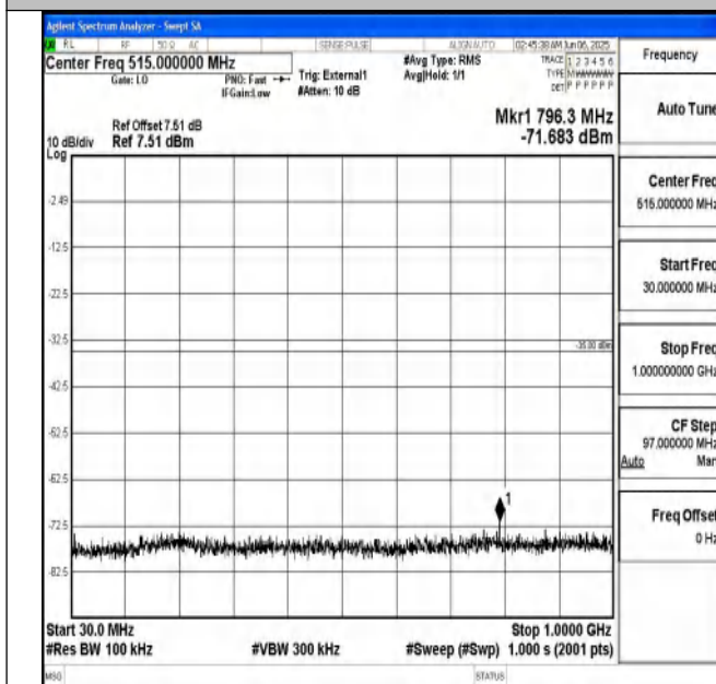
Band41_5MHz_QPSK_39675_1RB#0_30~1000_30~1000
