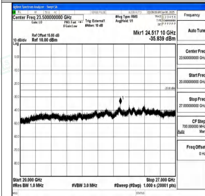
Band41_10MHz_QPSK_41540_1RB#0_20000~27000_20000~27000
