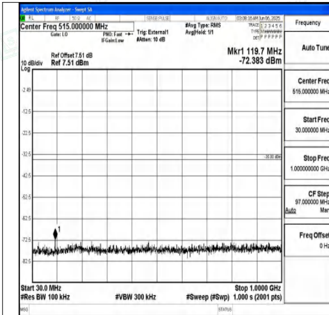
Band41_10MHz_QPSK_41540_1RB#0_30~1000_30~1000
