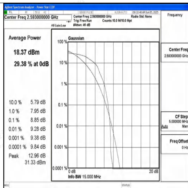
Band41-15MHz-16QAM-40620-1RB#0-PASS
