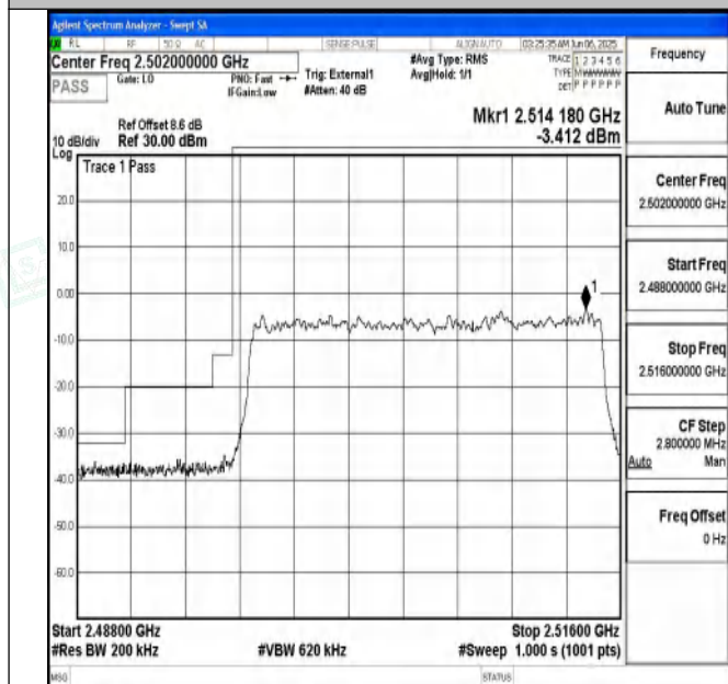
Band41_20MHz_QPSK_39750_100RB#0
