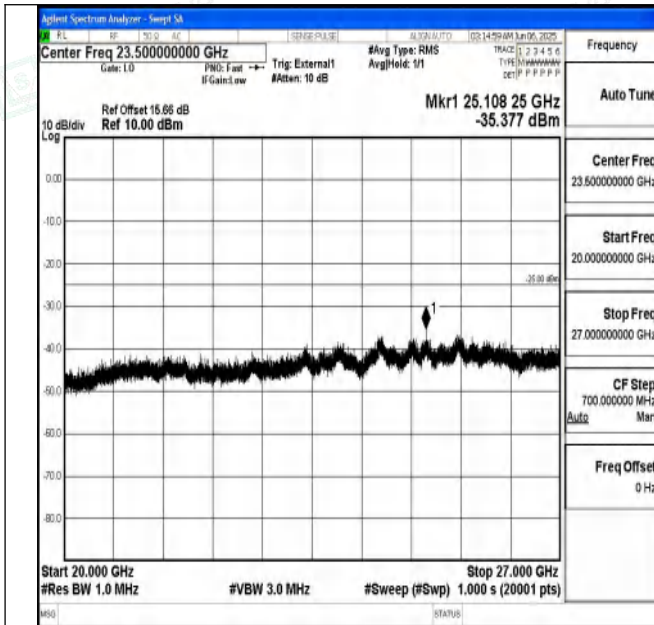
Band41_15MHz_QPSK_39725_1RB#0_20000~27000_2000 0~27000
