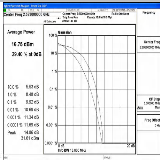
Band41-15MHz-16QAM-40620-75RB#0-PASS
