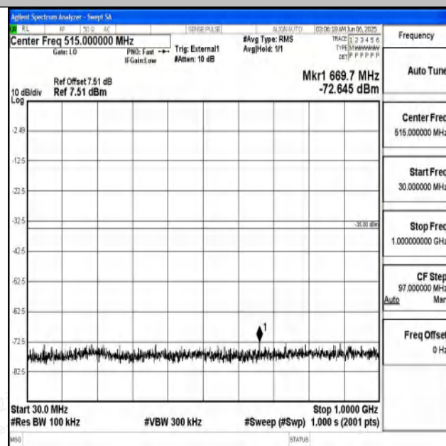
Band41_10MHz_16QAM_40620_1RB#0_30~1000_30~1000
