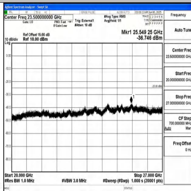
Band41_10MHz_16QAM_39700_1RB#0_20000~27000_20000~27000
