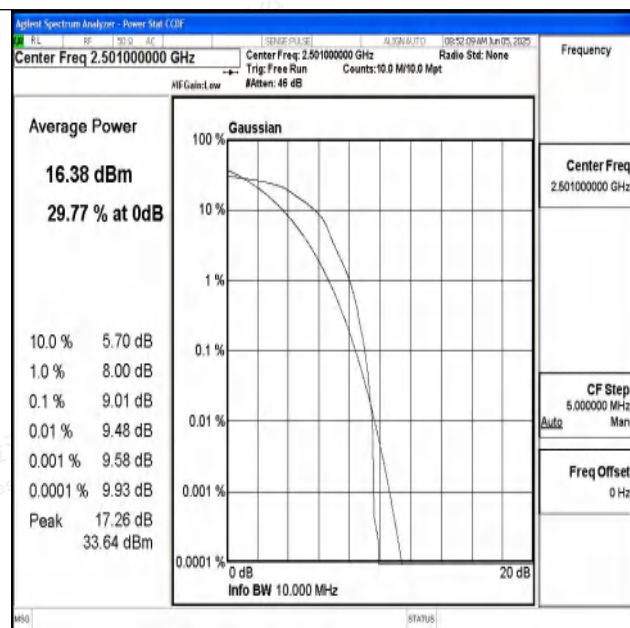
Band41-10MHz-16QAM-39700-1RB#0-PASS
