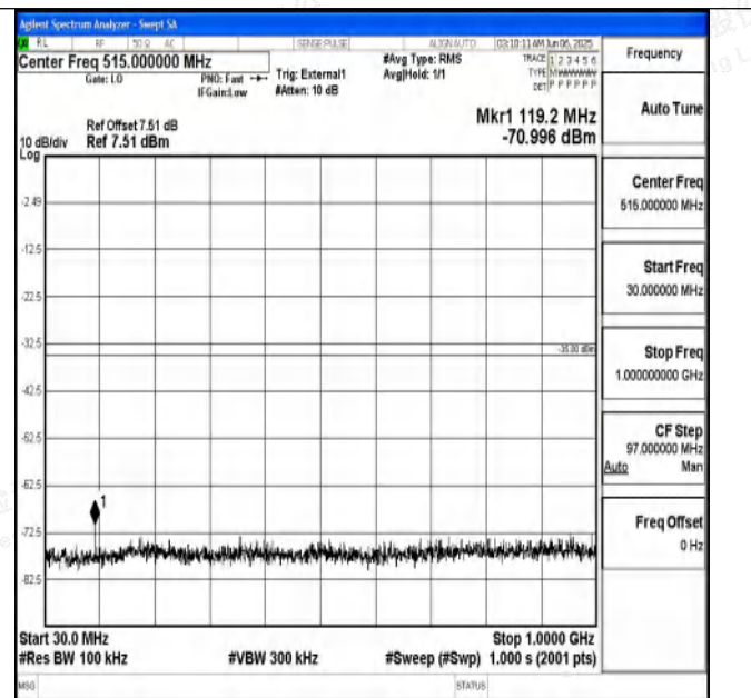
Band41_10MHz_16QAM_41540_1RB#0_30~1000_30~1000
