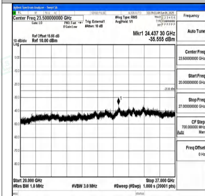
Band41_20MHz_QPSK_39750_1RB#0_20000~27000_20000~27000
