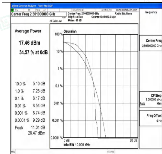
Band41-10MHz-QPSK-39700-1RB#0-PASS
