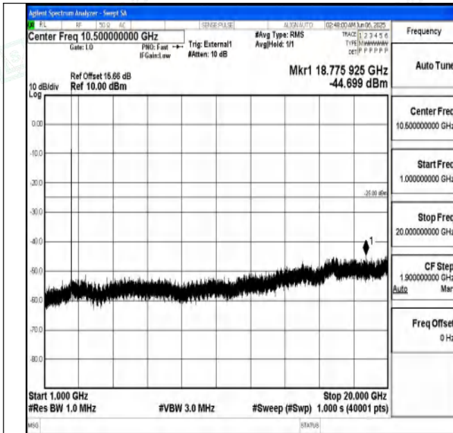
Band41_5MHz_16QAM_39675_1RB#0_1000~20000_1000~ 20000
