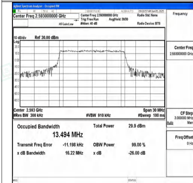
Band41-15MHz-QPSK-40620-75RB#0-PASS
