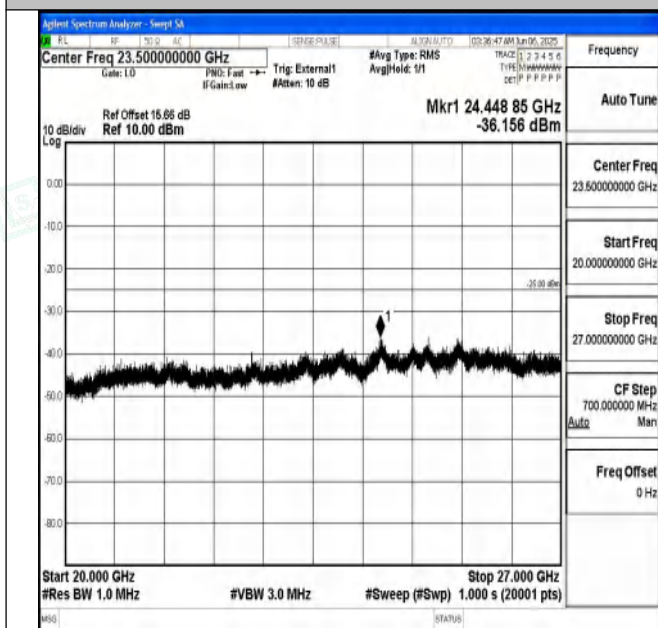
Band41_20MHz_QPSK_41490_1RB#0_20000~27000_20000~27000
