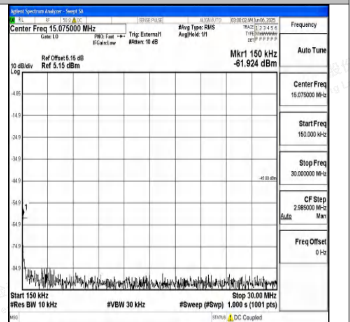
Band41_5MHz_16QAM_41565_1RB#0_20000~27000_20000~27000
