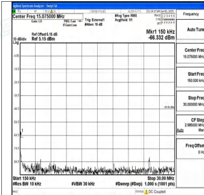
Band41_15MHz_16QAM_40620_1RB#0_0.15~30_0.15~30
