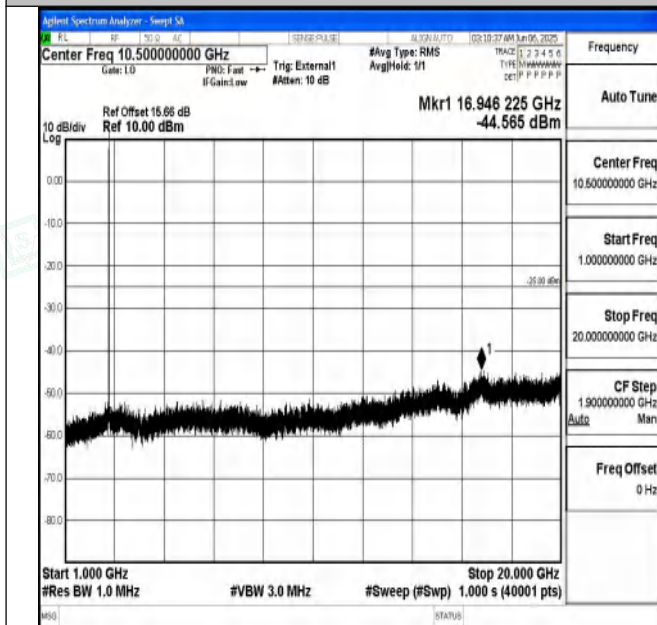
Band41_10MHz_16QAM_41540_1RB#0_1000~20000_1000 ~20000
