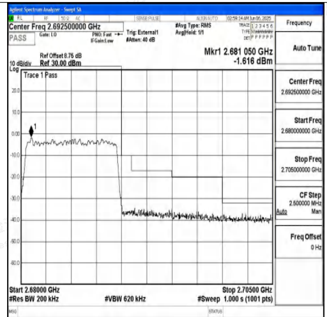
Band41_10MHz_16QAM_41540_50RB#0
