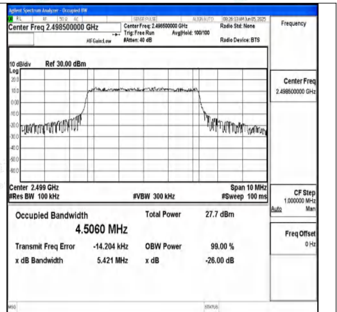
Band41-5MHz-16QAM-39675-25RB#0-PASS
