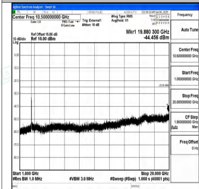
Band41_20MHz_16QAM_39750_1RB#0_1000~20000_1000 ~20000
