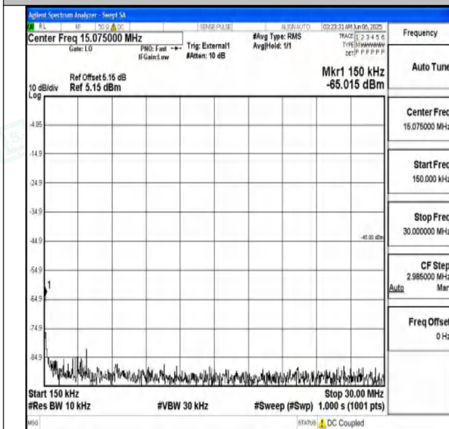
Band41_15MHz_16QAM_41515_1RB#0_0.15~30_0.15~30
