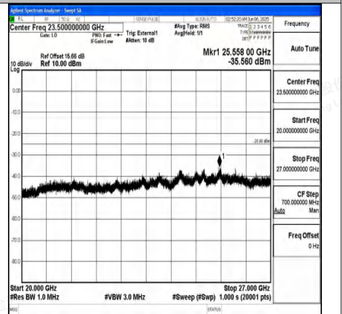
Band41_5MHz_16QAM_40620_1RB#0_20000~27000_20000~27000
