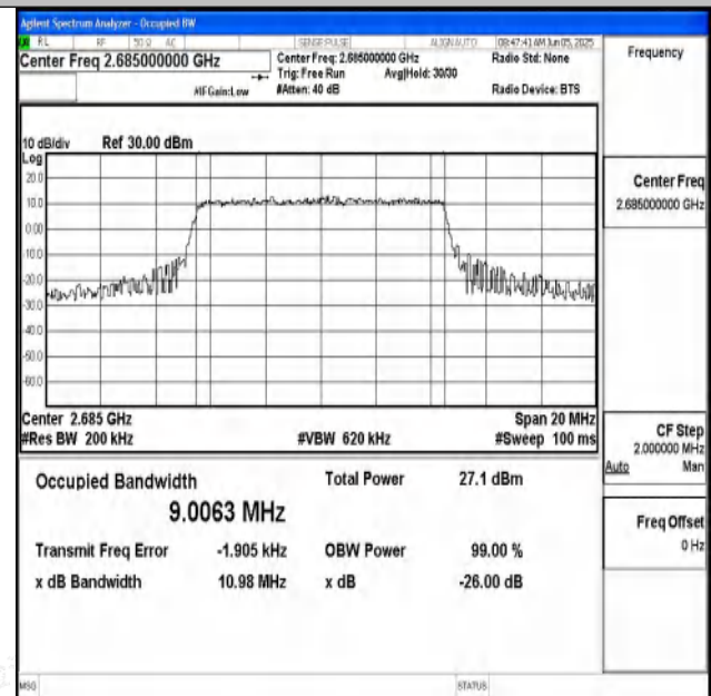
Band41-10MHz-16QAM-41540-50RB#0-PASS
