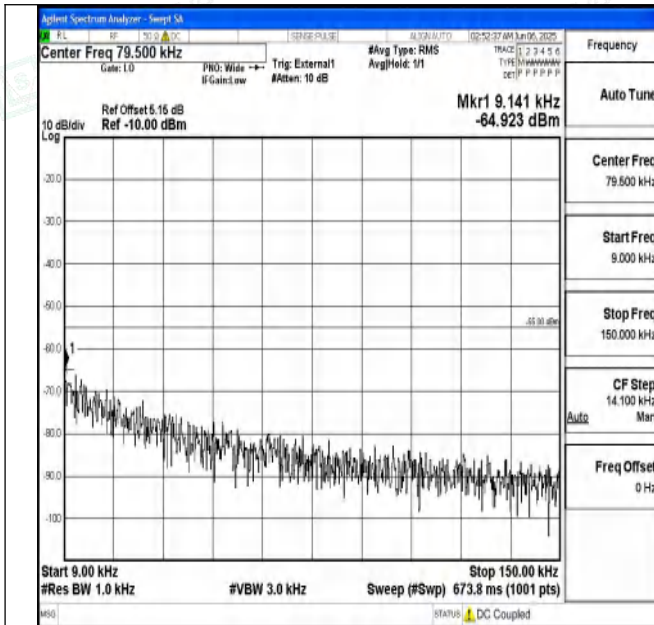
Band41_5MHz_QPSK_41565_1RB#0_0.009~0.15_0.009~0.
