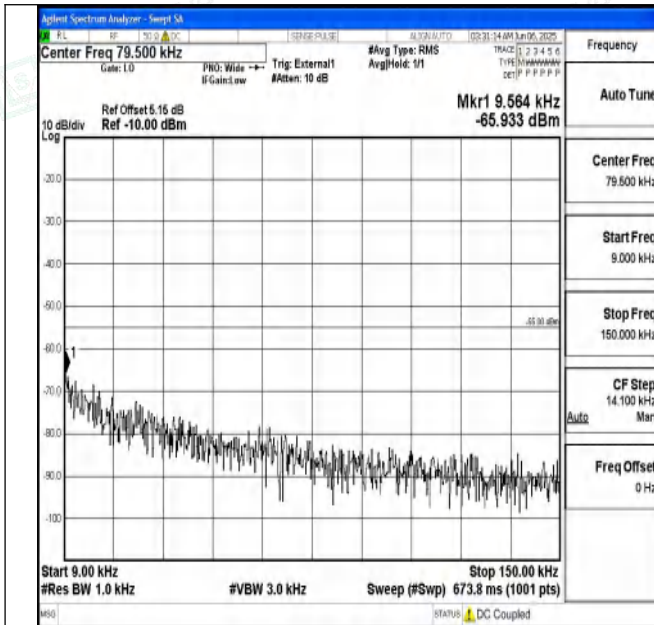
Band41_20MHz_QPSK_40620_1RB#0_0.009~0.15_0.009~0.15
