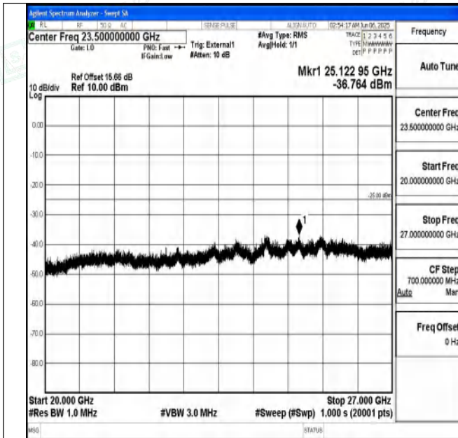
Band41_5MHz_QPSK_41565_1RB#0_20000~27000_20000 ~27000
