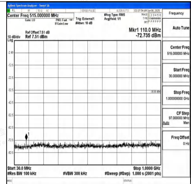
Band41_20MHz_16QAM_41490_1RB#0_30~1000_30~1000
