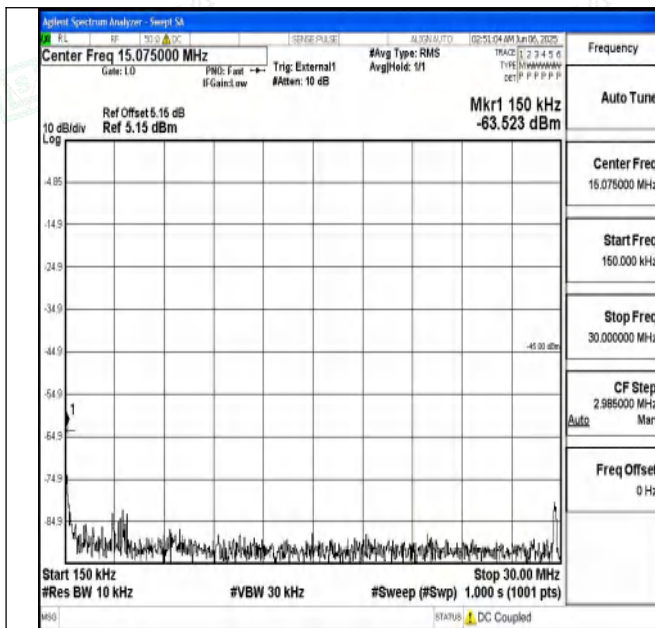
Band41_5MHz_16QAM_40620_1RB#0_0.15~30_0.15~30
