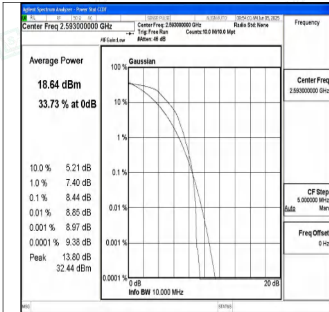
Band41-10MHz-QPSK-40620-1RB#0-PASS
