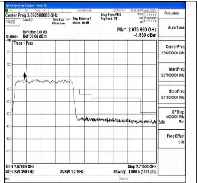
Band41_20MHz_16QAM_41490_100RB#0
