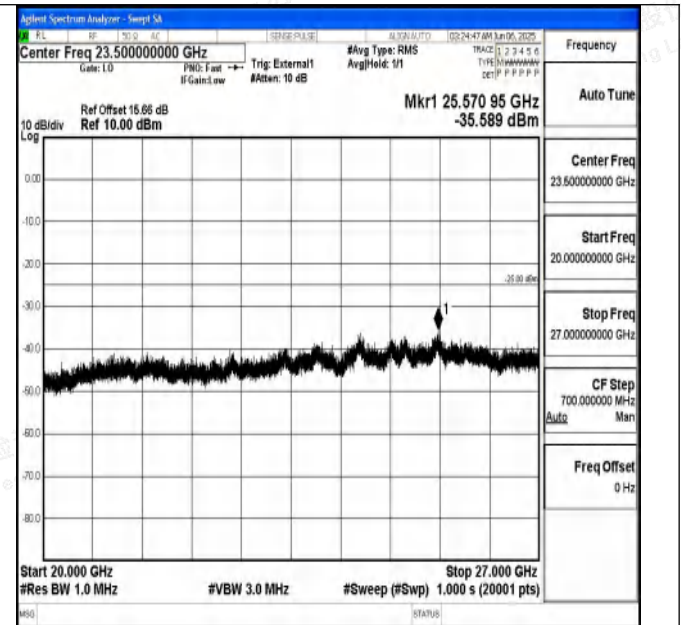
Band41_15MHz_16QAM_41515_1RB#0_20000~27000_2000 0~27000
