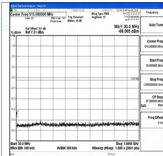
Band41_5MHz_QPSK_40620_1RB#0_30~1000_30~1000
