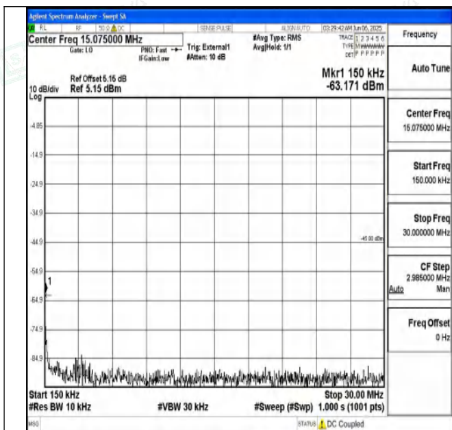
Band41_20MHz_16QAM_39750_1RB#0_0.15~30_0.15~30
