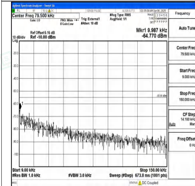
Band41_20MHz_QPSK_41490_1RB#0_0.009~0.15_0.009~0.15
