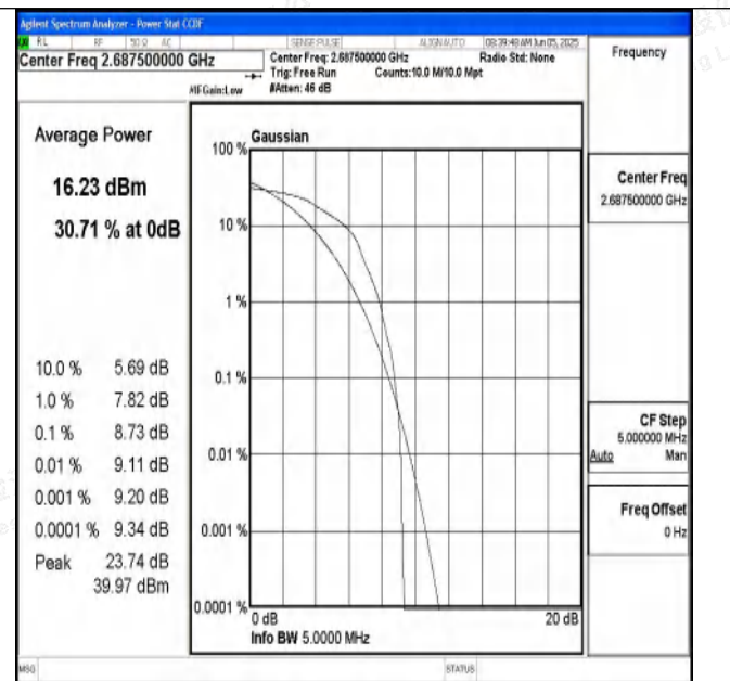
Band41-5MHz-16QAM-41565-1RB#0-PASS
