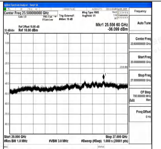
Band41_10MHz_16QAM_41540_1RB#0_20000~27000_2000 0~27000
