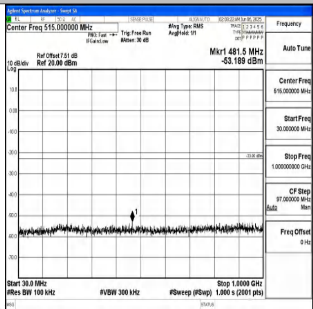
Band25_20MHz_16QAM_26365_1RB#0_30~1000_30~1000
