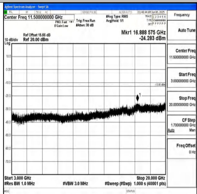
Band25_5MHz_16QAM_26365_1RB#0_3000~20000_30
