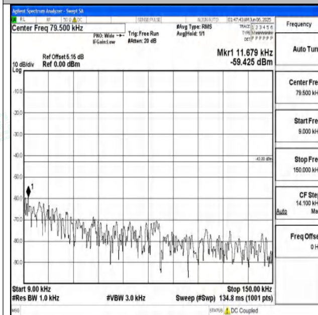
Band25_5MHz_QPSK_26365_1RB#0_0.009~0.15_0.00 9~0.15
