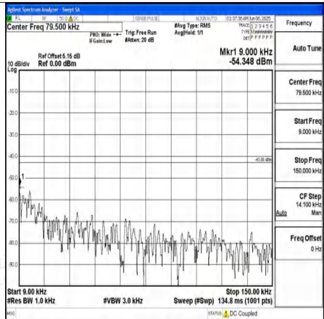
Band25_1.4MHz_16QAM_26047_1RB#0_0.009~0.15_0.009~0.15
