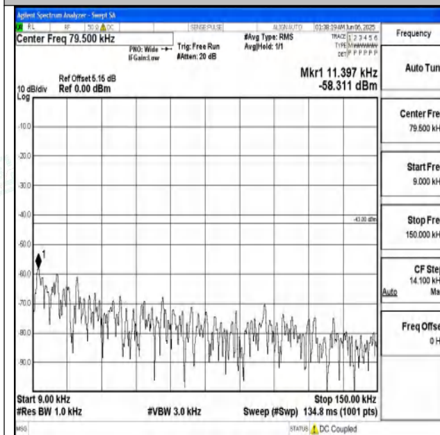
Band25_1.4MHz_QPSK_26365_1RB#0_0.009~0.15_0. 009~0.15
