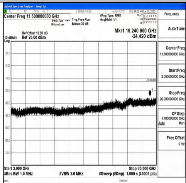
Band25_1.4MHz_16QAM_26365_1RB#0_3000~20000_3 000~20000
