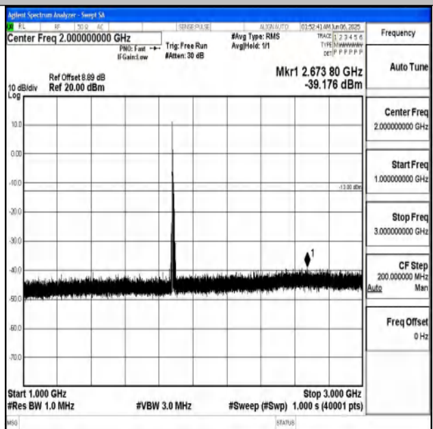
Band25_10MHz_QPSK_26365_1RB#0_1000~3000_100 0~3000
