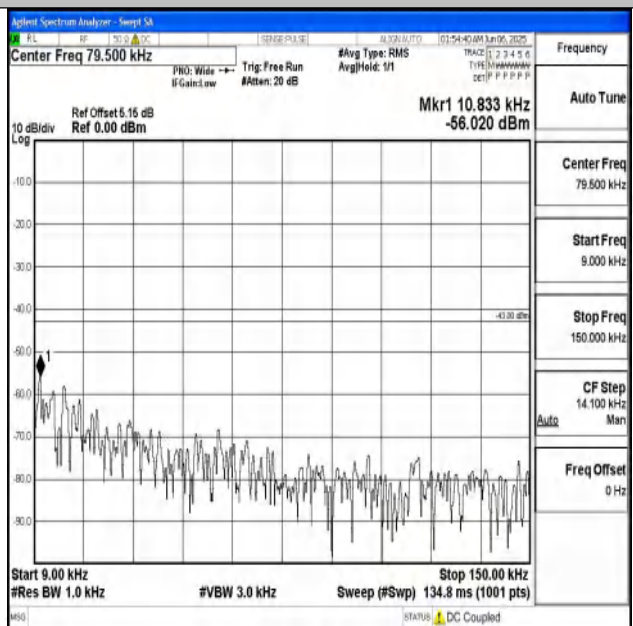
Band25_10MHz_16QAM_26640_1RB#0_0.009~0.15_0.009~0.15
