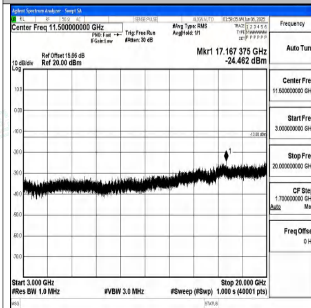
Band25_15MHz_QPSK_26365_1RB#0_3000~20000_3000~20000
