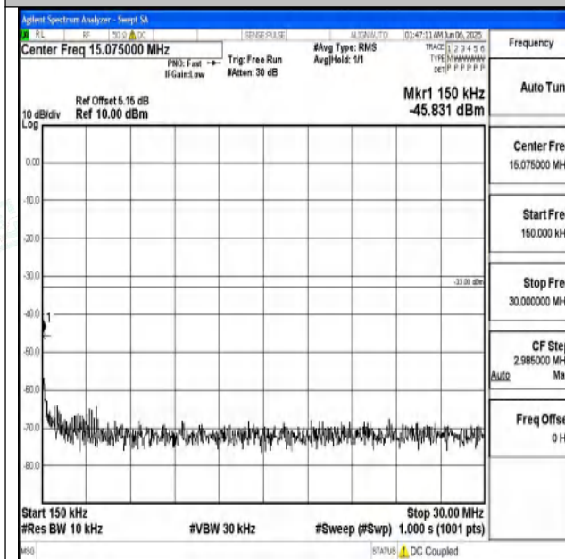
Band25_5MHz_16QAM_26065_1RB#0_0.15~30_0.15~30
