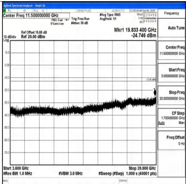
Band25_5MHz_16QAM_26665_1RB#0_3000~20000_30 00~20000
