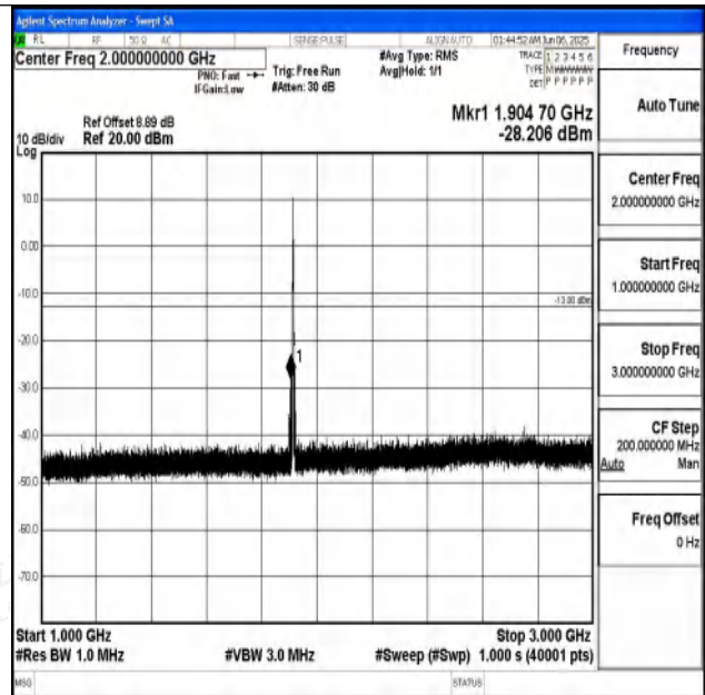
Band25_3MHz_QPSK_26675_1RB#0_1000~3000_1000
