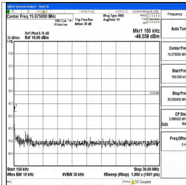
Band25_10MHz_16QAM_26640_1RB#0_0.15~30_0.15 ~30
