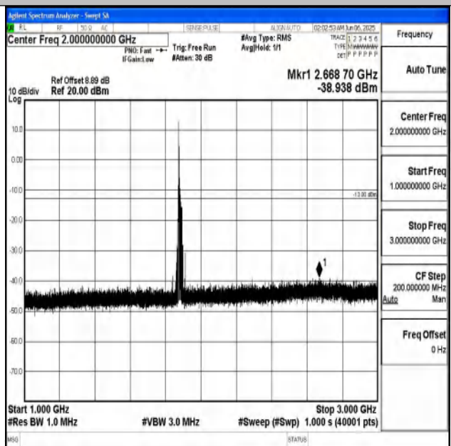
Band25_20MHz_QPSK_26365_1RB#0_1000~3000_100 0~3000
