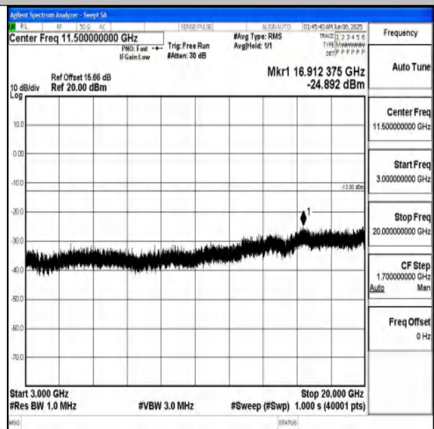
Band25_3MHz_16QAM_26675_1RB#0_3000~20000_30
