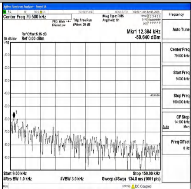
Band25_10MHz_16QAM_26090_1RB#0_0.009~0.15_0.009~0.15
