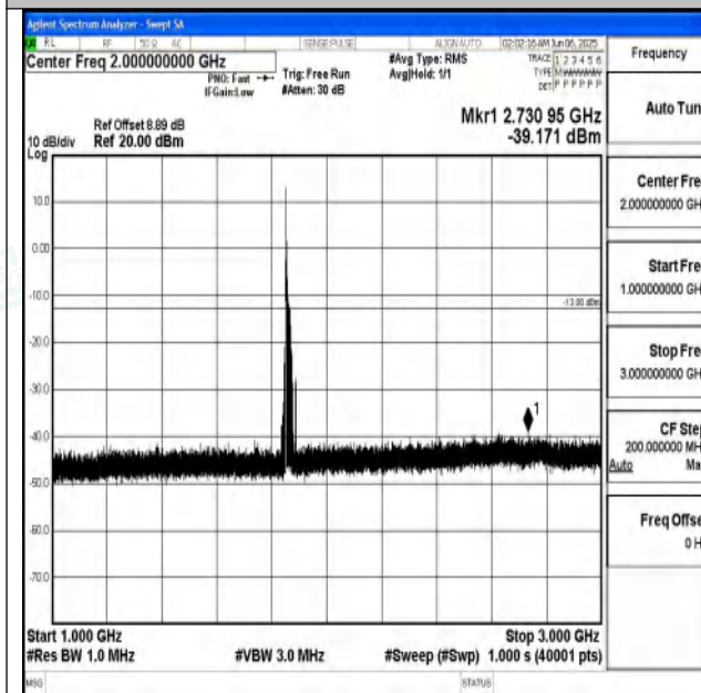
Band25_20MHz_16QAM_26140_1RB#0_1000~3000_1 000~3000
