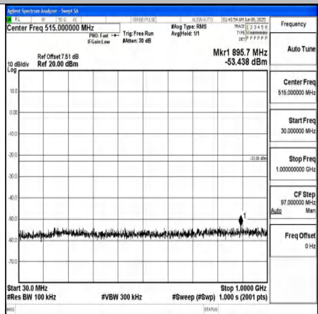
Band25_3MHz_16QAM_26365_1RB#0_30~1000_30~10 00
