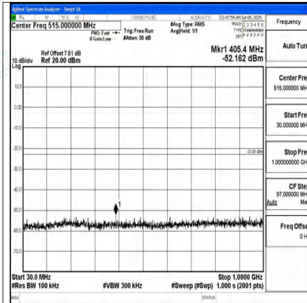
Band25_5MHz_QPSK_26365_1RB#0_30~1000_30~10
