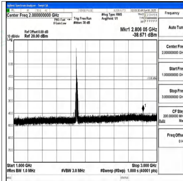
Band25_20MHz_16QAM_26365_1RB#0_1000~3000_1 000~3000
