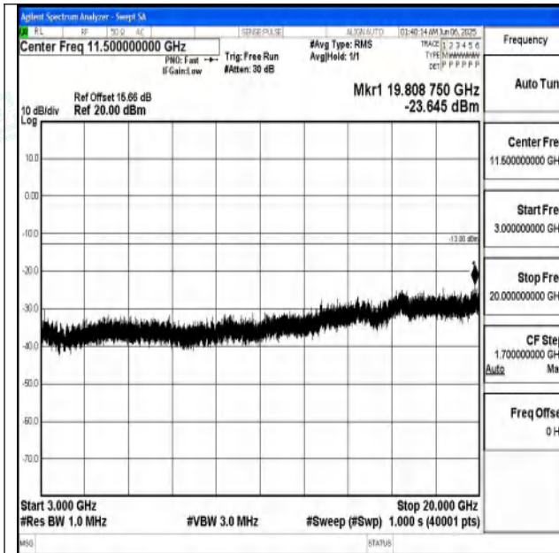
Band25_1.4MHz_QPSK_26683_1RB#0_3000~20000_3000~20000
