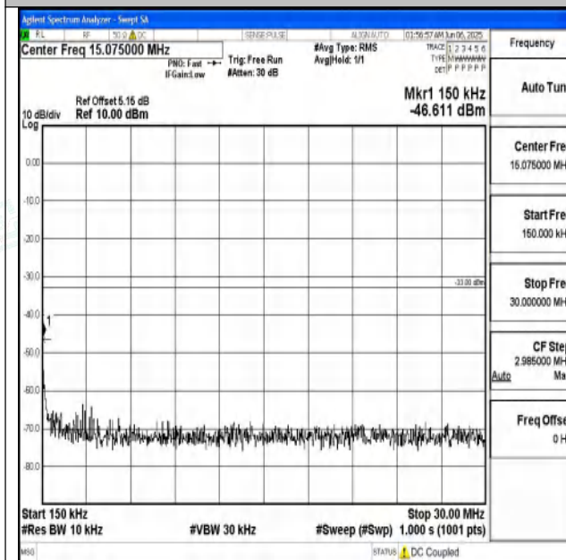
Band25_15MHz_16QAM_26115_1RB#0_0.15~30_0.15~30
