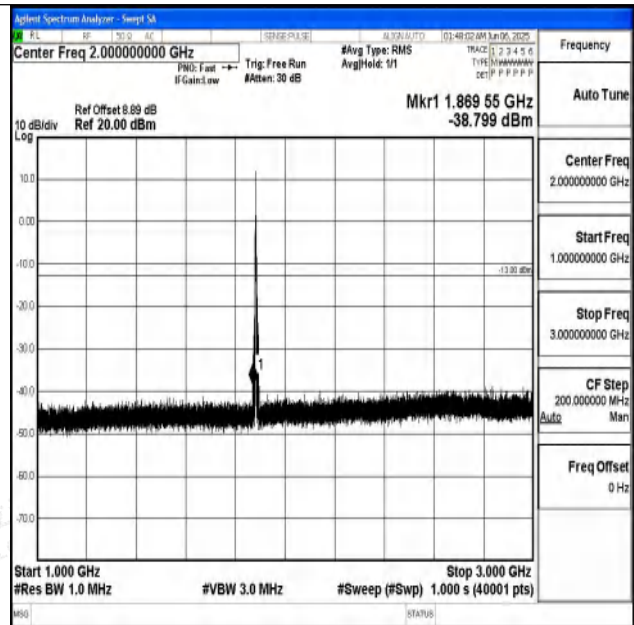
Band25_5MHz_QPSK_26365_1RB#0_1000~3000_1000
