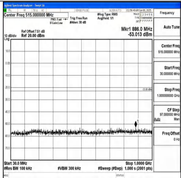
Band25_15MHz_16QAM_26615_1RB#0_30~1000_30~1000
