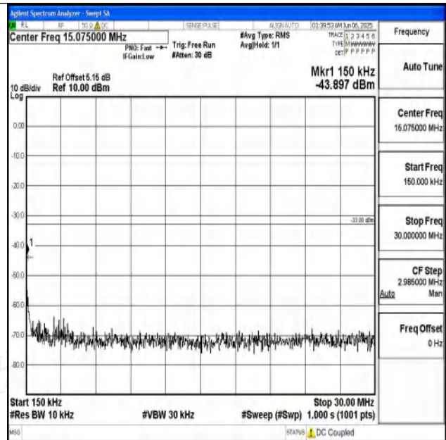
Band25_1.4MHz_QPSK_26683_1RB#0_0.15~30_0.15~30
