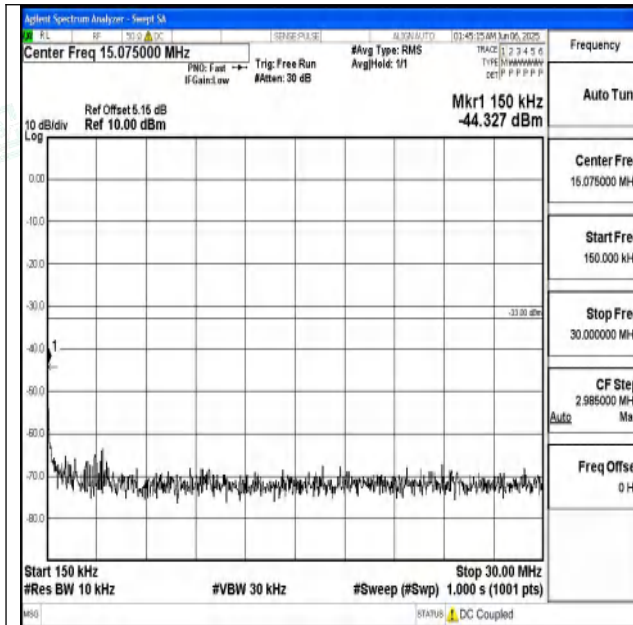
Band25_3MHz_16QAM_26675_1RB#0_0.15~30_0.15~
