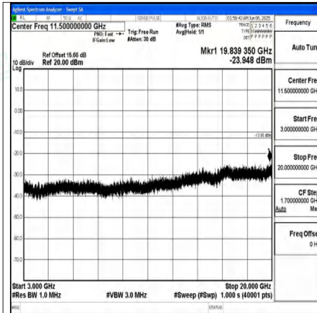
Band25_15MHz_QPSK_26115_1RB#0_3000~20000_3000~20000
