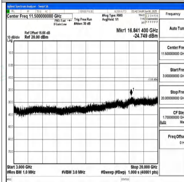
Band25_3MHz_QPSK_26055_1RB#0_3000~20000_30 00~20000
