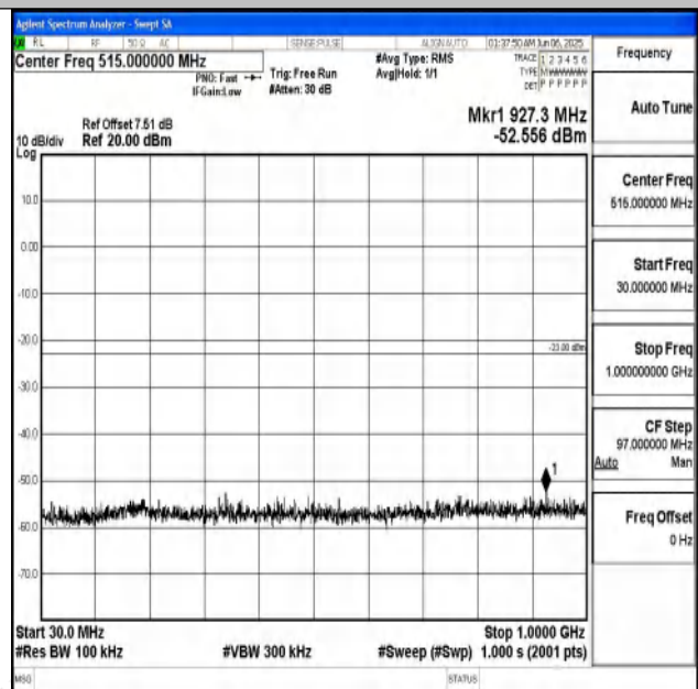
Band25_1.4MHz_16QAM_26047_1RB#0_30~1000_30~1000
