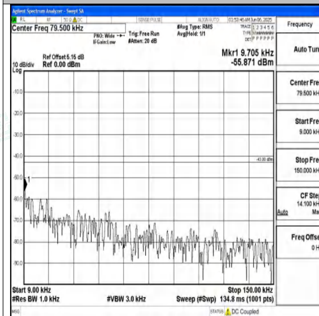
Band25_10MHz_QPSK_26640_1RB#0_0.009~0.15_0.0 09~0.15
