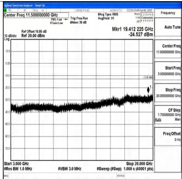
Band25_10MHz_16QAM_26365_1RB#0_3000~20000_3 000~20000
