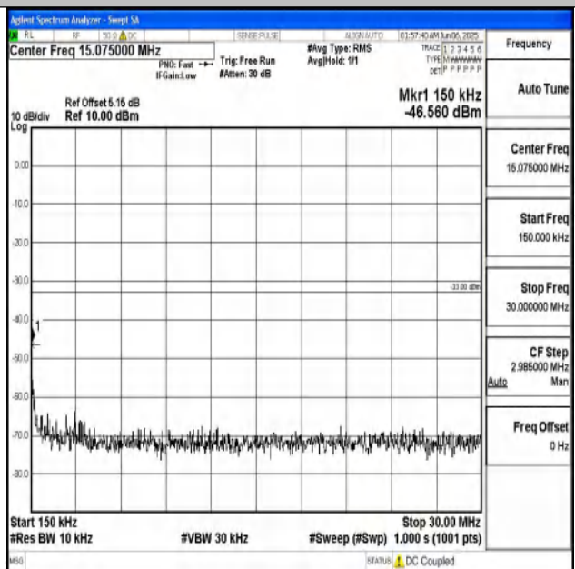
Band25_15MHz_QPSK_26365_1RB#0_0.15~30_0.15~30 0
