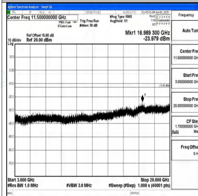
Band25_3MHz_QPSK_26675_1RB#0_3000~20000_30
