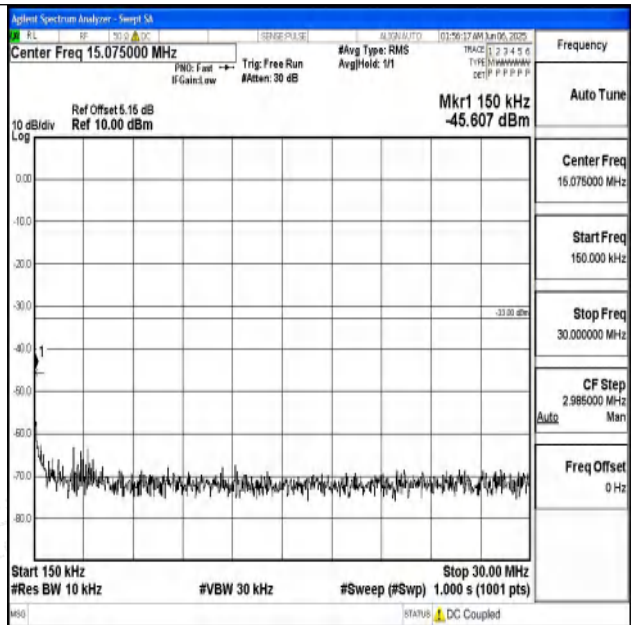
Band25_15MHz_QPSK_26115_1RB#0_0.15~30_0.15~3 0
