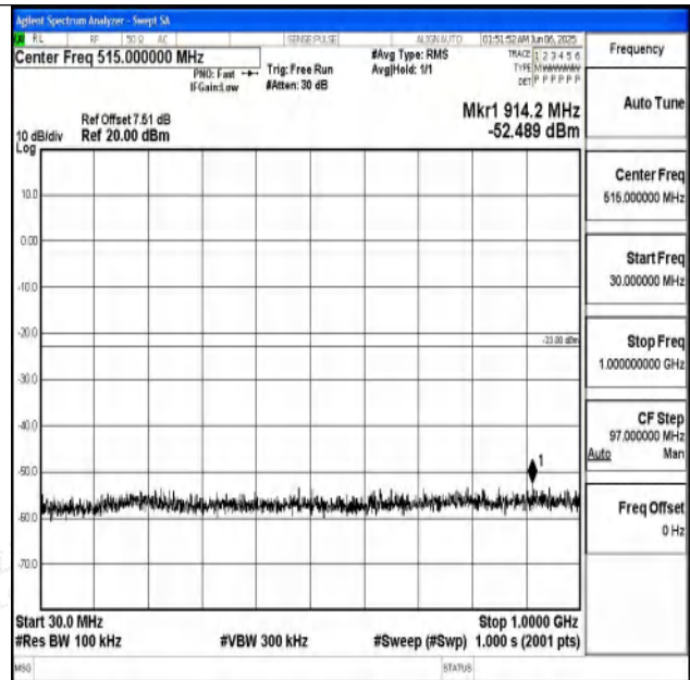
Band25_10MHz_16QAM_26090_1RB#0_30~1000_30~1 000
