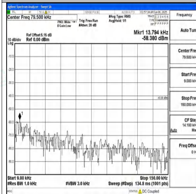
Band25_15MHz_QPSK_26365_1RB#0_0.009~0.15_0.0 09~0.15
