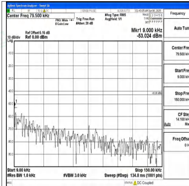
Band25_3MHz_QPSK_26365_1RB#0_0.009~0.15_0.00 9~0.15
