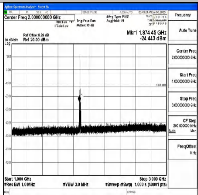
Band25_3MHz_QPSK_26365_1RB#0_1000~3000_1000 ~3000
