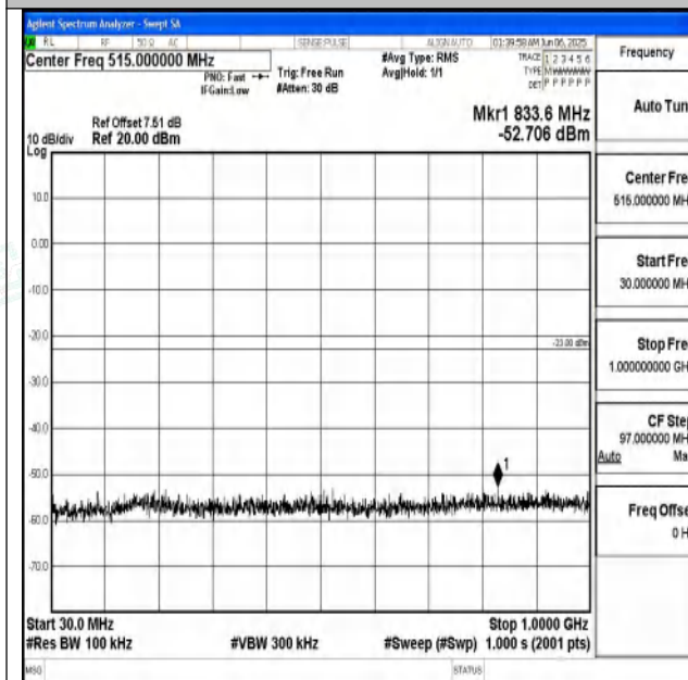
Band25_1.4MHz_QPSK_26683_1RB#0_30~1000_30~1000
