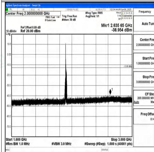
Band25_20MHz_16QAM_26590_1RB#0_1000~3000_1 000~3000
