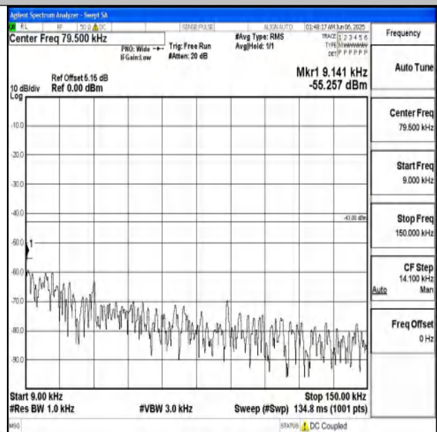
Band25_5MHz_16QAM_26365_1RB#0_0.009~0.15_0.00
