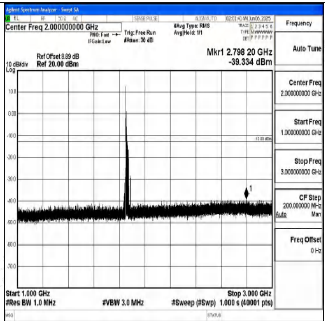
Band25_20MHz_QPSK_26140_1RB#0_1000~3000_100 0~3000
