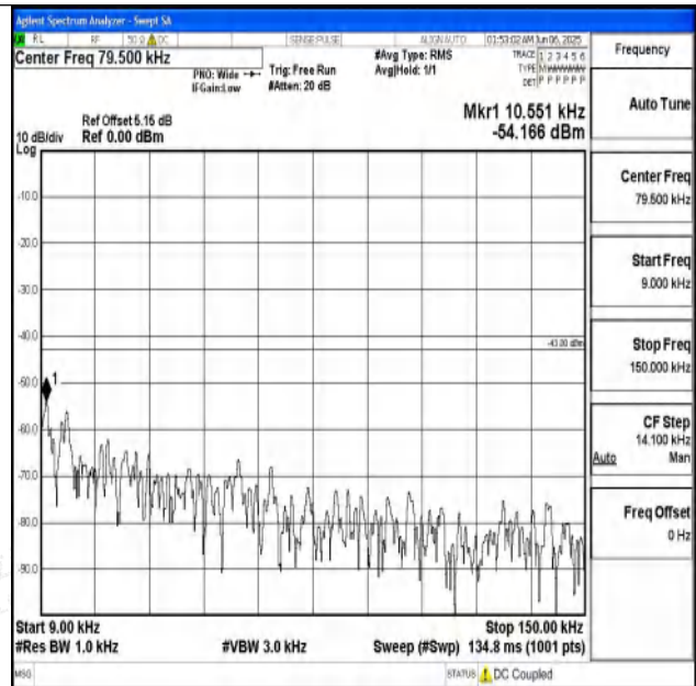
Band25_10MHz_16QAM_26365_1RB#0_0.009~0.15_0.009~0.15
