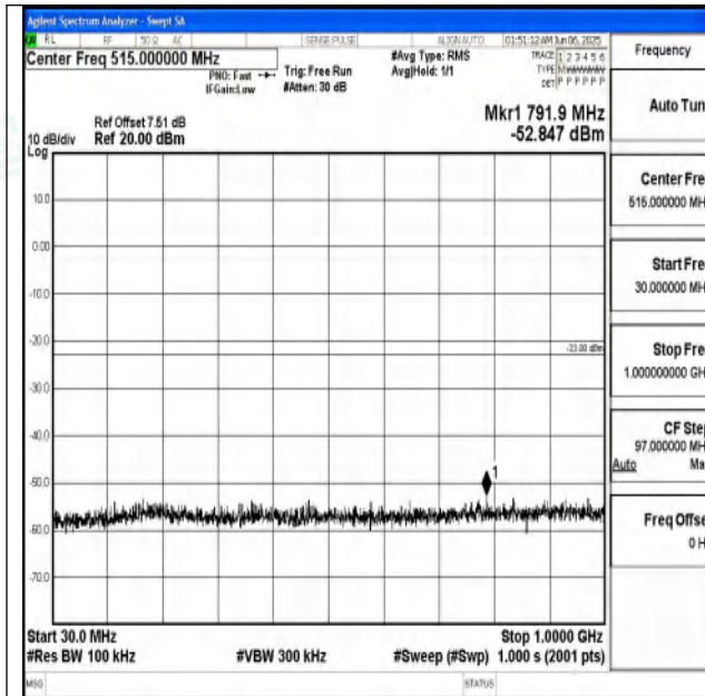
Band25_10MHz_QPSK_26090_1RB#0_30~1000_30~1000
