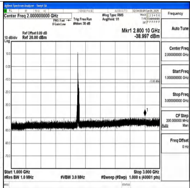
Band25_20MHz_QPSK_26590_1RB#0_1000~3000_1000~3000
