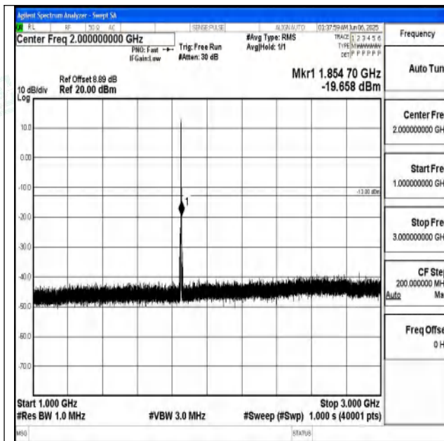
Band25_1.4MHz_16QAM_26047_1RB#0_1000~3000_1 000~3000
