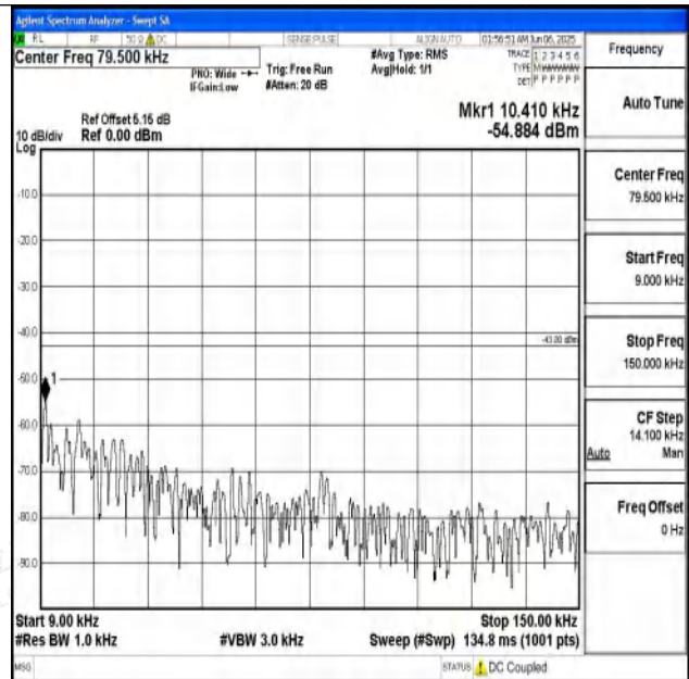
Band25_15MHz_16QAM_26115_1RB#0_0.009~0.15_0.09~0.15
