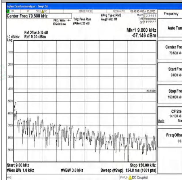
Band25_3MHz_QPSK_26055_1RB#0_0.009~0.15_0.00 9~0.15
