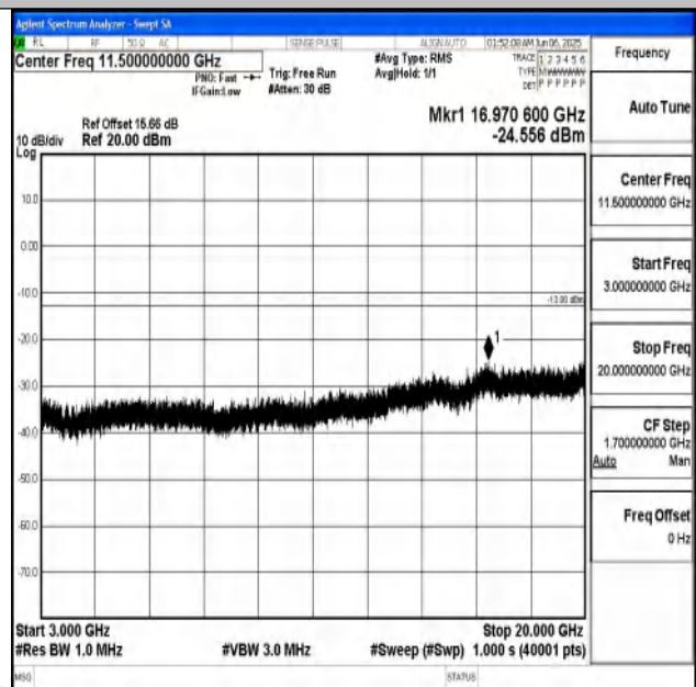
Band25_10MHz_16QAM_26090_1RB#0_3000~20000_3 000~20000
