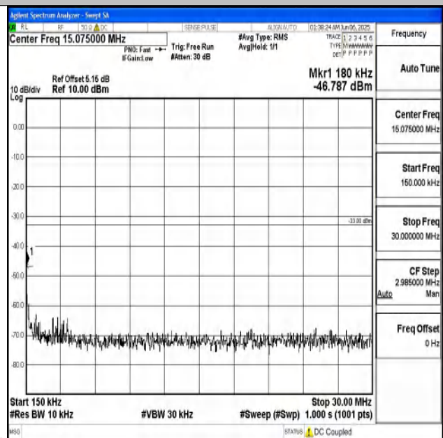
Band25_1.4MHz_QPSK_26365_1RB#0_0.15~30_0.15~30 0
