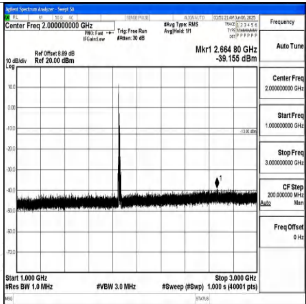
Band25_10MHz_QPSK_26090_1RB#0_1000~3000_1000~3000
