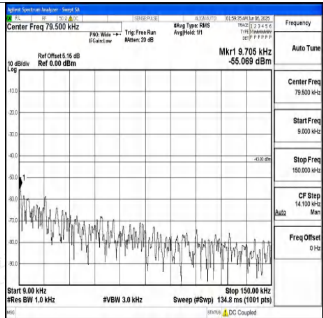
Band25_15MHz_16QAM_26615_1RB#0_0.009~0.15_0.09~0.15
