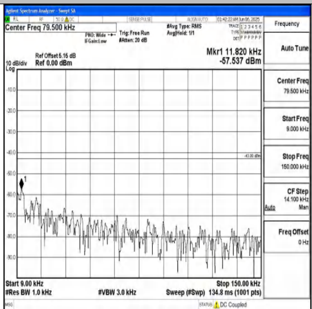
Band25_3MHz_16QAM_26055_1RB#0_0.009~0.15_0.00 9~0.15
