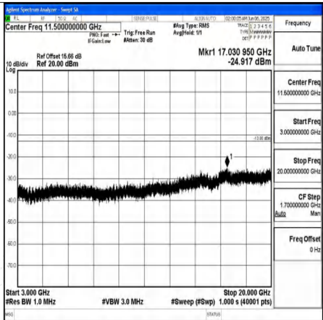
Band25_15MHz_16QAM_26615_1RB#0_3000~20000_3 000~20000
