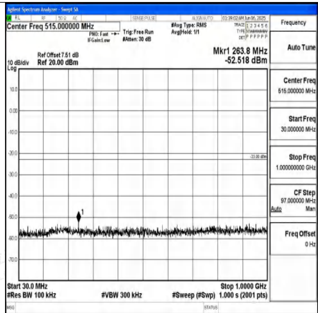
Band25_1.4MHz_16QAM_26365_1RB#0_30~1000_30~1 000
