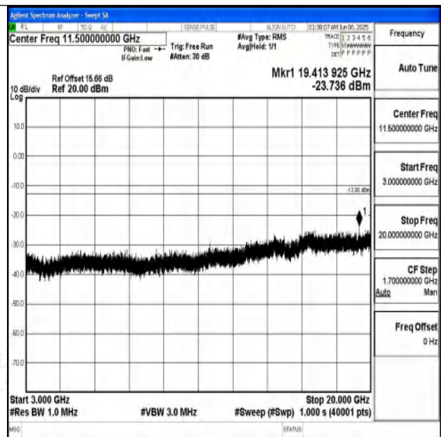
Band25_1.4MHz_16QAM_26047_1RB#0_3000~20000_3 000~20000
