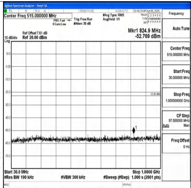
Band25_3MHz_16QAM_26055_1RB#0_30~1000_30~10
