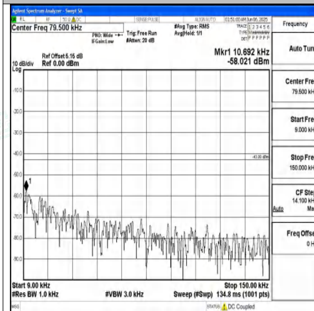
Band25_10MHz_QPSK_26090_1RB#0_0.009~0.15_0.0 09~0.15
