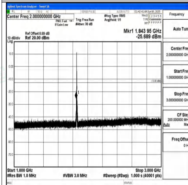
Band25_3MHz_16QAM_26055_1RB#0_1000~3000_10
