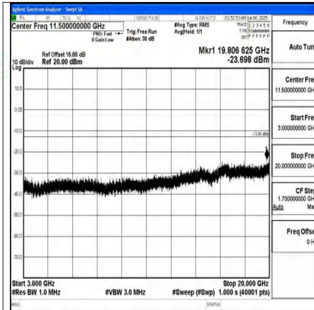
Band25_10MHz_QPSK_26365_1RB#0_3000~20000_3000~20000
