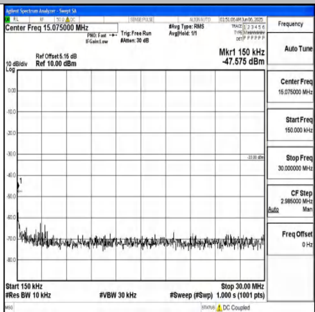
Band25_10MHz_QPSK_26090_1RB#0_0.15~30_0.15~3 0
