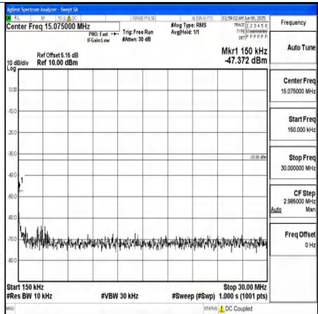
Band25_15MHz_QPSK_26615_1RB#0_0.15~30_0.15~3 0
