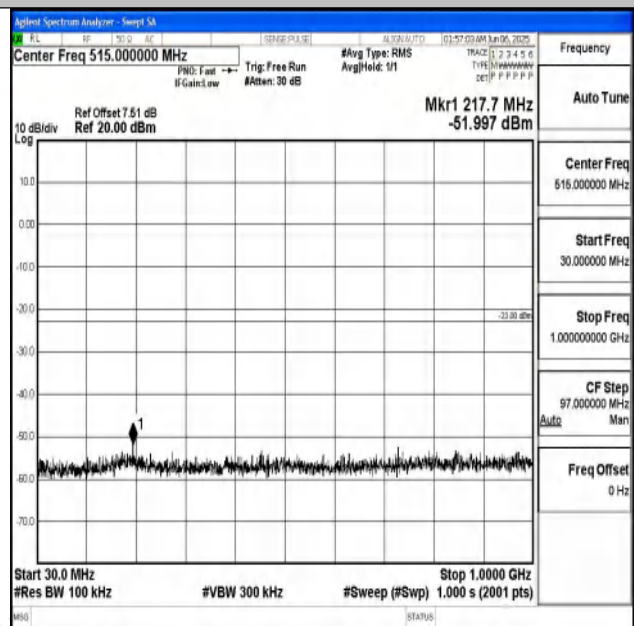
Band25_15MHz_16QAM_26115_1RB#0_30~1000_30~1000
