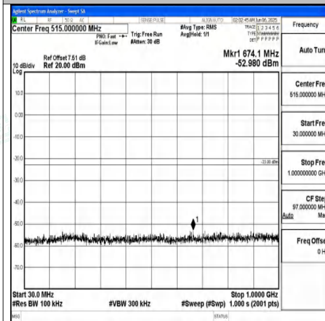
Band25_20MHz_QPSK_26365_1RB#0_30~1000_30~1 000
