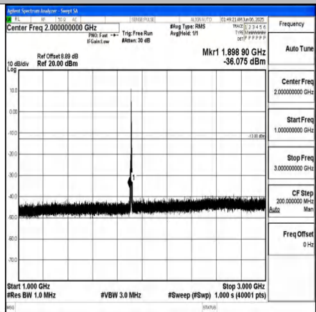
Band25_5MHz_QPSK_26665_1RB#0_1000~3000_1000 ~3000
