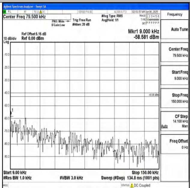
Band25_20MHz_16QAM_26140_1RB#0_0.009~0.15_0.0 09~0.15
