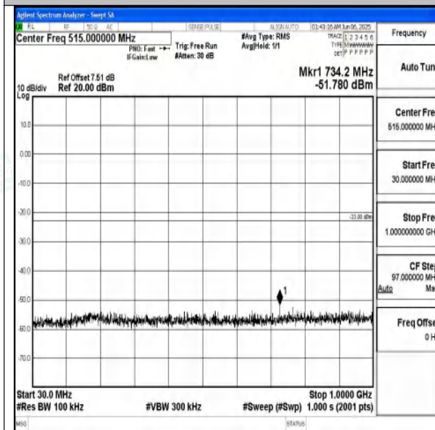
Band25_3MHz_QPSK_26365_1RB#0_30~1000_30~10 00
