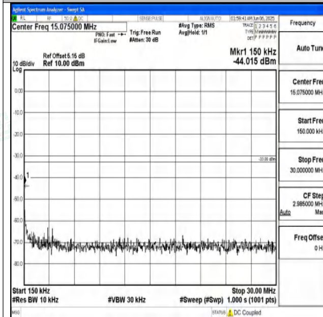
Band25_15MHz_16QAM_26615_1RB#0_0.15~30_0.15~30
