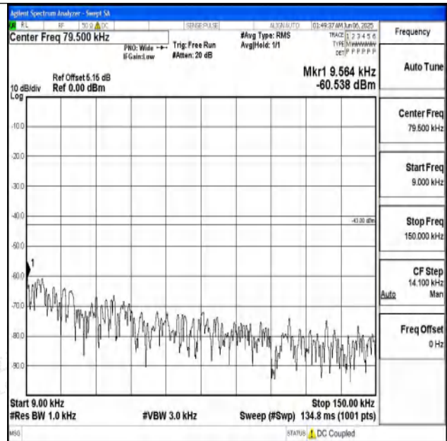
Band25_5MHz_16QAM_26665_1RB#0_0.009~0.15_0.009~0.15
