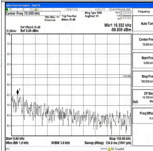
Band25_3MHz_QPSK_26675_1RB#0_0.009~0.15_0.009~0.15
