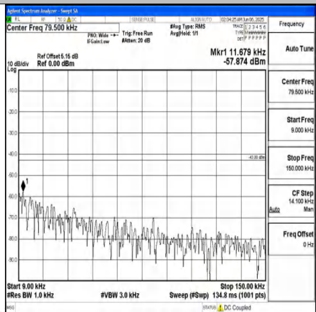
Band25_20MHz_16QAM_26590_1RB#0_0.009~0.15_0.009~0.15
