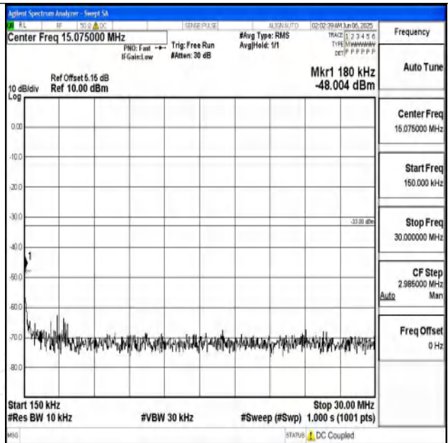
Band25_20MHz_QPSK_26365_1RB#0_0.15~30_0.15~3 0
