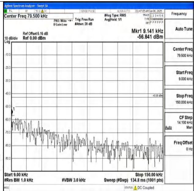
Band25_5MHz_16QAM_26065_1RB#0_0.009~0.15_0.009~0.15
