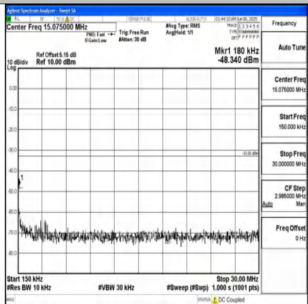
Band25_3MHz_QPSK_26675_1RB#0_0.15~30_0.15~30
