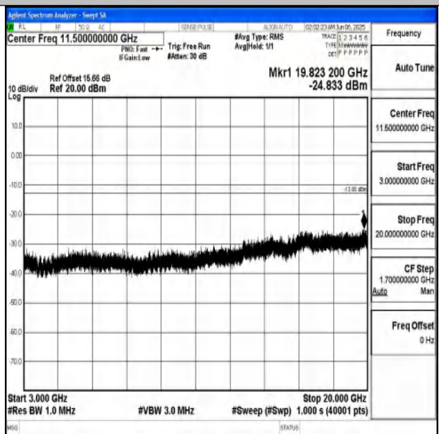
Band25_20MHz_16QAM_26140_1RB#0_3000~20000_3 000~20000
