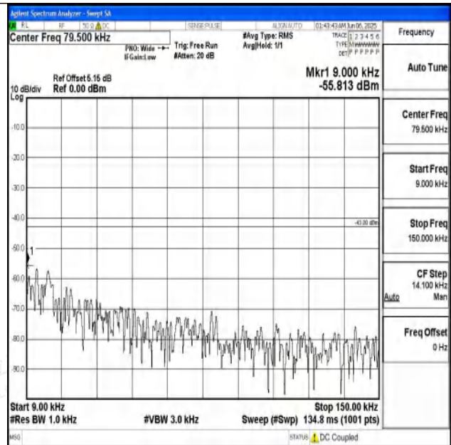
Band25_3MHz_16QAM_26365_1RB#0_0.009~0.15_0.00 9~0.15
