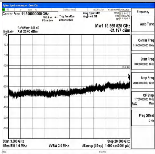
Band25_15MHz_16QAM_26365_1RB#0_3000~20000_3 000~20000
