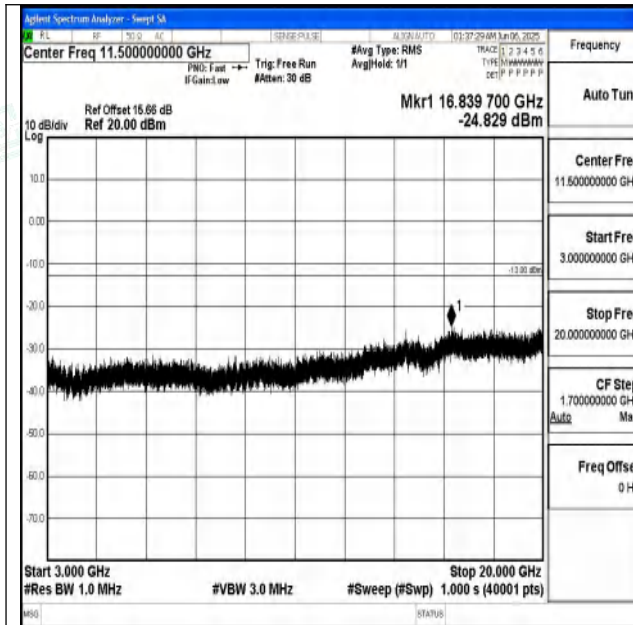
Band25_1.4MHz_QPSK_26047_1RB#0_3000~20000_3000~20000
