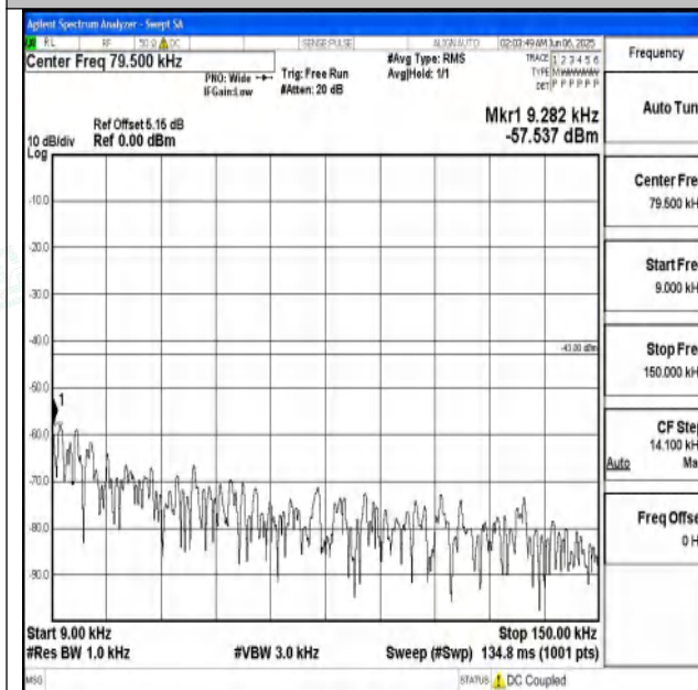
Band25_20MHz_QPSK_26590_1RB#0_0.009~0.15_0.0 09~0.15
