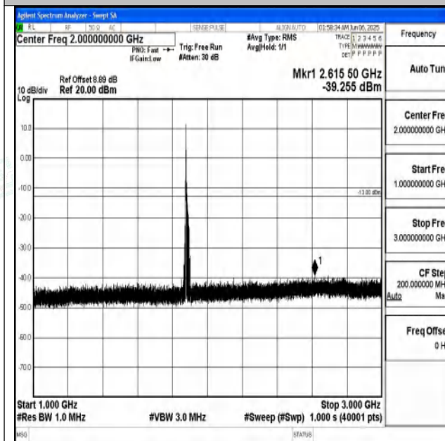
Band25_15MHz_16QAM_26365_1RB#0_1000~3000_1 000~3000
