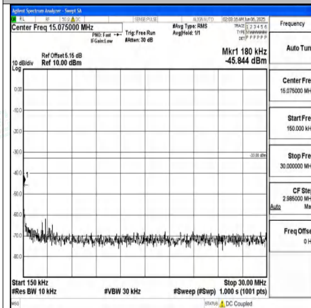
Band25_20MHz_16QAM_26365_1RB#0_0.15~30_0.15~30
