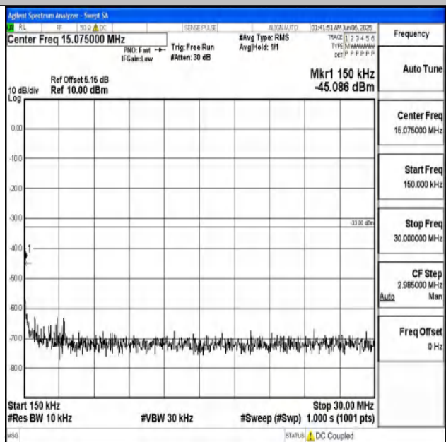
Band25_3MHz_QPSK_26055_1RB#0_0.15~30_0.15~30
