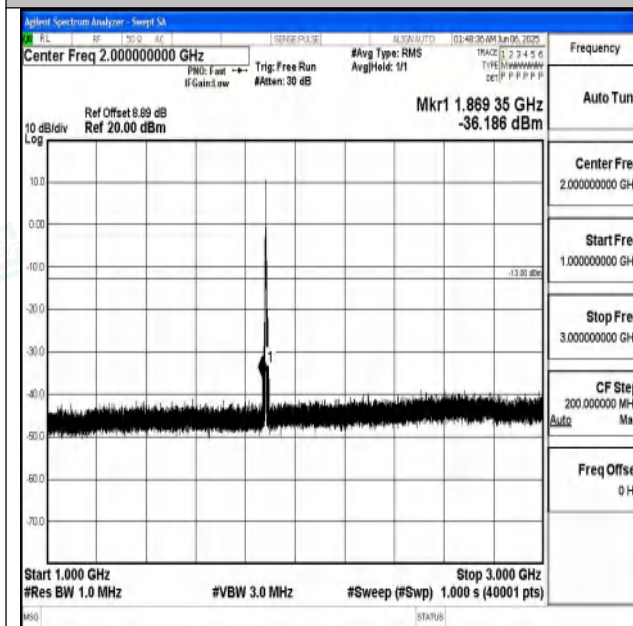
Band25_5MHz_16QAM_26365_1RB#0_1000~3000_10
