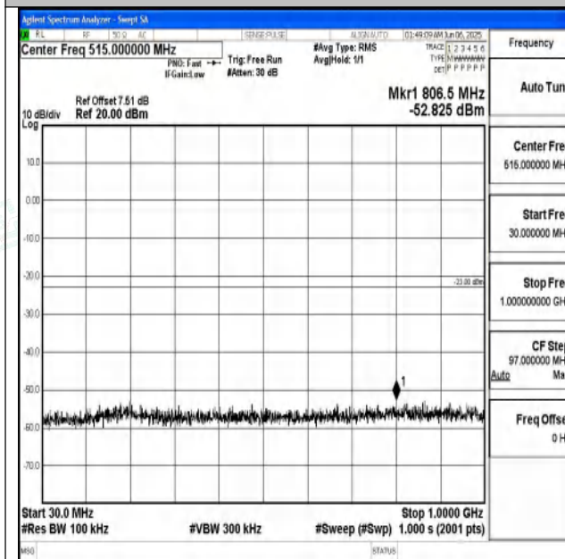
Band25_5MHz_QPSK_26665_1RB#0_30~1000_30~10 00
