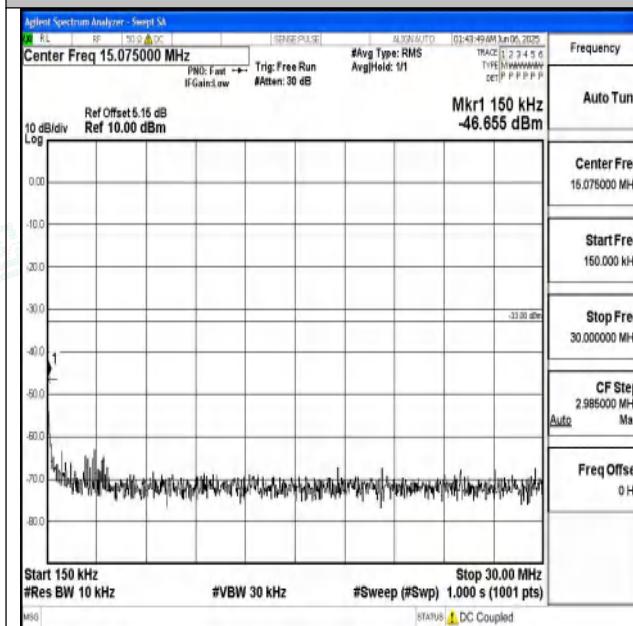
Band25_3MHz_16QAM_26365_1RB#0_0.15~30_0.15~ 30
