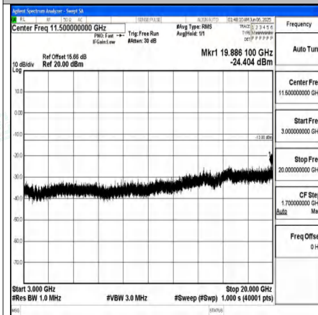
Band25_5MHz_QPSK_26365_1RB#0_3000~20000_30
