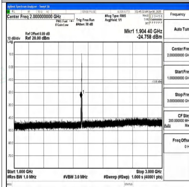
Band25_3MHz_16QAM_26675_1RB#0_1000~3000_10
