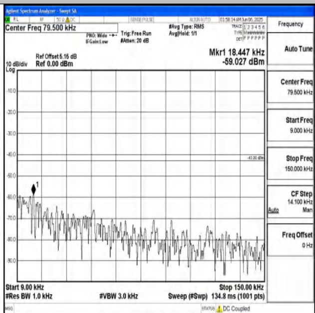
Band25_15MHz_16QAM_26365_1RB#0_0.009~0.15_0.009~0.15
