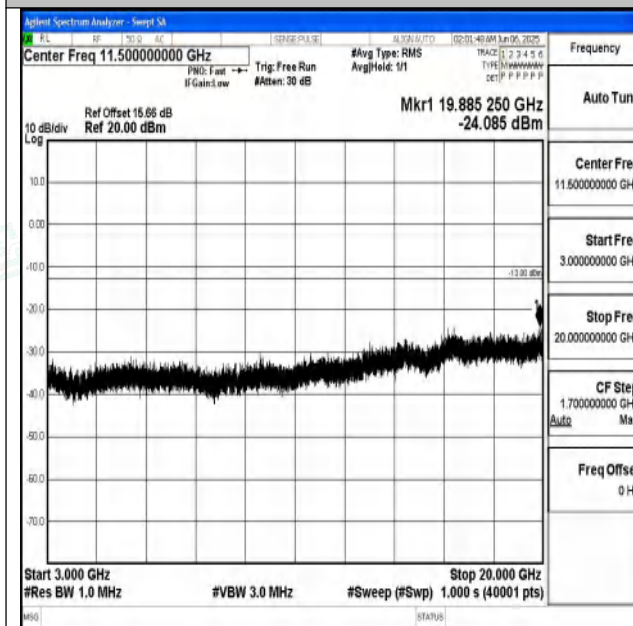
Band25_20MHz_QPSK_26140_1RB#0_3000~20000_3 000~20000
