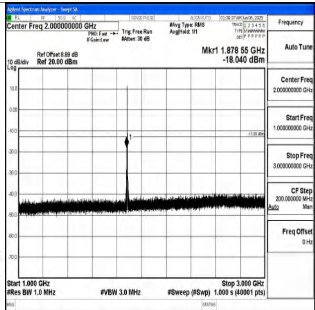
Band25_1.4MHz_QPSK_26365_1RB#0_1000~3000_1000~3000
