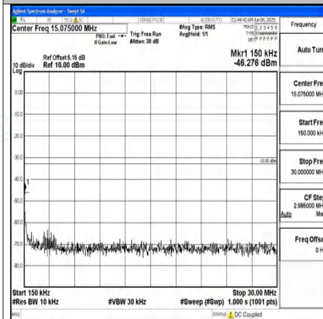
Band25_5MHz_16QAM_26665_1RB#0_0.15~30_0.15~30
