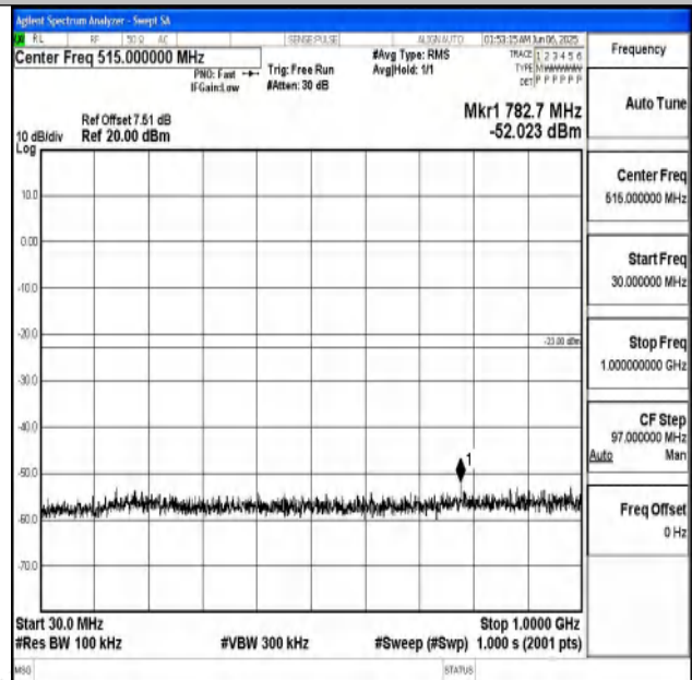
Band25_10MHz_16QAM_26365_1RB#0_30~1000_30~1000
