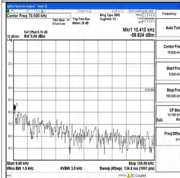
Band25_20MHz_QPSK_26140_1RB#0_0.009~0.15_0.0 09~0.15
