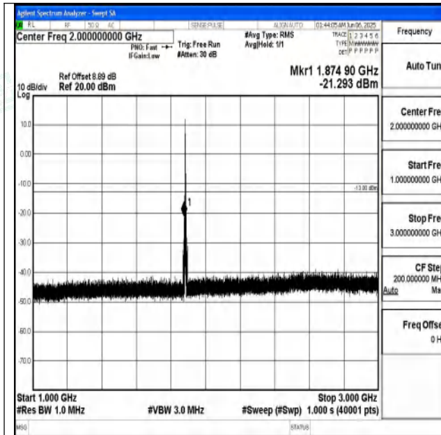
Band25_3MHz_16QAM_26365_1RB#0_1000~3000_1000~3000
