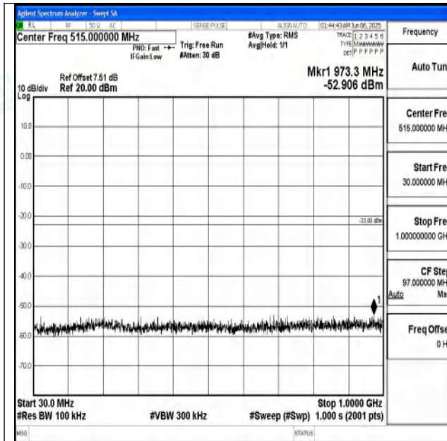
Band25_3MHz_QPSK_26675_1RB#0_30~1000_30~10
