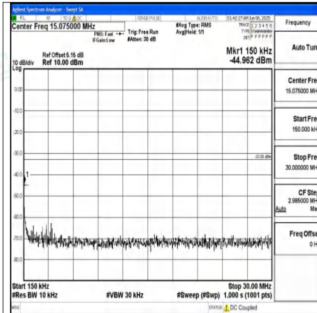
Band25_3MHz_16QAM_26055_1RB#0_0.15~30_0.15~
