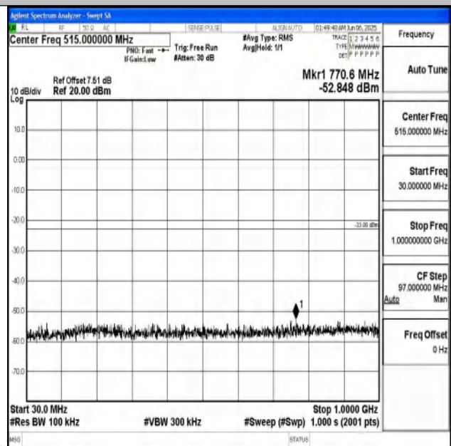
Band25_5MHz_16QAM_26665_1RB#0_30~1000_30~1000
