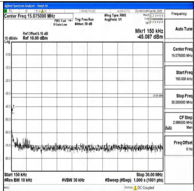
Band25_5MHz_QPSK_26665_1RB#0_0.15~30_0.15~30
