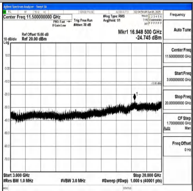
Band25_20MHz_16QAM_26590_1RB#0_3000~20000_3 000~20000
