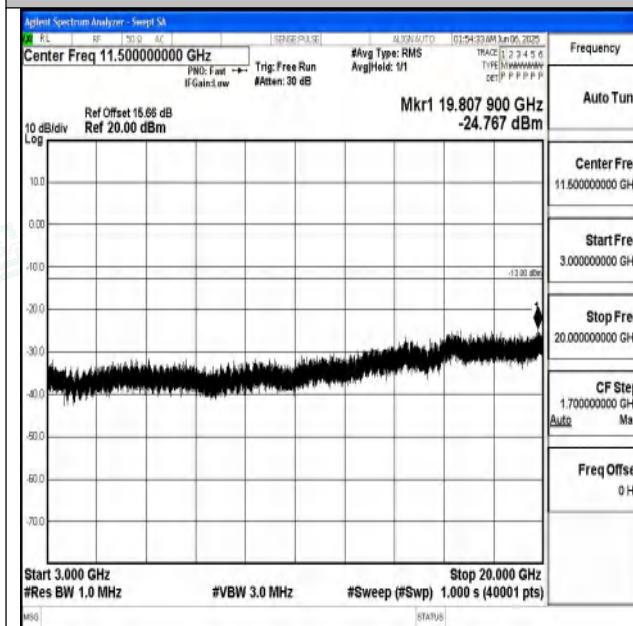
Band25_10MHz_QPSK_26640_1RB#0_3000~20000_3000~20000
