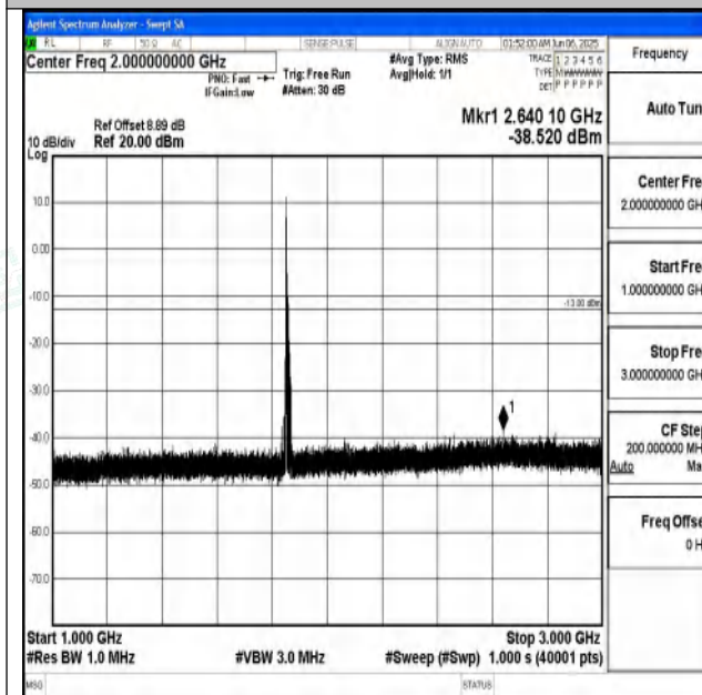
Band25_10MHz_16QAM_26090_1RB#0_1000~3000_1 000~3000
