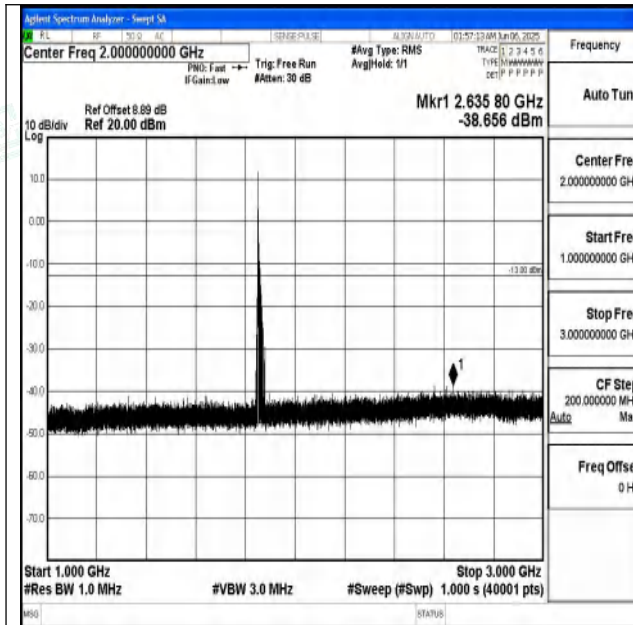
Band25_15MHz_16QAM_26115_1RB#0_1000~3000_1 000~3000
