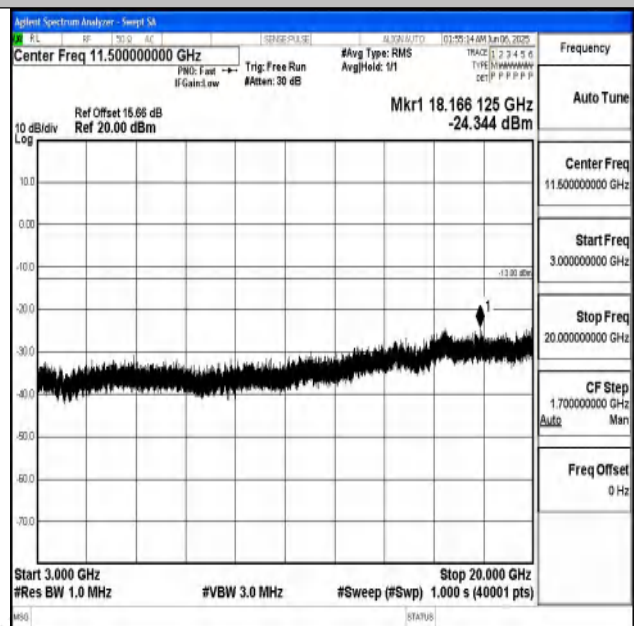
Band25_10MHz_16QAM_26640_1RB#0_3000~20000_3 000~20000
