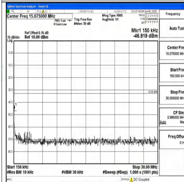
Band25_1.4MHz_16QAM_26047_1RB#0_0.15~30_0.15~30
