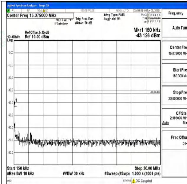
Band25_20MHz_16QAM_26590_1RB#0_0.15~30_0.15 ~30
