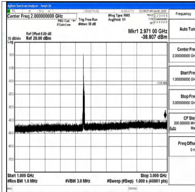
Band25_15MHz_16QAM_26615_1RB#0_1000~3000_1 000~3000
