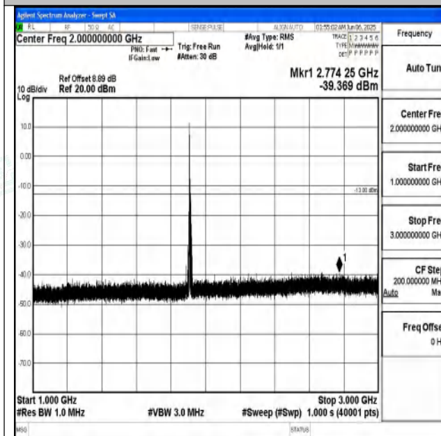
Band25_10MHz_16QAM_26640_1RB#0_1000~3000_1 000~3000
