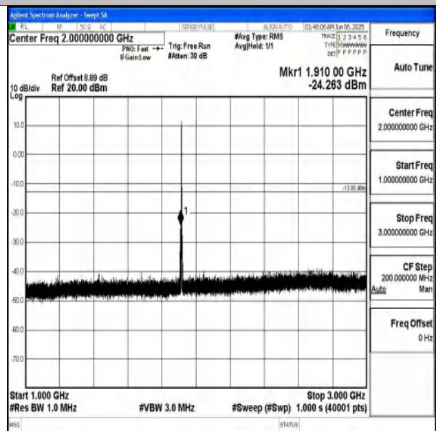
Band25_1.4MHz_QPSK_26683_1RB#0_1000~3000_1000~3000
