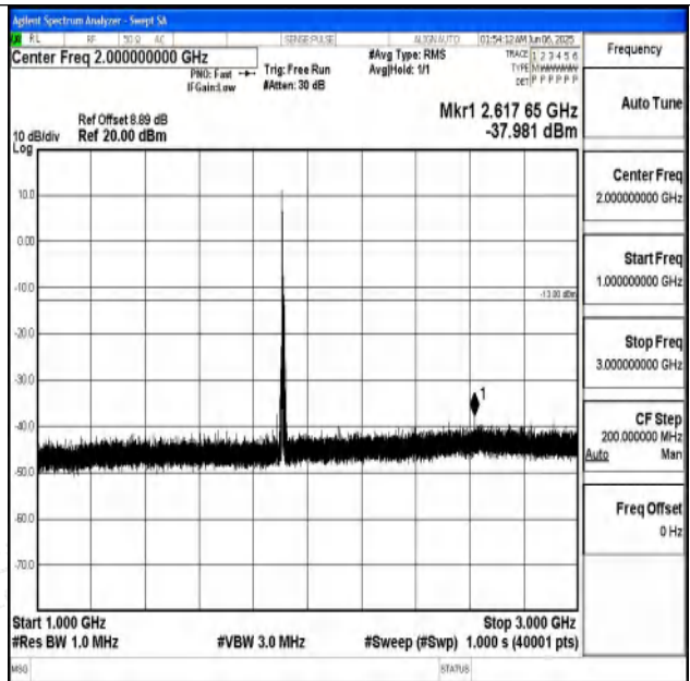
Band25_10MHz_QPSK_26640_1RB#0_1000~3000_1000~3000
