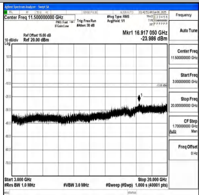
Band25_3MHz_16QAM_26055_1RB#0_3000~20000_30
