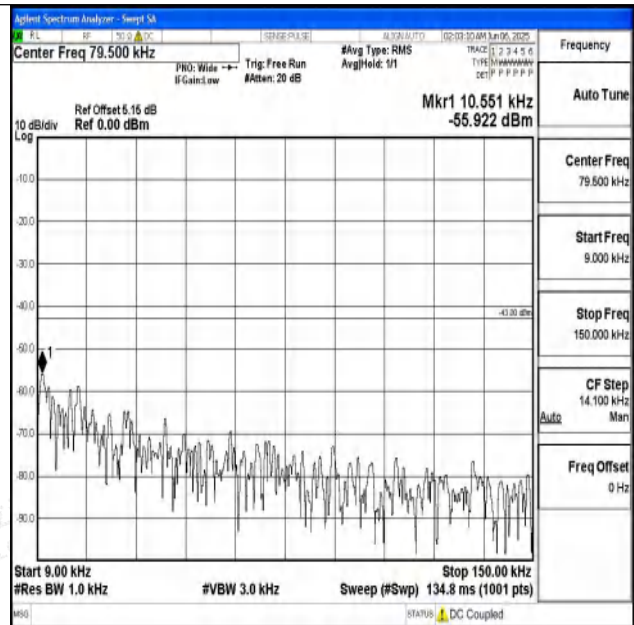
Band25_20MHz_16QAM_26365_1RB#0_0.009~0.15_0.009~0.15
