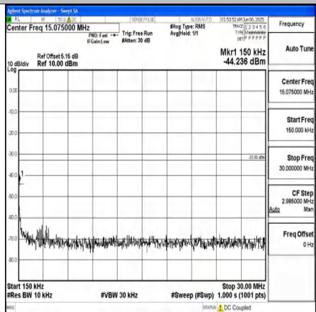
Band25_10MHz_QPSK_26640_1RB#0_0.15~30_0.15~3 0
