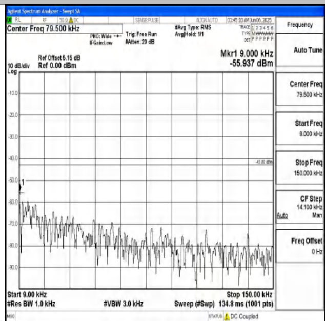
Band25_3MHz_16QAM_26675_1RB#0_0.009~0.15_0.00
