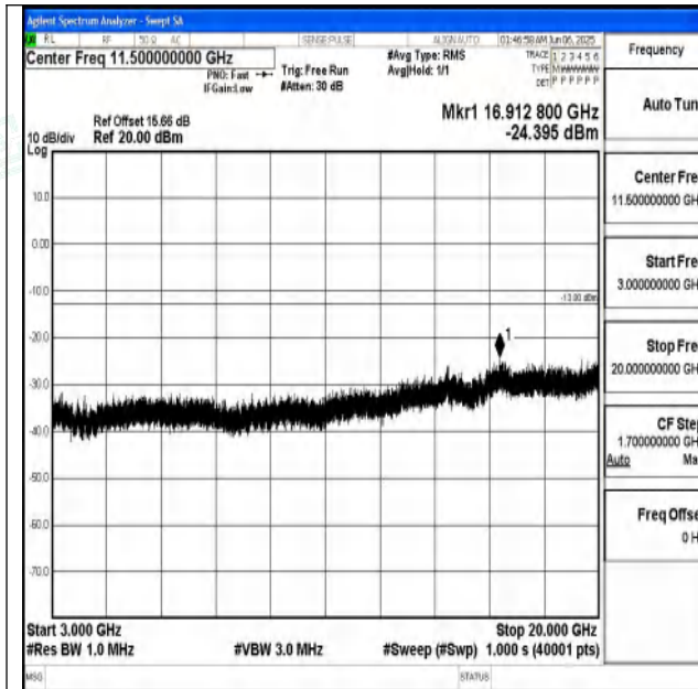
Band25_5MHz_QPSK_26065_1RB#0_3000~20000_3000~20000
