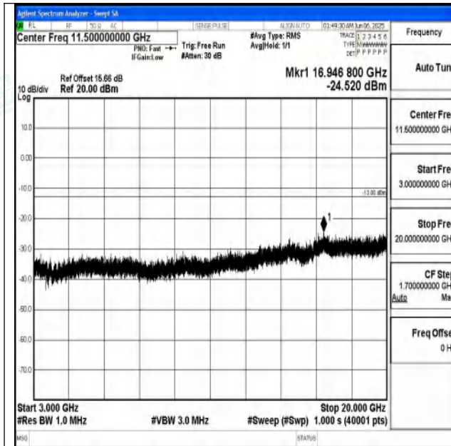
Band25_5MHz_QPSK_26665_1RB#0_3000~20000_3000~20000
