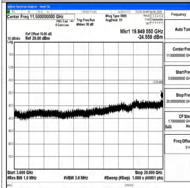
Band25_10MHz_QPSK_26090_1RB#0_3000~20000_3000~20000
