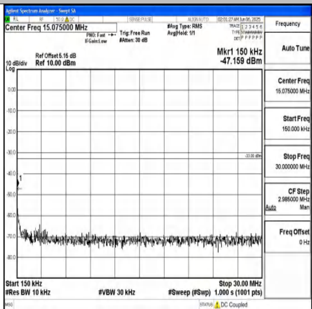
Band25_20MHz_QPSK_26140_1RB#0_0.15~30_0.15~3 0
