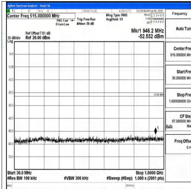
Band25_10MHz_QPSK_26640_1RB#0_30~1000_30~1000
