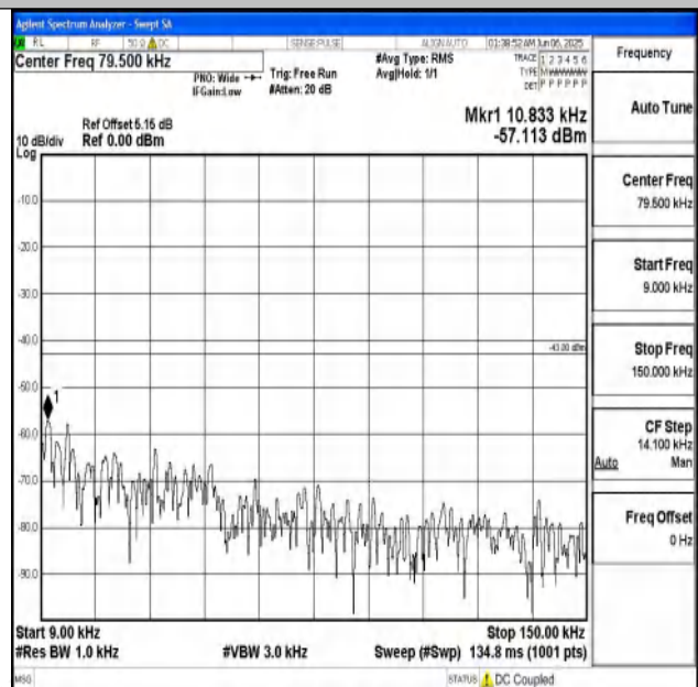
Band25_1.4MHz_16QAM_26365_1RB#0_0.009~0.15_0.009~0.15
