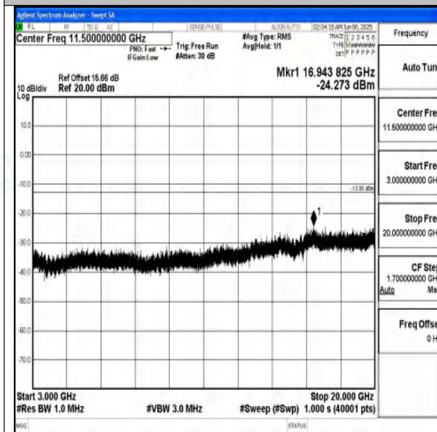
Band25_20MHz_QPSK_26590_1RB#0_3000~20000_3000~20000
