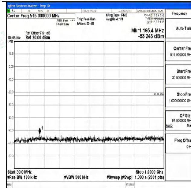
Band25_20MHz_QPSK_26140_1RB#0_30~1000_30~1 000
