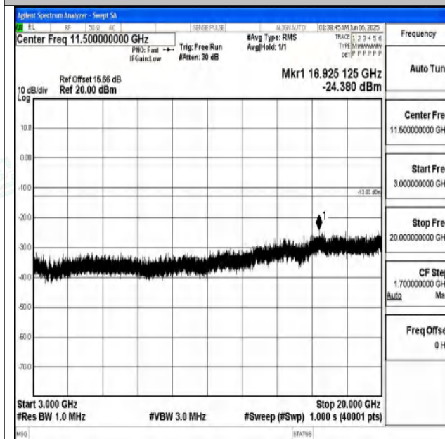
Band25_1.4MHz_QPSK_26365_1RB#0_3000~20000_3000~20000
