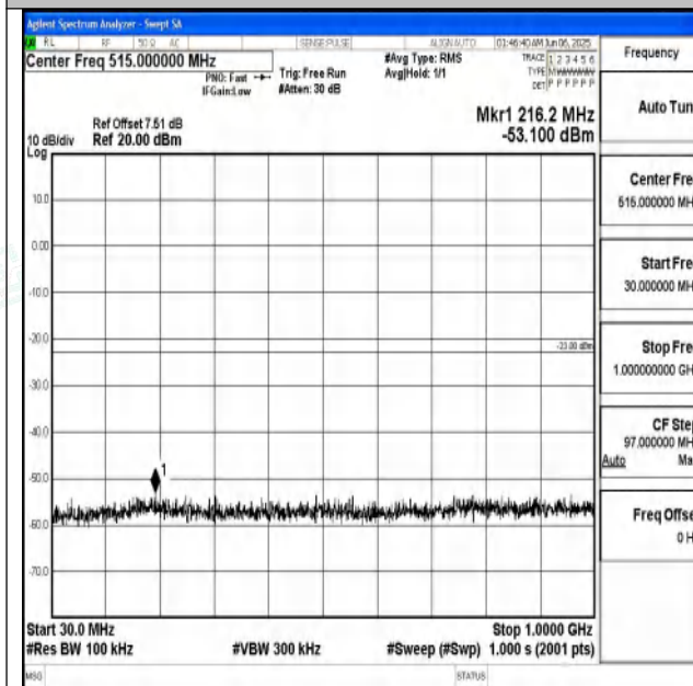
Band25_5MHz_QPSK_26065_1RB#0_30~1000_30~10 00
