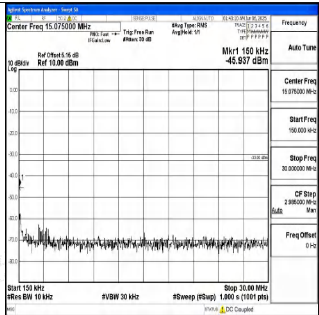
Band25_3MHz_QPSK_26365_1RB#0_0.15~30_0.15~30
