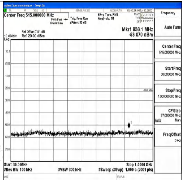
Band25_3MHz_16QAM_26675_1RB#0_30~1000_30~10
