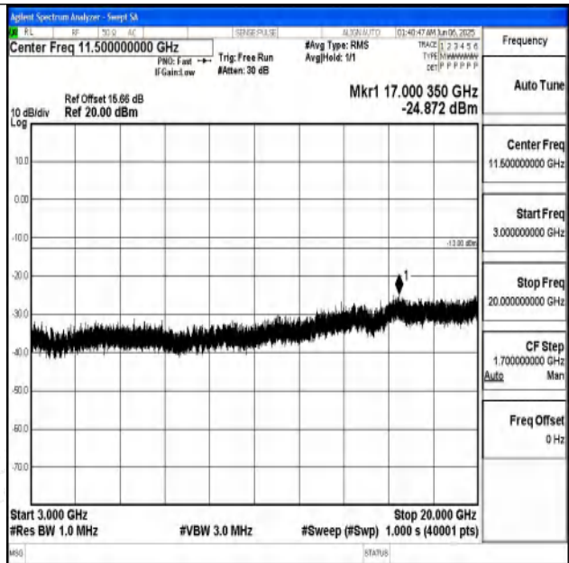
Band25_1.4MHz_16QAM_26683_1RB#0_3000~20000_3 000~20000
