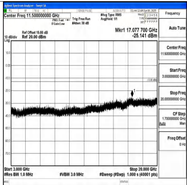
Band25_3MHz_16QAM_26365_1RB#0_3000~20000_3000~20000
