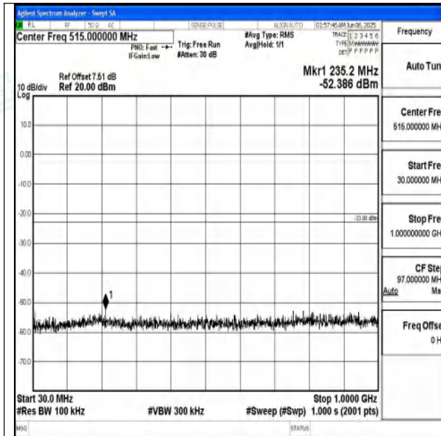
Band25_15MHz_QPSK_26365_1RB#0_30~1000_30~1000
