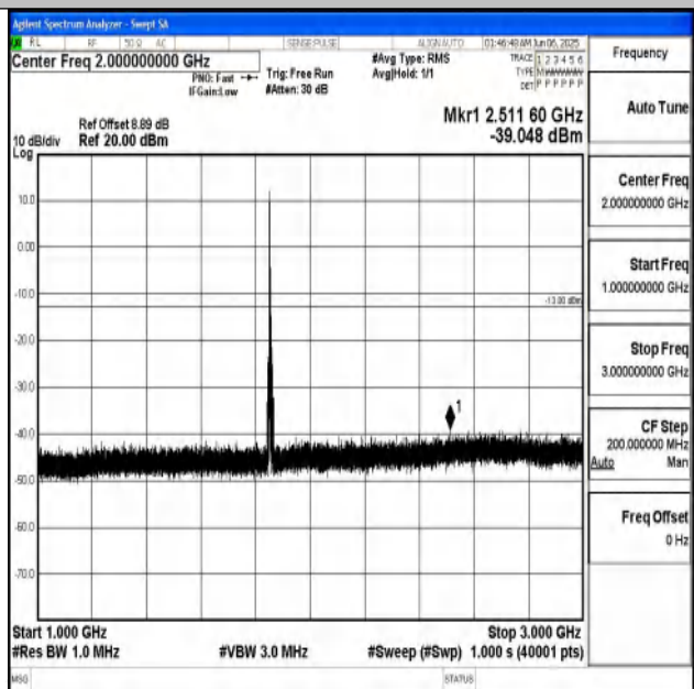
Band25_5MHz_QPSK_26065_1RB#0_1000~3000_1000 ~3000
