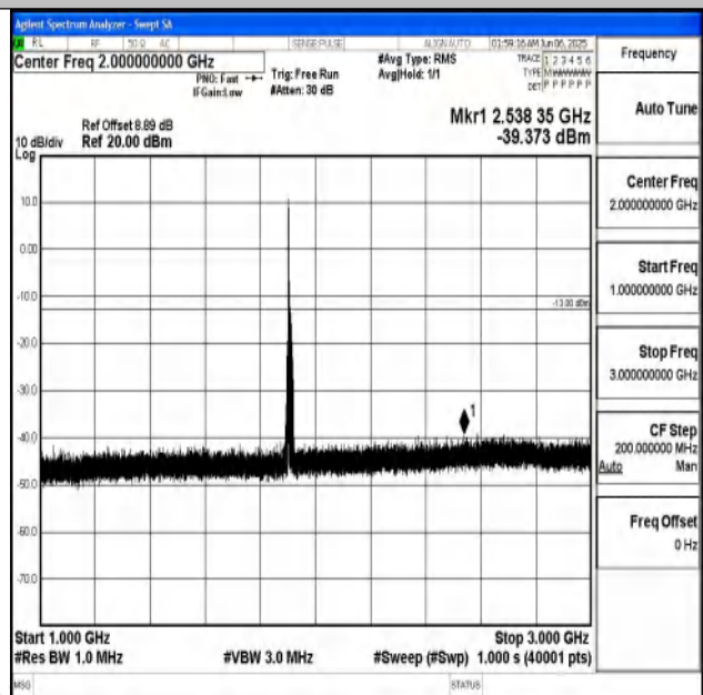
Band25_15MHz_QPSK_26615_1RB#0_1000~3000_100 0~3000
