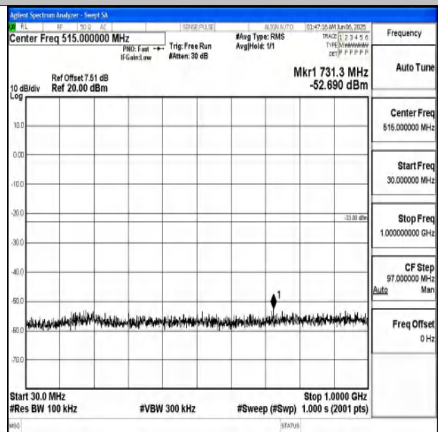
Band25_5MHz_16QAM_26065_1RB#0_30~1000_30~1000
