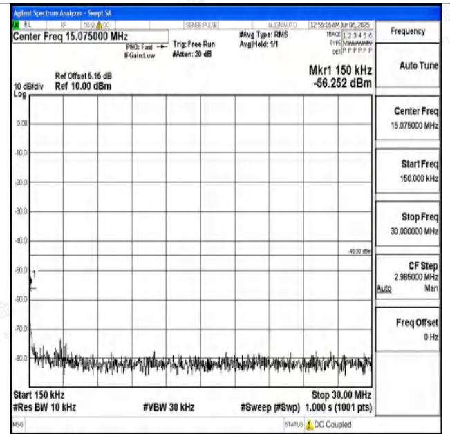
Band7_15MHz_QPSK_20825_1RB#0_0.15~30_0.15~30
