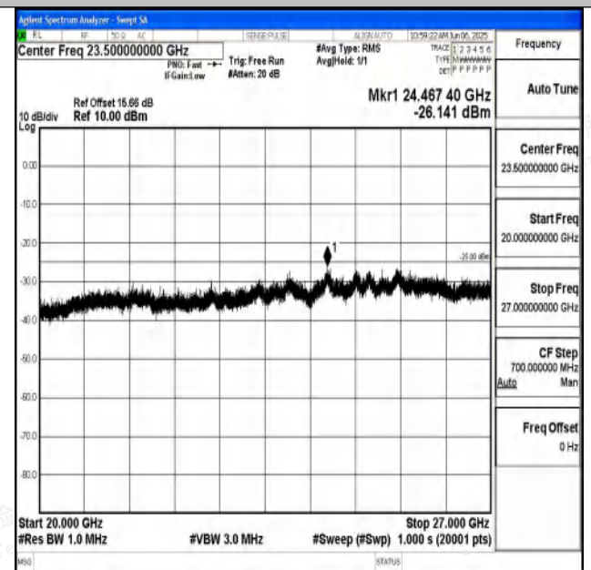
Band7_5MHz_16QAM_21425_1RB#0_20000~27000_20000~27000
