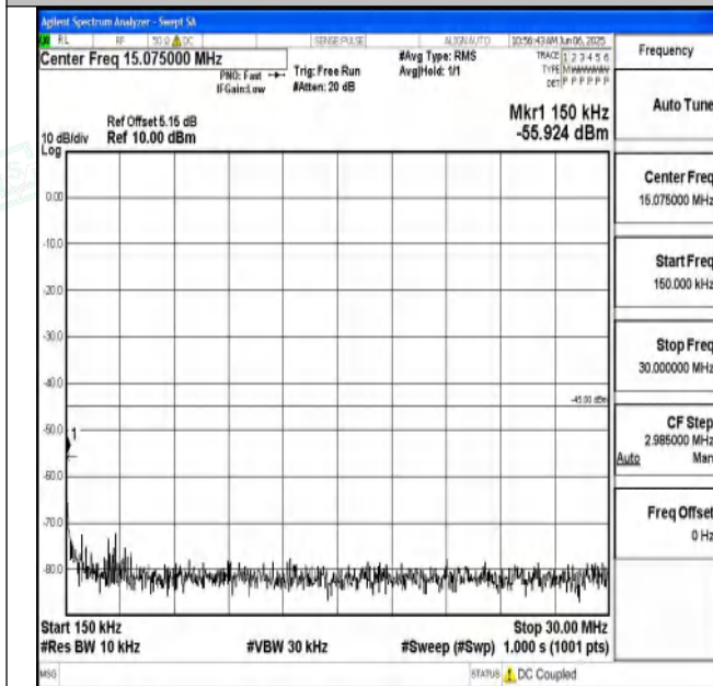
Band7_5MHz_16QAM_20775_1RB#0_0.15~30_0.15~30
