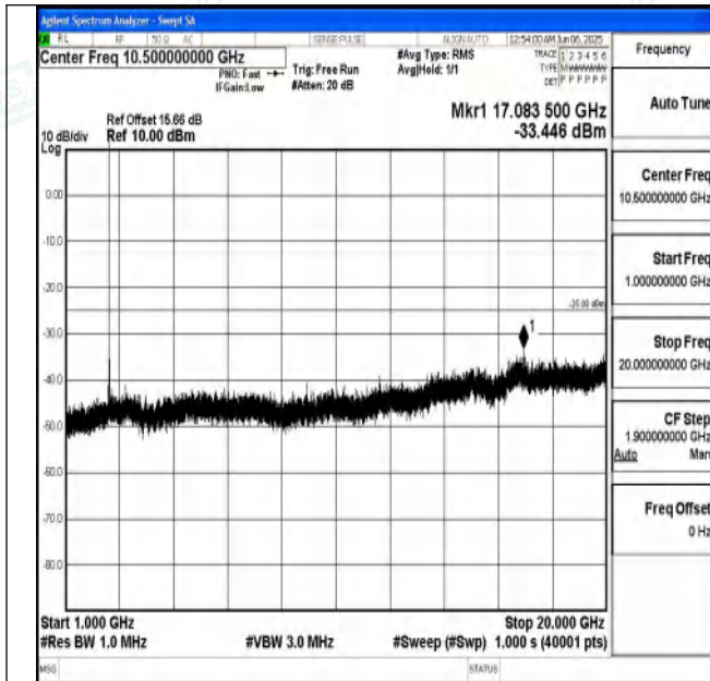
Band7_10MHz_16QAM_21100_1RB#0_1000~20000_1000~20000
