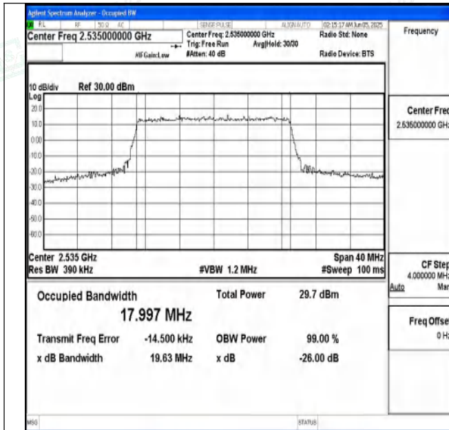
Band7-20MHz-QPSK-21100-100RB#0-PASS
