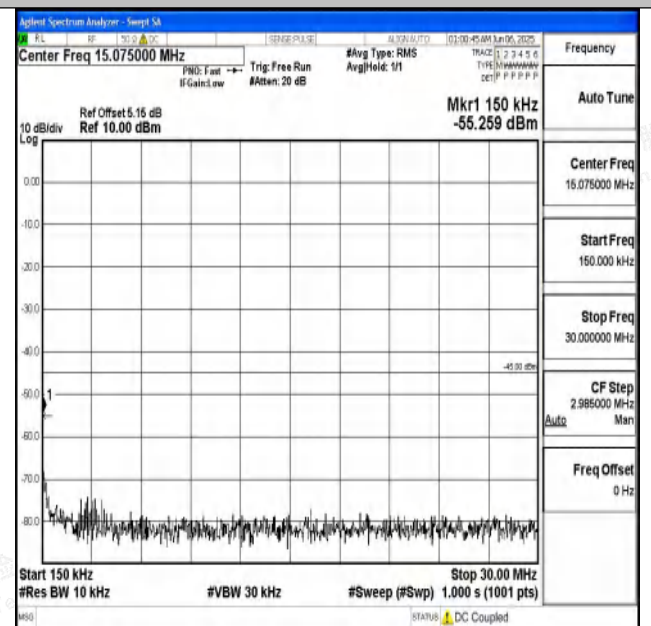
Band7_15MHz_16QAM_21375_1RB#0_20000~27000_20000 ~27000
