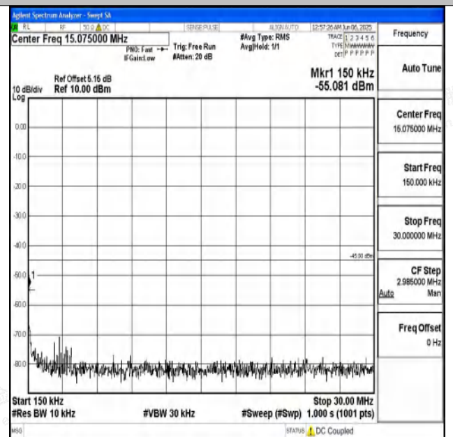
Band7_15MHz_QPSK_21100_1RB#0_0.15~30_0.15~30
