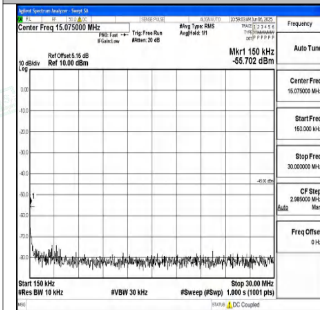
Band7_5MHz_16QAM_21425_1RB#0_0.15~30_0.15~30
