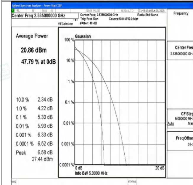
Band7-5MHz-QPSK-21100-25RB#0-PASS
