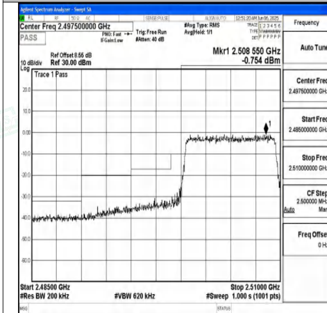
Band7_10MHz_QPSK_20800_50RB#0
