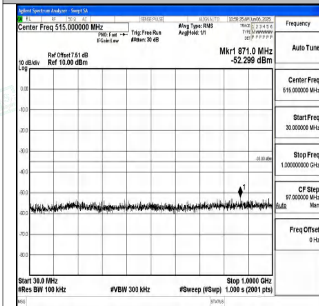
Band7_5MHz_QPSK_21425_1RB#0_30~1000_30~1000
