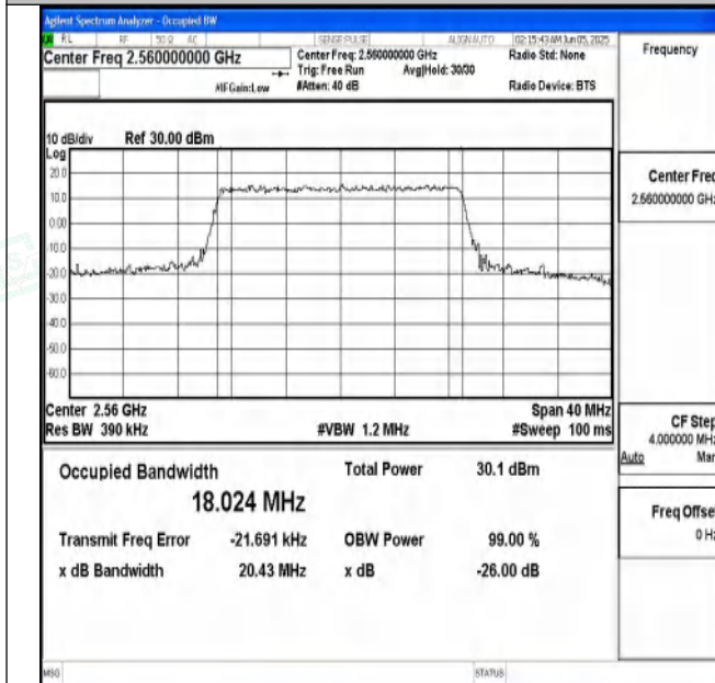
Band7-20MHz-QPSK-21350-100RB#0-PASS
