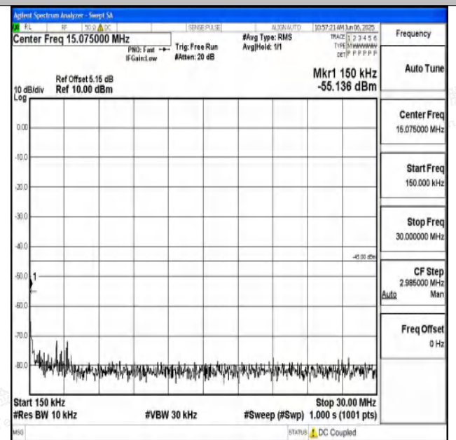
Band7_5MHz_QPSK_21100_1RB#0_0.15~30_0.15~30
