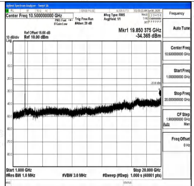
Band7_20MHz_QPSK_21350_1RB#0_1000~20000_1000~20000
