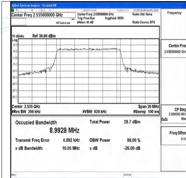
Band7-10MHz-QPSK-21100-50RB#0-PASS
