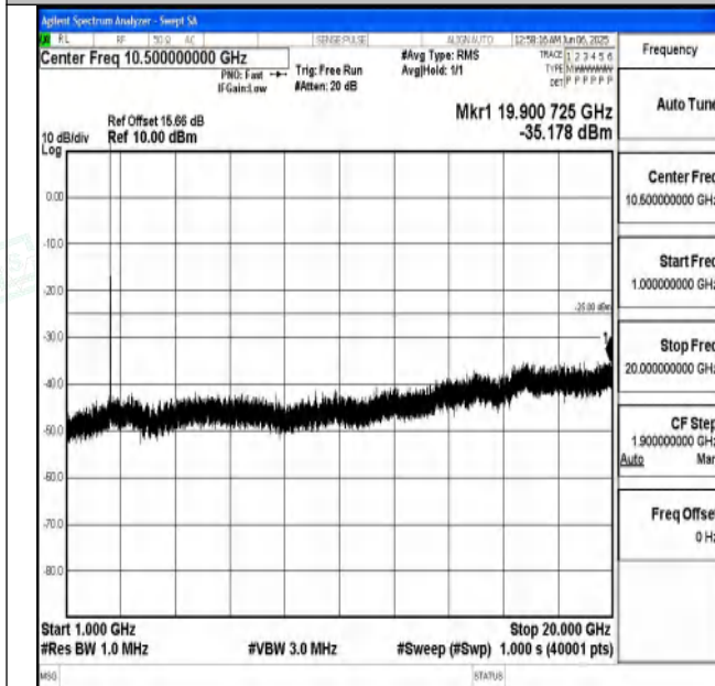
Band7_15MHz_16QAM_21100_1RB#0_1000~20000_1000~ 20000
