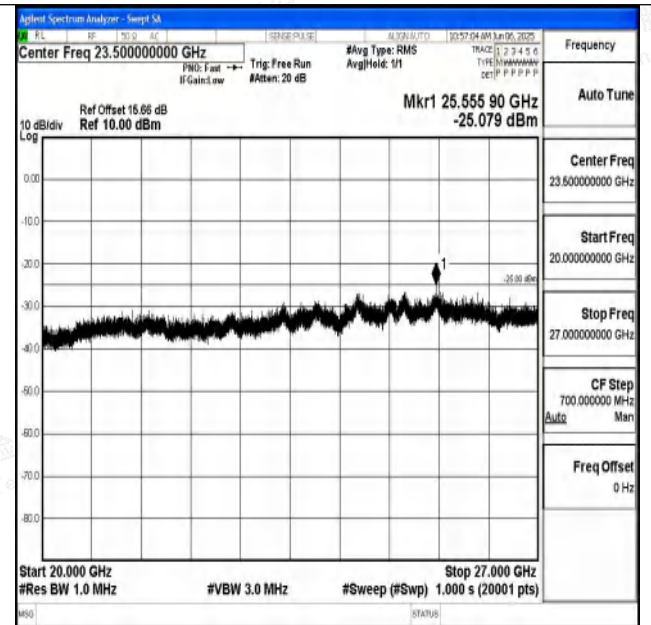
Band7_5MHz_16QAM_20775_1RB#0_20000~27000_20000~27000
