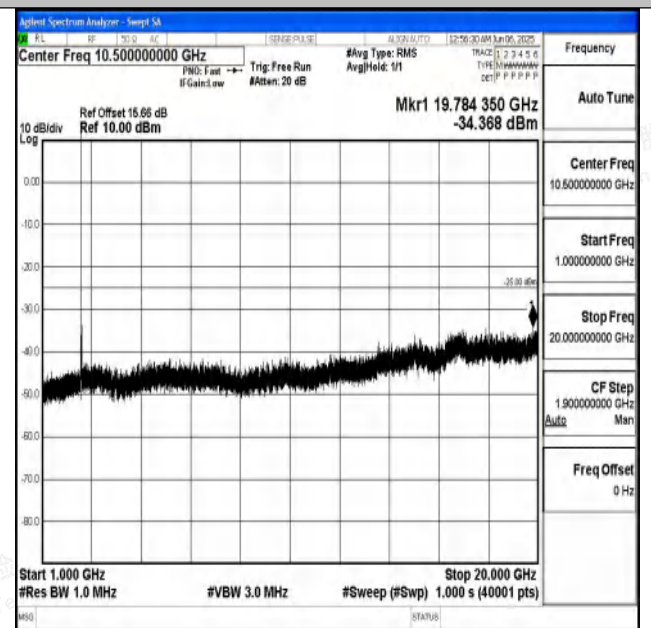
Band7_15MHz_QPSK_20825_1RB#0_1000~20000_1000~20000
