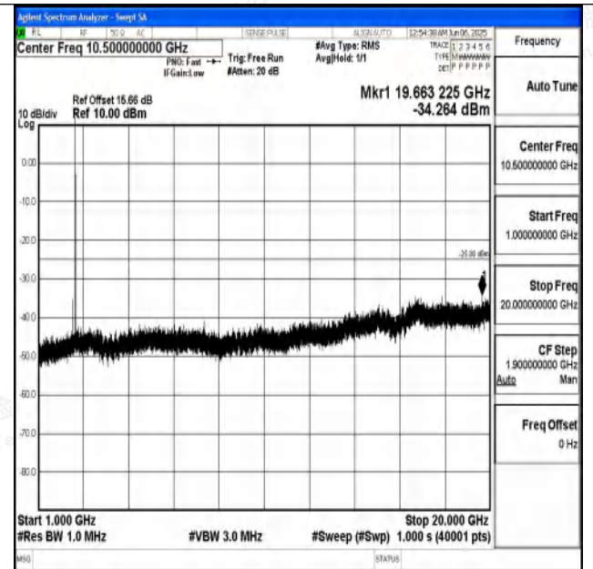
Band7_10MHz_QPSK_21400_1RB#0_1000~20000_1000~20000
