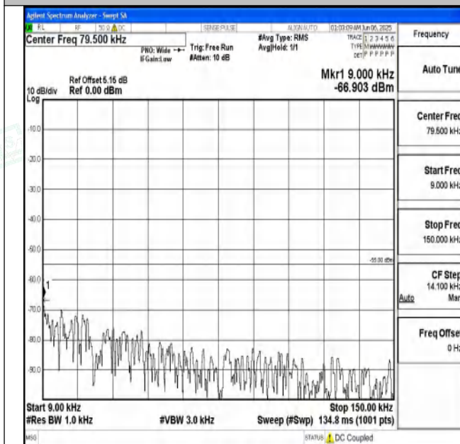
Band7_20MHz_QPSK_21350_1RB#0_0.009~0.15_0.009~0. 15
