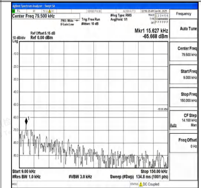
Band7_5MHz_16QAM_20775_1RB#0_0.009~0.15_0.009~0.15
