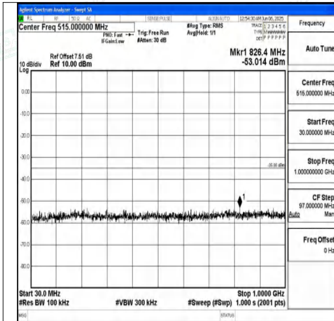
Band7_10MHz_QPSK_21400_1RB#0_30~1000_30~1000
