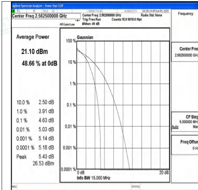
Band7-15MHz-QPSK-21375-1RB#0-PASS
