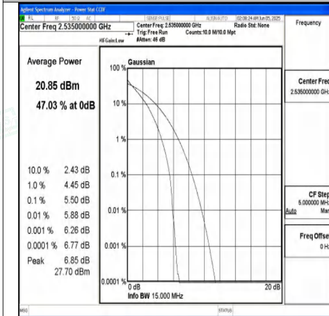
Band7-15MHz-QPSK-21100-75RB#0-PASS
