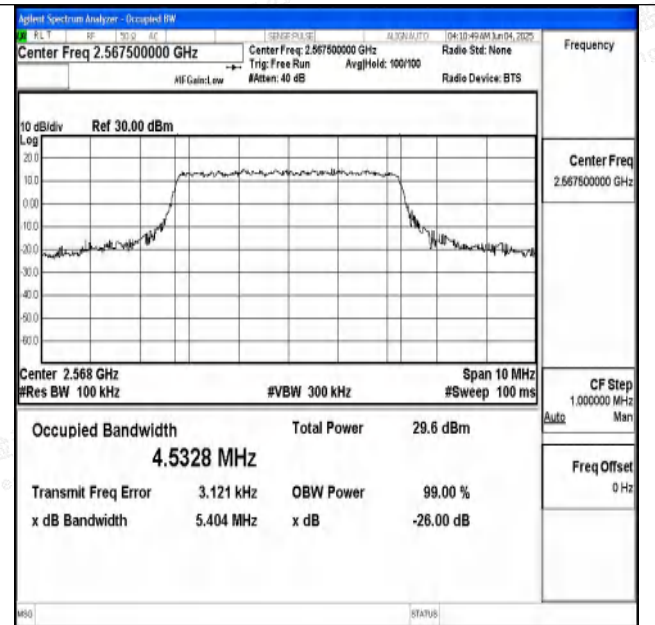
Band7-5MHz-16QAM-21425-25RB#0-PASS
