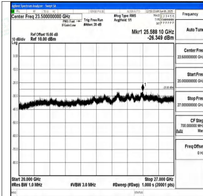
Band7_10MHz_QPSK_21100_1RB#0_20000~27000_20000~27000
