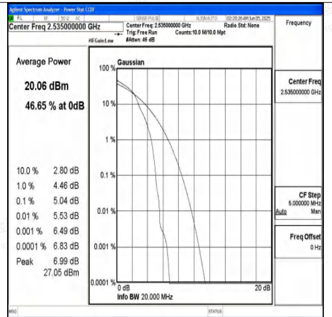
Band7-20MHz-16QAM-21100-1RB#0-PASS
