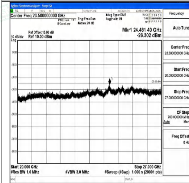
Band7_5MHz_QPSK_20775_1RB#0_20000~27000_20000~27000
