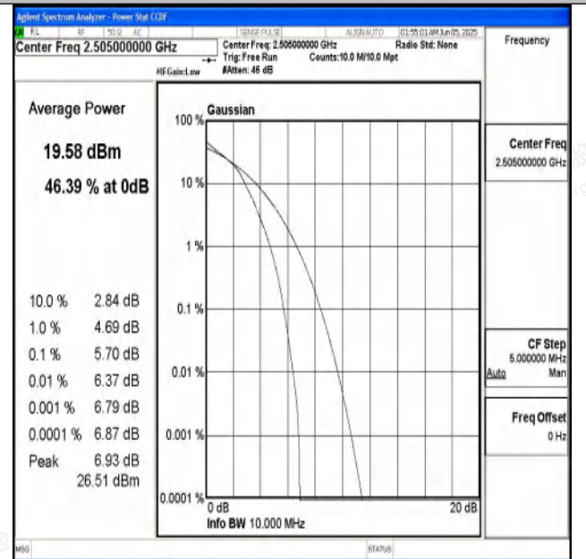
Band7-10MHz-16QAM-20800-50RB#0-PASS
