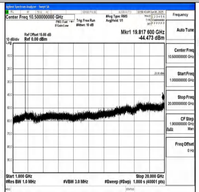
Band7_5MHz_QPSK_21425_1RB#0_1000~20000_1000~20000
