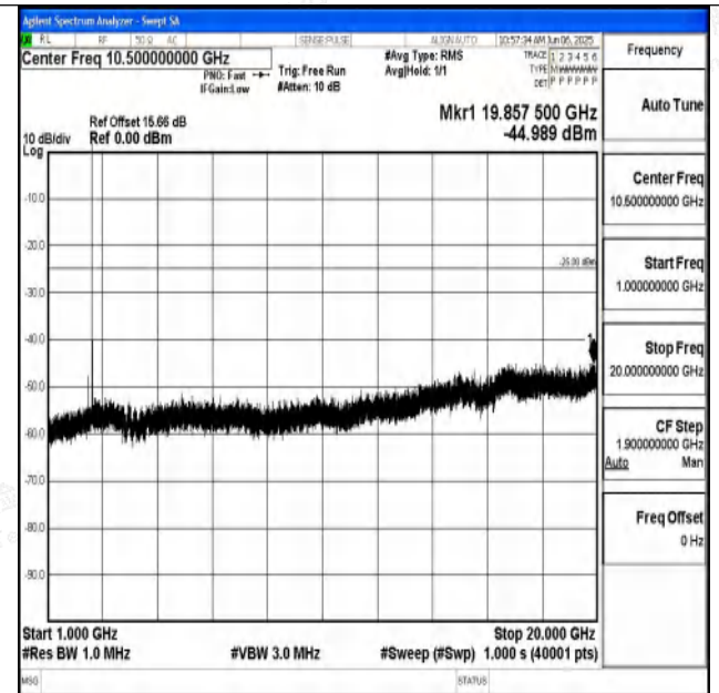
Band7_5MHz_QPSK_21100_1RB#0_1000~20000_1000~200 00
