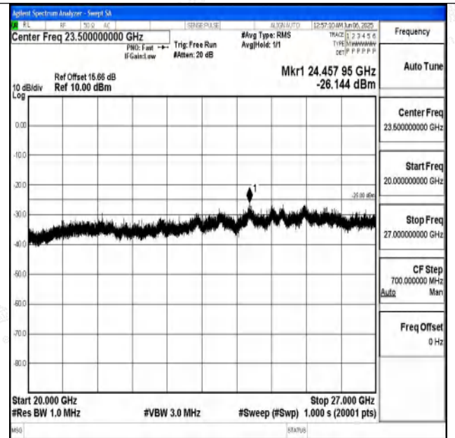
Band7_15MHz_16QAM_20825_1RB#0_20000~27000_20000~27000
