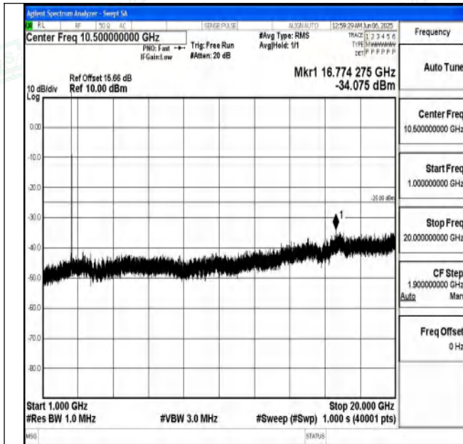
Band7_15MHz_16QAM_21375_1RB#0_1000~20000_1000~ 20000
