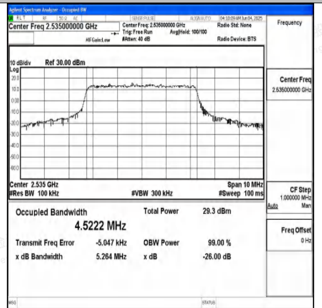
Band7-5MHz-16QAM-21100-25RB#0-PASS
