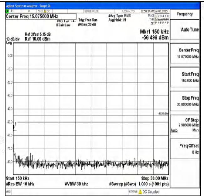
Band7_15MHz_QPSK_21375_1RB#0_0.15~30_0.15~30
