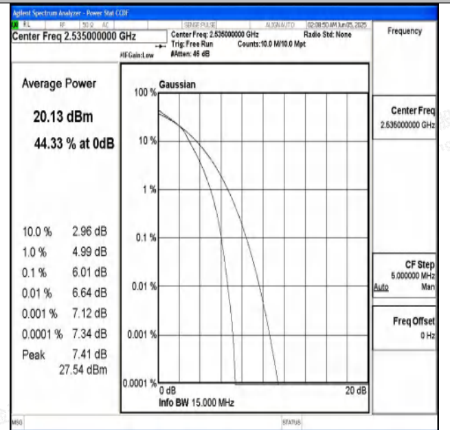
Band7-15MHz-16QAM-21100-75RB#0-PASS
