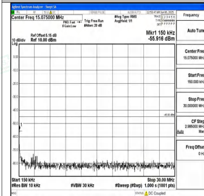
Band7_10MHz_16QAM_21100_1RB#0_0.15~30_0.15~30
