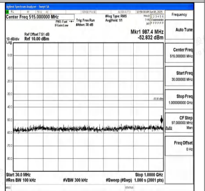
Band7_5MHz_16QAM_21425_1RB#0_30~1000_30~1000
