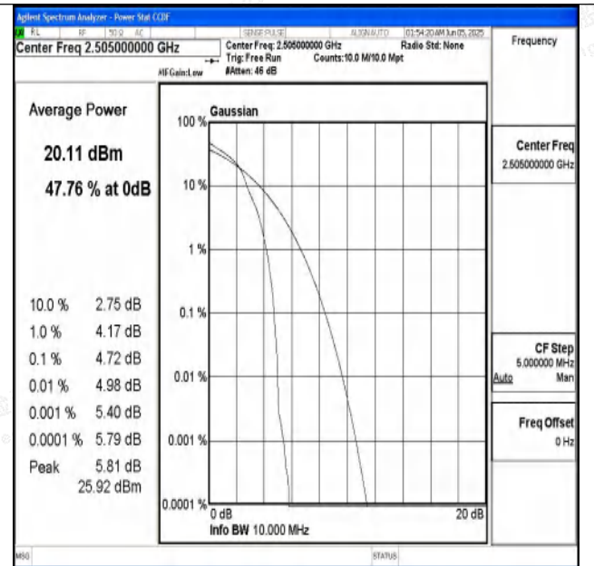
Band7-10MHz-16QAM-20800-1RB#0-PASS
