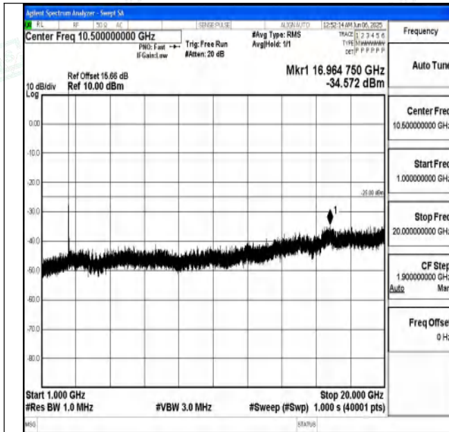
Band7_10MHz_QPSK_20800_1RB#0_1000~20000_1000~20000
