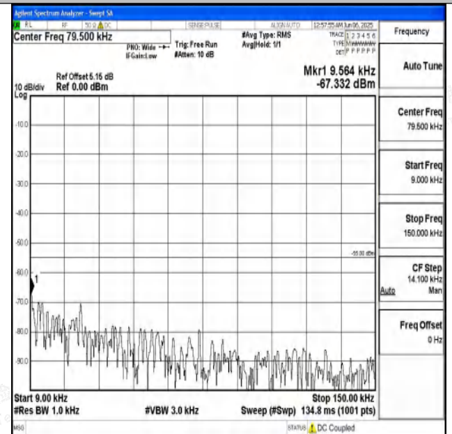
Band7_15MHz_16QAM_21100_1RB#0_0.009~0.15_0.009~0.15
