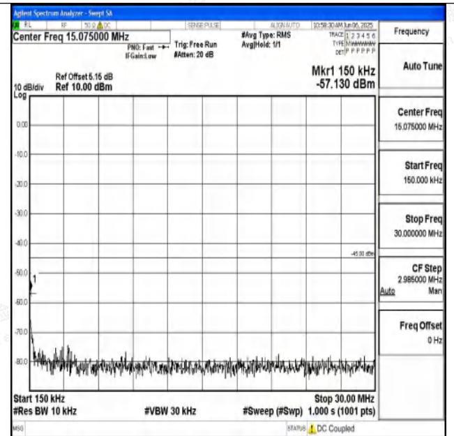
Band7_5MHz_QPSK_21425_1RB#0_0.15~30_0.15~30
