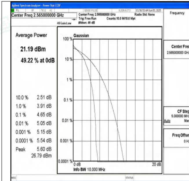
Band7-10MHz-QPSK-21400-1RB#0-PASS
