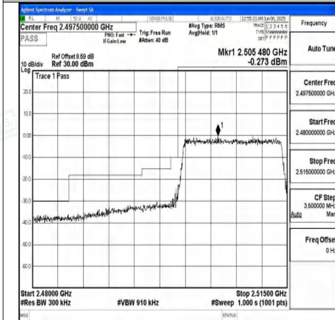
Band7_15MHz_QPSK_20825_75RB#0
