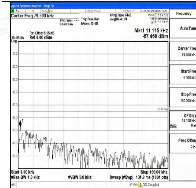
Band7_20MHz_QPSK_21100_1RB#0_0.009~0.15_0.009~0.
