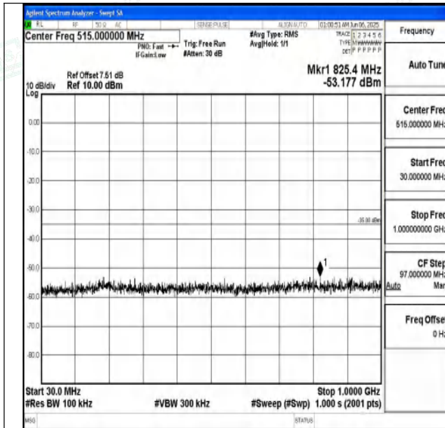
Band7_20MHz_QPSK_20850_1RB#0_30~1000_30~1000
