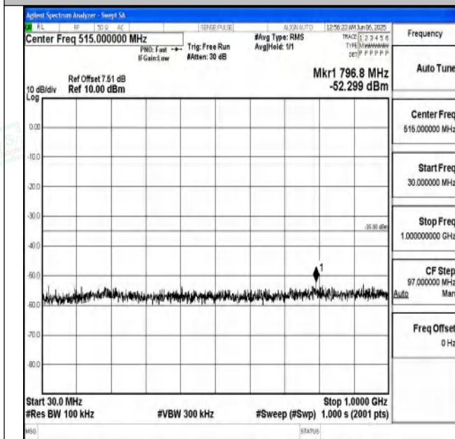
Band7_15MHz_QPSK_20825_1RB#0_30~1000_30~1000
