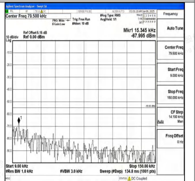
Band7_20MHz_16QAM_20850_1RB#0_0.009~0.15_0.009~0.15
