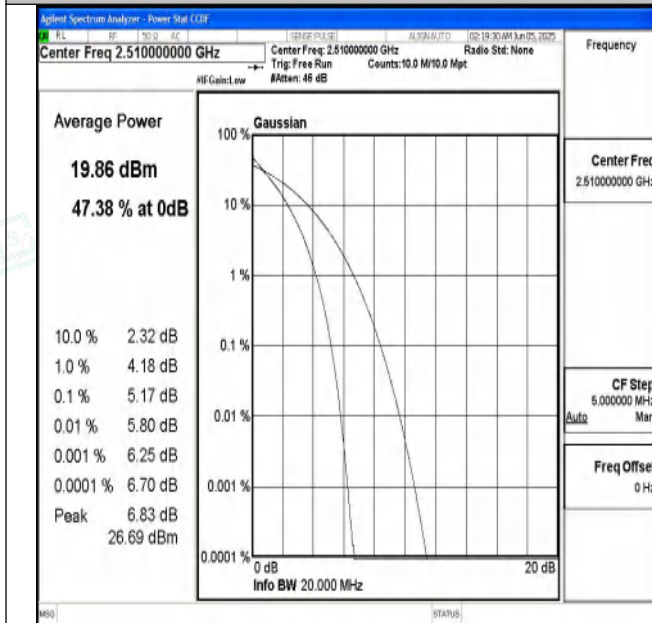
Band7-20MHz-QPSK-20850-100RB#0-PASS
