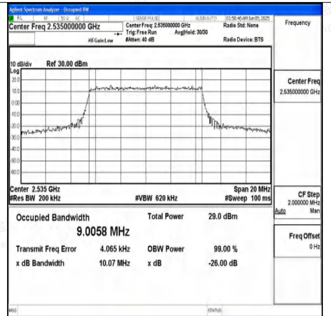
Band7-10MHz-16QAM-21100-50RB#0-PASS
