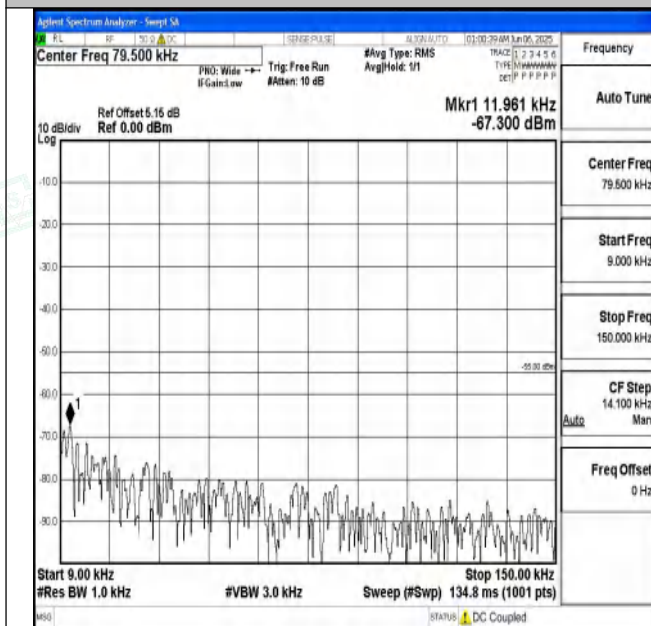
Band7_20MHz_QPSK_20850_1RB#0_0.009~0.15_0.009~0. 15
