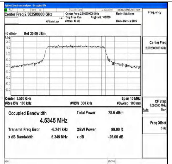
Band7-5MHz-16QAM-20775-25RB#0-PASS
