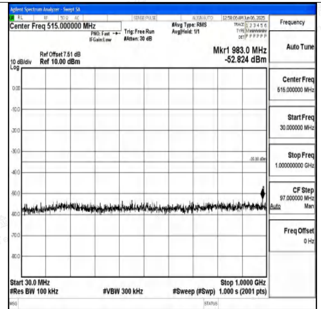
Band7_15MHz_16QAM_21100_1RB#0_30~1000_30~1000
