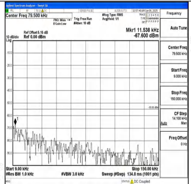
Band7_5MHz_16QAM_21100_1RB#0_0.009~0.15_0.009~0.1 5
