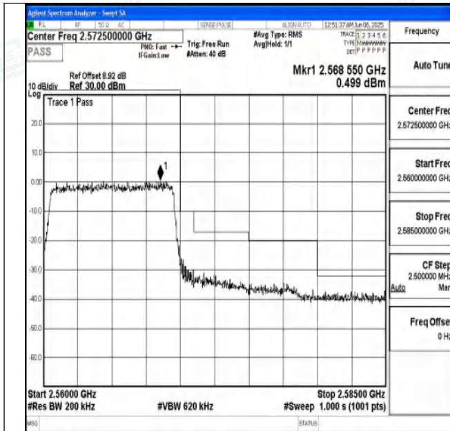
Band7_10MHz_QPSK_21400_50RB#0
