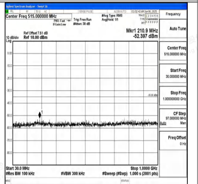
Band7_20MHz_16QAM_21100_1RB#0_30~1000_30~1000
