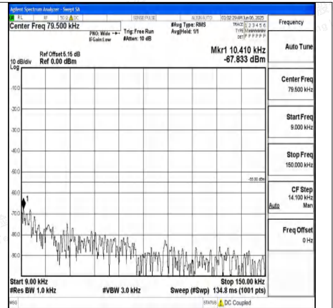
Band7_20MHz_16QAM_21100_1RB#0_0.009~0.15_0.009~0.15 15
