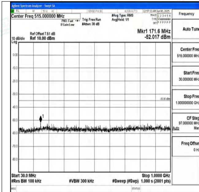
Band7_15MHz_QPSK_21100_1RB#0_30~1000_30~1000
