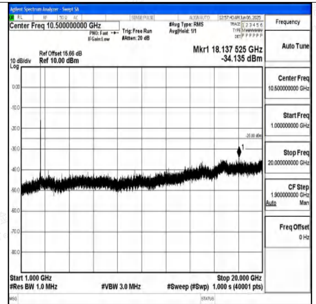
Band7_15MHz_QPSK_21100_1RB#0_1000~20000_1000~20000
