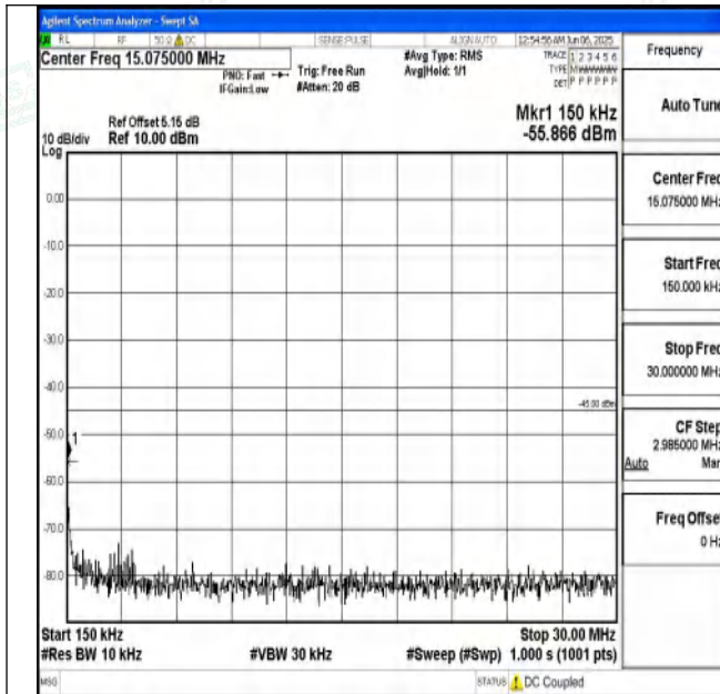
Band7_10MHz_16QAM_21400_1RB#0_0.15~30_0.15~30
