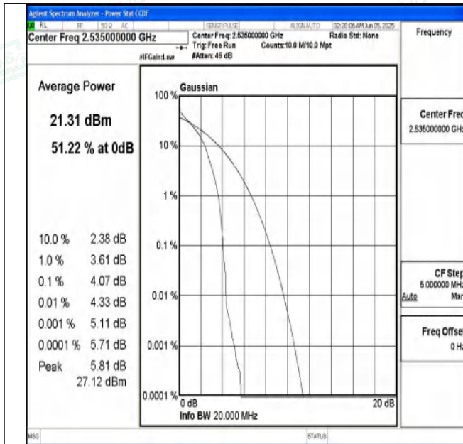
Band7-20MHz-QPSK-21100-1RB#0-PASS
