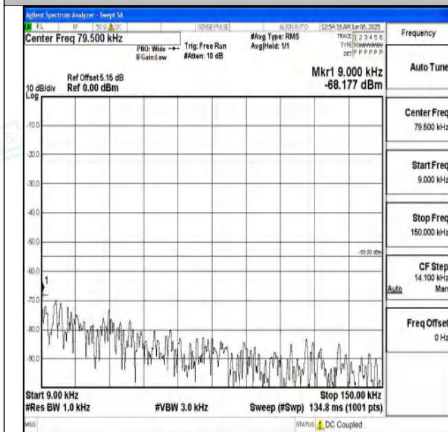
Band7_10MHz_QPSK_21400_1RB#0_0.009~0.15_0.009~0.15
