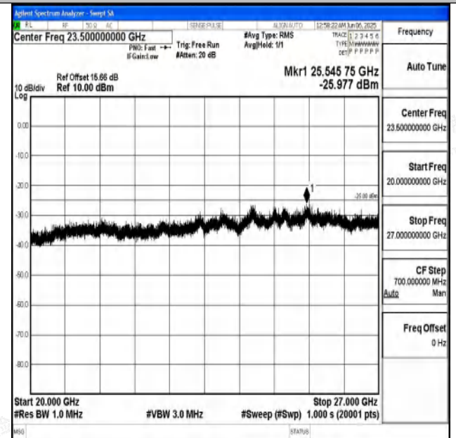
Band7_15MHz_16QAM_21100_1RB#0_20000~27000_20000 ~27000
