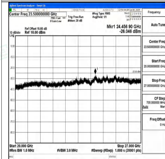
Band7_10MHz_QPSK_21400_1RB#0_20000~27000_20000~27000
