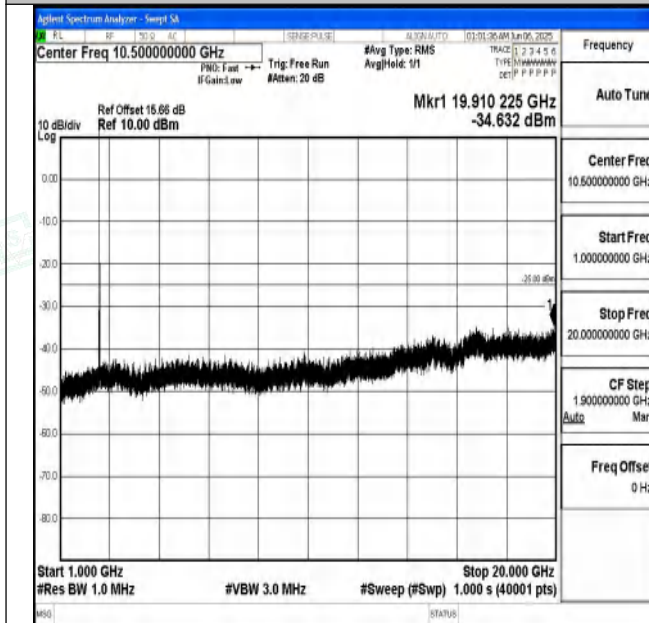
Band7_20MHz_16QAM_20850_1RB#0_1000~20000_1000~ 20000
