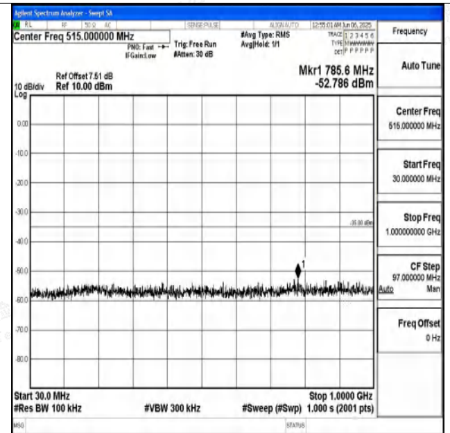
Band7_10MHz_16QAM_21400_1RB#0_30~1000_30~1000
