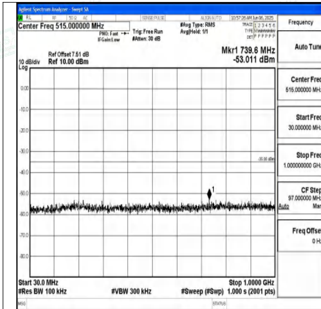
Band7_5MHz_QPSK_21100_1RB#0_30~1000_30~1000
