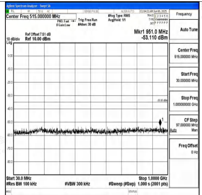
Band7_20MHz_16QAM_21350_1RB#0_30~1000_30~1000
