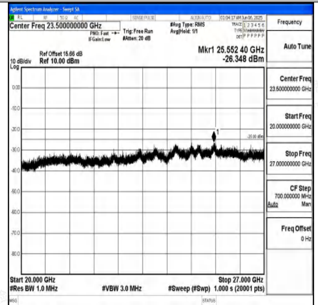
Band7_20MHz_16QAM_21350_1RB#0_20000~27000_20000 ~27000
