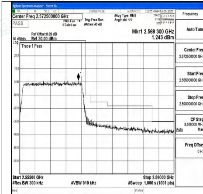
Band7_15MHz_QPSK_21375_75RB#0
