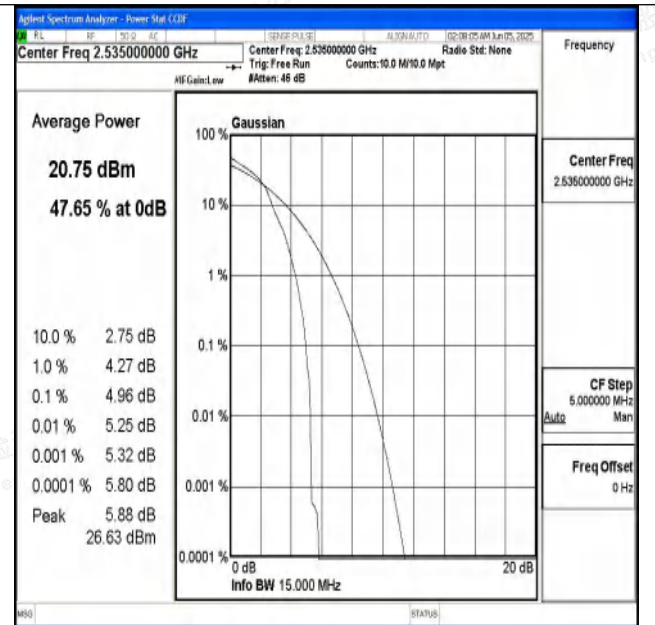
Band7-15MHz-16QAM-21100-1RB#0-PASS
