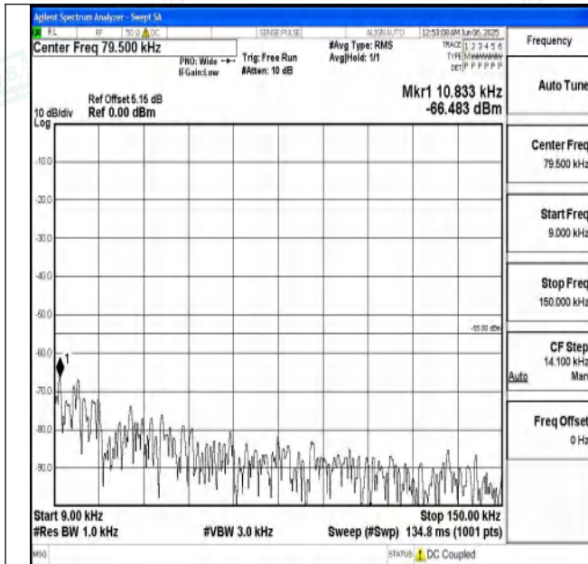
Band7_10MHz_QPSK_21100_1RB#0_0.009~0.15_0.009~0.15
