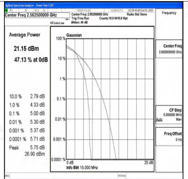
Band7-15MHz-16QAM-21375-1RB#0-PASS
