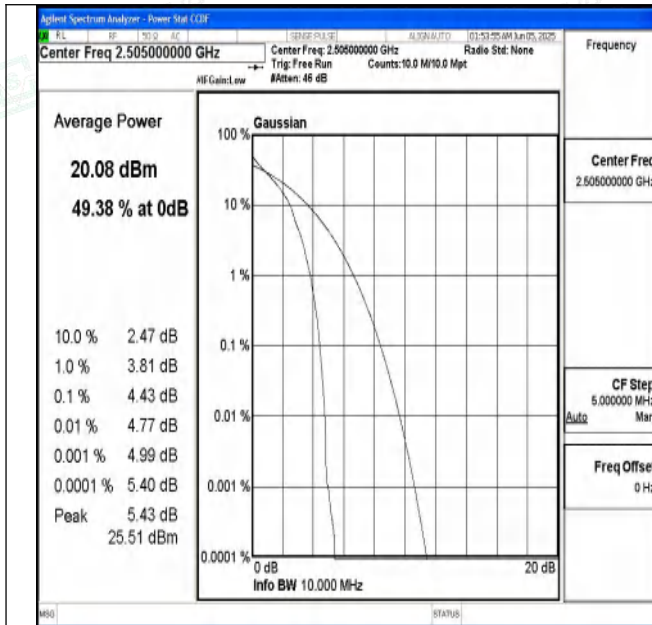
Band7-10MHz-QPSK-20800-1RB#0-PASS
