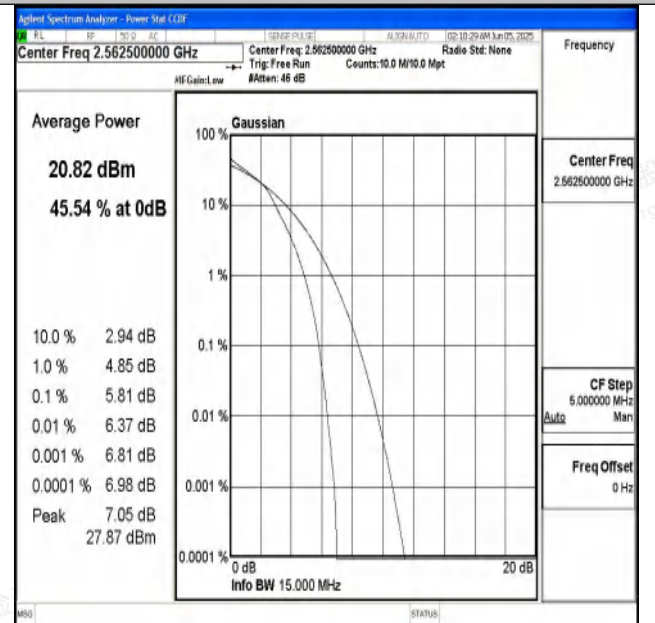
Band7-15MHz-16QAM-21375-75RB#0-PASS
