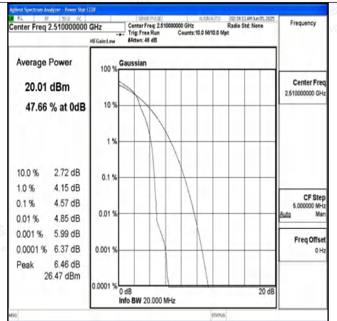
Band7-20MHz-16QAM-20850-1RB#0-PASS
