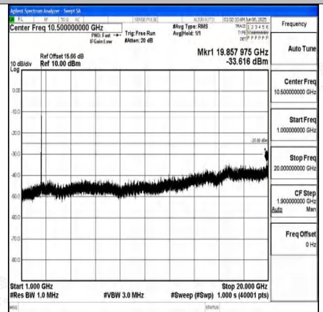
Band7_20MHz_QPSK_21100_1RB#0_1000~20000_1000~20000
