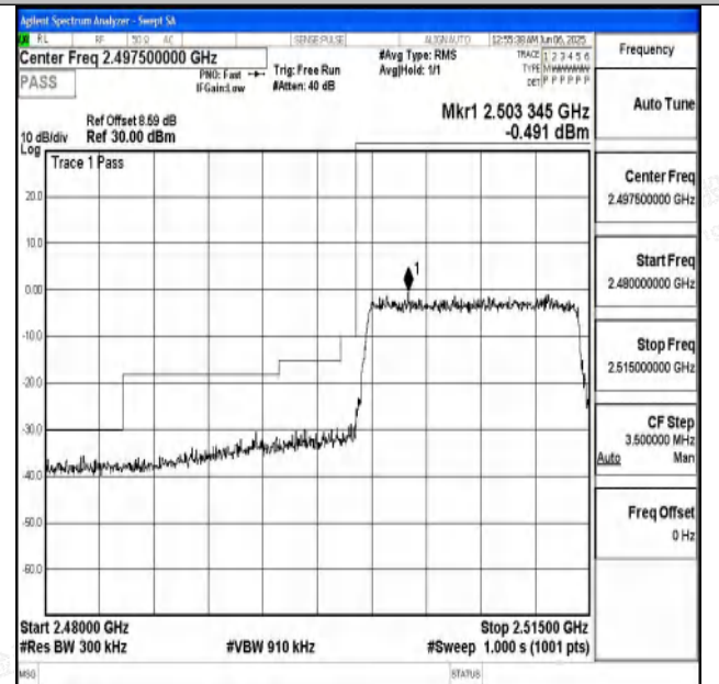
Band7_15MHz_16QAM_20825_75RB#0
