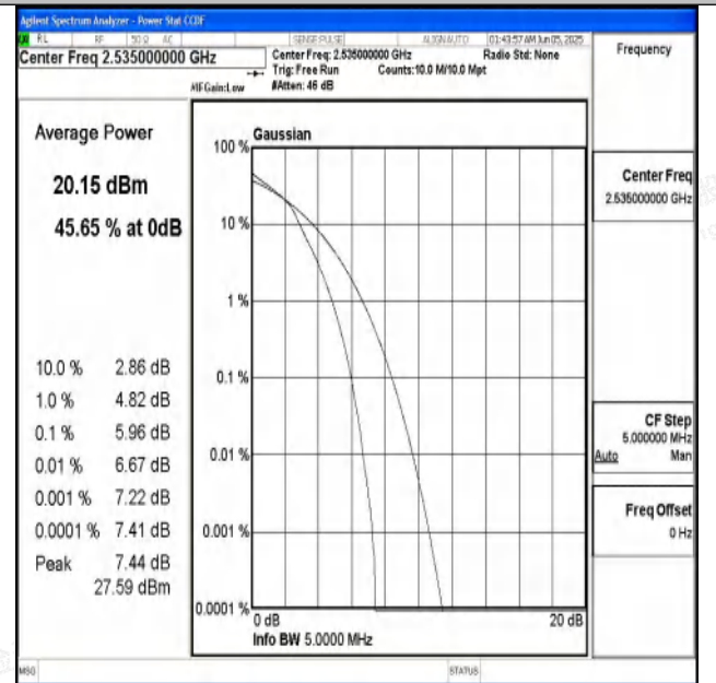
Band7-5MHz-16QAM-21100-25RB#0-PASS
