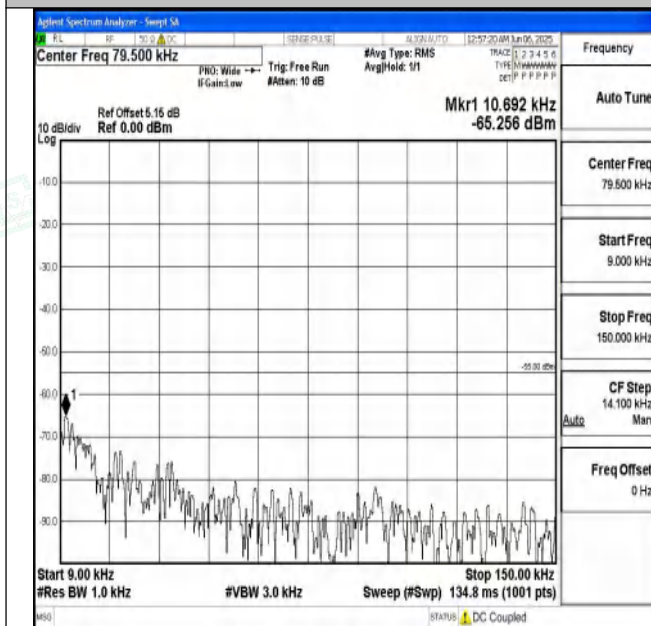
Band7_15MHz_QPSK_21100_1RB#0_0.009~0.15_0.009~0.15
