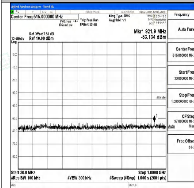
Band7_20MHz_QPSK_21100_1RB#0_30~1000_30~1000
