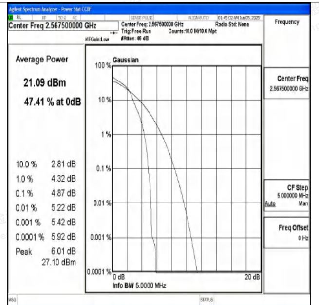
Band7-5MHz-16QAM-21425-1RB#0-PASS
