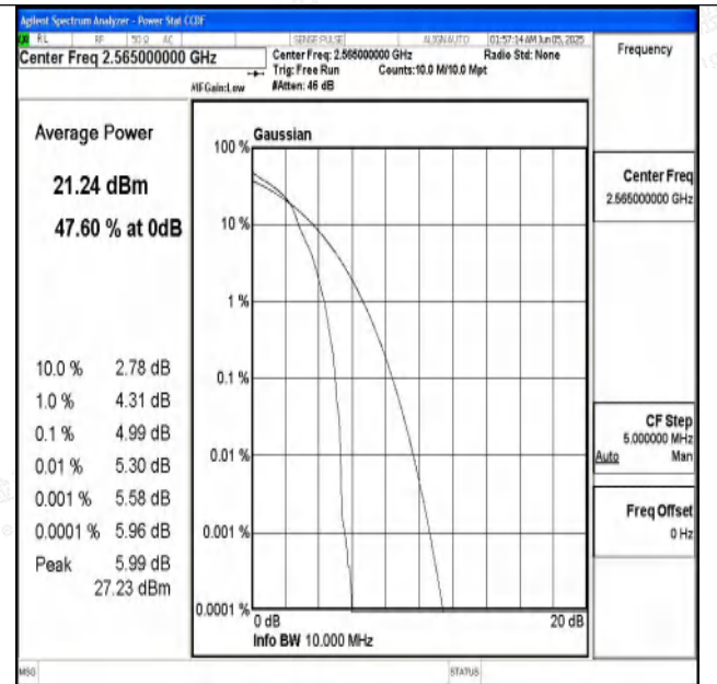
Band7-10MHz-16QAM-21400-1RB#0-PASS
