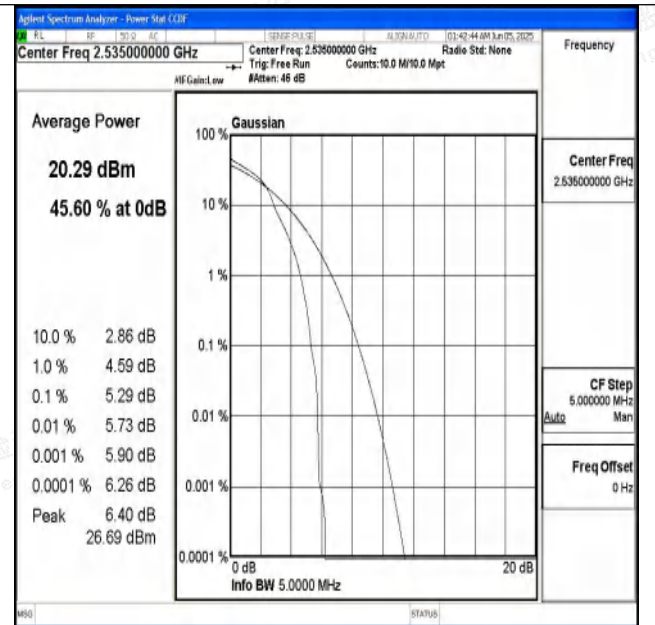
Band7-5MHz-16QAM-21100-1RB#0-PASS
