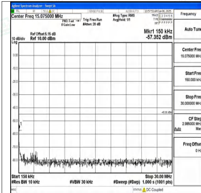
Band7_5MHz_16QAM_21100_1RB#0_0.15~30_0.15~30
