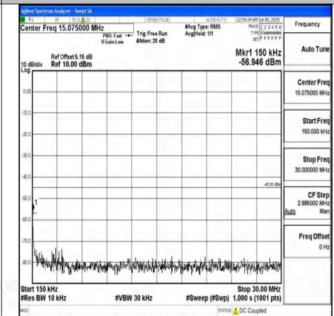
Band7_10MHz_QPSK_21400_1RB#0_0.15~30_0.15~30
