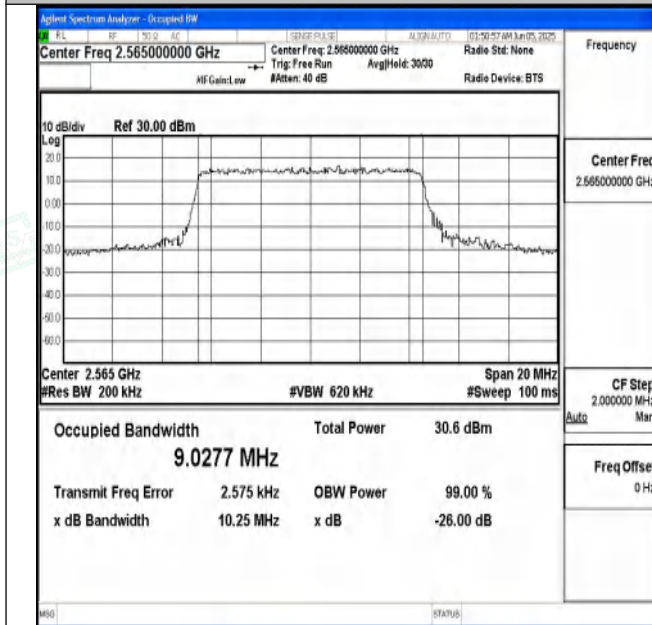
Band7-10MHz-QPSK-21400-50RB#0-PASS
