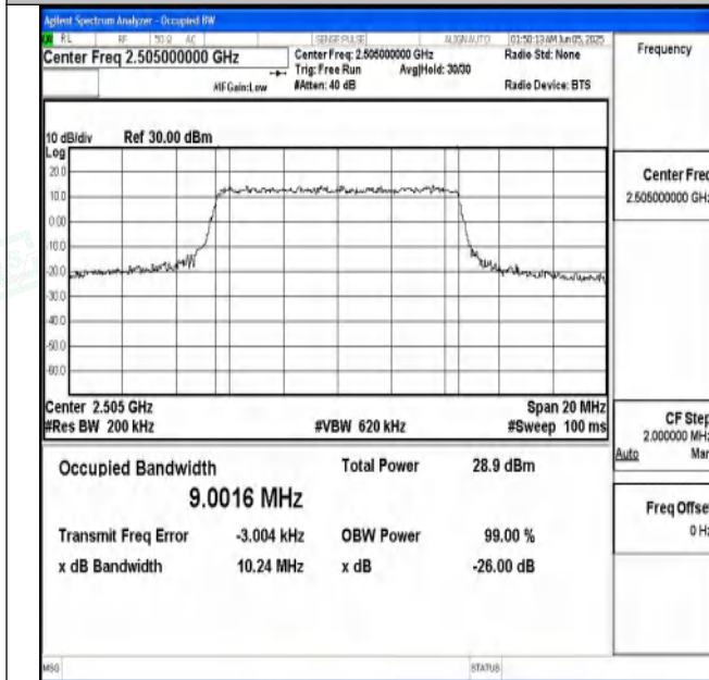
Band7-10MHz-QPSK-20800-50RB#0-PASS
