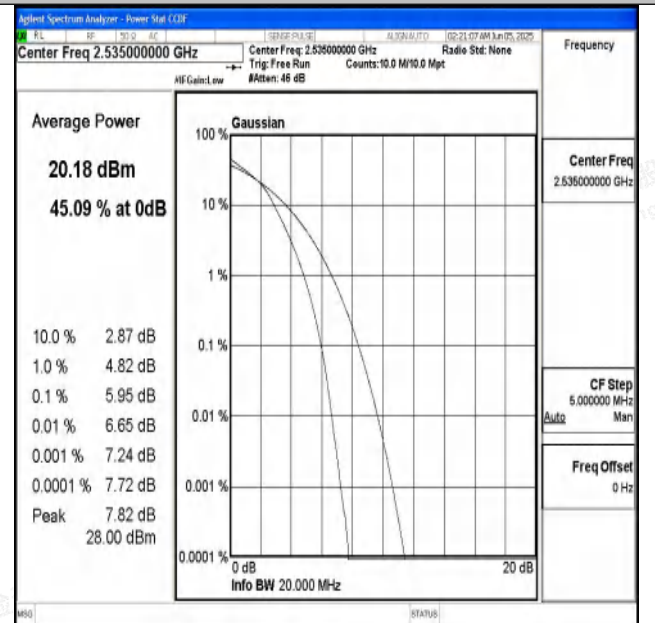
Band7-20MHz-16QAM-21100-100RB#0-PASS
