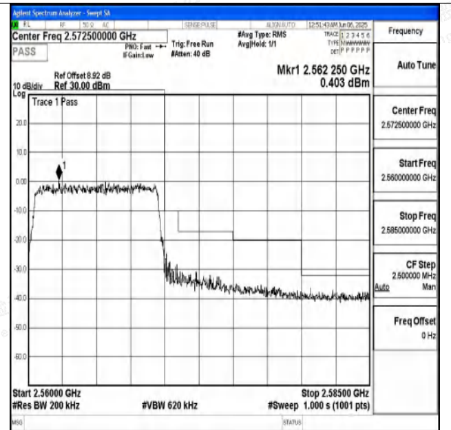
Band7_10MHz_16QAM_21400_50RB#0
