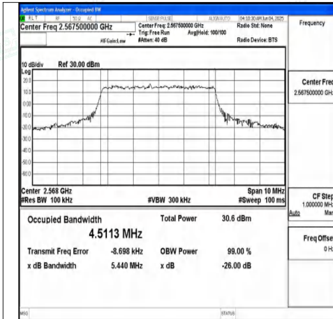
Band7-5MHz-QPSK-21425-25RB#0-PASS
