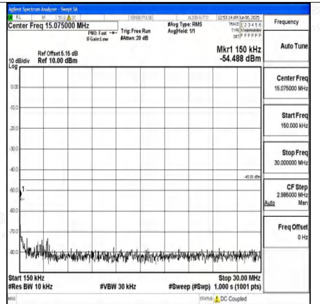
Band7_10MHz_QPSK_21100_1RB#0_0.15~30_0.15~30
