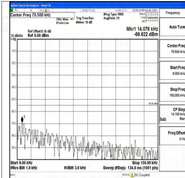
Band7_5MHz_QPSK_21425_1RB#0_0.009~0.15_0.009~0.1
