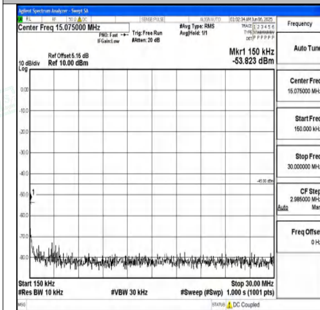
Band7_20MHz_16QAM_21100_1RB#0_0.15~30_0.15~30
