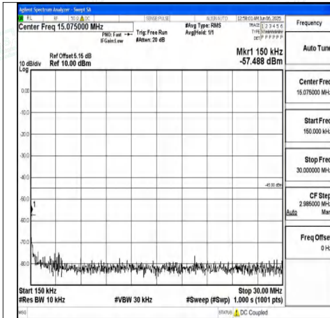
Band7_15MHz_16QAM_21100_1RB#0_0.15~30_0.15~30
