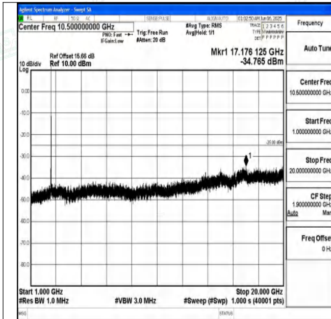
Band7_20MHz_16QAM_21100_1RB#0_1000~20000_1000~ 20000
