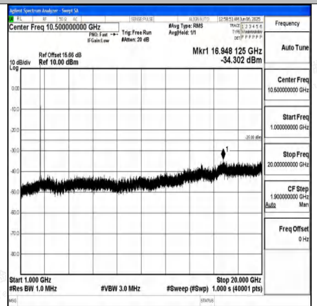
Band7_15MHz_QPSK_21375_1RB#0_1000~20000_1000~20000
