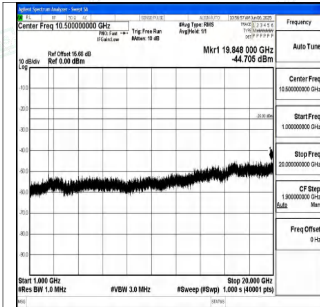
Band7_5MHz_16QAM_20775_1RB#0_1000~20000_1000~20000
