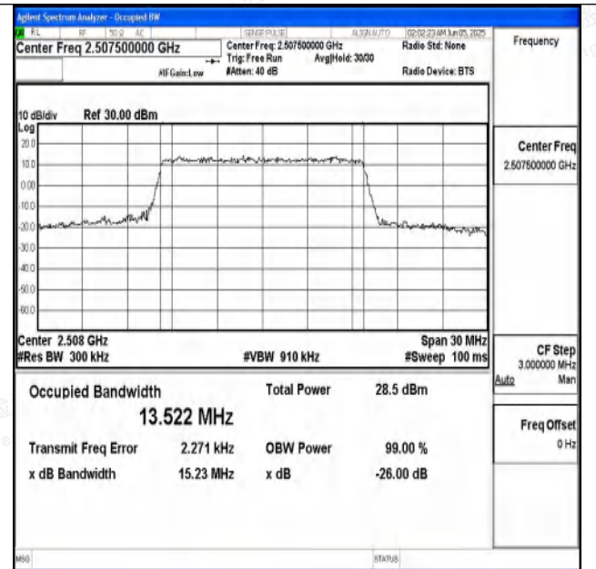
Band7-15MHz-16QAM-20825-75RB#0-PASS
