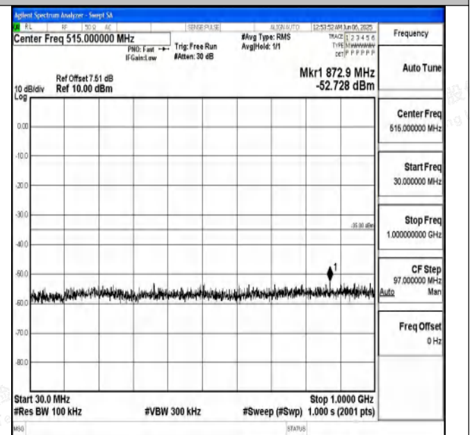
Band7_10MHz_16QAM_21100_1RB#0_30~1000_30~1000
