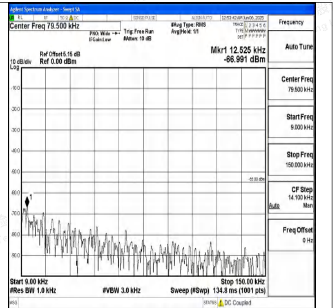
Band7_10MHz_16QAM_21100_1RB#0_0.009~0.15_0.009~0.15
