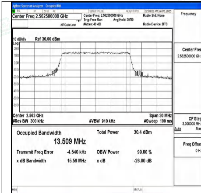
Band7-15MHz-QPSK-21375-75RB#0-PASS
