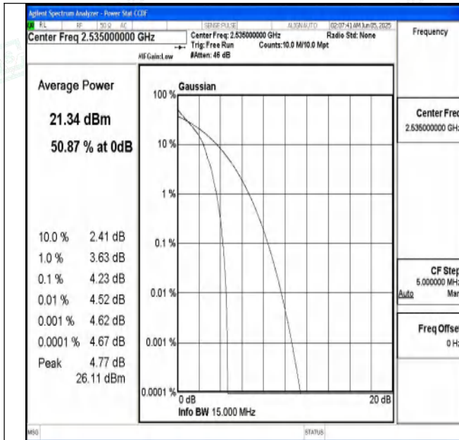
Band7-15MHz-QPSK-21100-1RB#0-PASS
