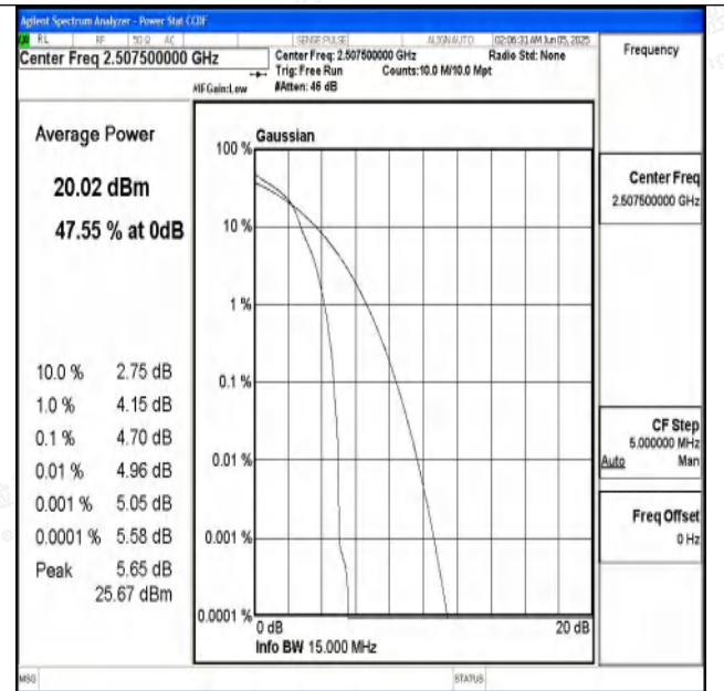
Band7-15MHz-16QAM-20825-1RB#0-PASS
