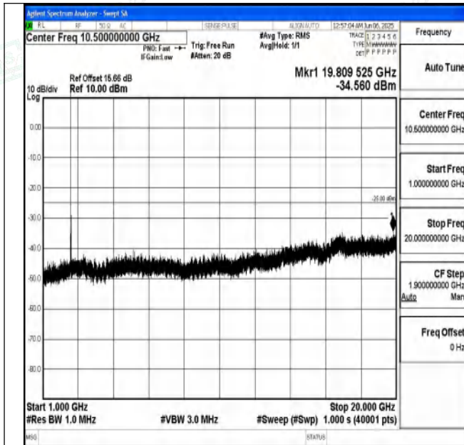
Band7_15MHz_16QAM_20825_1RB#0_1000~20000_1000~20000
