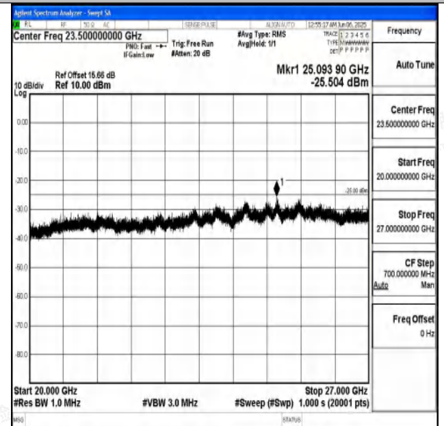
Band7_10MHz_16QAM_21400_1RB#0_20000~27000_20000 ~27000
