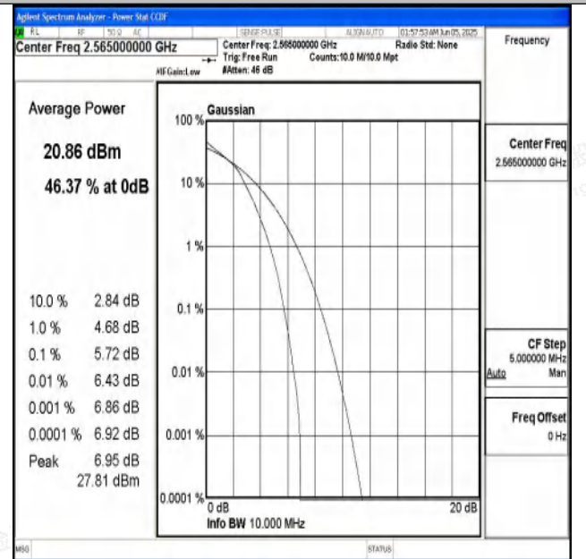
Band7-10MHz-16QAM-21400-50RB#0-PASS
