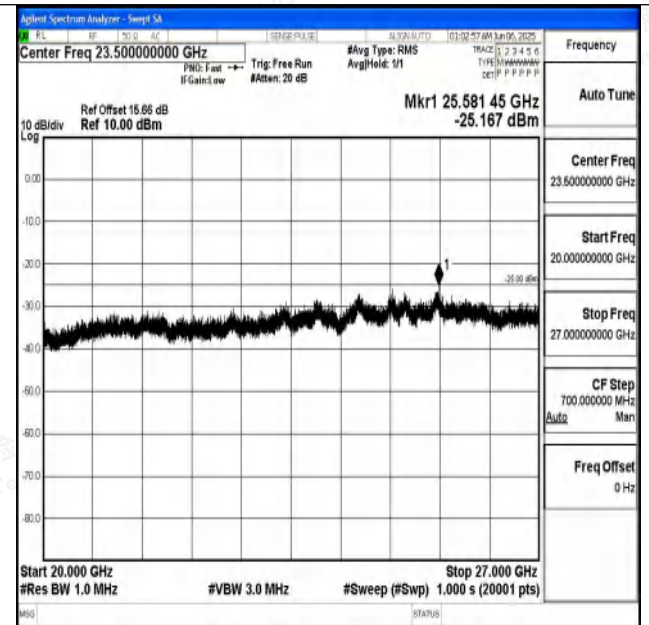
Band7_20MHz_16QAM_21100_1RB#0_20000~27000_20000 ~27000
