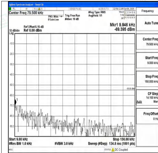
Band7_15MHz_QPSK_20825_1RB#0_0.009~0.15_0.009~0.
