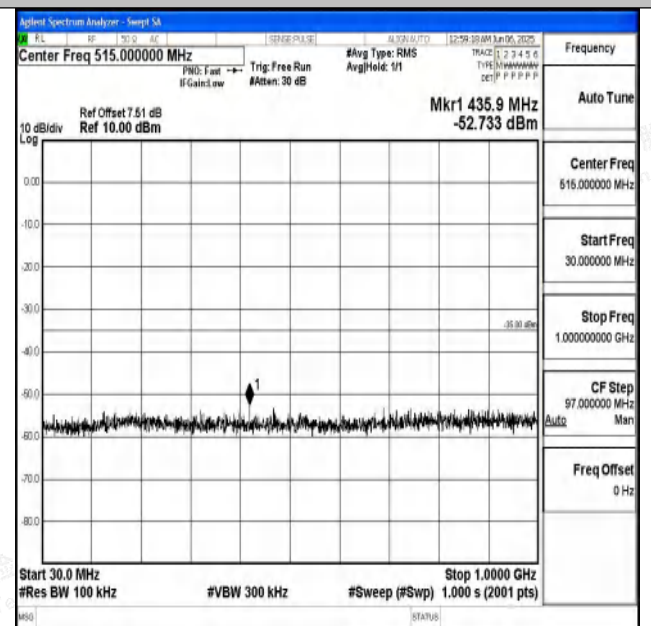
Band7_15MHz_16QAM_21375_1RB#0_30~1000_30~1000
