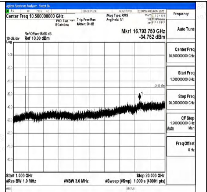
Band7_20MHz_QPSK_20850_1RB#0_1000~20000_1000~20000
