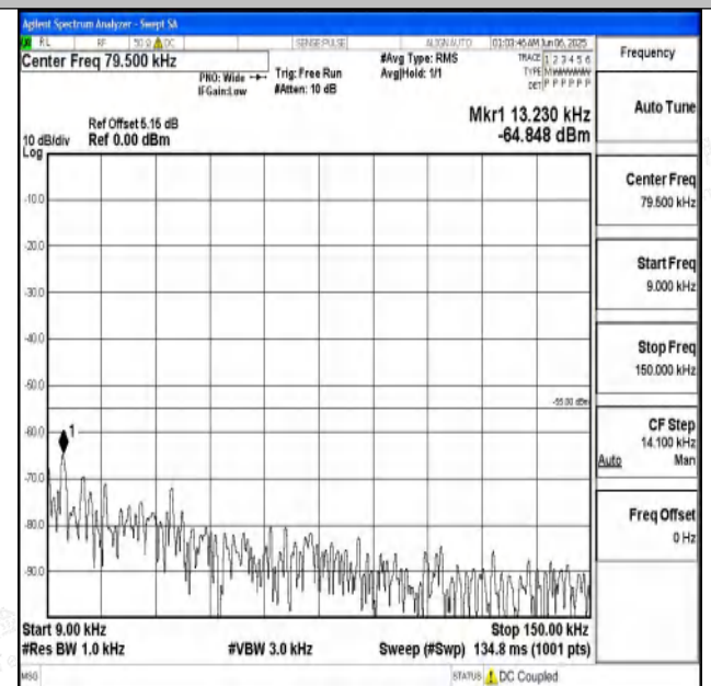
Band7_20MHz_16QAM_21350_1RB#0_0.009~0.15_0.009~0.15
