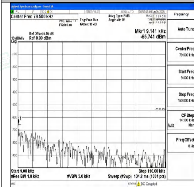
Band7_5MHz_QPSK_21100_1RB#0_0.009~0.15_0.009~0.1
