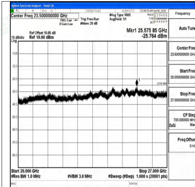
Band7_5MHz_QPSK_21425_1RB#0_20000~27000_20000~27000
