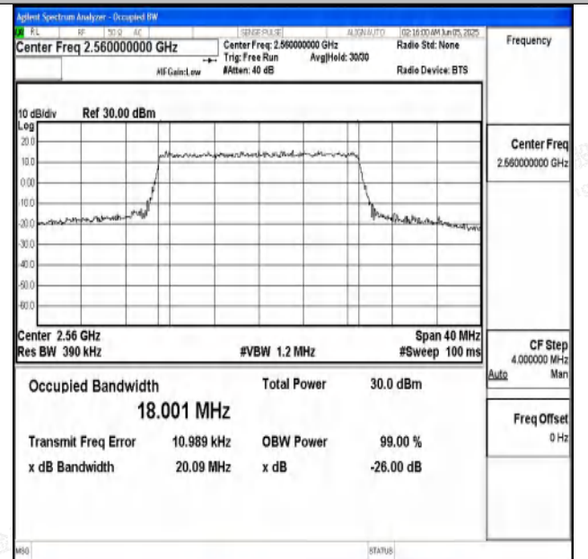
Band7-20MHz-16QAM-21350-100RB#0-PASS
