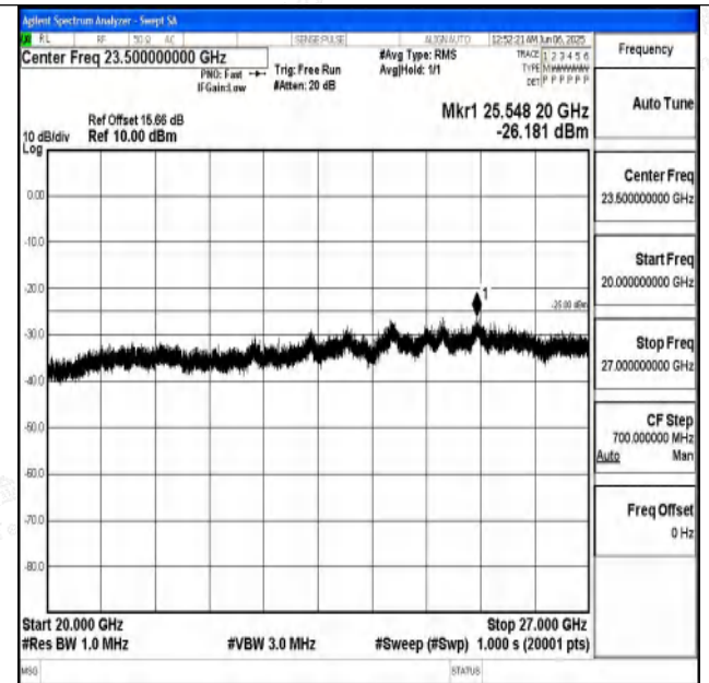
Band7_10MHz_QPSK_20800_1RB#0_20000~27000_20000~27000
