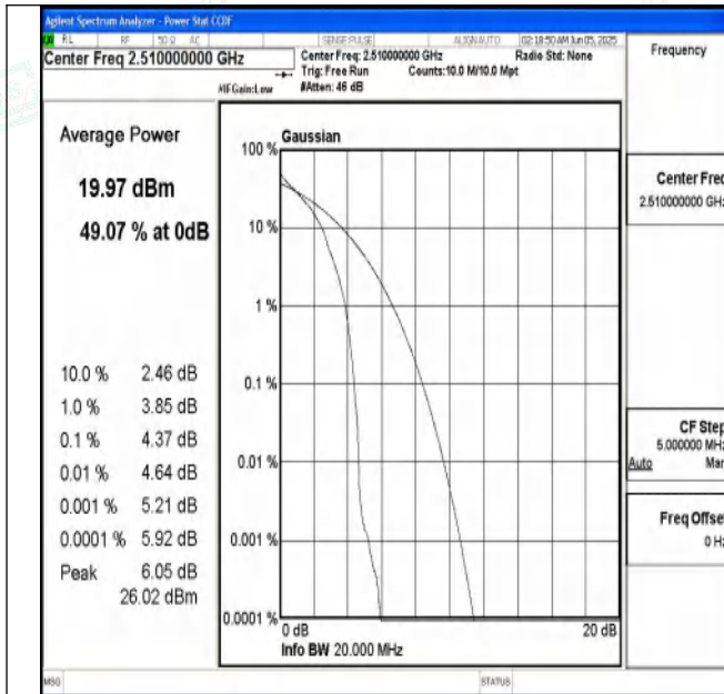
Band7-20MHz-QPSK-20850-1RB#0-PASS
