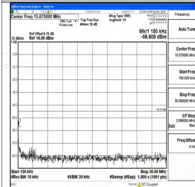
Band7_15MHz_16QAM_21375_1RB#0_0.15~30_0.15~30
