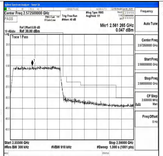
Band7_15MHz_16QAM_21375_75RB#0
