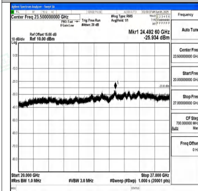
Band7_20MHz_QPSK_21350_1RB#0_20000~27000_20000~27000
