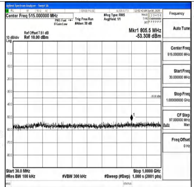
Band7_10MHz_16QAM_20800_1RB#0_30~1000_30~1000
