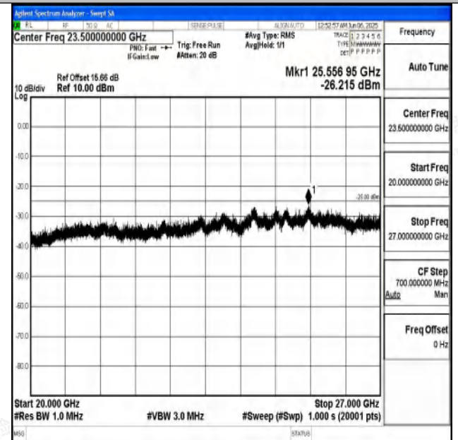
Band7_10MHz_16QAM_20800_1RB#0_20000~27000_20000 ~27000
