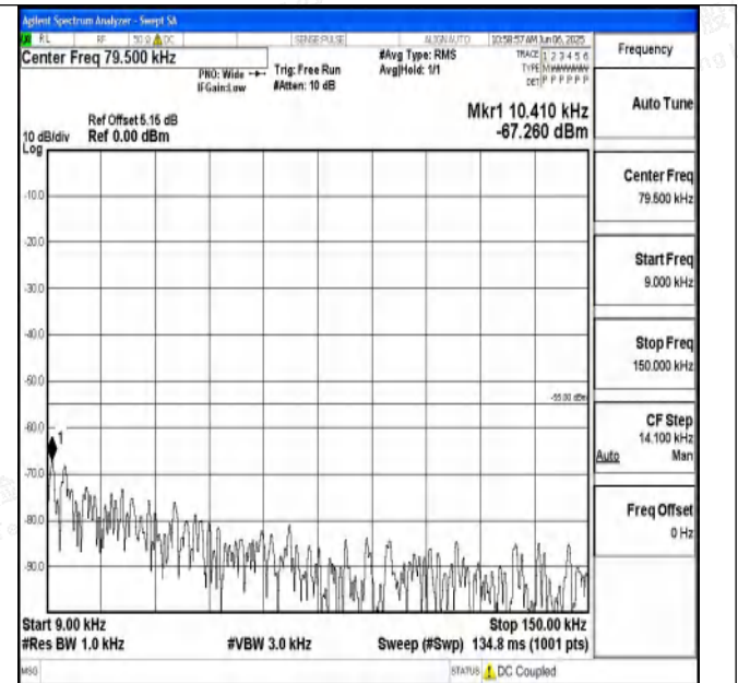
Band7_5MHz_16QAM_21425_1RB#0_0.009~0.15_0.009~0.1 5
