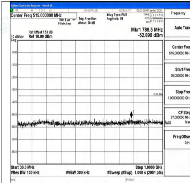
Band7_20MHz_QPSK_21350_1RB#0_30~1000_30~1000
