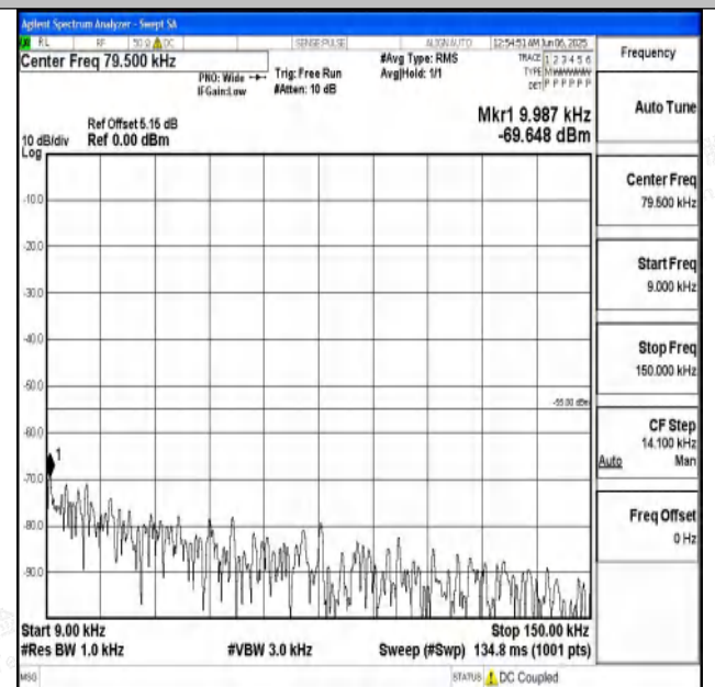
Band7_10MHz_16QAM_21400_1RB#0_0.009~0.15_0.009~0.15
