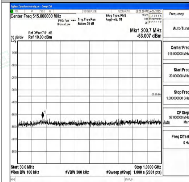
Band7_10MHz_QPSK_21100_1RB#0_30~1000_30~1000
