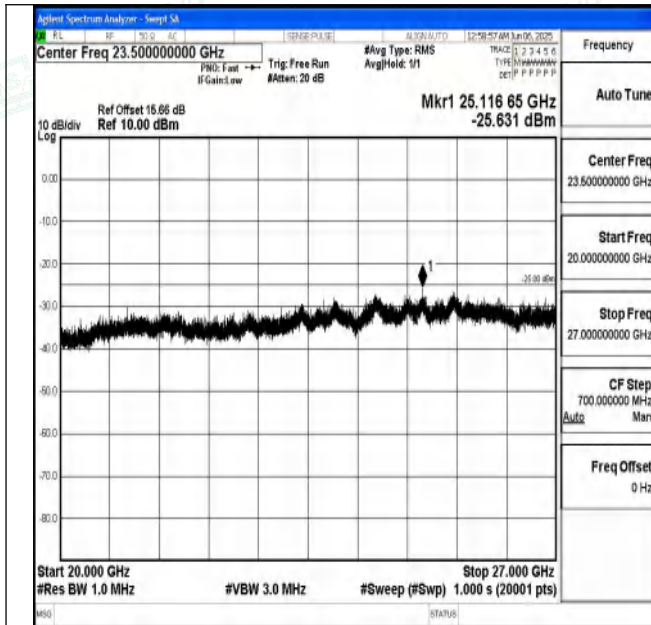
Band7_15MHz_QPSK_21375_1RB#0_20000~27000_20000 ~27000
