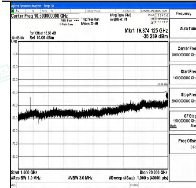
Band7_10MHz_16QAM_20800_1RB#0_1000~20000_1000~ 20000
