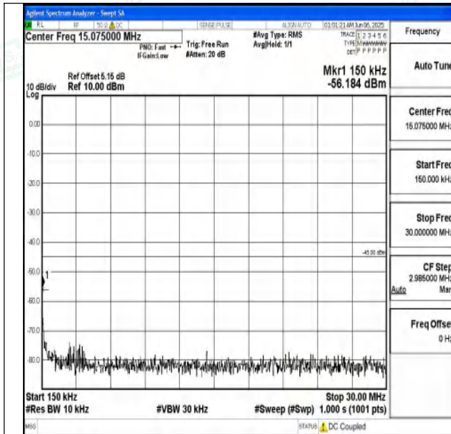
Band7_20MHz_16QAM_20850_1RB#0_0.15~30_0.15~30
