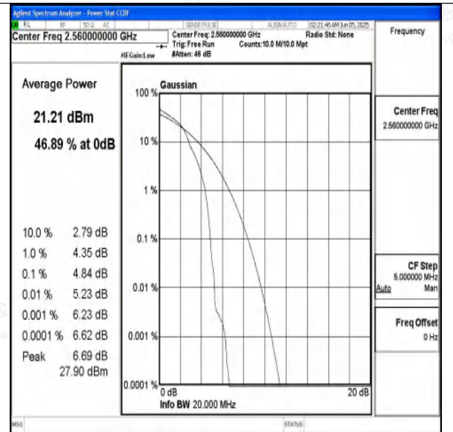
Band7-20MHz-16QAM-21350-1RB#0-PASS
