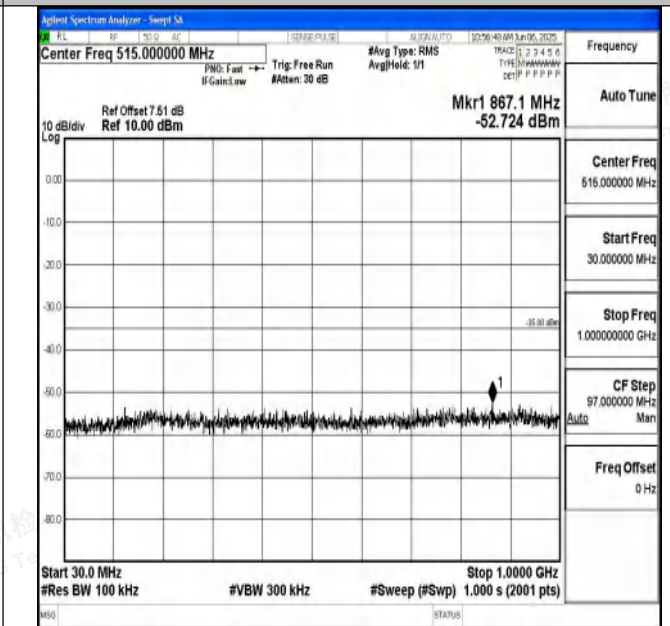
Band7_5MHz_16QAM_20775_1RB#0_30~1000_30~1000
