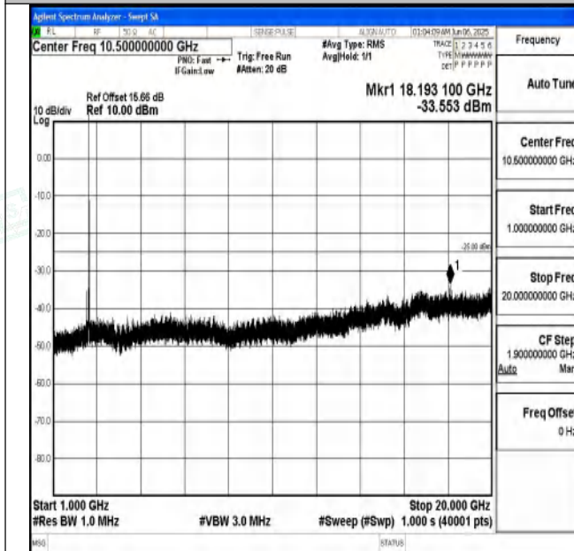
Band7_20MHz_16QAM_21350_1RB#0_1000~20000_1000~ 20000
