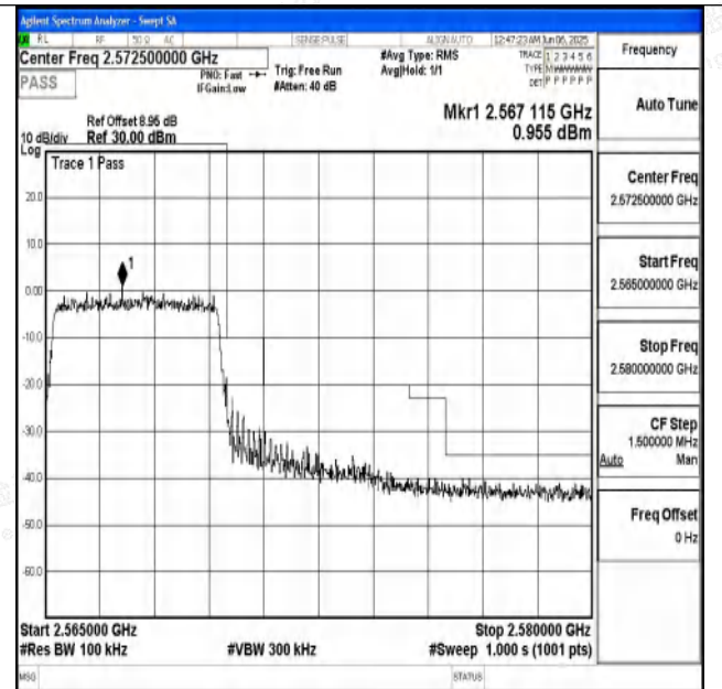
Band7_5MHz_16QAM_21425_25RB#0
