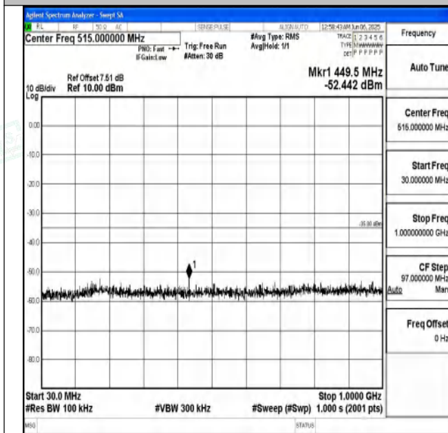
Band7_15MHz_QPSK_21375_1RB#0_30~1000_30~1000
