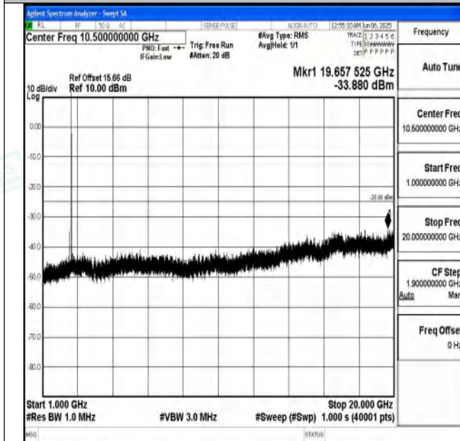
Band7_10MHz_16QAM_21400_1RB#0_1000~20000_1000~ 20000
