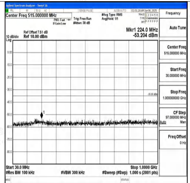
Band7_20MHz_16QAM_20850_1RB#0_30~1000_30~1000
