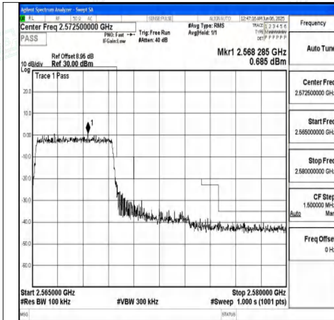
Band7_5MHz_QPSK_21425_25RB#0
