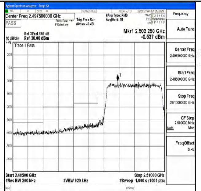
Band7_10MHz_16QAM_20800_50RB#0
