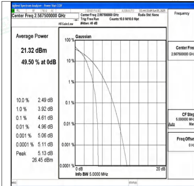
Band7-5MHz-QPSK-21425-1RB#0-PASS
