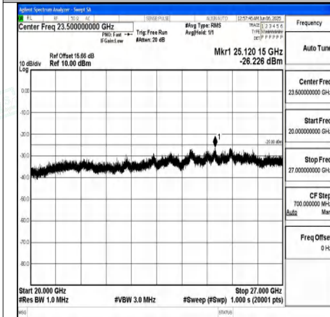
Band7_15MHz_QPSK_21100_1RB#0_20000~27000_20000~27000
