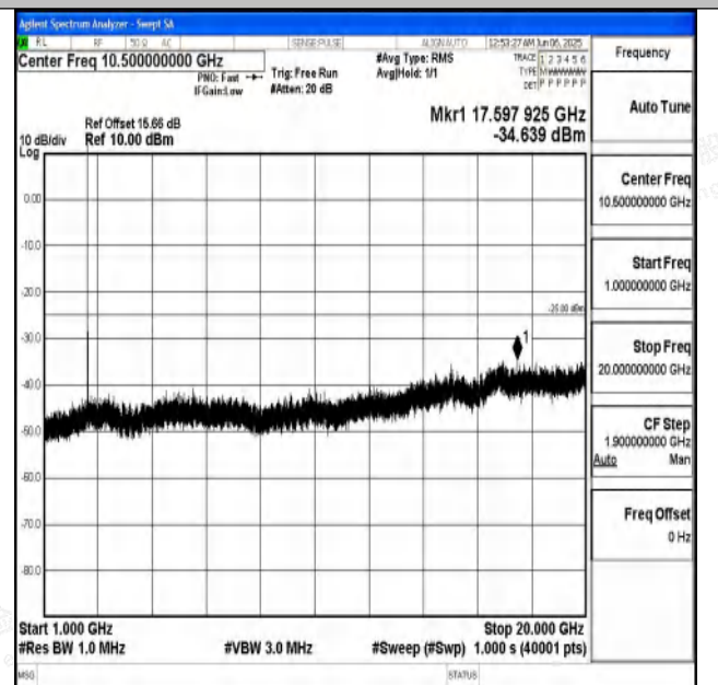
Band7_10MHz_QPSK_21100_1RB#0_1000~20000_1000~20000
