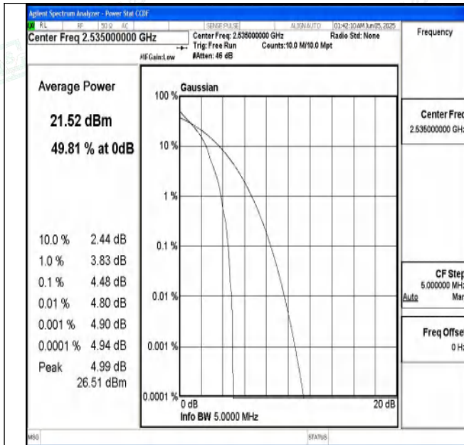
Band7-5MHz-QPSK-21100-1RB#0-PASS
