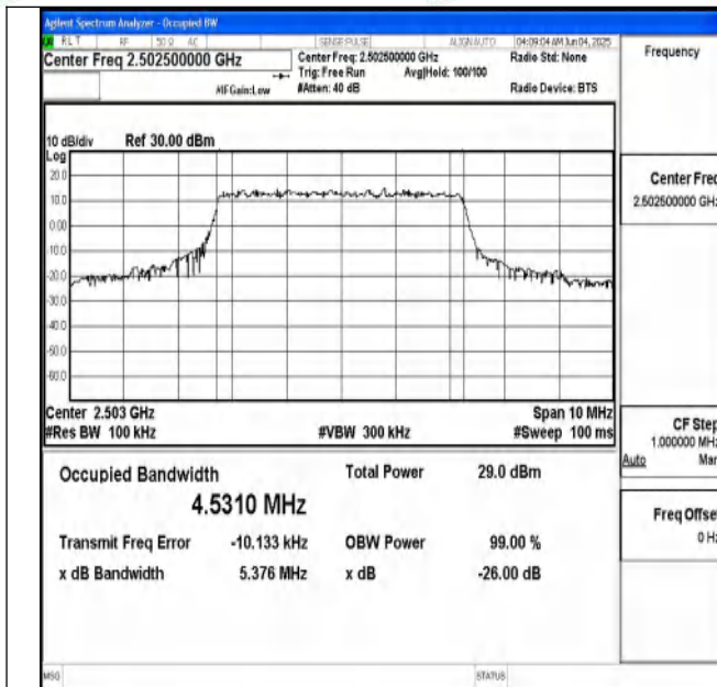
Band7-5MHz-QPSK-20775-25RB#0-PASS
