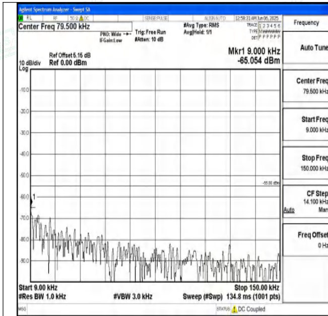
Band7_15MHz_QPSK_21375_1RB#0_0.009~0.15_0.009~0.15
