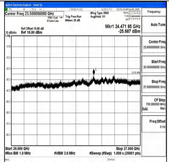
Band7_20MHz_16QAM_20850_1RB#0_20000~27000_20000 ~27000
