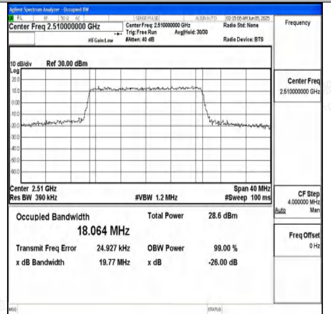
Band7-20MHz-16QAM-20850-100RB#0-PASS
