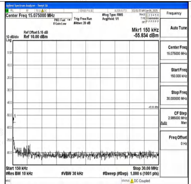
Band7_20MHz_QPSK_21100_1RB#0_0.15~30_0.15~30
