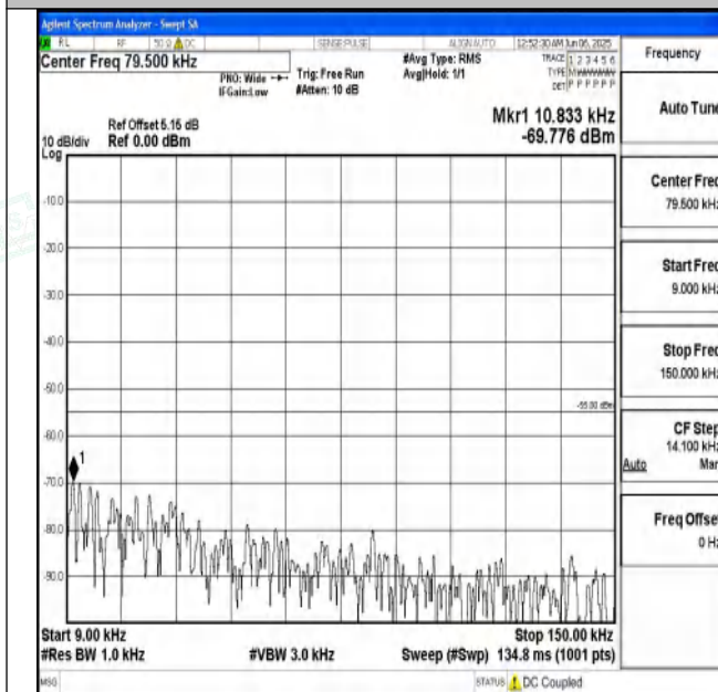
Band7_10MHz_16QAM_20800_1RB#0_0.009~0.15_0.009~0.15
