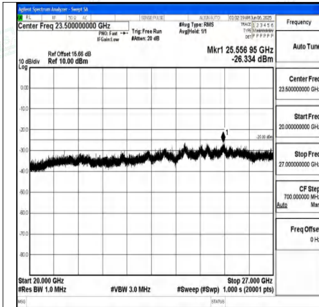
Band7_20MHz_QPSK_21100_1RB#0_20000~27000_20000 ~27000
