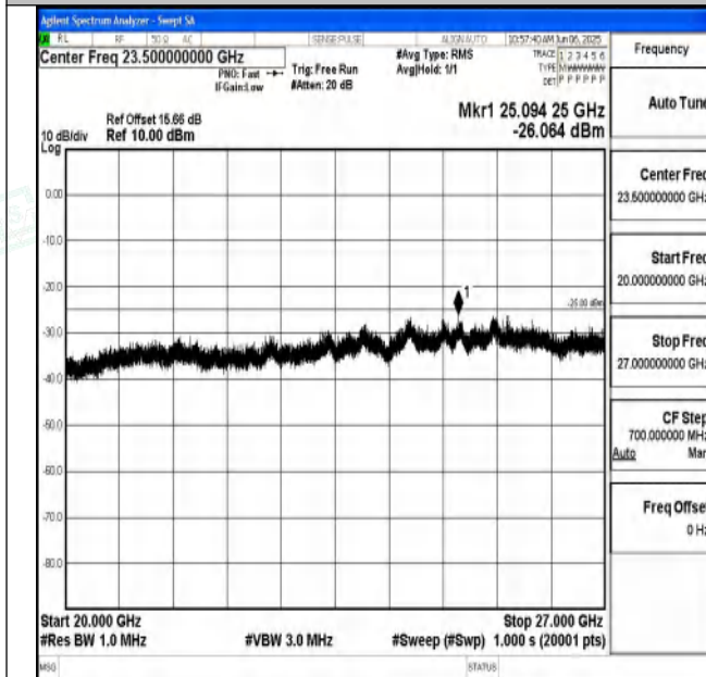
Band7_5MHz_QPSK_21100_1RB#0_20000~27000_20000~ 27000
