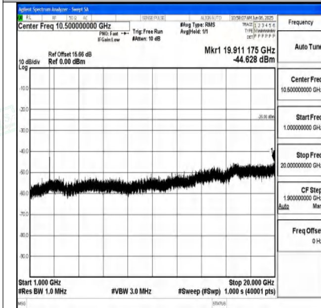
Band7_5MHz_16QAM_21100_1RB#0_1000~20000_1000~20000
