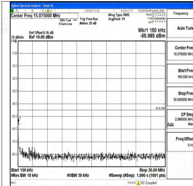
Band7_20MHz_16QAM_21350_1RB#0_0.15~30_0.15~30
