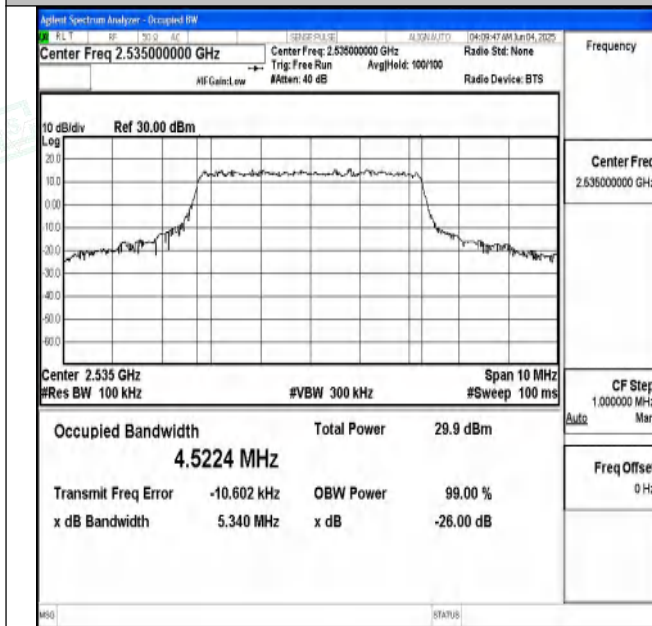
Band7-5MHz-QPSK-21100-25RB#0-PASS
