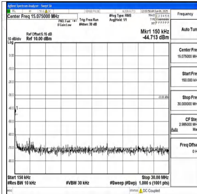
Band4_20MHz_16QAM_20050_1RB#0_0.15~30_0.15~
