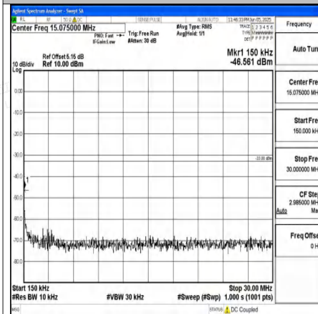
Band4_3MHz_16QAM_20175_1RB#0_0.15~30_0.15~3 0
