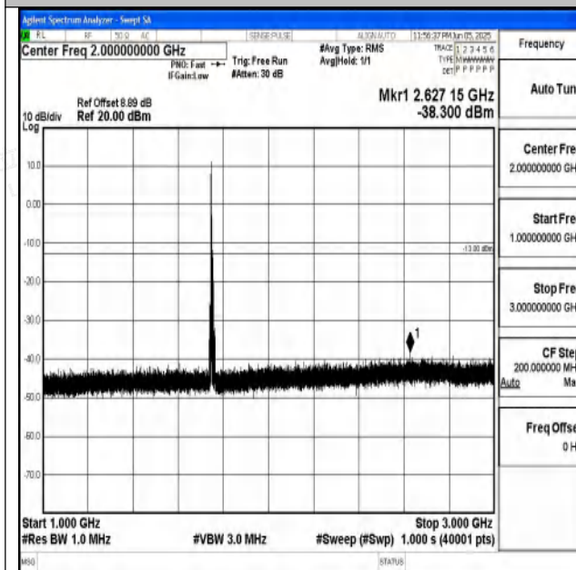
Band4_10MHz_16QAM_20350_1RB#0_1000~3000_10
