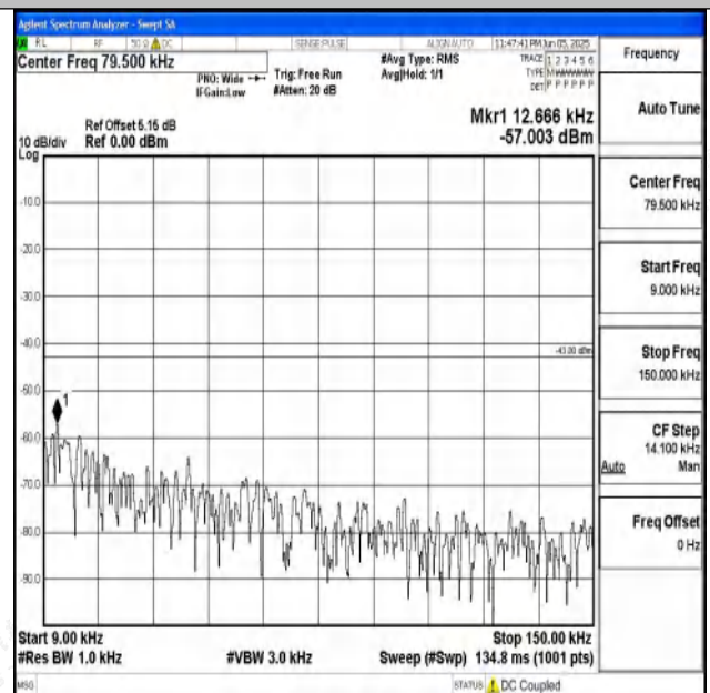
Band4_3MHz_16QAM_20385_1RB#0_0.009~0.15_0.009
