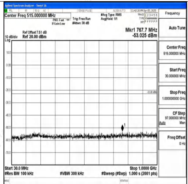
Band4_1.4MHz_16QAM_20175_1RB#0_30~1000_30~10
