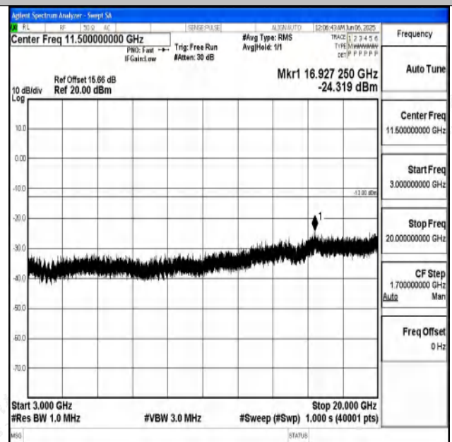
Band4_20MHz_16QAM_20300_1RB#0_3000~20000_30
