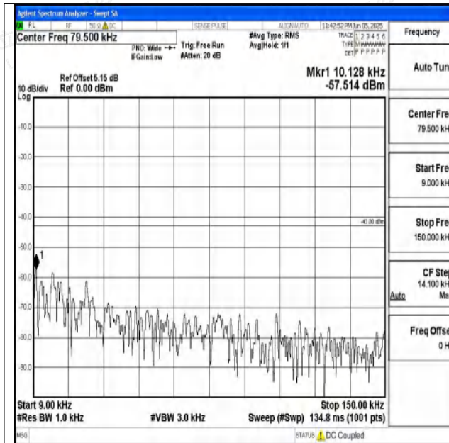
Band4_1.4MHz_QPSK_20393_1RB#0_0.009~0.15_0.0 09~0.15
