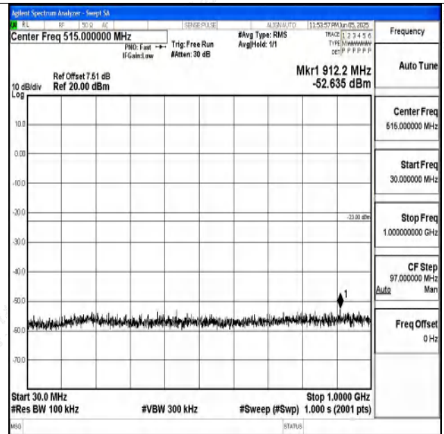
Band4_10MHz_16QAM_20000_1RB#0_30~1000_30~10
