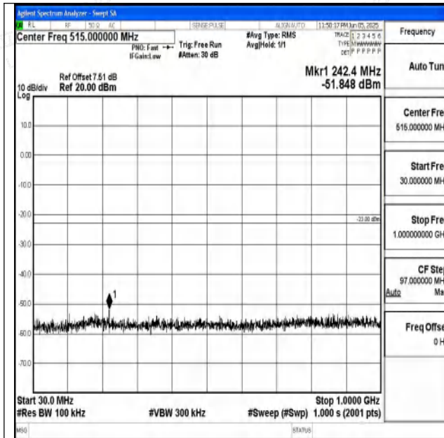
Band4_5MHz_QPSK_20175_1RB#0_30~1000_30~100
