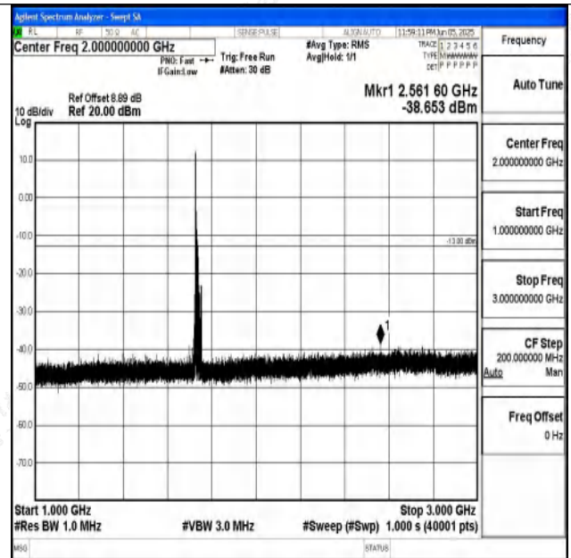
Band4_15MHz_QPSK_20175_1RB#0_1000~3000_1000
