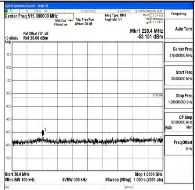
Band4_5MHz_16QAM_19975_1RB#0_30~1000_30~100 0
