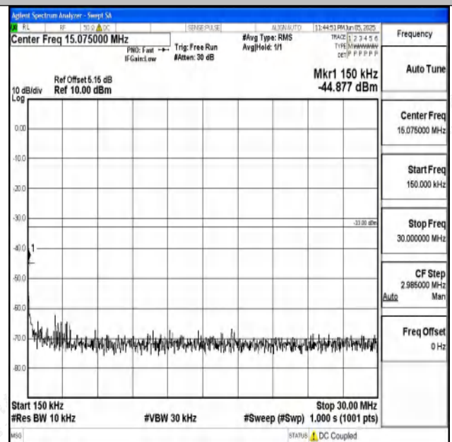
Band4_3MHz_QPSK_19965_1RB#0_0.15~30_0.15~30
