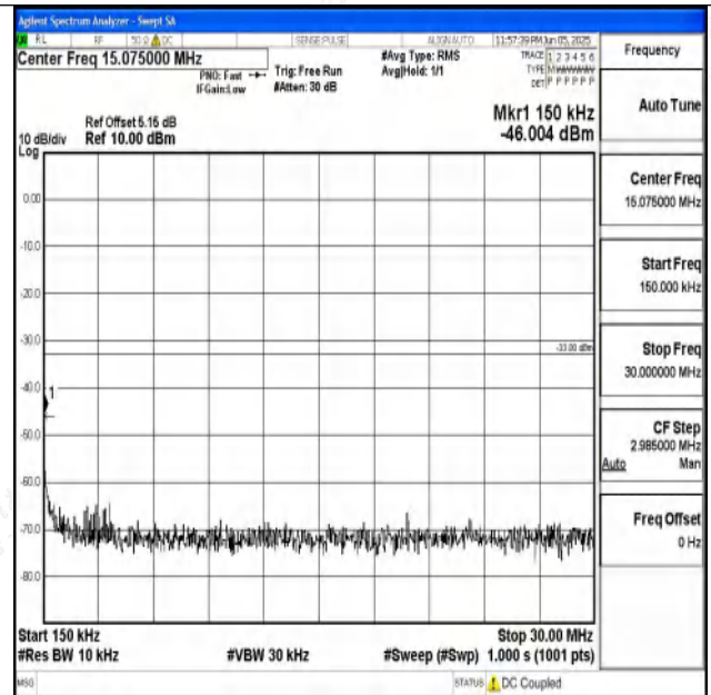
Band4_15MHz_QPSK_20025_1RB#0_0.15~30_0.15~30
