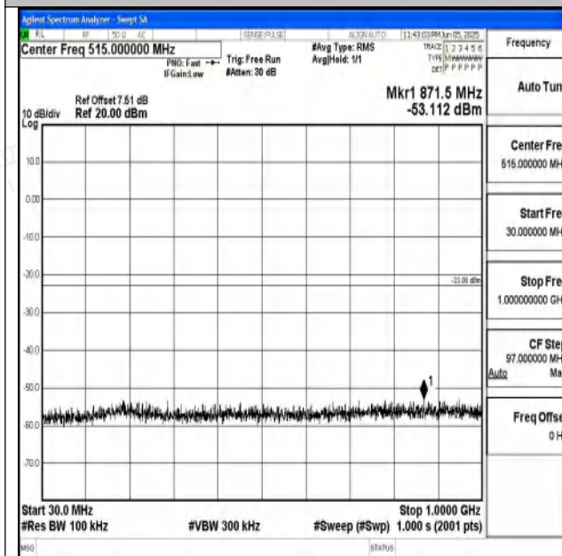
Band4_1.4MHz_QPSK_20393_1RB#0_30~1000_30~10 00
