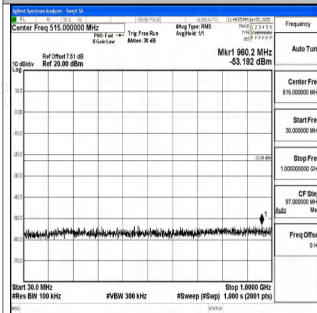
Band4_5MHz_QPSK_19975_1RB#0_30~1000_30~100 0
