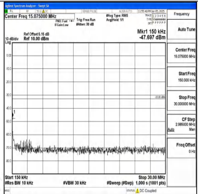
Band4_10MHz_QPSK_20350_1RB#0_0.15~30_0.15~30
