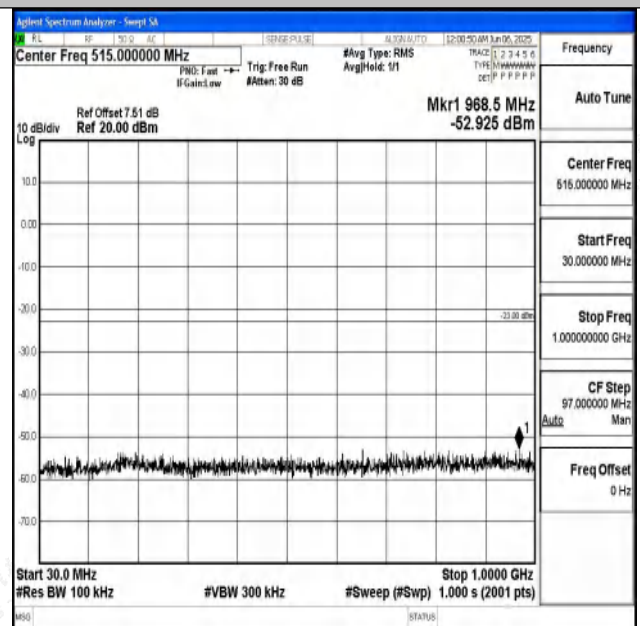
Band4_15MHz_16QAM_20325_1RB#0_30~1000_30~10 00
