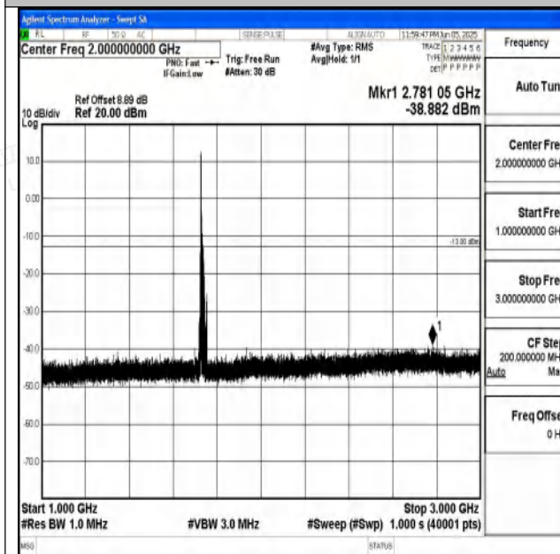
Band4_15MHz_16QAM_20175_1RB#0_1000~3000_1000~3000
