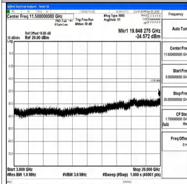
Band4_3MHz_QPSK_20385_1RB#0_3000~20000_300
