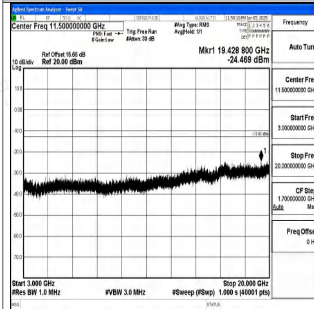
Band4_15MHz_QPSK_20175_1RB#0_3000~20000_3000~20000
