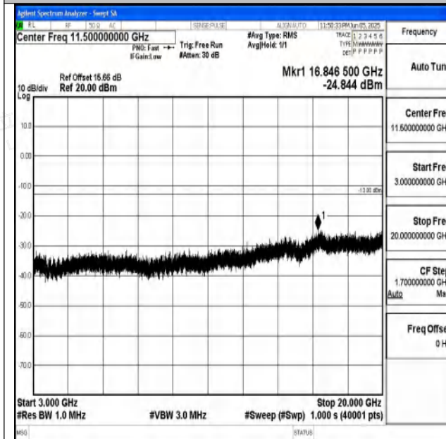
Band4_5MHz_QPSK_20175_1RB#0_3000~20000_300
