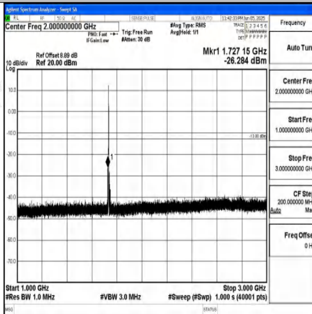
Band4_1.4MHz_16QAM_20175_1RB#0_1000~3000_10
