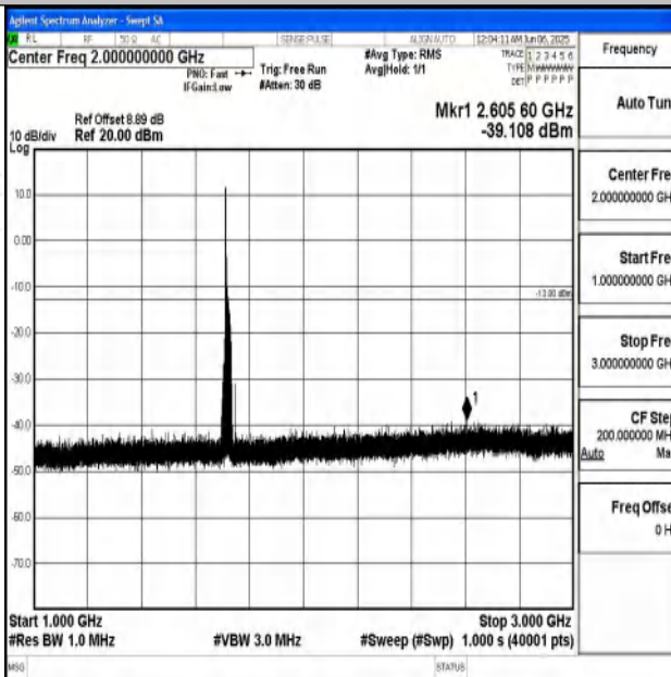
Band4_20MHz_16QAM_20050_1RB#0_1000~3000_10
