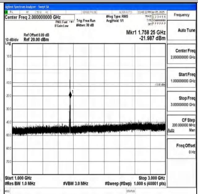
Band4_1.4MHz_QPSK_20393_1RB#0_1000~3000_1000 ~3000
