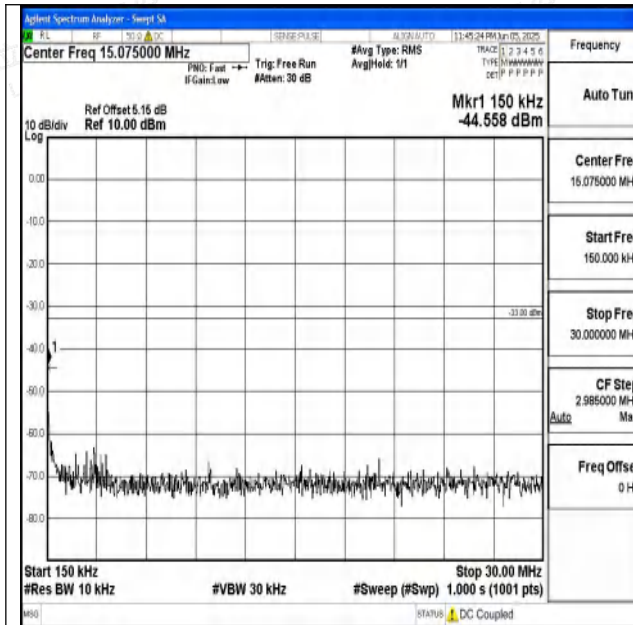
Band4_3MHz_16QAM_19965_1RB#0_0.15~30_0.15~3
