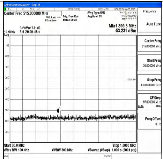
Band4_10MHz_16QAM_20350_1RB#0_30~1000_30~10
