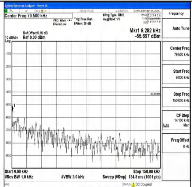
Band4_15MHz_16QAM_20175_1RB#0_0.009~0.15_0.009~0.15
