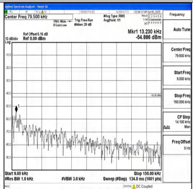
Band4_20MHz_16QAM_20300_1RB#0_0.009~0.15_0.009~0.15
