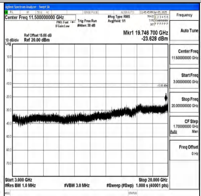
Band4_3MHz_16QAM_19965_1RB#0_3000~20000_300
