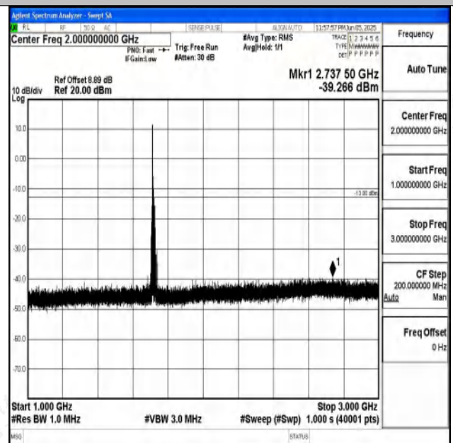
Band4_15MHz_QPSK_20025_1RB#0_1000~3000_1000 ~3000
