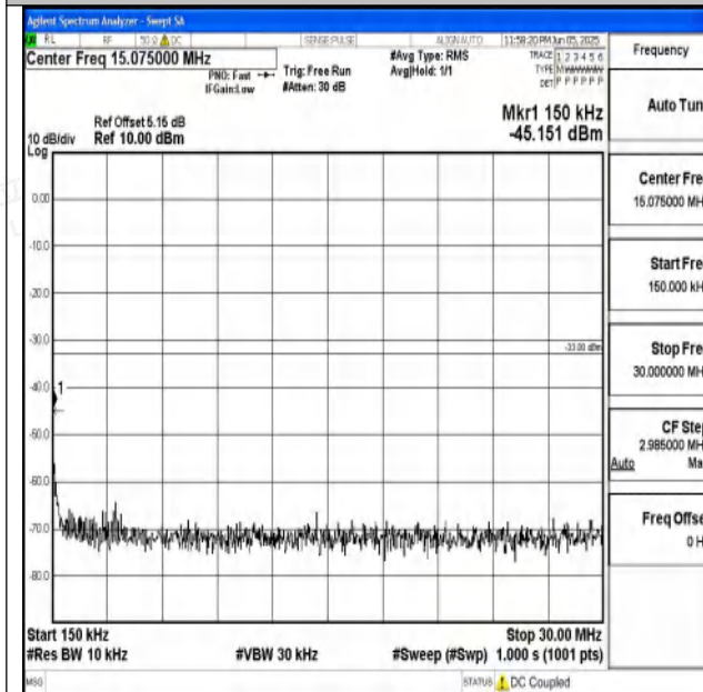
Band4_15MHz_16QAM_20025_1RB#0_0.15~30_0.15~ 30
