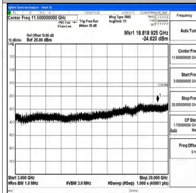
Band4_1.4MHz_QPSK_20175_1RB#0_3000~20000_3000~20000
