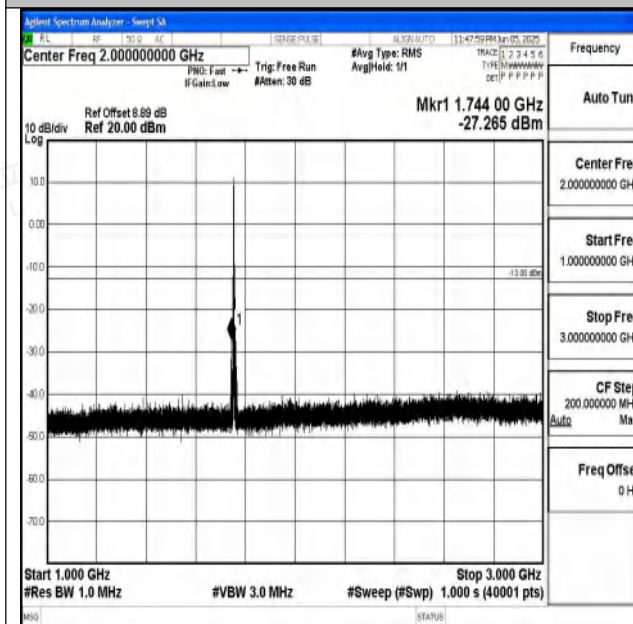
Band4_3MHz_16QAM_20385_1RB#0_1000~3000_100
