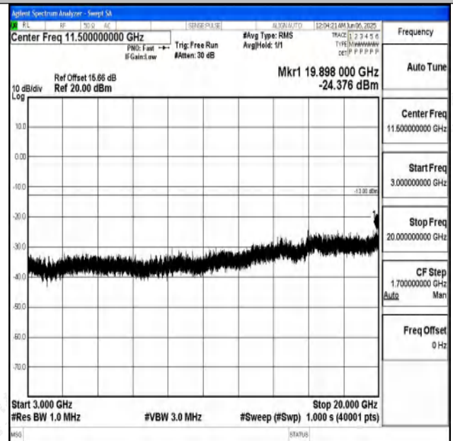
Band4_20MHz_16QAM_20050_1RB#0_3000~20000_30
