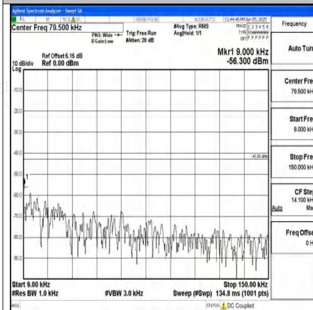
Band4_3MHz_QPSK_19965_1RB#0_0.009~0.15_0.009~0.15
