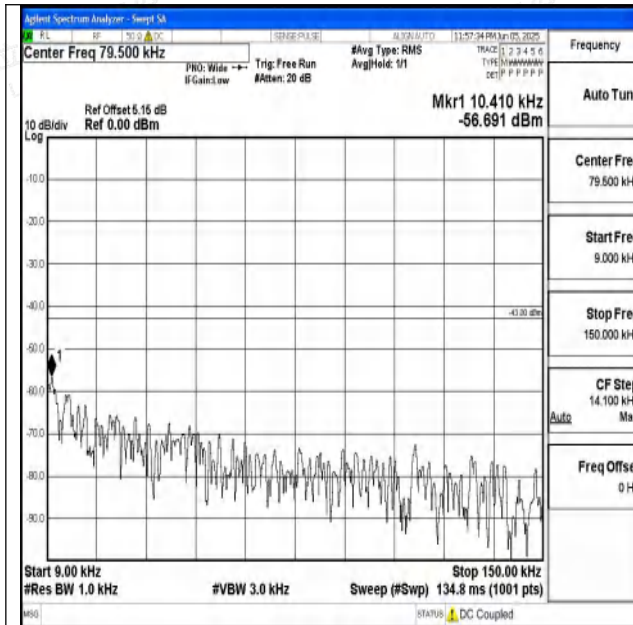
Band4_15MHz_QPSK_20025_1RB#0_0.009~0.15_0.00 9~0.15
