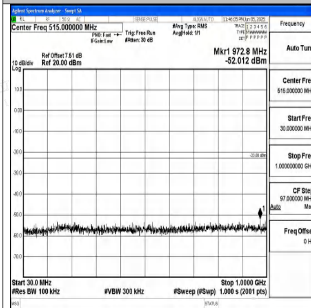
Band4_3MHz_QPSK_20175_1RB#0_30~1000_30~100 0
