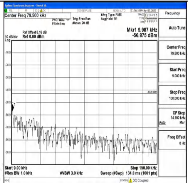
Band4_10MHz_16QAM_20350_1RB#0_0.009~0.15_0.009~0.15
