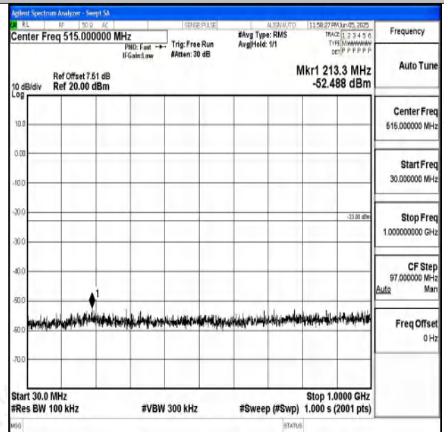
Band4_15MHz_16QAM_20025_1RB#0_30~1000_30~10 00
