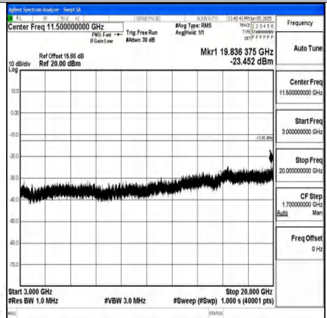
Band4_1.4MHz_16QAM_20175_1RB#0_3000~20000_30
