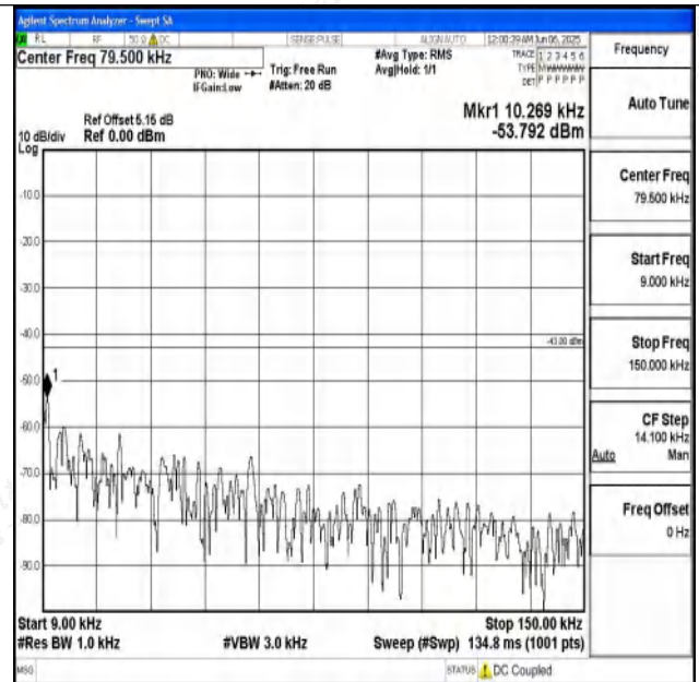
Band4_15MHz_16QAM_20325_1RB#0_0.009~0.15_0.00 9~0.15
