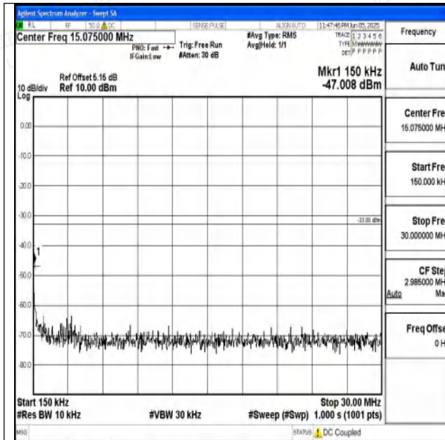
Band4_3MHz_16QAM_20385_1RB#0_0.15~30_0.15~3
