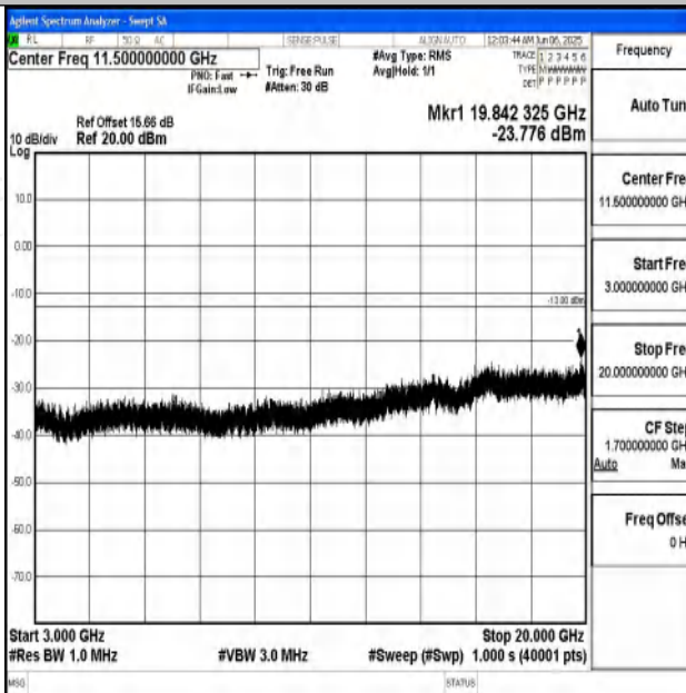
Band4_20MHz_QPSK_20050_1RB#0_3000~20000_3000~20000
