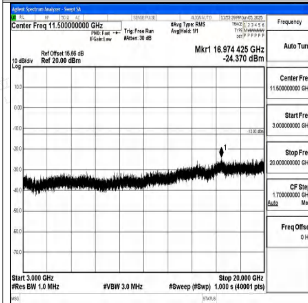
Band4_10MHz_QPSK_20000_1RB#0_3000~20000_3000~20000
