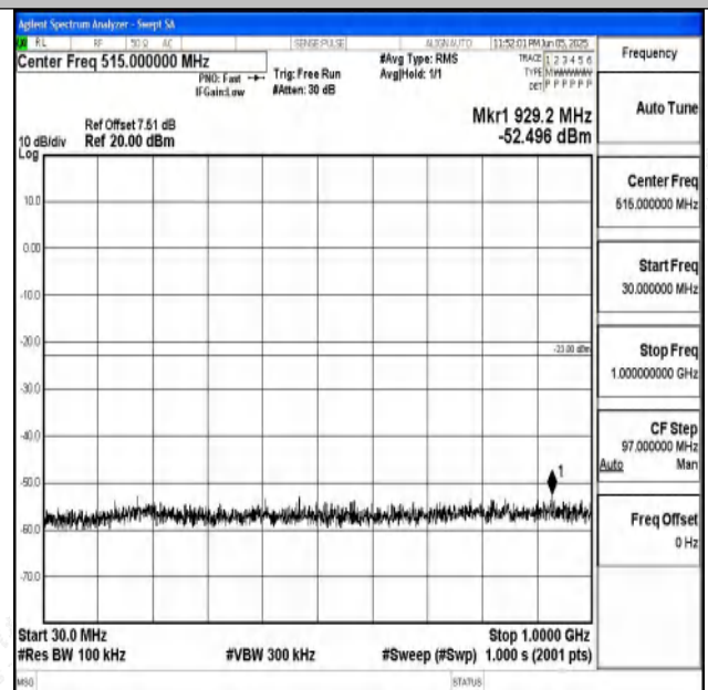
Band4_5MHz_16QAM_20375_1RB#0_30~1000_30~100 0
