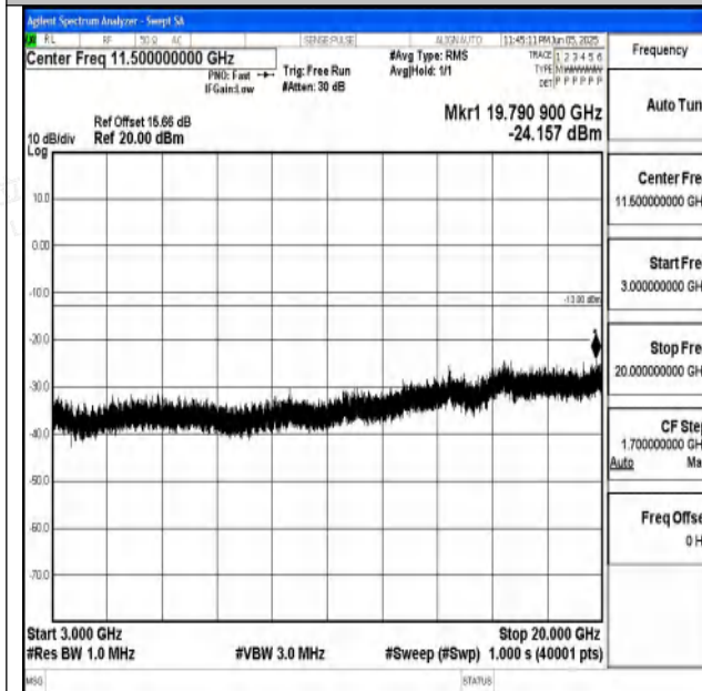
Band4_3MHz_QPSK_19965_1RB#0_3000~20000_300
