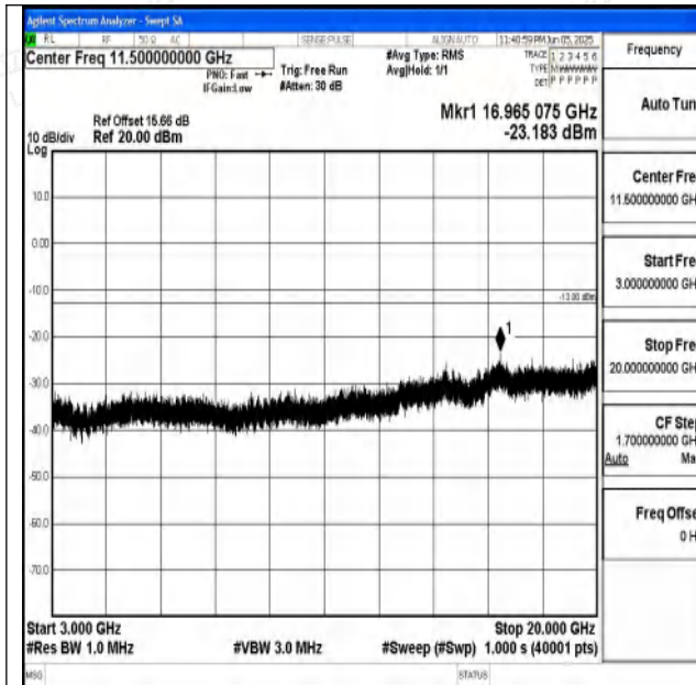
Band4_1.4MHz_QPSK_19957_1RB#0_3000~20000_30 00~20000
