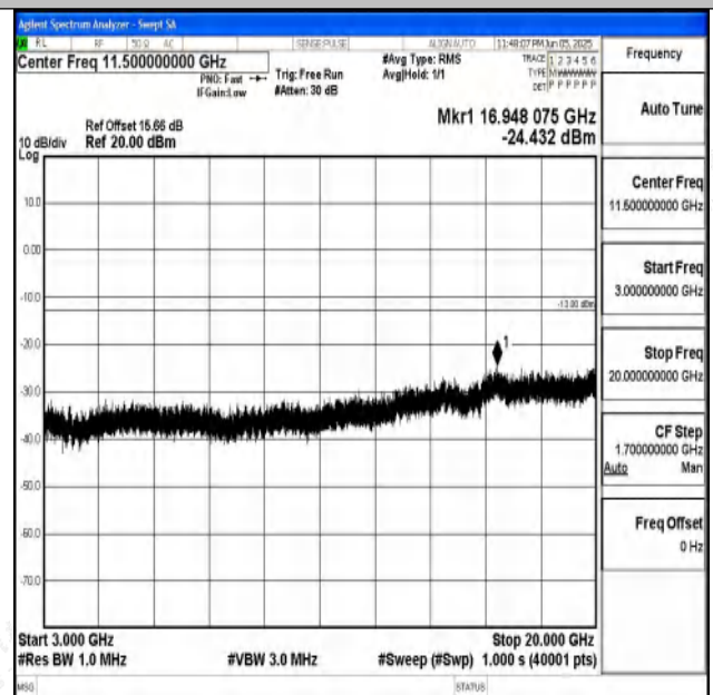
Band4_3MHz_16QAM_20385_1RB#0_3000~20000_300
