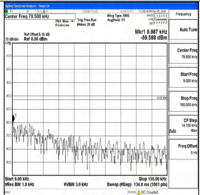
Band4_5MHz_16QAM_20175_1RB#0_0.009~0.15_0.009
