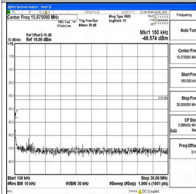
Band4_15MHz_16QAM_20325_1RB#0_0.15~30_0.15~ 30
