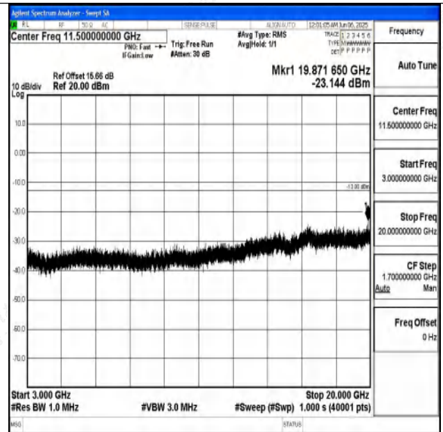
Band4_15MHz_16QAM_20325_1RB#0_3000~20000_30 00~20000
