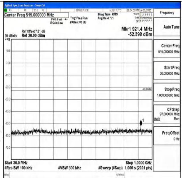
Band4_20MHz_16QAM_20050_1RB#0_30~1000_30~10
