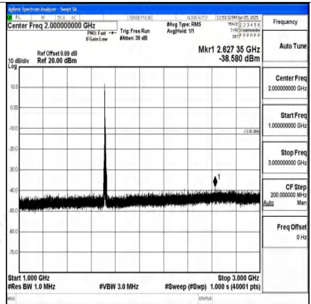
Band4_10MHz_QPSK_20000_1RB#0_1000~3000_1000~3000
