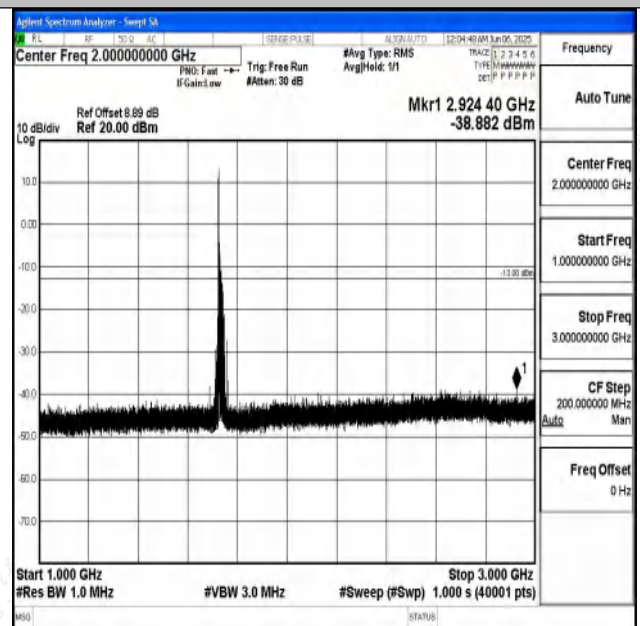
Band4_20MHz_QPSK_20175_1RB#0_1000~3000_1000 ~3000
