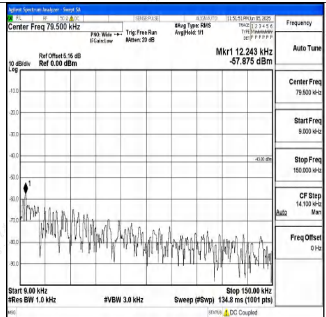
Band4_5MHz_16QAM_20375_1RB#0_0.009~0.15_0.009 ~0.15
