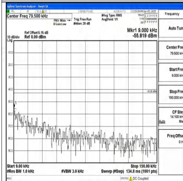
Band4_10MHz_QPSK_20000_1RB#0_0.009~0.15_0.00 9~0.15
