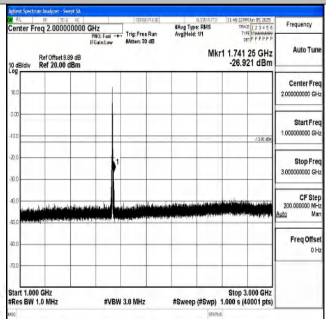
Band4_3MHz_QPSK_20175_1RB#0_1000~3000_1000~ 3000
