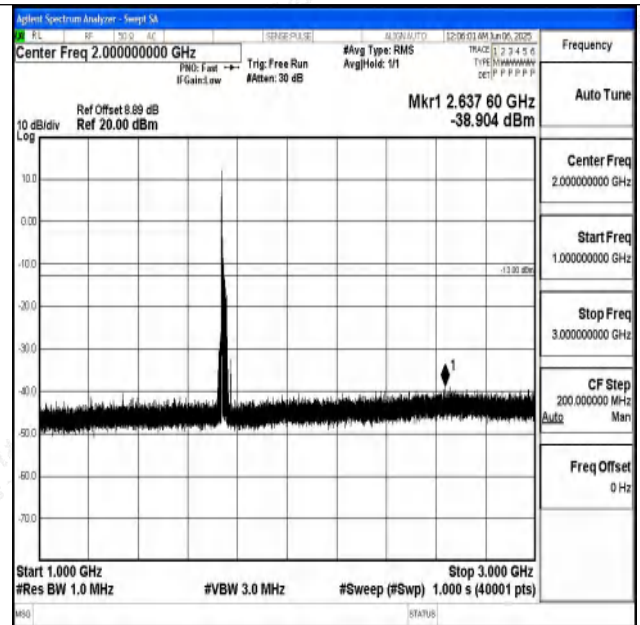
Band4_20MHz_QPSK_20300_1RB#0_1000~3000_1000~3000
