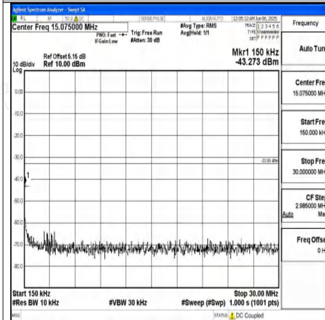
Band4_20MHz_16QAM_20175_1RB#0_0.15~30_0.15~ 30
