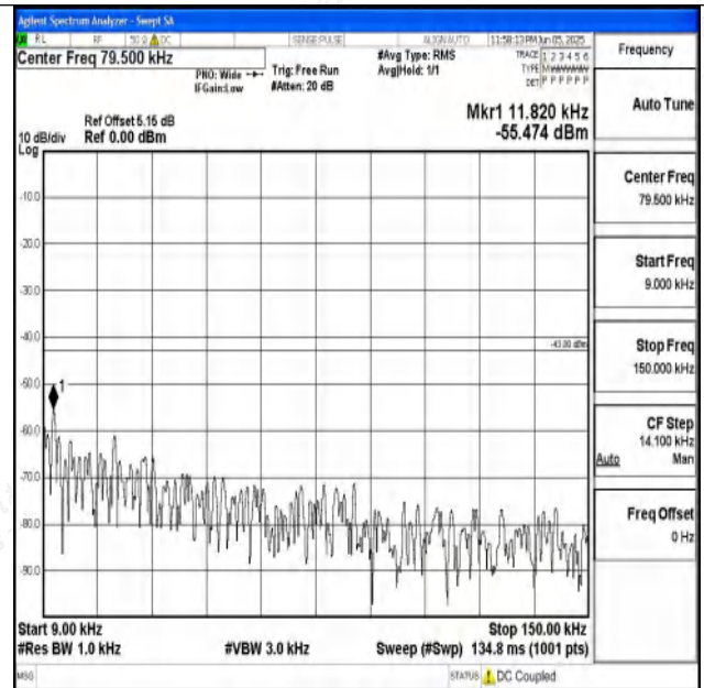
Band4_15MHz_16QAM_20025_1RB#0_0.009~0.15_0.00 9~0.15
