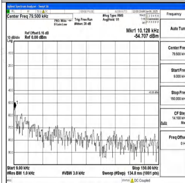
Band4_20MHz_QPSK_20050_1RB#0_0.009~0.15_0.00 9~0.15
