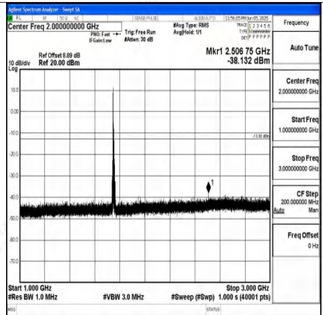
Band4_10MHz_QPSK_20350_1RB#0_1000~3000_1000~3000
