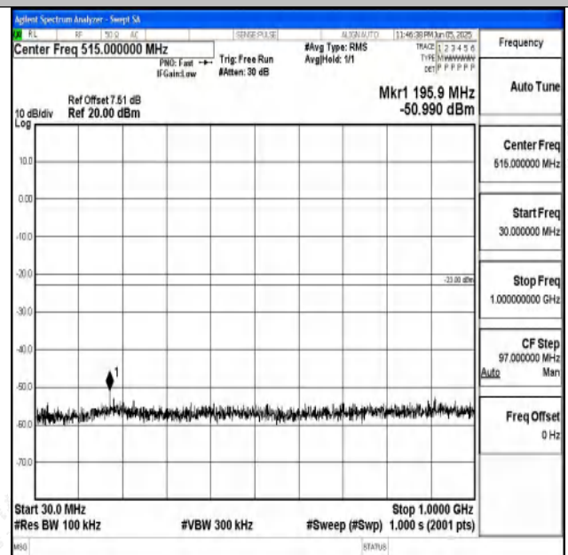
Band4_3MHz_16QAM_20175_1RB#0_30~1000_30~100 0
