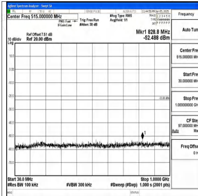
Band4_3MHz_QPSK_19965_1RB#0_30~1000_30~100
