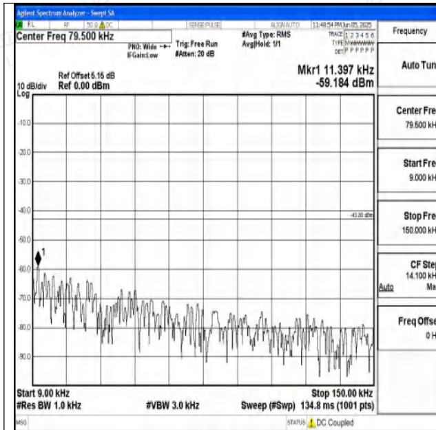
Band4_5MHz_QPSK_19975_1RB#0_0.009~0.15_0.009 ~0.15
