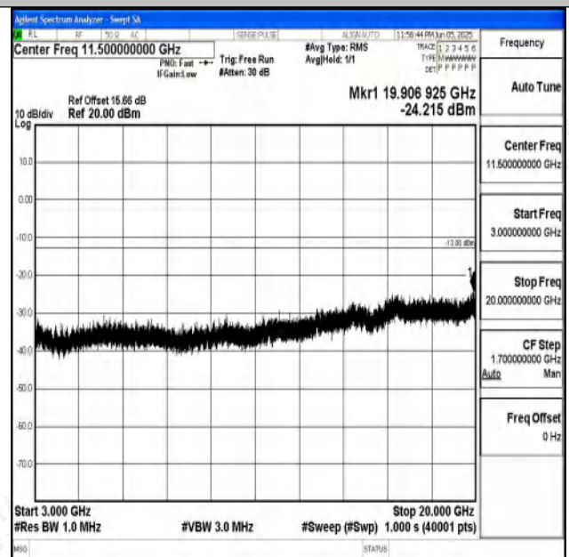
Band4_10MHz_16QAM_20350_1RB#0_3000~20000_30
