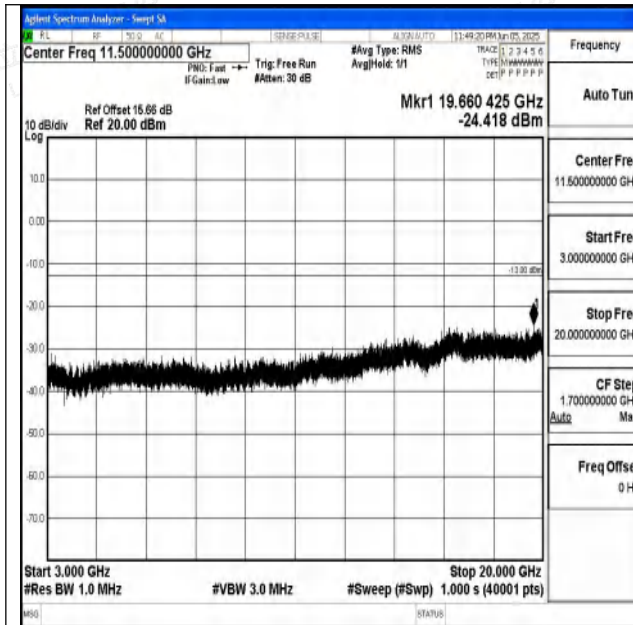
Band4_5MHz_QPSK_19975_1RB#0_3000~20000_300 0~20000
