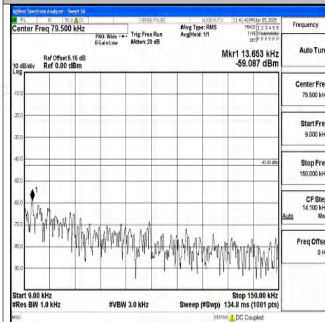
Band4_1.4MHz_QPSK_20175_1RB#0_0.009~0.15_0.0 09~0.15
