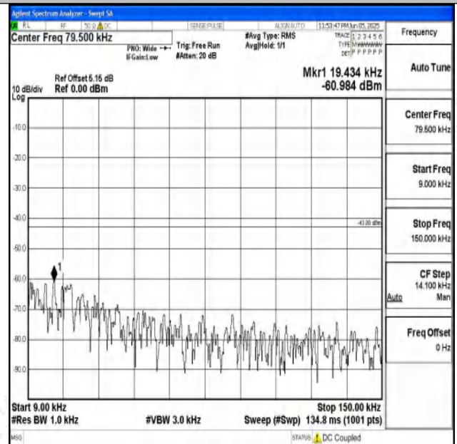
Band4_10MHz_16QAM_20000_1RB#0_0.009~0.15_0.009~0.15
