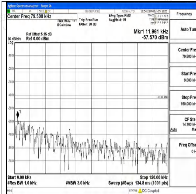
Band4_10MHz_QPSK_20175_1RB#0_0.009~0.15_0.00 9~0.15
