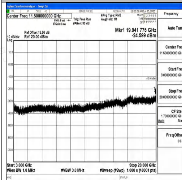
Band4_20MHz_QPSK_20300_1RB#0_3000~20000_3000~20000
