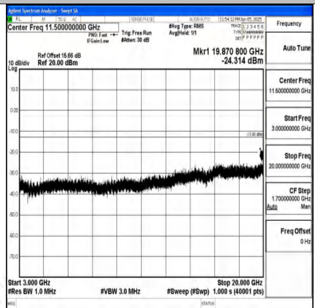
Band4_10MHz_16QAM_20000_1RB#0_3000~20000_30
