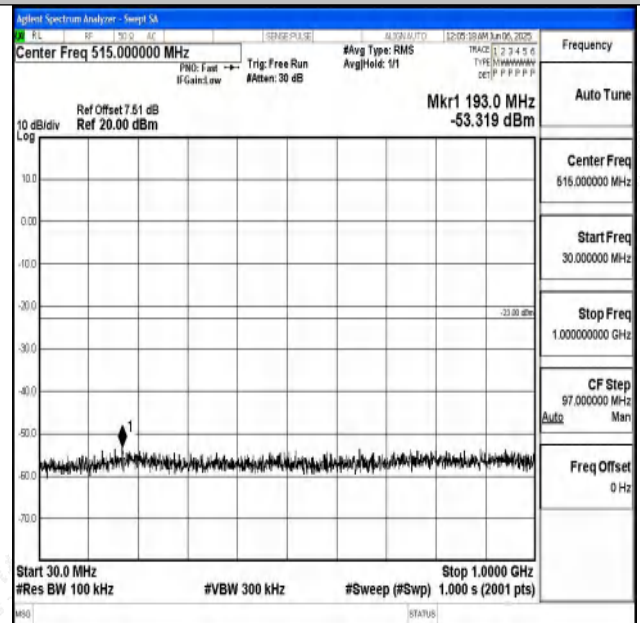
Band4_20MHz_16QAM_20175_1RB#0_30~1000_30~10 00
