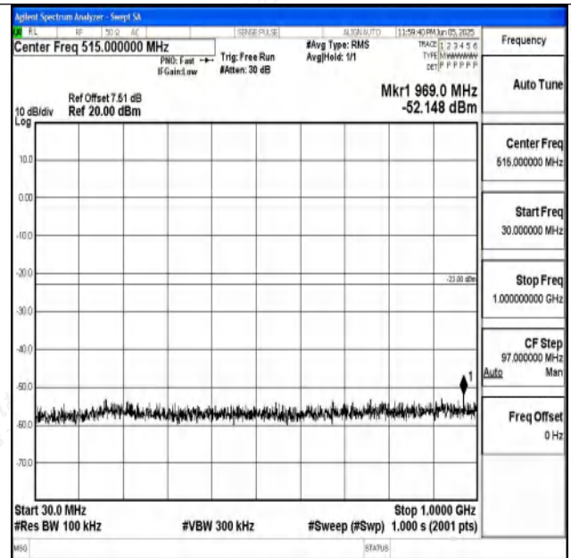
Band4_15MHz_16QAM_20175_1RB#0_30~1000_30~10
