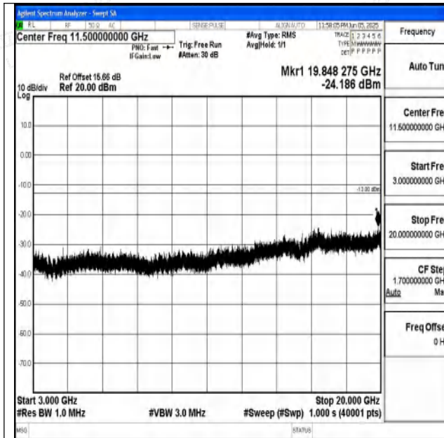
Band4_15MHz_QPSK_20025_1RB#0_3000~20000_30 00~20000
