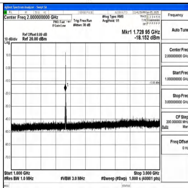
Band4_1.4MHz_QPSK_20175_1RB#0_1000~3000_1000~3000
