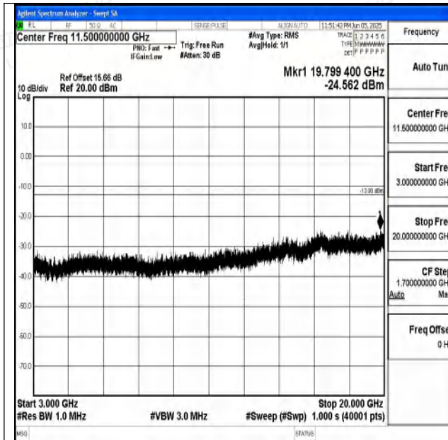
Band4_5MHz_QPSK_20375_1RB#0_3000~20000_300 0~20000
