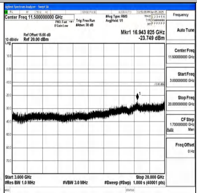
Band4_5MHz_16QAM_20175_1RB#0_3000~20000_300
