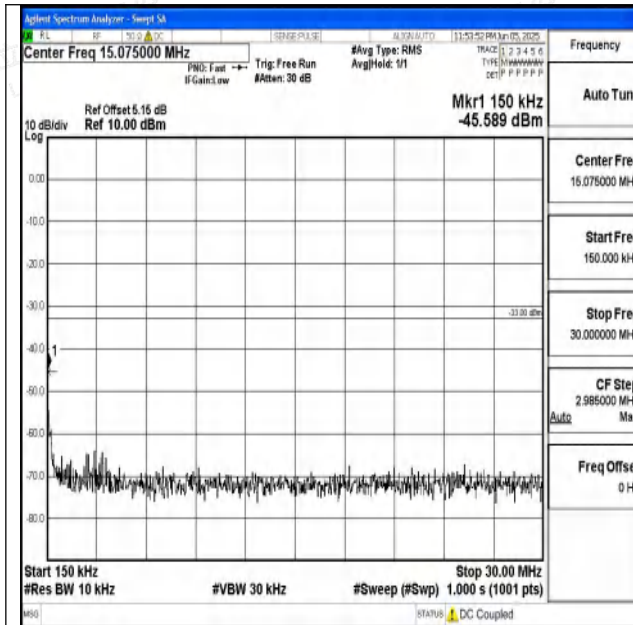
Band4_10MHz_16QAM_20000_1RB#0_0.15~30_0.15~
