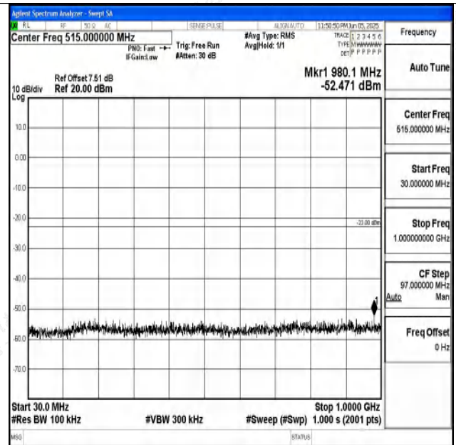
Band4_5MHz_16QAM_20175_1RB#0_30~1000_30~100
