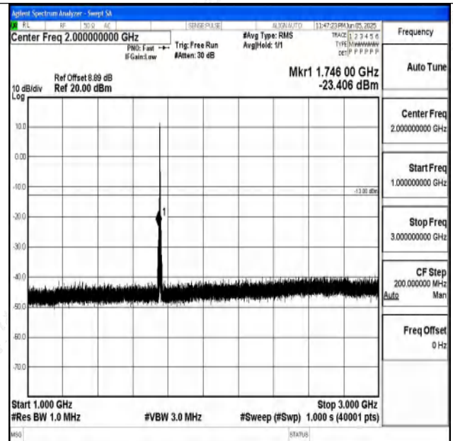
Band4_3MHz_QPSK_20385_1RB#0_1000~3000_1000~
