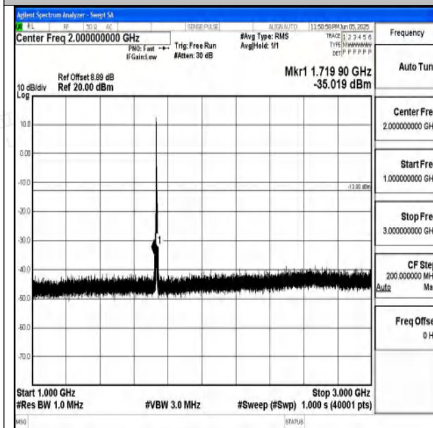
Band4_5MHz_16QAM_20175_1RB#0_1000~3000_100
