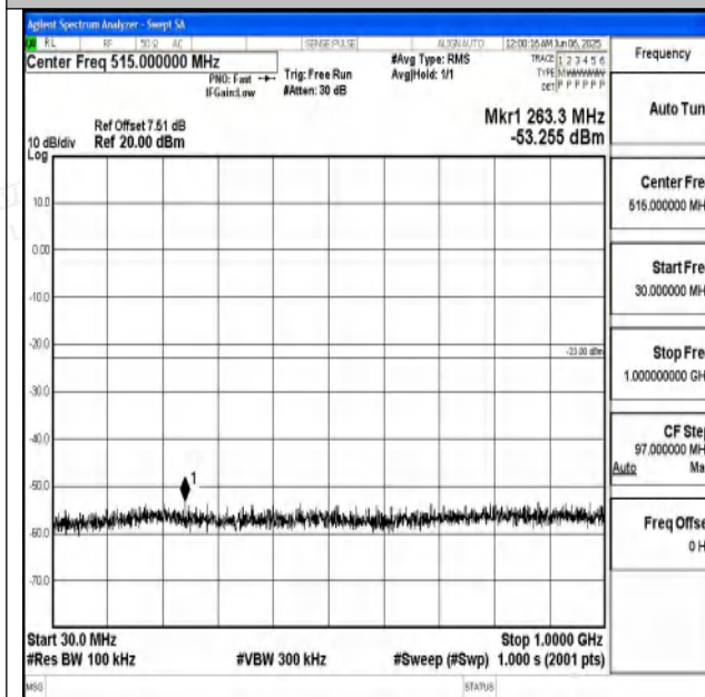
Band4_15MHz_QPSK_20325_1RB#0_30~1000_30~10 00
