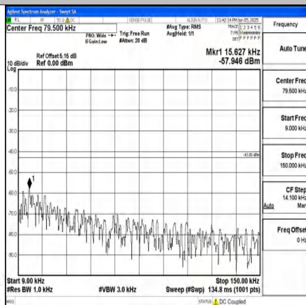
Band4_1.4MHz_16QAM_20175_1RB#0_0.009~0.15_0.009~0.15
