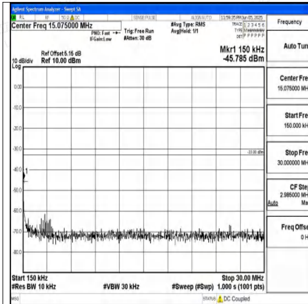
Band4_15MHz_16QAM_20175_1RB#0_0.15~30_0.15~30
