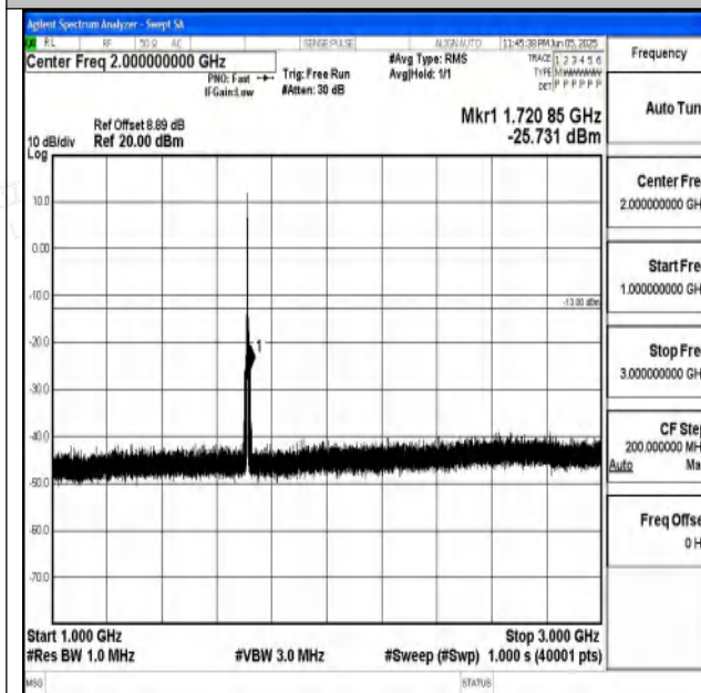
Band4_3MHz_16QAM_19965_1RB#0_1000~3000_100
