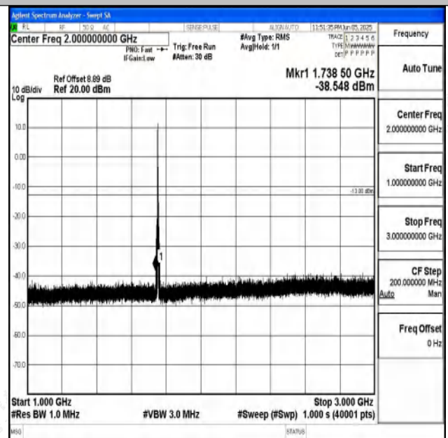
Band4_5MHz_QPSK_20375_1RB#0_1000~3000_1000~ 3000
