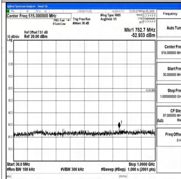
Band4_5MHz_QPSK_20375_1RB#0_30~1000_30~100 0
