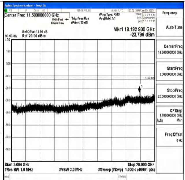
Band4_5MHz_16QAM_20375_1RB#0_3000~20000_300 0~20000
