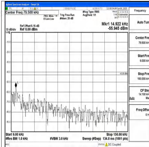
Band4_15MHz_QPSK_20325_1RB#0_0.009~0.15_0.00 9~0.15
