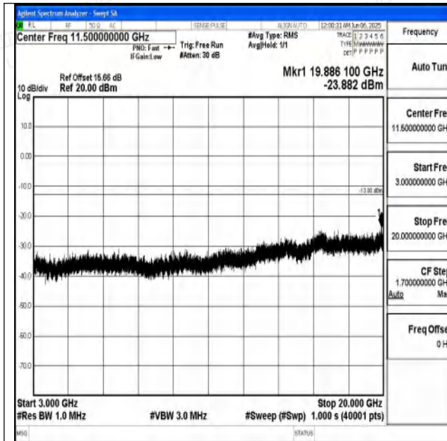
Band4_15MHz_QPSK_20325_1RB#0_3000~20000_30 00~20000
