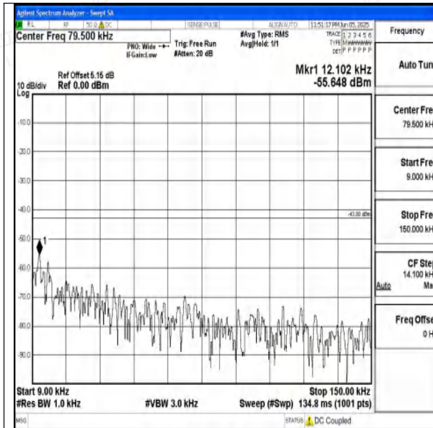
Band4_5MHz_QPSK_20375_1RB#0_0.009~0.15_0.009 ~0.15
