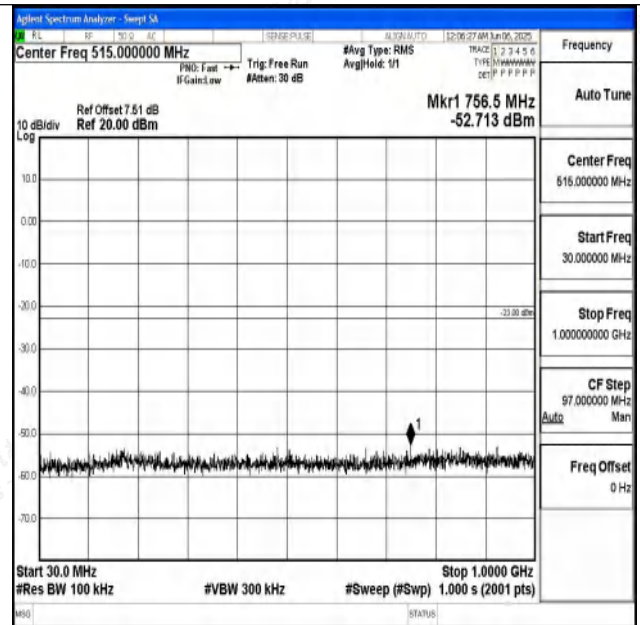
Band4_20MHz_16QAM_20300_1RB#0_30~1000_30~10
