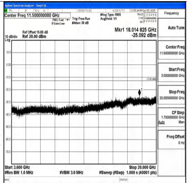
Band4_10MHz_16QAM_20175_1RB#0_3000~20000_30 00~20000
