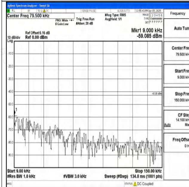
Band4_10MHz_QPSK_20350_1RB#0_0.009~0.15_0.00 9~0.15
