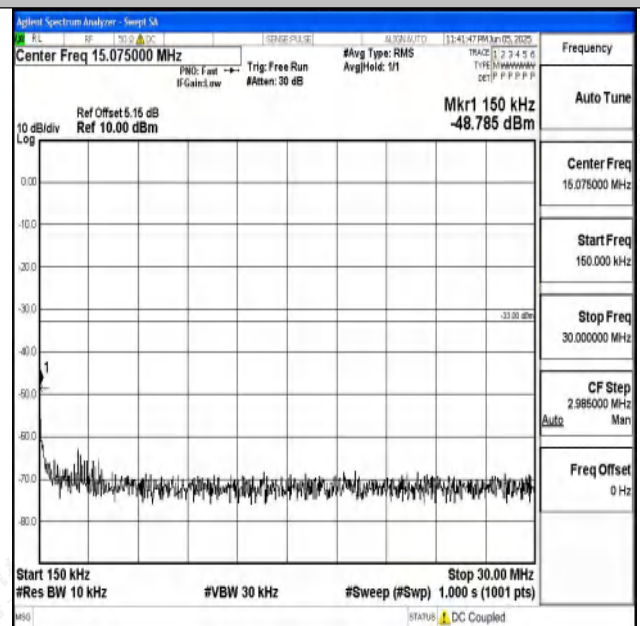
Band4_1.4MHz_QPSK_20175_1RB#0_0.15~30_0.15~30
