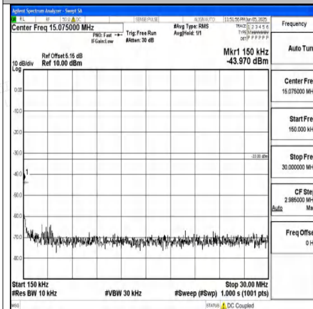
Band4_5MHz_16QAM_20375_1RB#0_0.15~30_0.15~3 0
