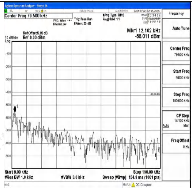
Band4_20MHz_16QAM_20175_1RB#0_0.009~0.15_0.00 9~0.15
