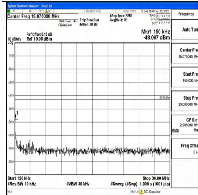
Band4_1.4MHz_16QAM_20175_1RB#0_0.15~30_0.15~
