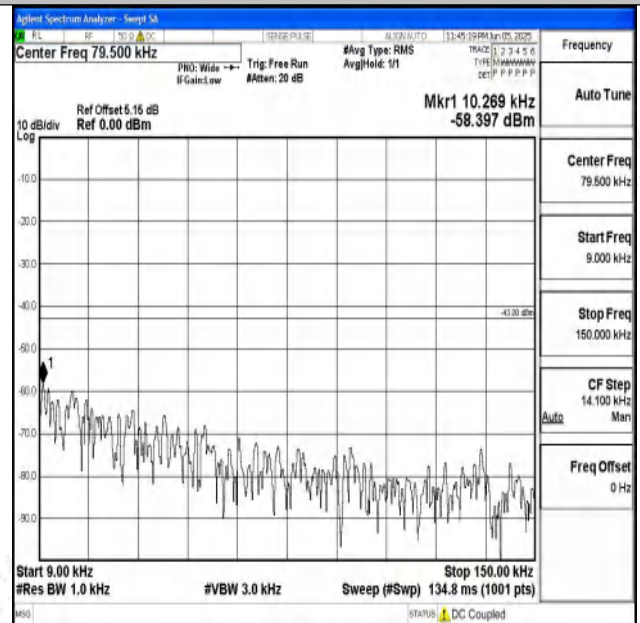
Band4_3MHz_16QAM_19965_1RB#0_0.009~0.15_0.009
