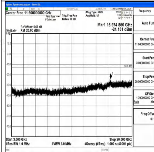
Band4_10MHz_QPSK_20350_1RB#0_3000~20000_3000~20000
