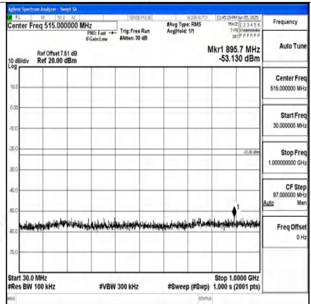
Band4_3MHz_16QAM_19965_1RB#0_30~1000_30~100
