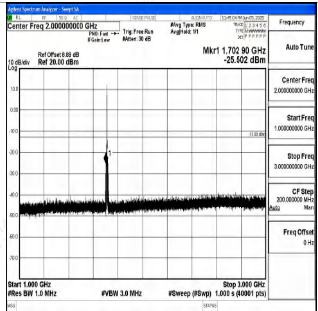
Band4_3MHz_QPSK_19965_1RB#0_1000~3000_1000~
