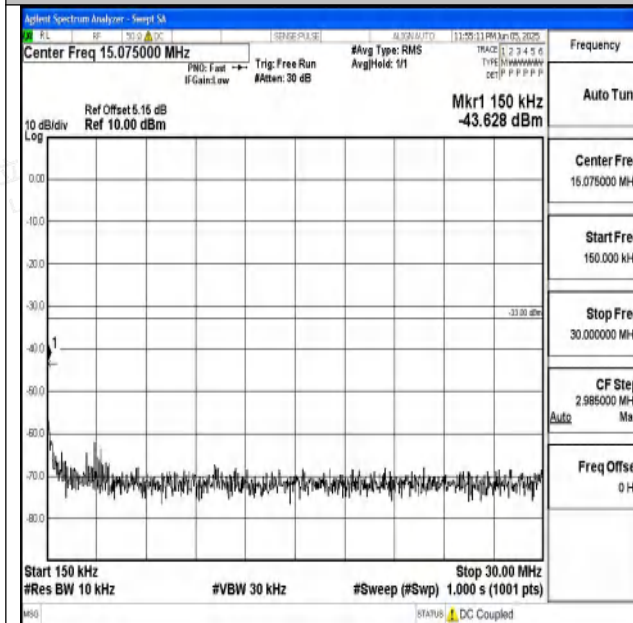
Band4_10MHz_16QAM_20175_1RB#0_0.15~30_0.15~ 30
