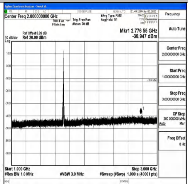
Band4_5MHz_QPSK_19975_1RB#0_1000~3000_1000~ 3000
