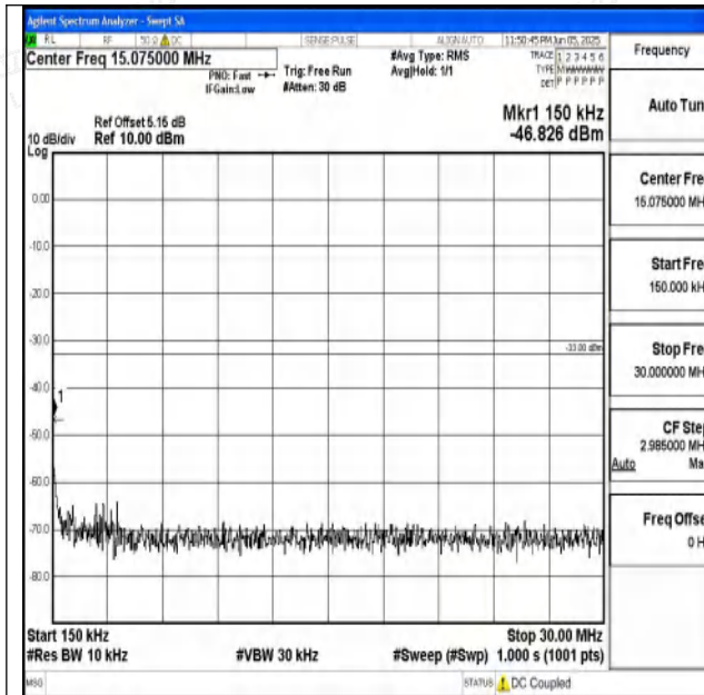
Band4_5MHz_16QAM_20175_1RB#0_0.15~30_0.15~3
