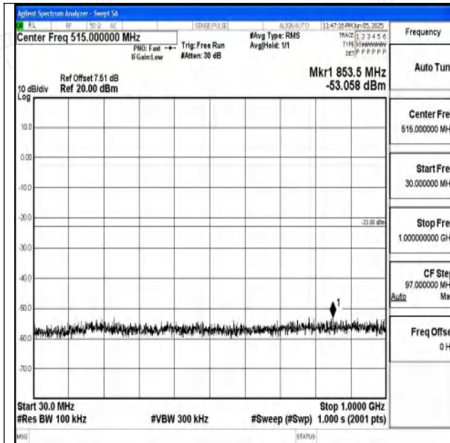
Band4_3MHz_QPSK_20385_1RB#0_30~1000_30~100
