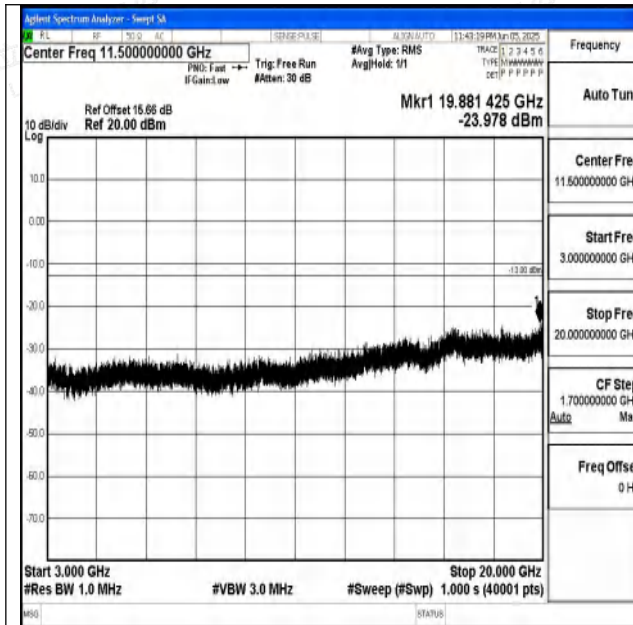
Band4_1.4MHz_QPSK_20393_1RB#0_3000~20000_30 00~20000
