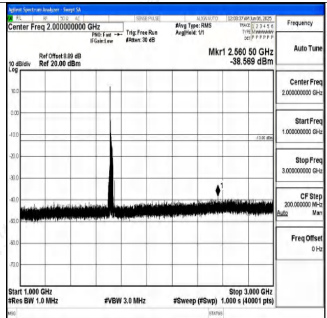
Band4_20MHz_QPSK_20050_1RB#0_1000~3000_1000
