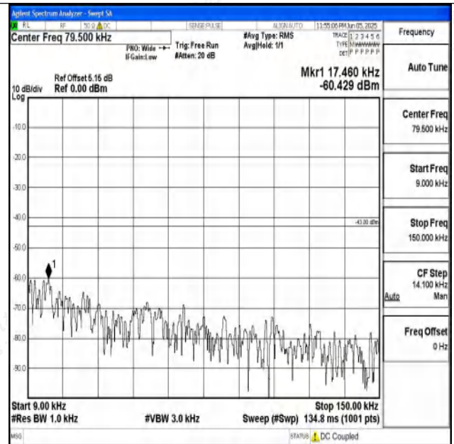
Band4_10MHz_16QAM_20175_1RB#0_0.009~0.15_0.00 9~0.15
