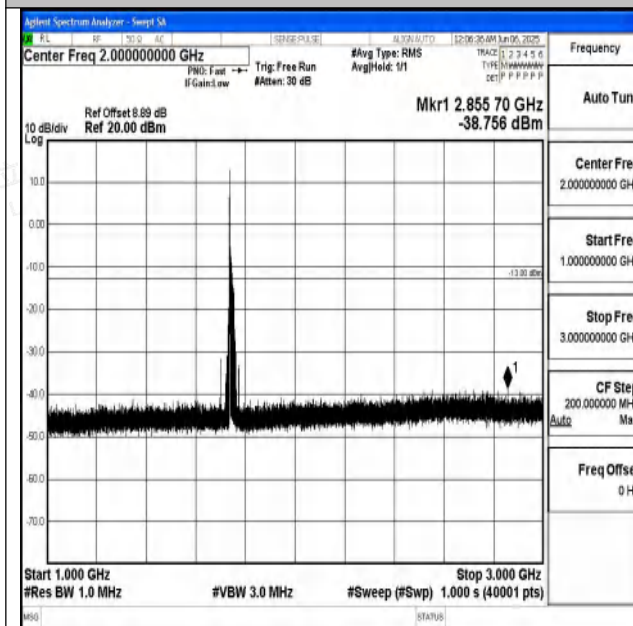
Band4_20MHz_16QAM_20300_1RB#0_1000~3000_10
