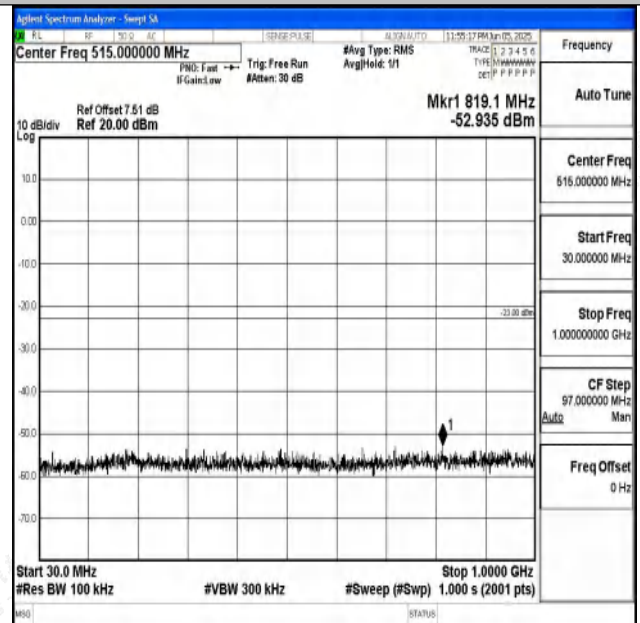
Band4_10MHz_16QAM_20175_1RB#0_30~1000_30~10 00
