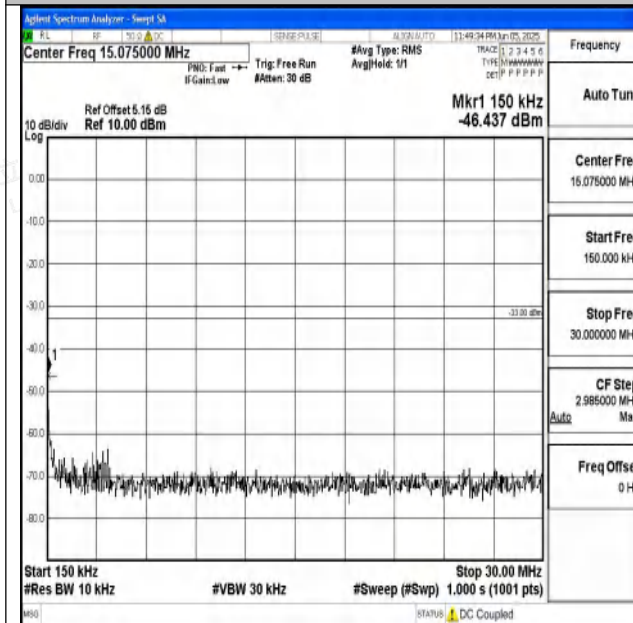
Band4_5MHz_16QAM_19975_1RB#0_0.15~30_0.15~3 0
