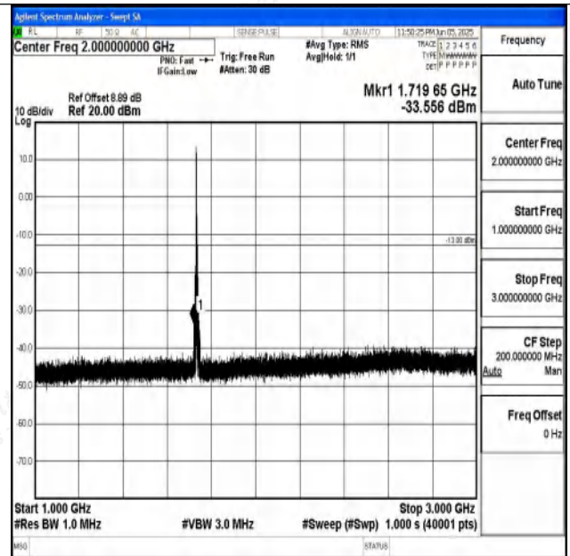
Band4_5MHz_QPSK_20175_1RB#0_1000~3000_1000~
