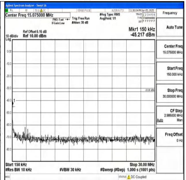
Band2_15MHz_QPSK_18675_1RB#0_0.15~30_0.15~30
