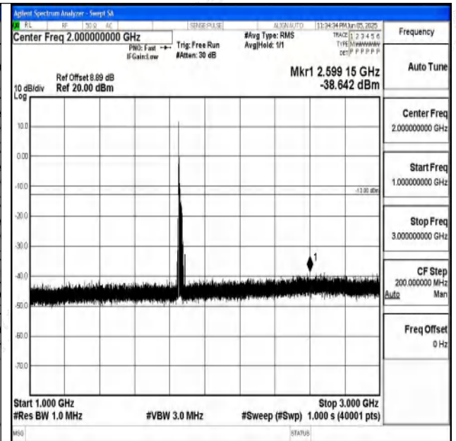
Band2_20MHz_QPSK_18700_1RB#0_1000~3000_1000 ~3000
