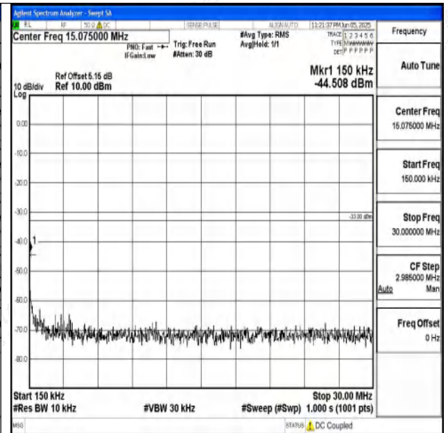
Band2_5MHz_QPSK_18625_1RB#0_0.15~30_0.15~30
