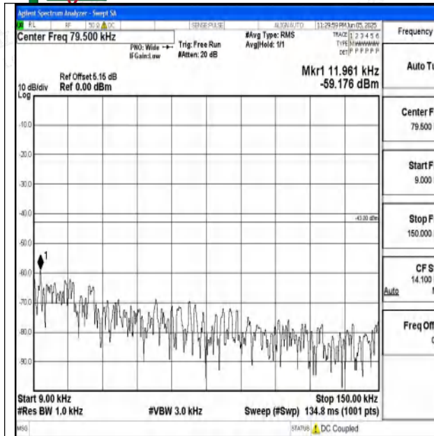
Band2_15MHz_QPSK_18675_1RB#0_0.009~0.15_0.09~0.15
