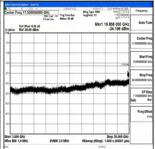
Band2_20MHz_16QAM_19100_1RB#0_3000~20000_30 00~20000
