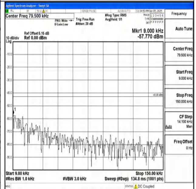
Band2_20MHz_16QAM_18700_1RB#0_0.009~0.15_0.0 09~0.15
