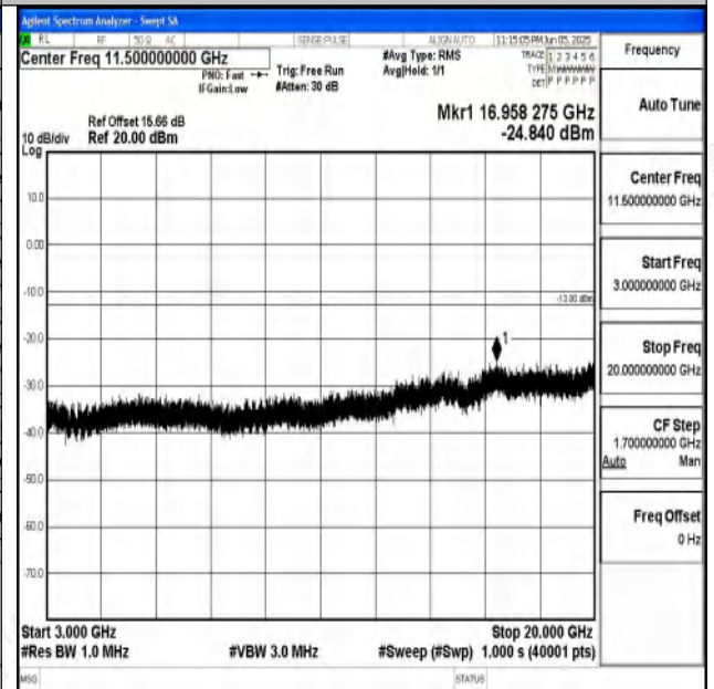
Band2_1.4MHz_16QAM_18900_1RB#0_3000~20000_3 000~20000
