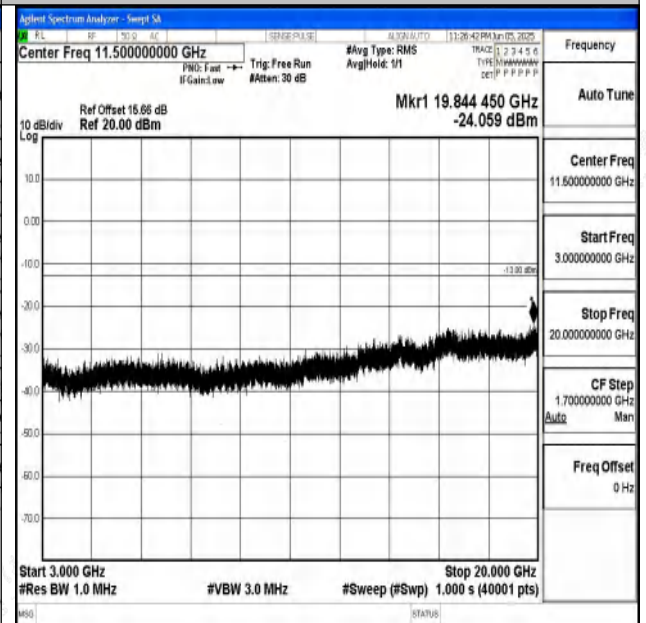
Band2_10MHz_16QAM_18650_1RB#0_3000~20000_3000~20000
