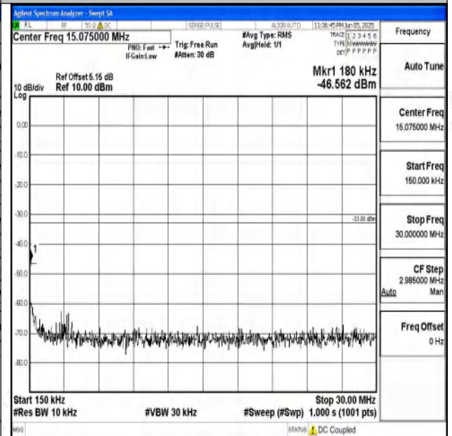
Band2_20MHz_QPSK_19100_1RB#0_0.15~30_0.15~30
