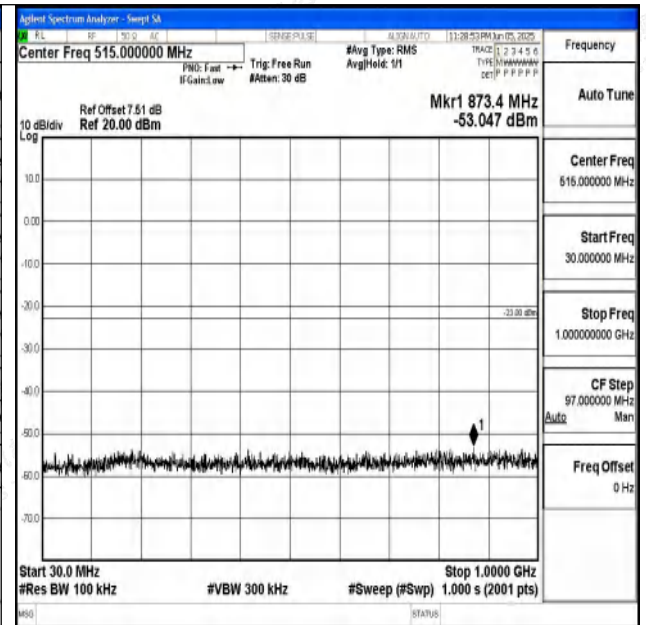
Band2_10MHz_16QAM_19150_1RB#0_30~1000_30~10 00
