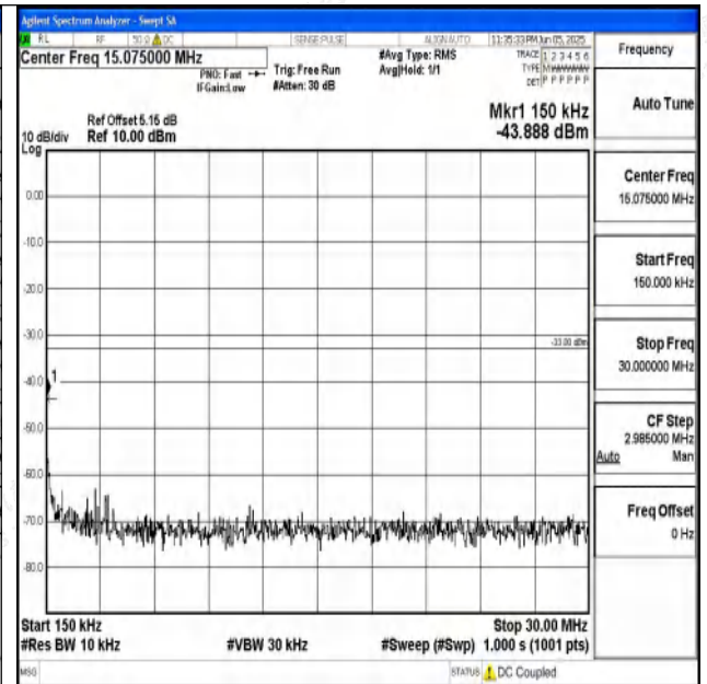
Band2_20MHz_QPSK_18900_1RB#0_0.15~30_0.15~30
