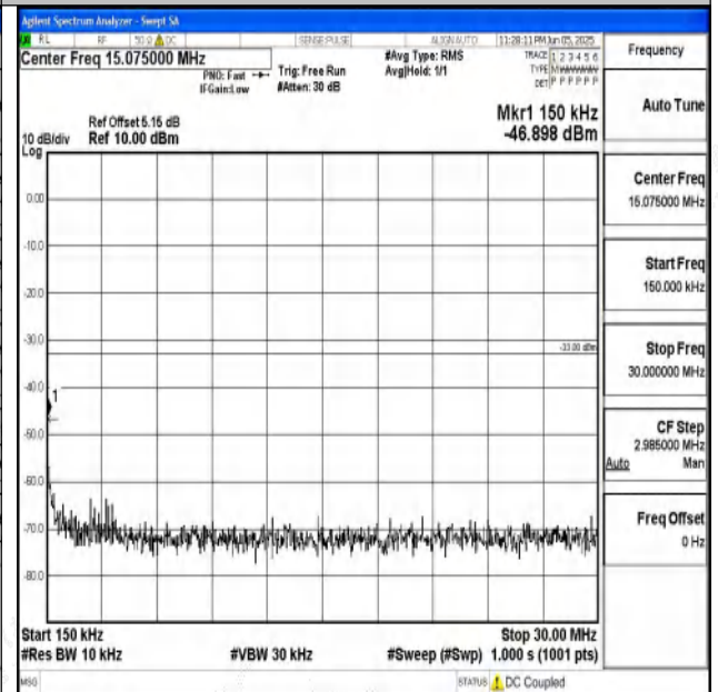
Band2_10MHz_QPSK_19150_1RB#0_0.15~30_0.15~30
