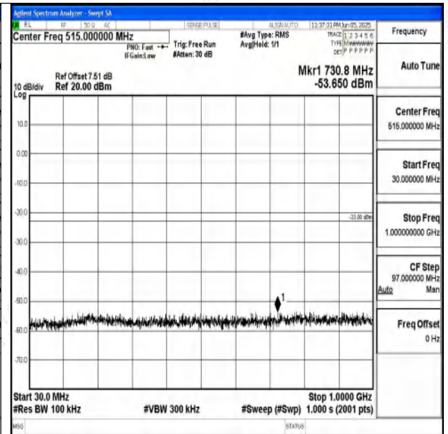
Band2_20MHz_16QAM_19100_1RB#0_30~1000_30~10 00
