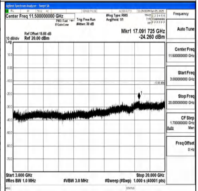
Band2_10MHz_16QAM_19150_1RB#0_3000~20000_30 00~20000
