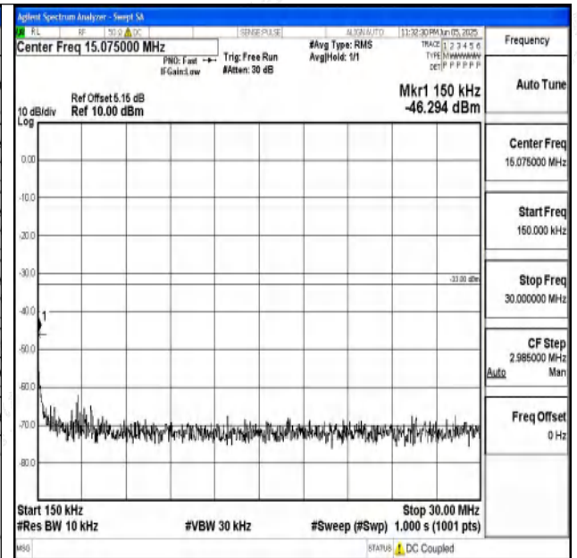
Band2_15MHz_QPSK_19125_1RB#0_0.15~30_0.15~30
