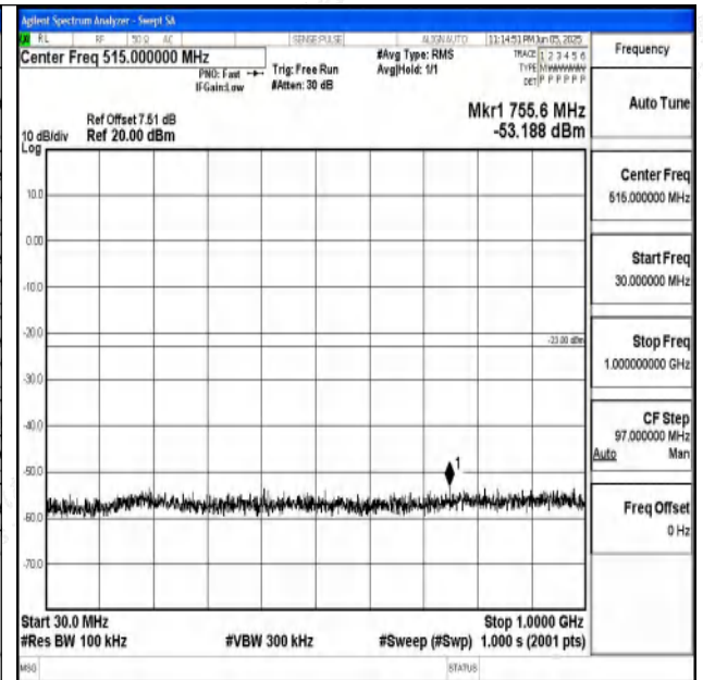
Band2_1.4MHz_16QAM_18900_1RB#0_30~1000_30~1 000
