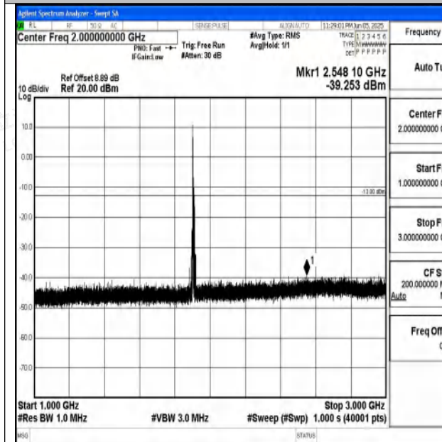
Band2_10MHz_16QAM_19150_1RB#0_1000~3000_10 00~3000
