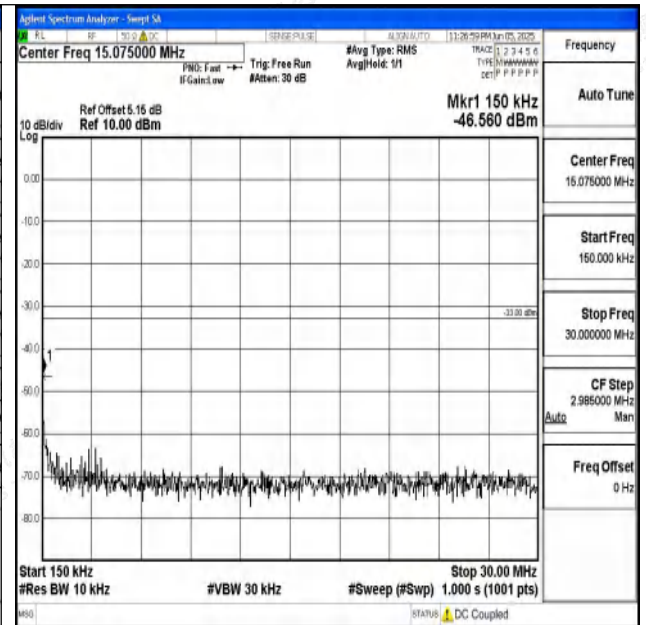
Band2_10MHz_QPSK_18900_1RB#0_0.15~30_0.15~30
