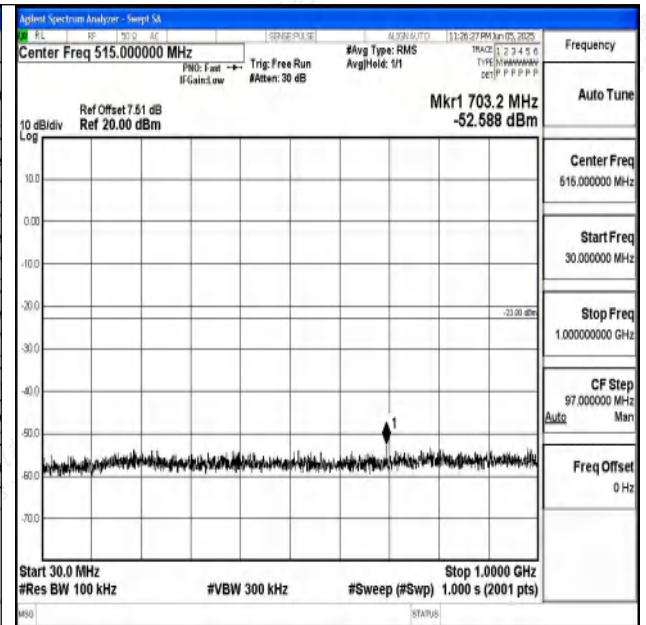
Band2_10MHz_16QAM_18650_1RB#0_30~1000_30~10
