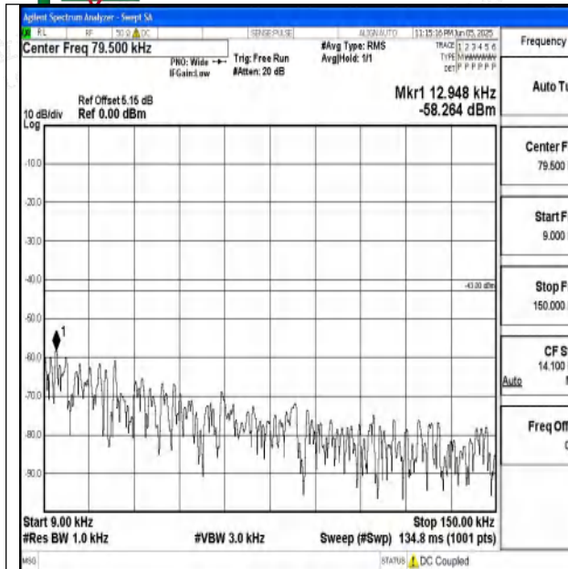
Band2_1.4MHz_QPSK_19193_1RB#0_0.009~0.15_0.09~0.15
