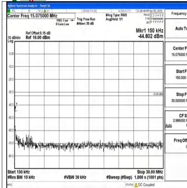
Band2_10MHz_16QAM_19150_1RB#0_0.15~30_0.15~30 30
