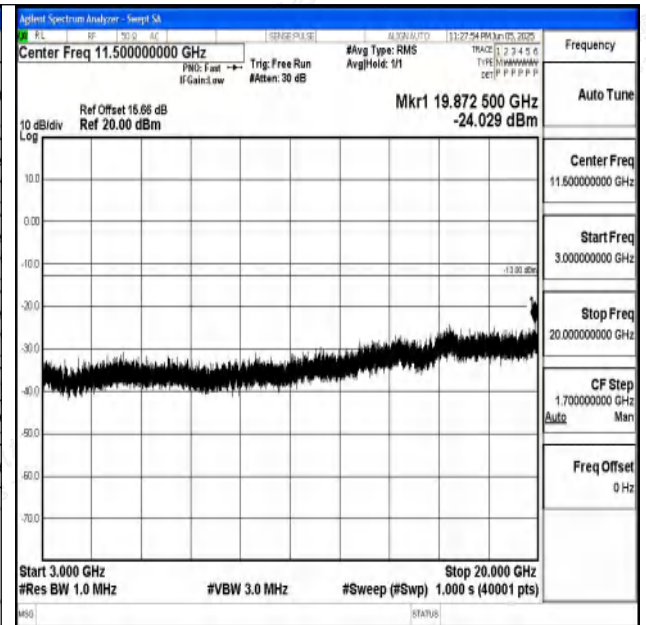
Band2_10MHz_16QAM_18900_1RB#0_3000~20000_30 00~20000
