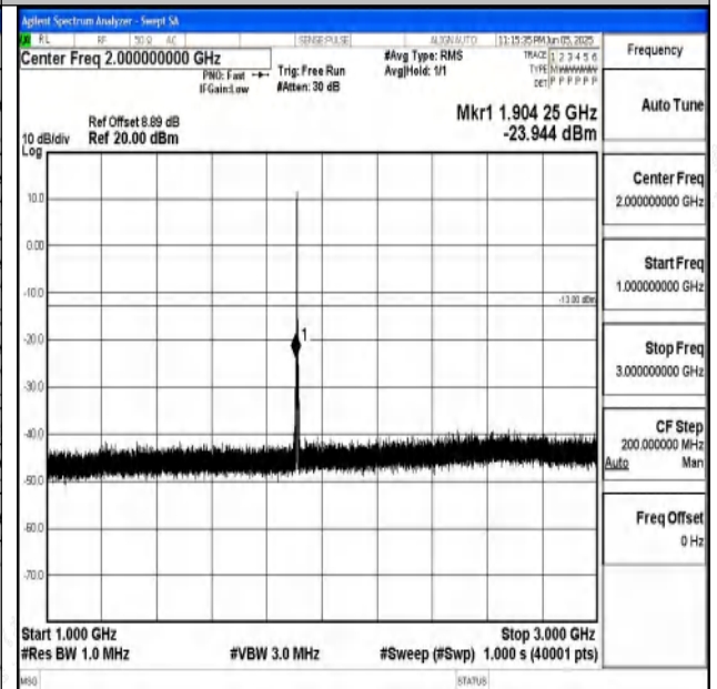
Band2_1.4MHz_QPSK_19193_1RB#0_1000~3000_1000~3000
