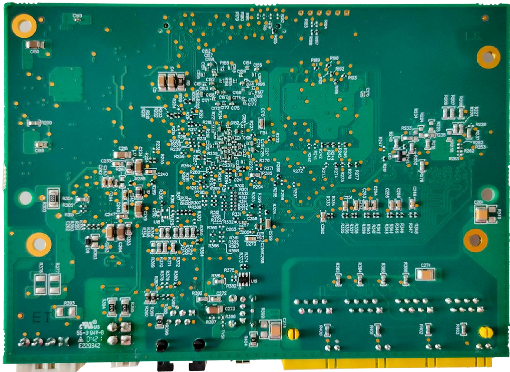
CUBE PLUS XA – Motherboard BOTTOM side
