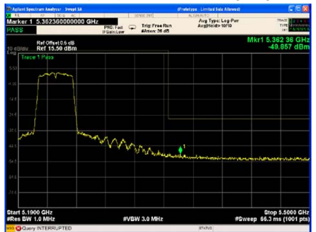
802.11(H40) U-NII-1 Band edge-right side
