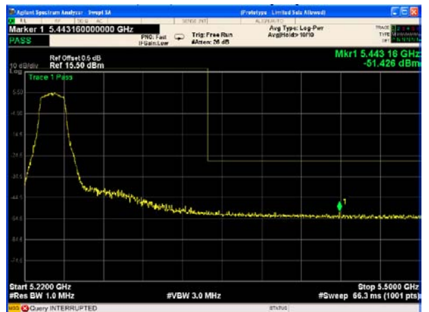
802.11(H20) U-NII-1 Band edge-right side
