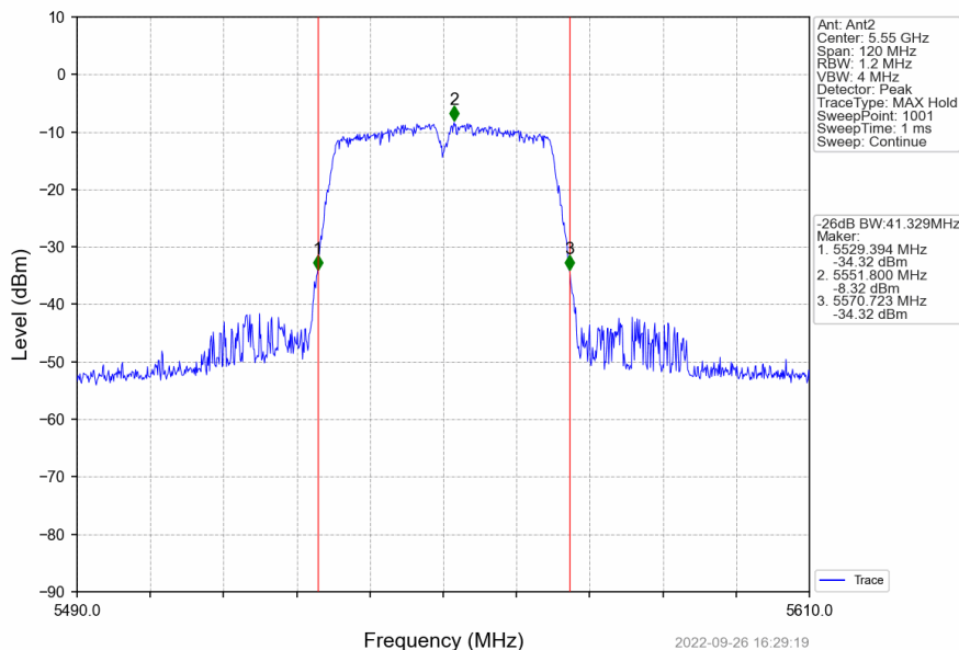
802.11n(HT40)_MCH_5550MHz_Ant2_NTNV
