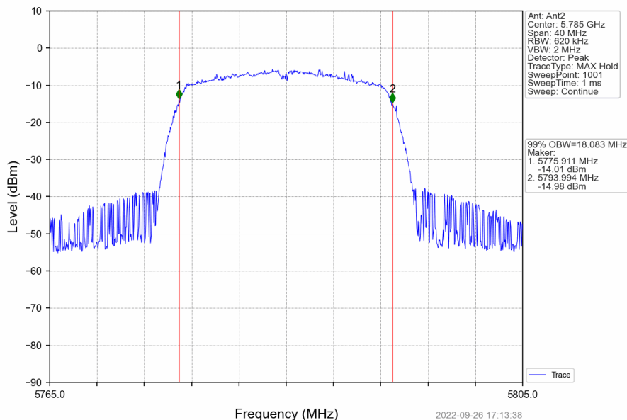
802.11n(HT20)_MCH_5785MHz_Ant2_NTNV
