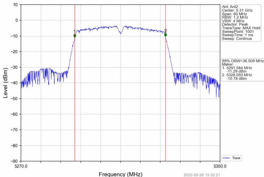
802.11n(HT40)_HCH_5310MHz_Ant2_NTNV
