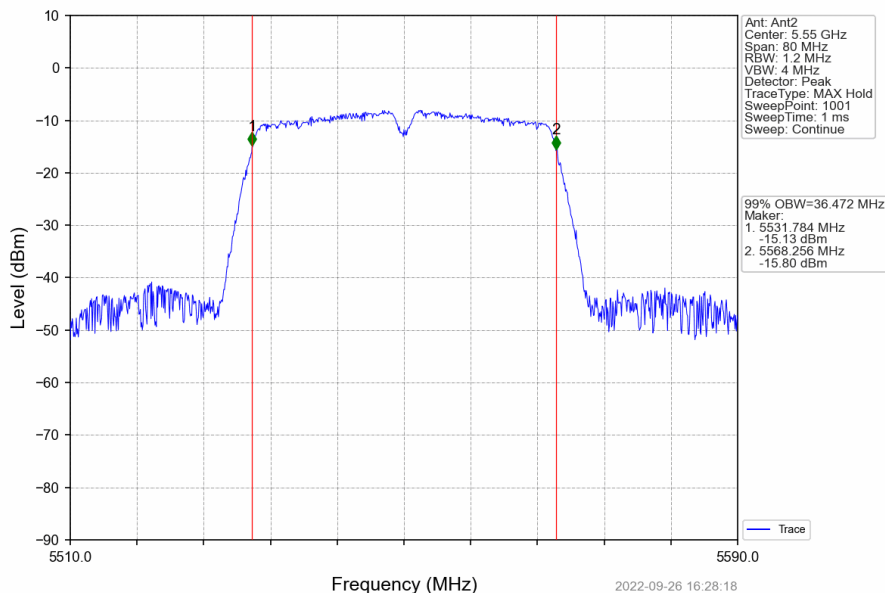
802.11n(HT40)_MCH_5550MHz_Ant2_NTNV
