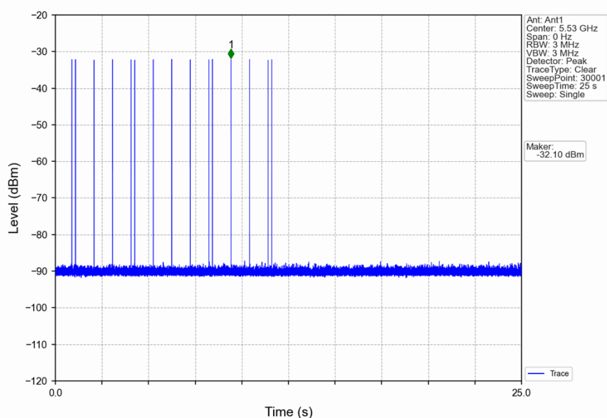
Signal Calibration_802.11ac(VHT80)_2C_5530MHz_RadarType0_Trial0
