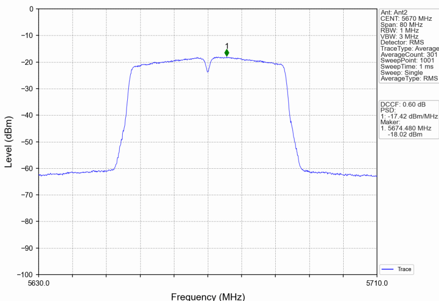
802.11ac(VHT40)_HCH_5670MHz_MIMO_NTNV
