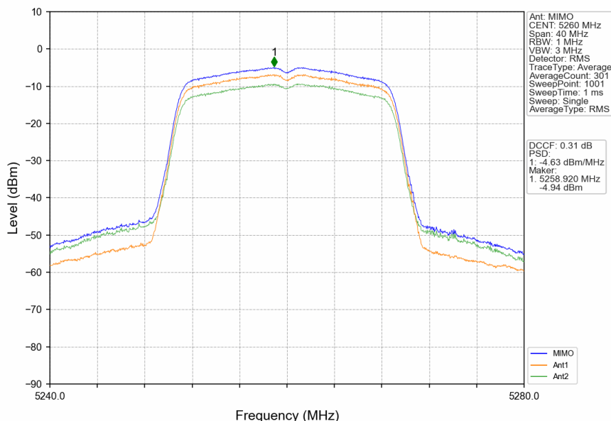
802.11ac(VHT20)_LCH_5260MHz_MIMO_NTNV
