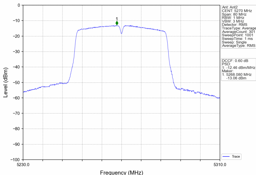
802.11ac(VHT40)_LCH_5270MHz_MIMO_NTNV
