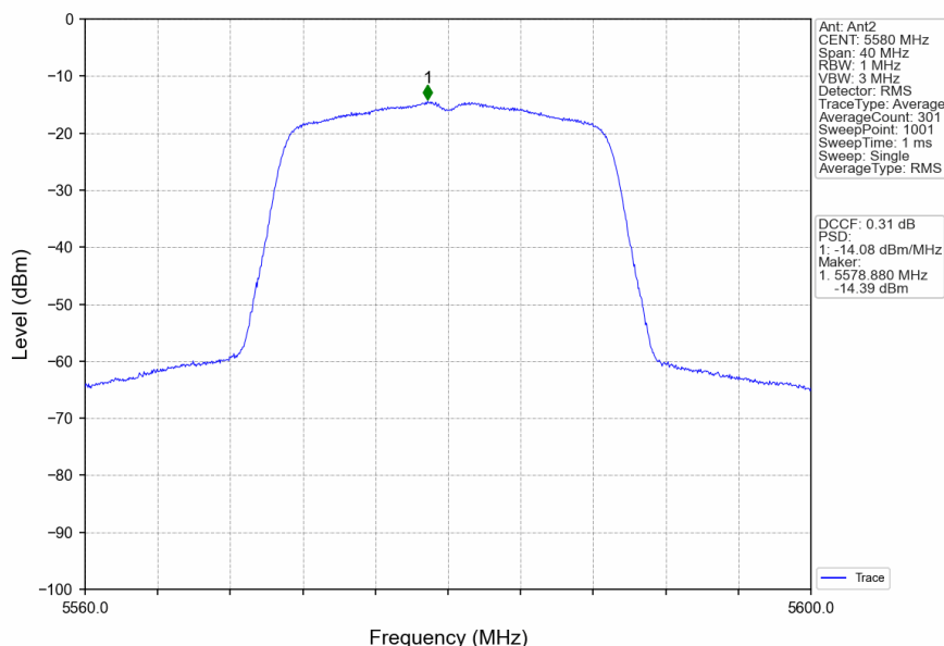
802.11ac(VHT20)_MCH_5580MHz_MIMO_NTNV
