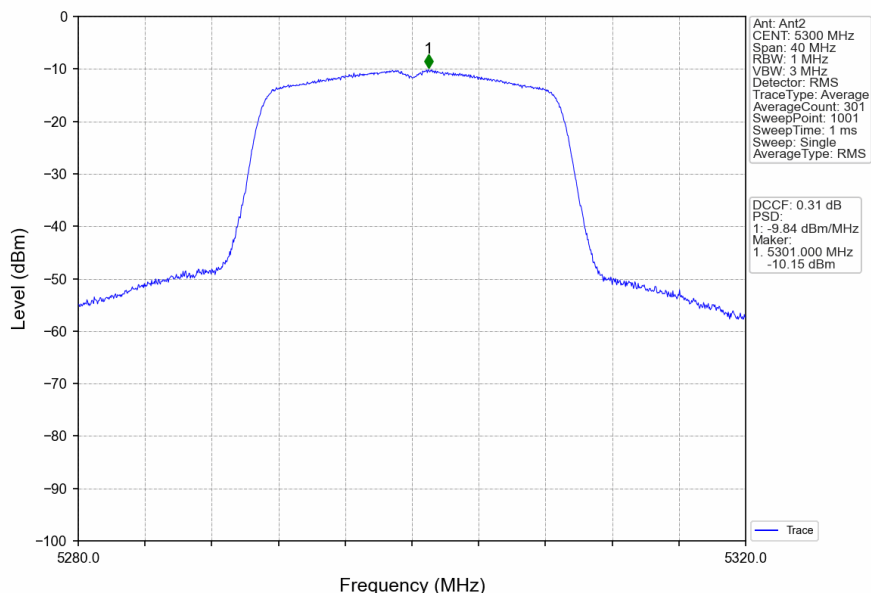
802.11ac(VHT20)_MCH_5300MHz_Ant2_NTNV
