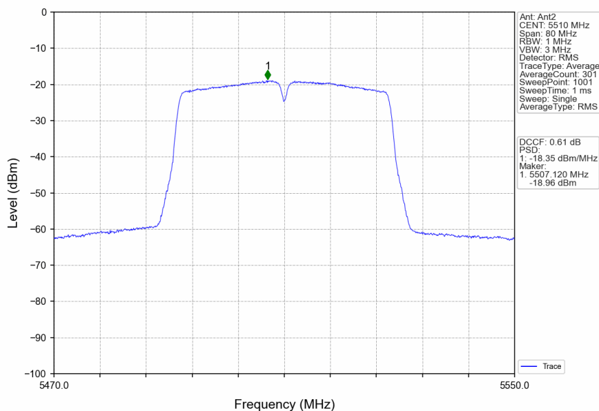
802.11ac(VHT40)_LCH_5510MHz_MIMO_NTNV
