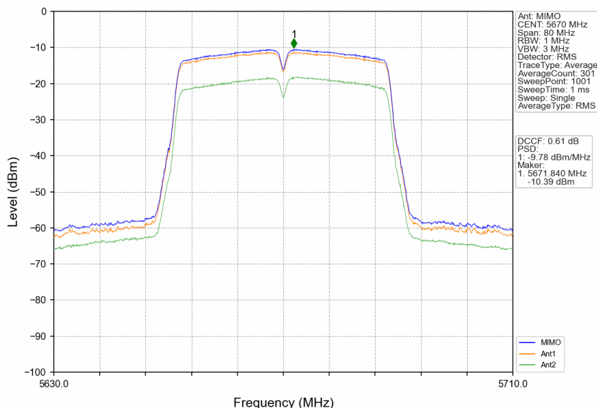
802.11n(HT40)_HCH_5670MHz_MIMO_NTNV
