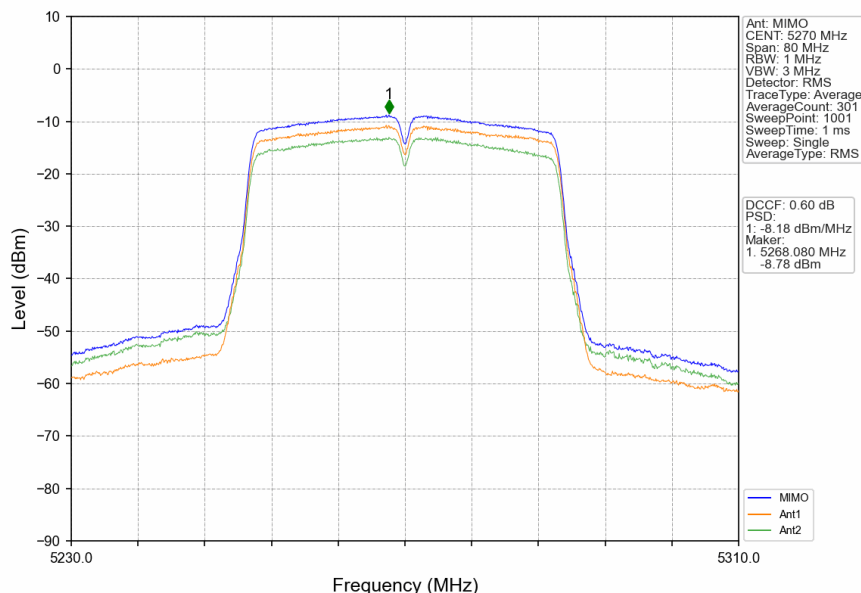
802.11ac(VHT40)_LCH_5270MHz_MIMO_NTNV
