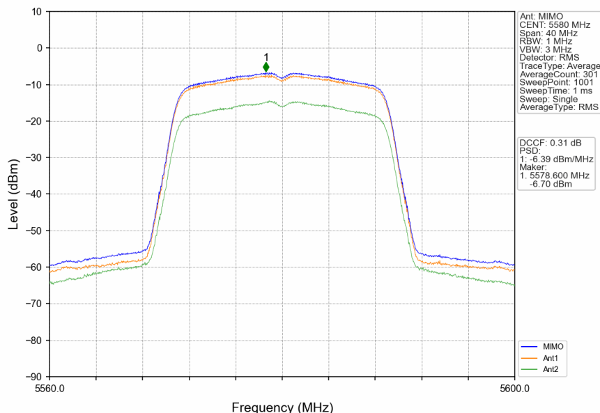
802.11ac(VHT20)_MCH_5580MHz_MIMO_NTNV
