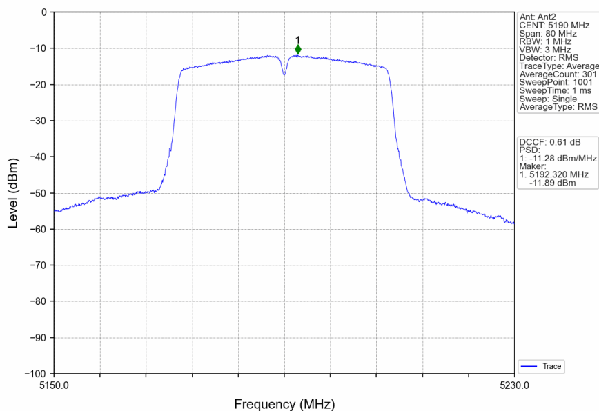
802.11ac(VHT40)_LCH_5190MHz_MIMO_NTNV
