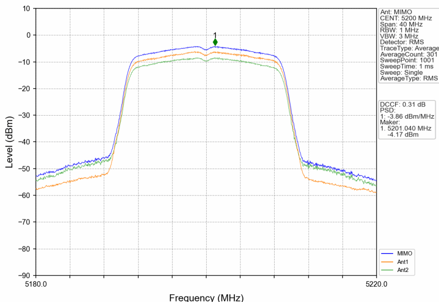
802.11ac(VHT20)_MCH_5200MHz_MIMO_NTNV
