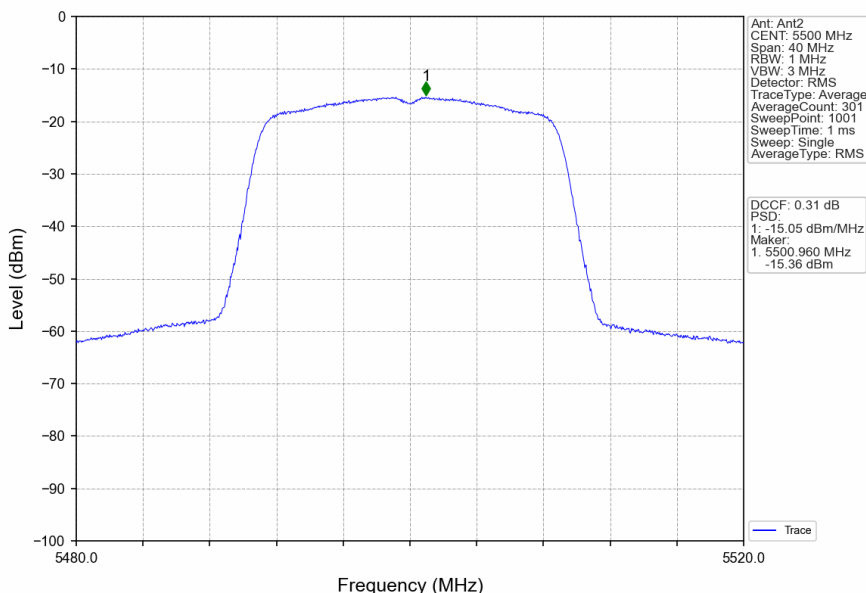
802.11ac(VHT20)_LCH_5500MHz_Ant2_NTNV
