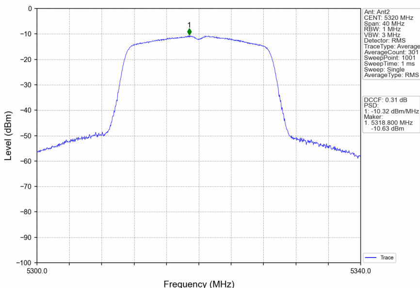
802.11ac(VHT20)_HCH_5320MHz_MIMO_NTNV
