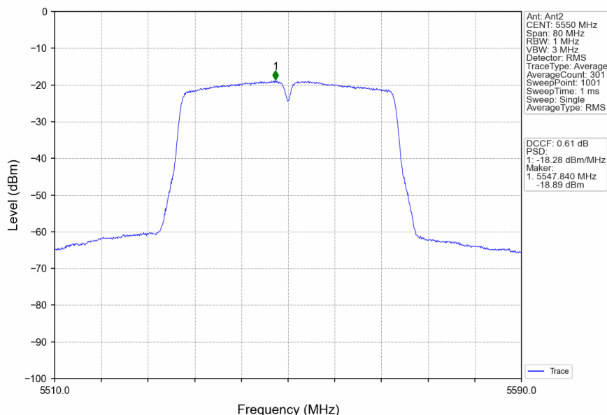
802.11ac(VHT40)_MCH_5550MHz_Ant2_NTNV
