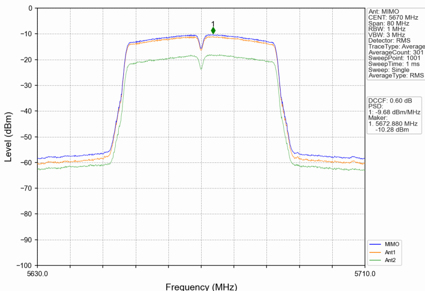
802.11ac(VHT40)_HCH_5670MHz_MIMO_NTNV
