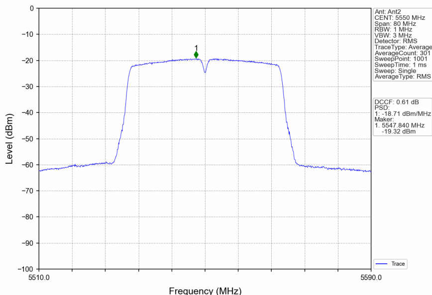
802.11n(HT40)_MCH_5550MHz_Ant2_NTNV
