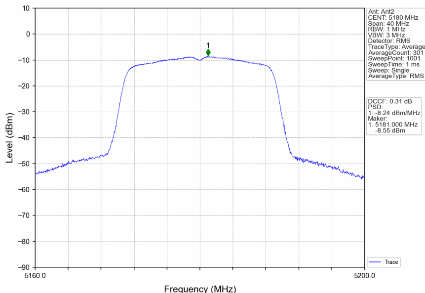
802.11ac(VHT20)_LCH_5180MHz_Ant2_NTNV
