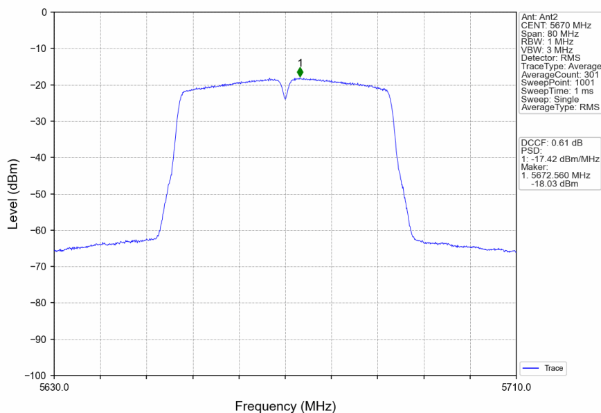
802.11n(HT40)_HCH_5670MHz_MIMO_NTNV
