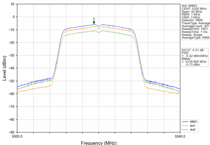
802.11ac(VHT20)_HCH_5320MHz_MIMO_NTNV
