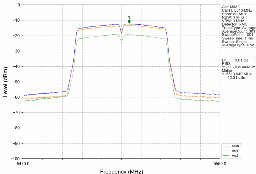
802.11ac(VHT40)_LCH_5510MHz_MIMO_NTNV
