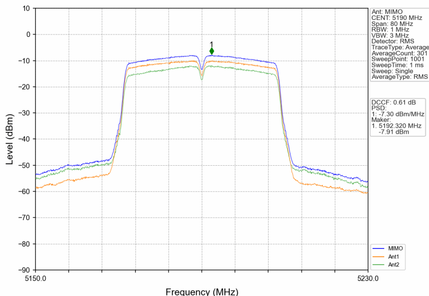
802.11ac(VHT40)_LCH_5190MHz_MIMO_NTNV
