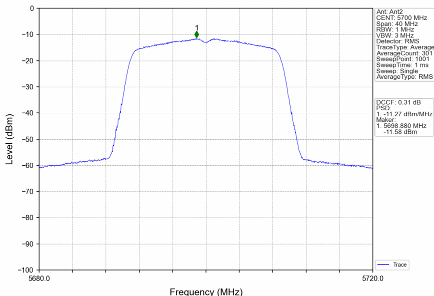
802.11ac(VHT20)_HCH_5700MHz_Ant2_NTNV
