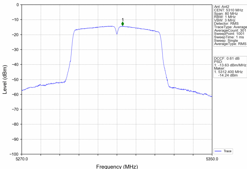
802.11ac(VHT40)_HCH_5310MHz_Ant2_NTNV
