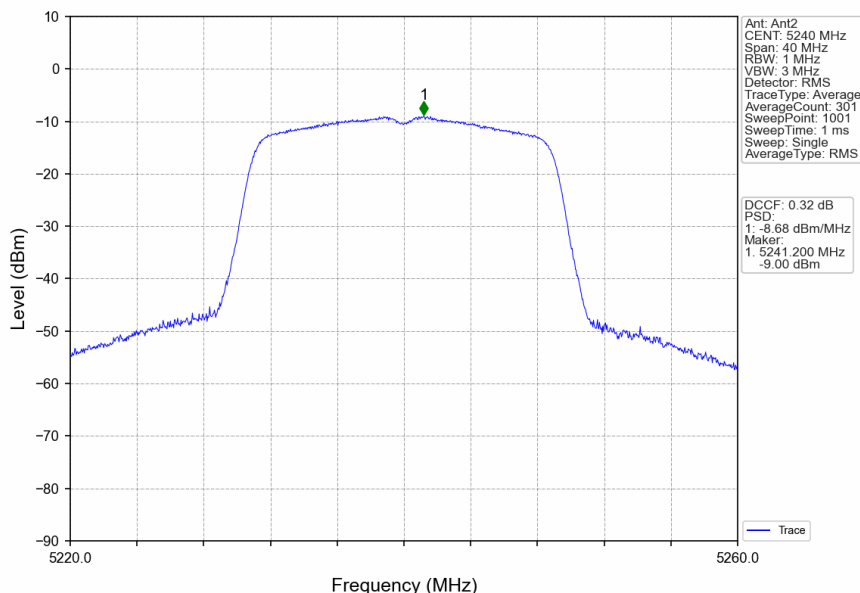
802.11n(HT20)_HCH_5240MHz_Ant2_NTNV
