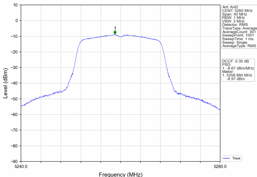
802.11a_LCH_5260MHz_Ant2_NTNV
