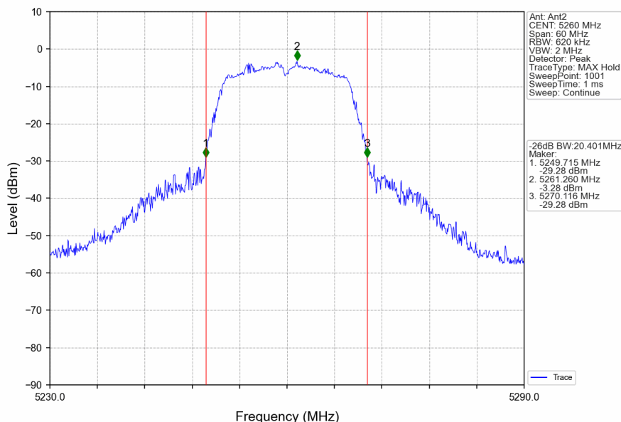
802.11a_LCH_5260MHz_Ant2_NTNV
