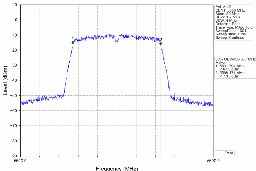
802.11ac(VHT40)_MCH_5550MHz_Ant2_NTNV
