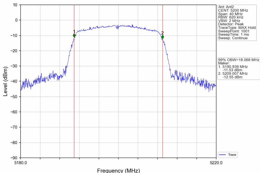
802.11ac(VHT20)_MCH_5200MHz_Ant2_NTNV
