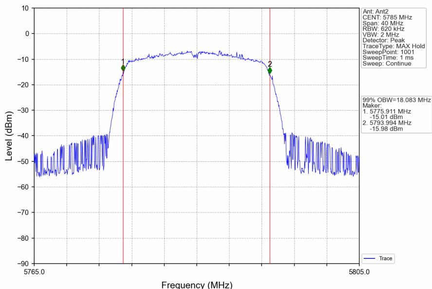
802.11n(HT20)_MCH_5785MHz_Ant2_NTNV
