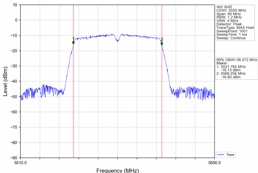
802.11n(HT40)_MCH_5550MHz_Ant2_NTNV
