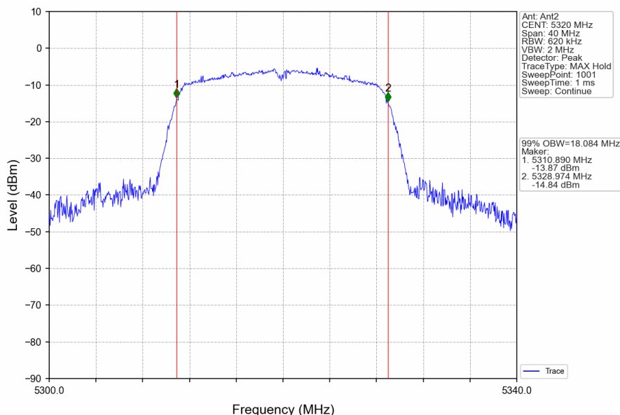
802.11ac(VHT20)_HCH_5320MHz_Ant2_NTNV
