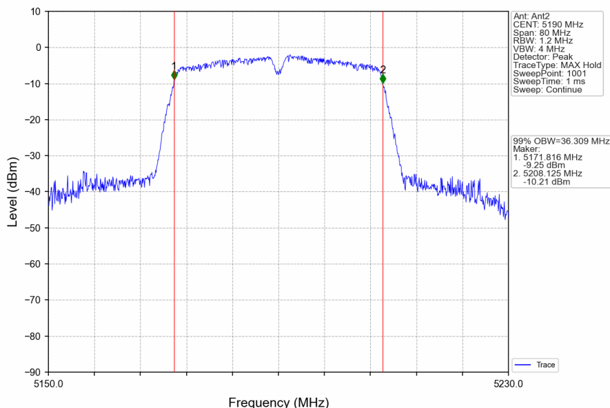
802.11ac(VHT40)_LCH_5190MHz_Ant2_NTNV
