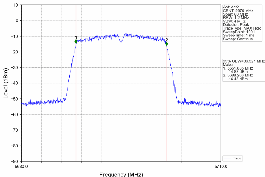
802.11ac(VHT40)_HCH_5670MHz_Ant2_NTNV
