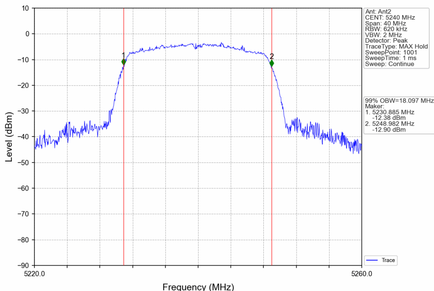
802.11ac(VHT20)_HCH_5240MHz_Ant2_NTNV
