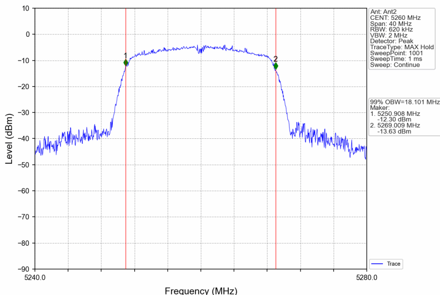
802.11ac(VHT20)_LCH_5260MHz_Ant2_NTNV
