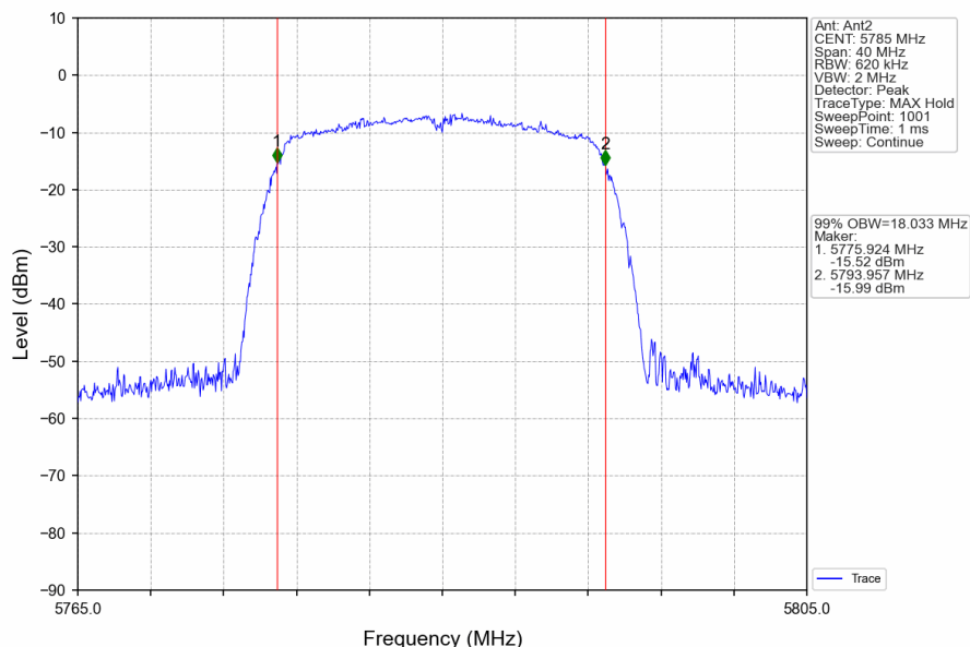
802.11ac(VHT20)_MCH_5785MHz_Ant2_NTNV
