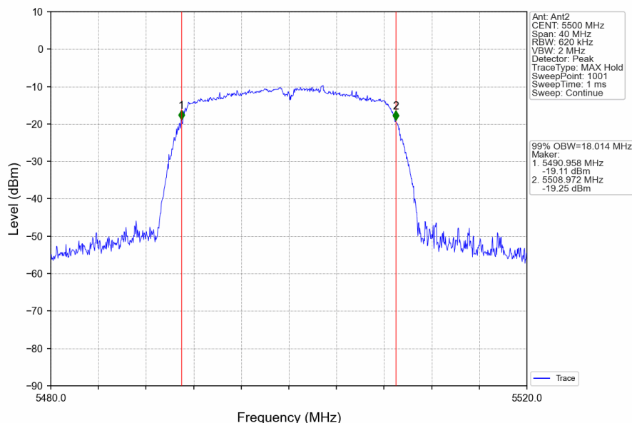
802.11ac(VHT20)_LCH_5500MHz_Ant2_NTNV
