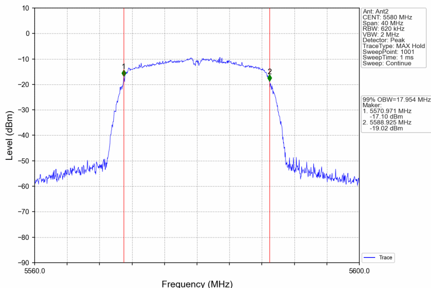
802.11ac(VHT20)_MCH_5580MHz_Ant2_NTNV
