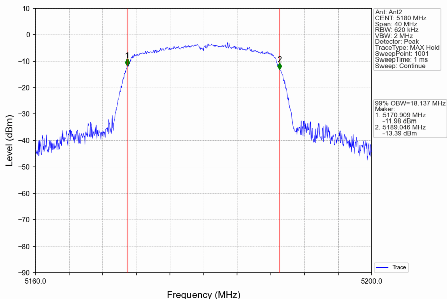
802.11ac(VHT20)_LCH_5180MHz_Ant2_NTNV
