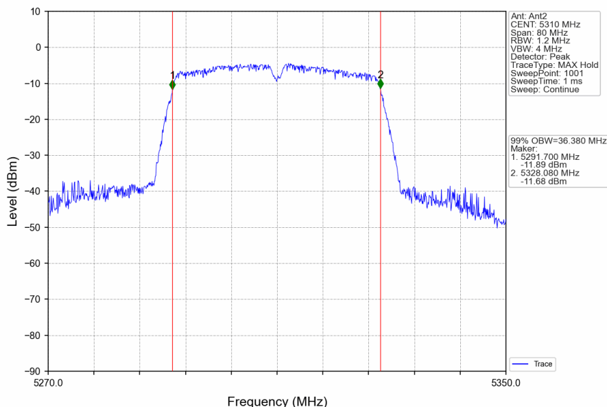
802.11ac(VHT40)_HCH_5310MHz_Ant2_NTNV
