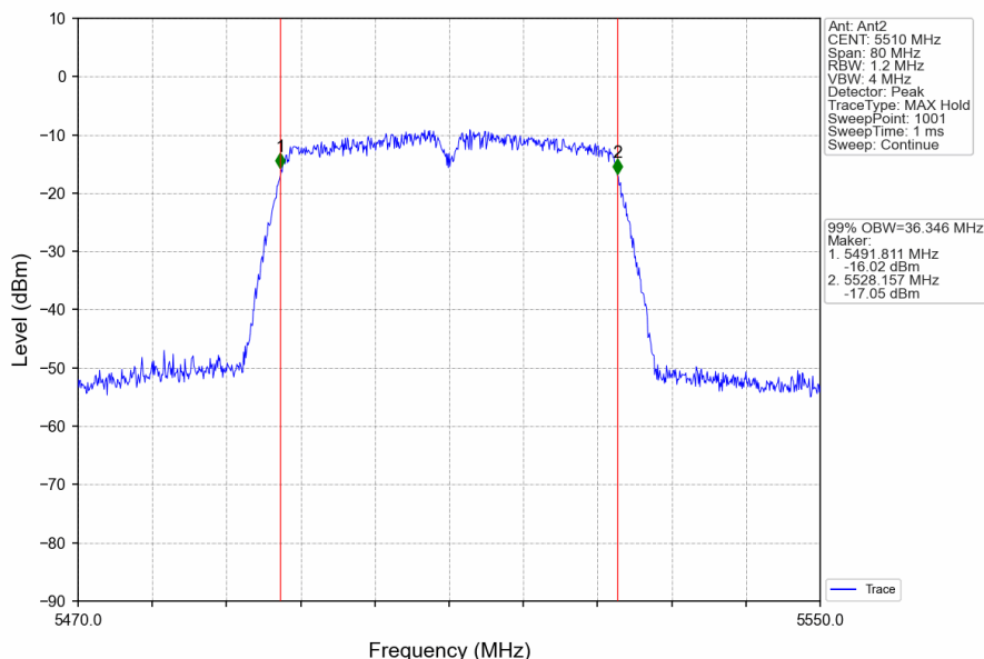
802.11ac(VHT40)_LCH_5510MHz_Ant2_NTNV
