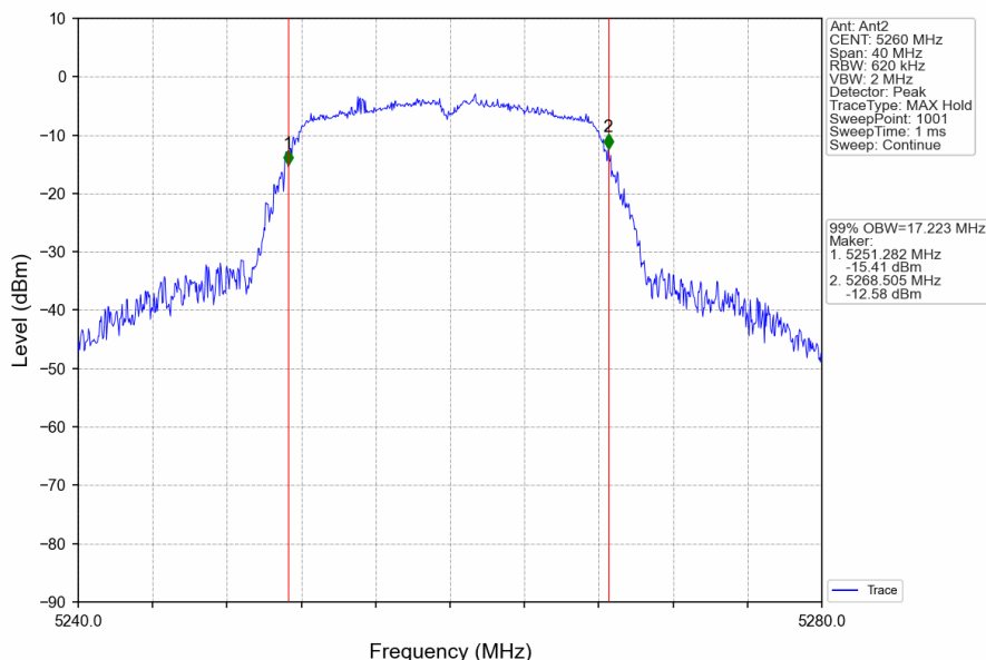
802.11a_LCH_5260MHz_Ant2_NTNV
