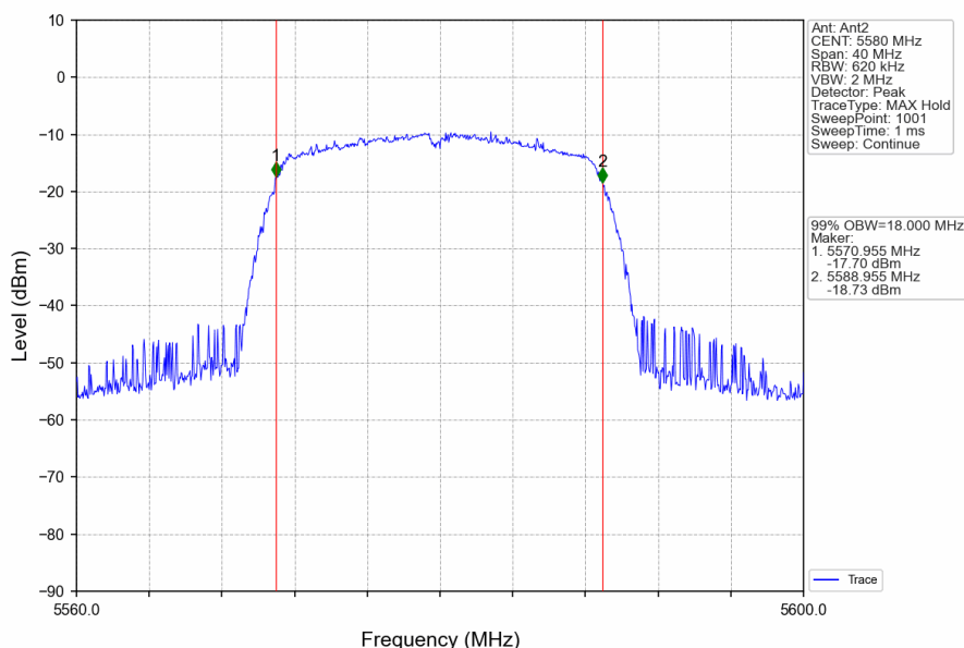
802.11n(HT20)_MCH_5580MHz_Ant2_NTNV
