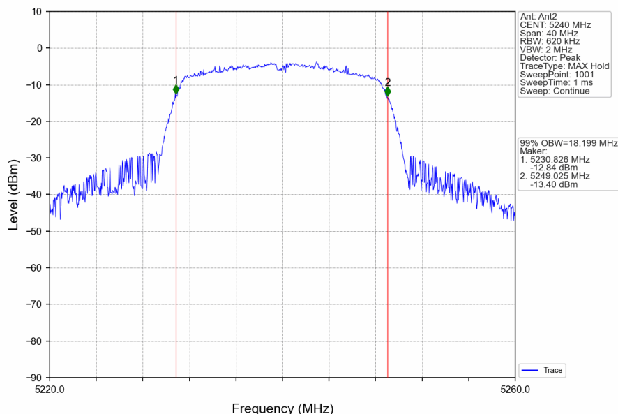
802.11n(HT20)_HCH_5240MHz_Ant2_NTNV
