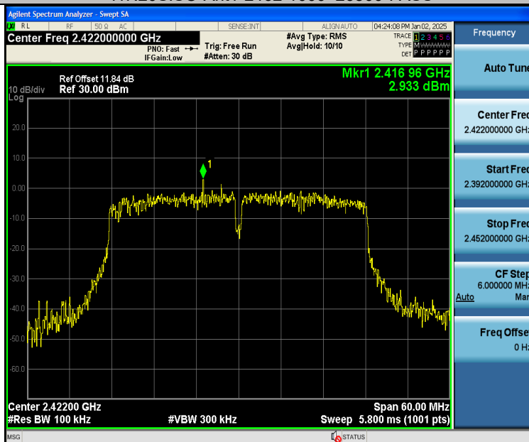
11N40SISO-Ant1-2422-0~Reference-PASS
