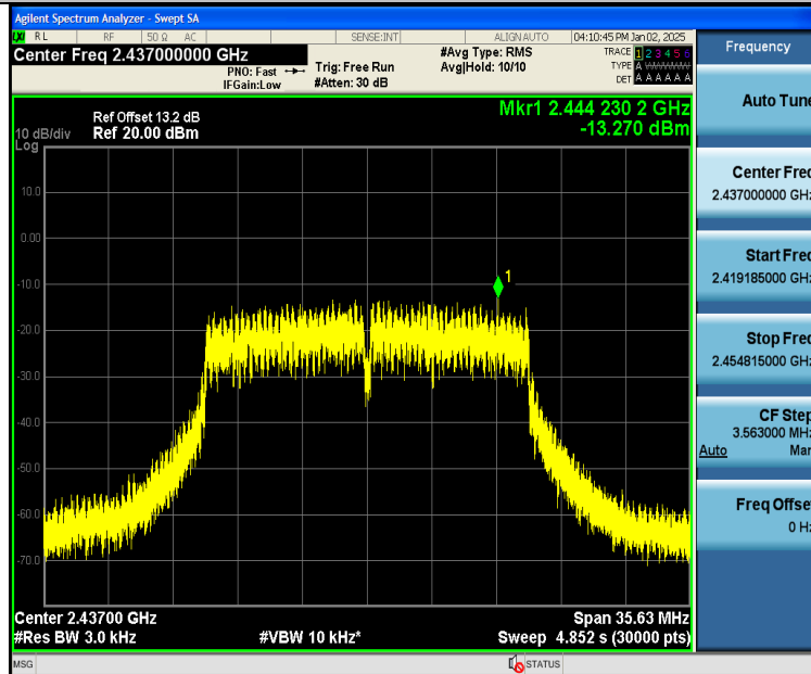
11N20SISO-Ant1-2437-PASS
