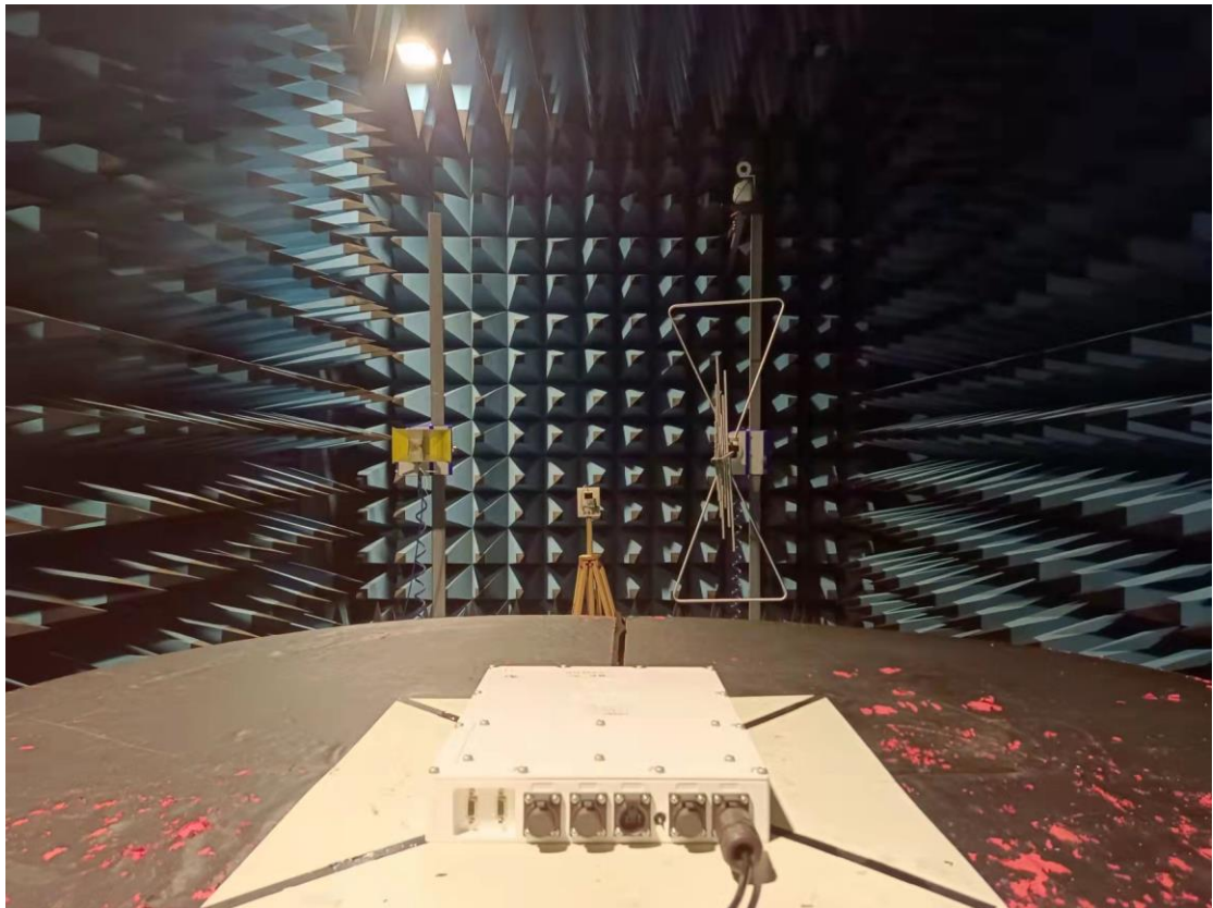
FCC Part15C Radiated Emission above 18-26GHz
