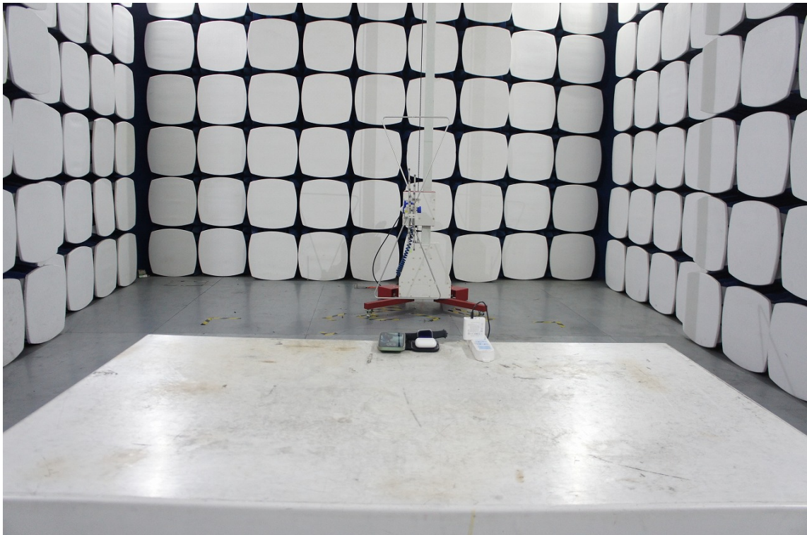
30MHz-1GHz
