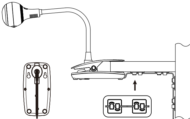
Cord management under the base
