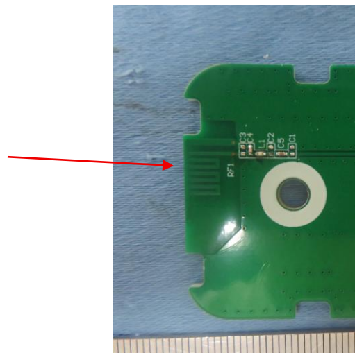
Antenna design:
