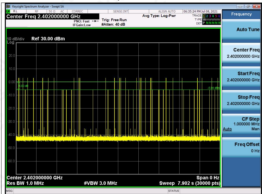
Test Graph BR HOP ANT1 NA 1Mbps 2402 Number of Burst
