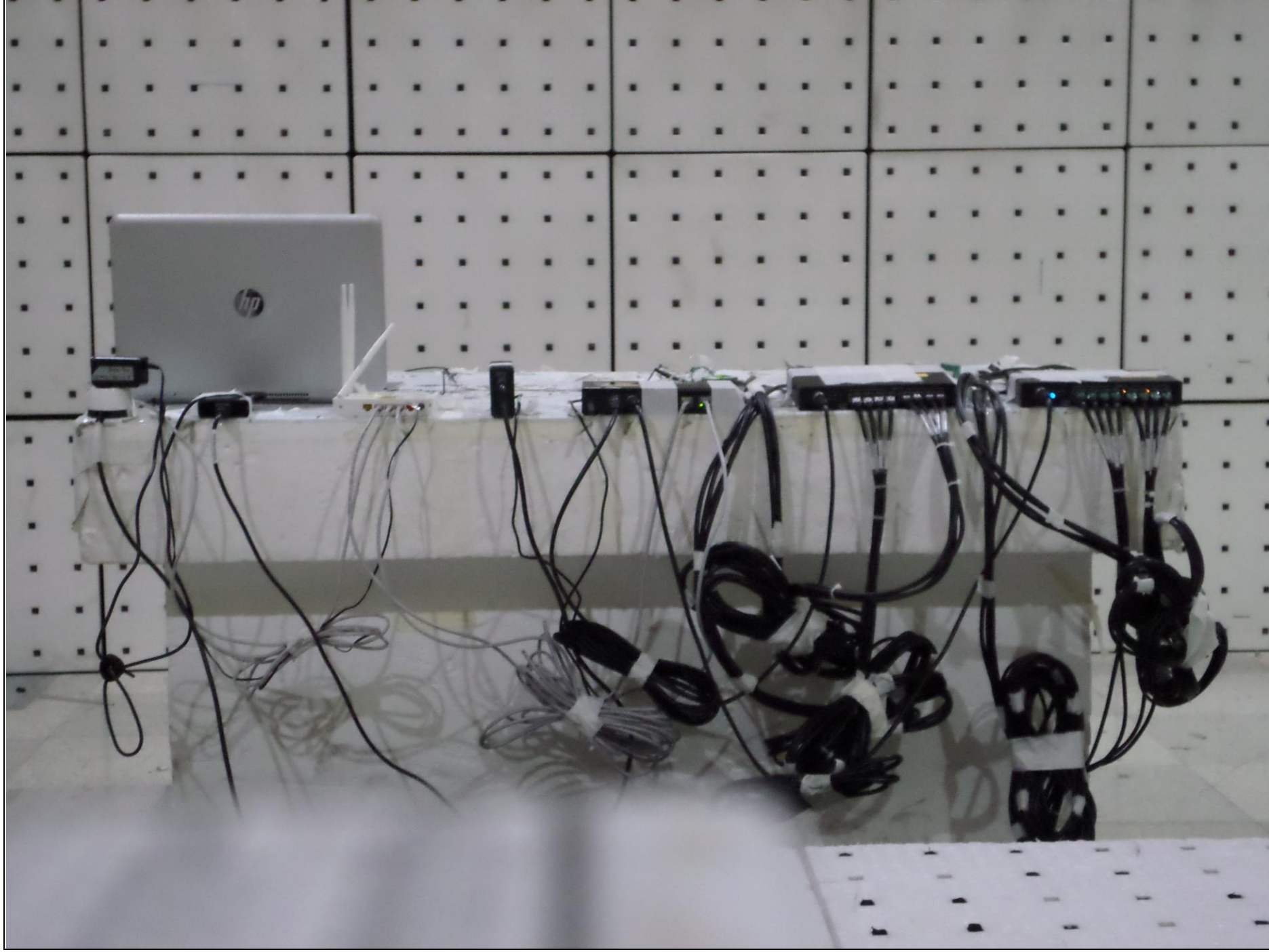
Radiated Emission (18 GHz – 30 GHz) _ Rear
