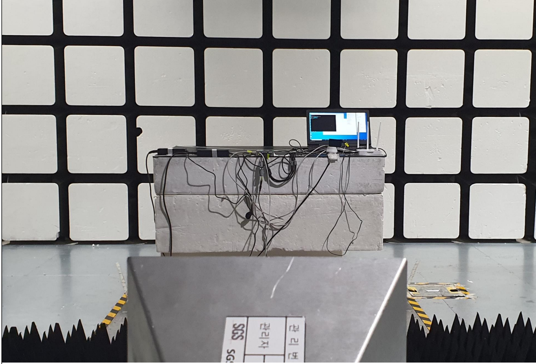
RE(Above 1 GHz_Rear
