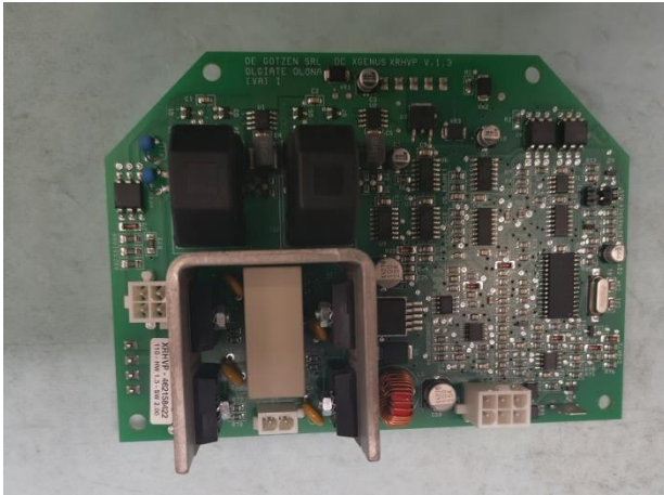
XRHVP board TOP
