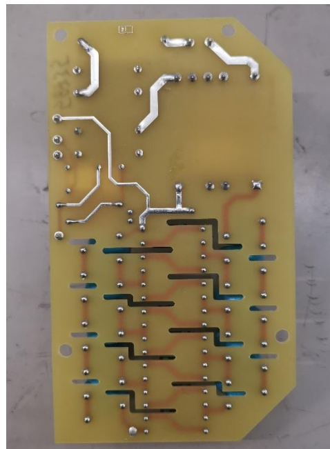
XRHVM board BOTTOM
