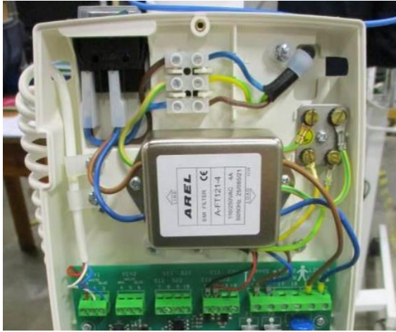
EMI filter
