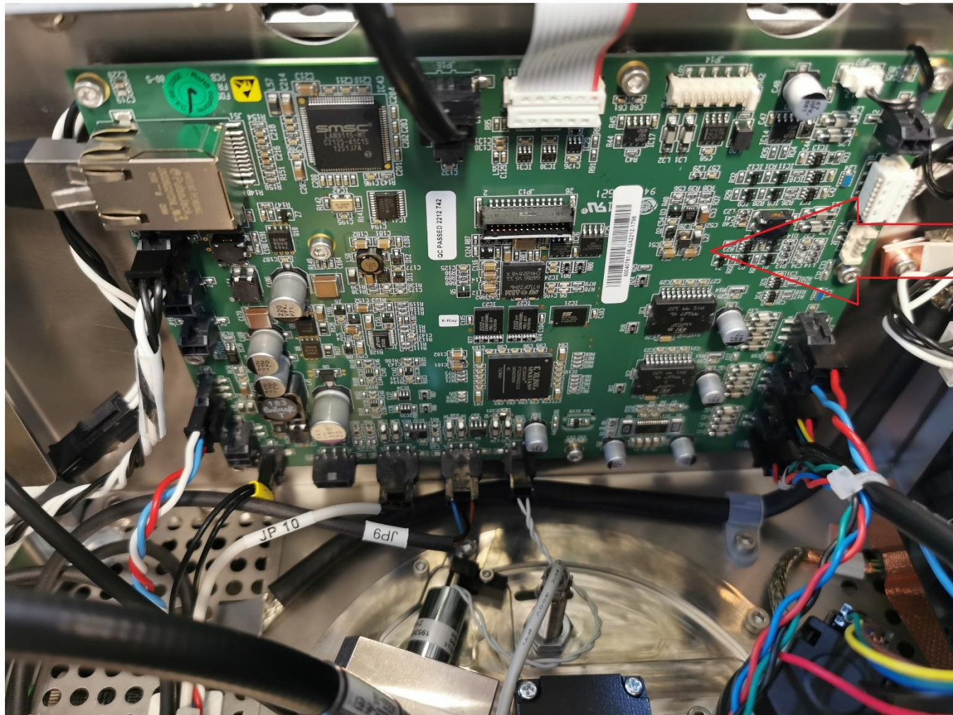
FR Control PCB 60040781
