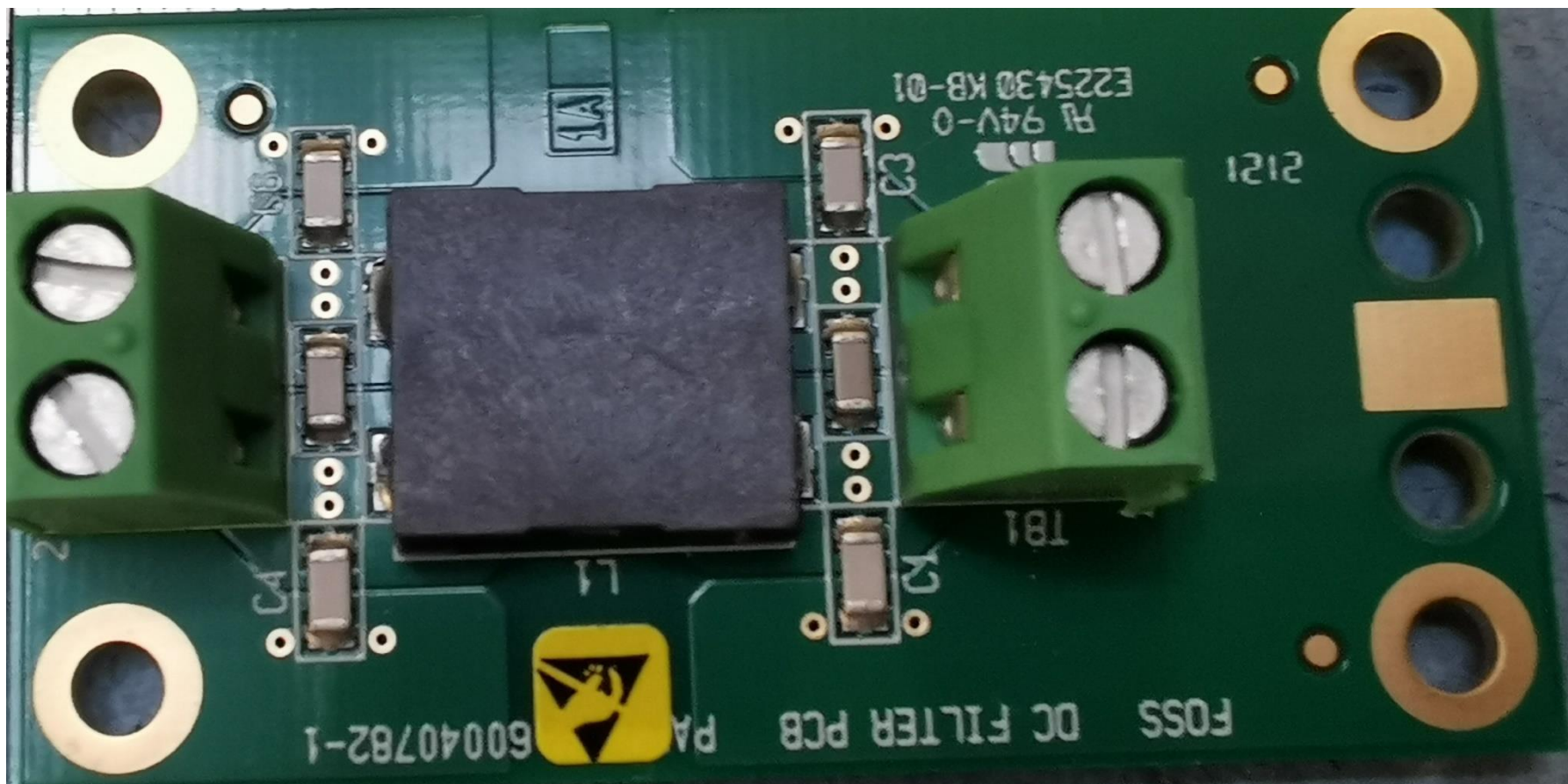
DC Filter PCB 60040783
