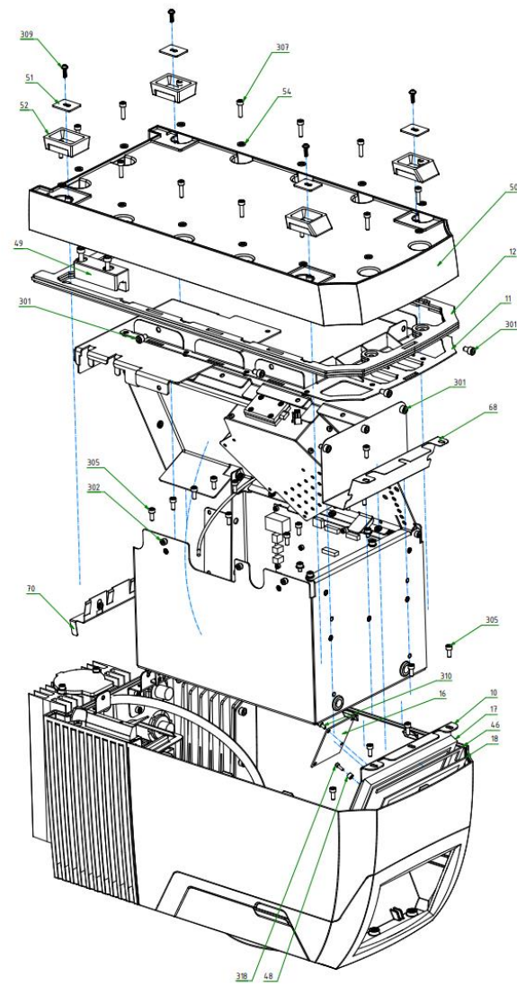
Basic unit FOSS NIRS DA1650
