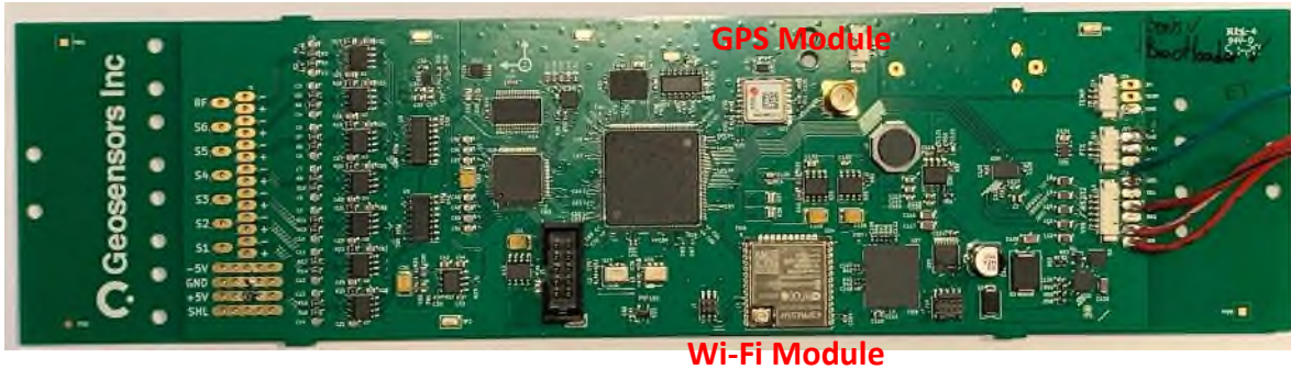
Figure 1 – EUT Internal Photo Front
