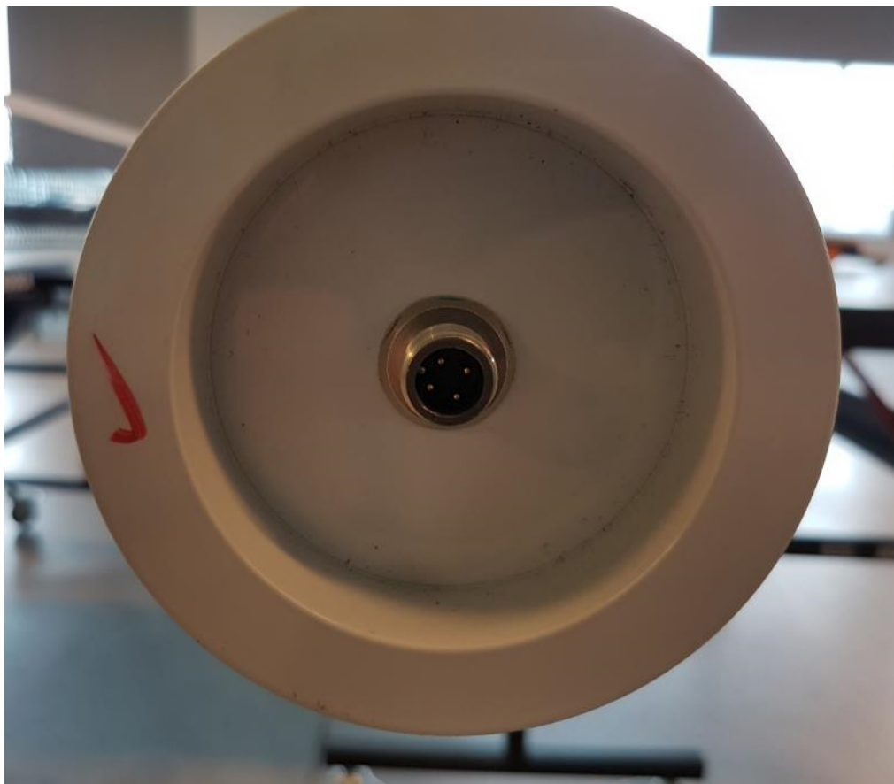
Figure 2 – EUT External Photo (Connector)
