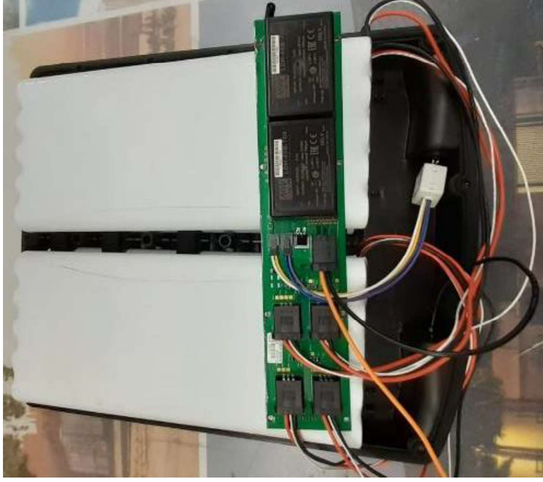
4 battery pack connected to the V4 electronic card
