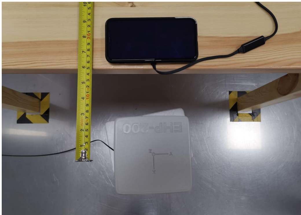
Test setup of B side
