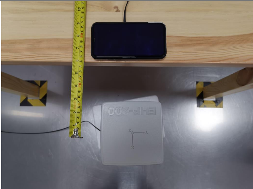
Test setup of A side
