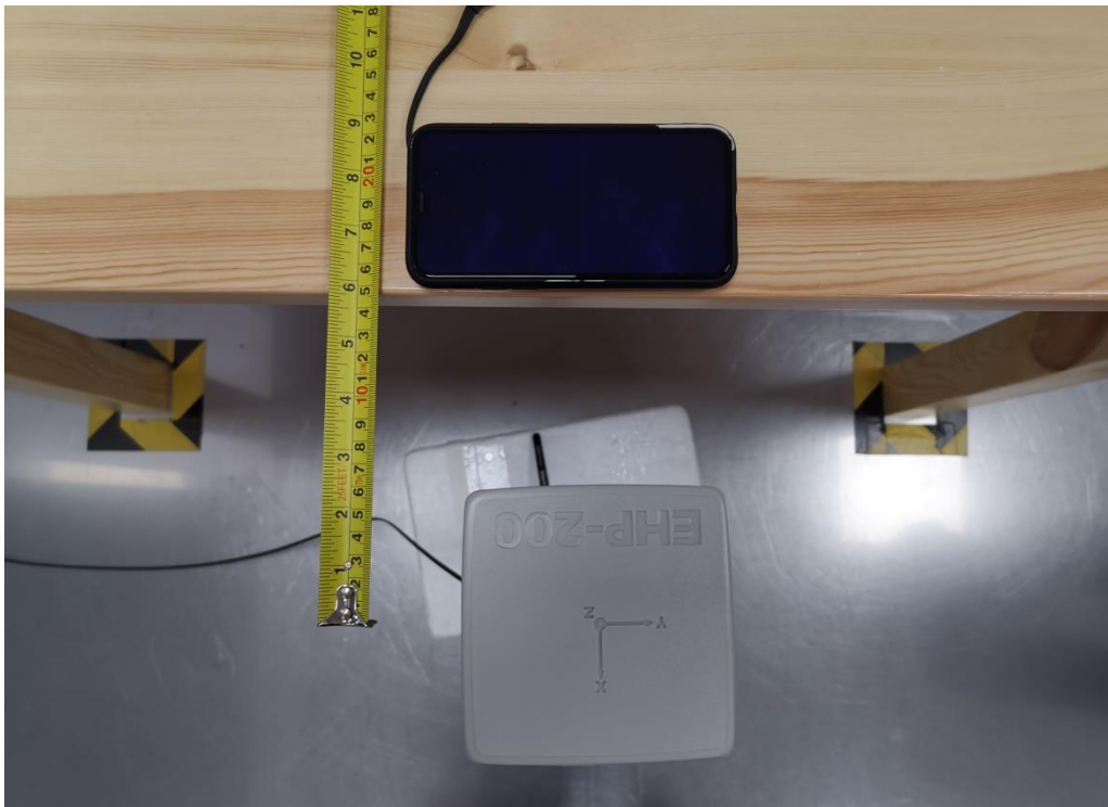
Test setup of C side
