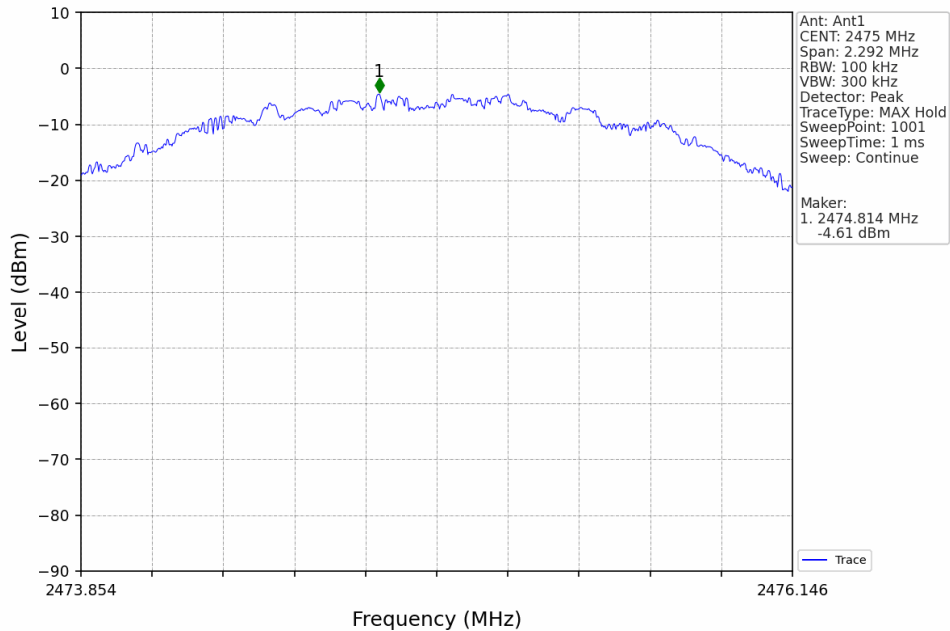
Zigbee_HCH_2475MHz_Ant1_NTNV
