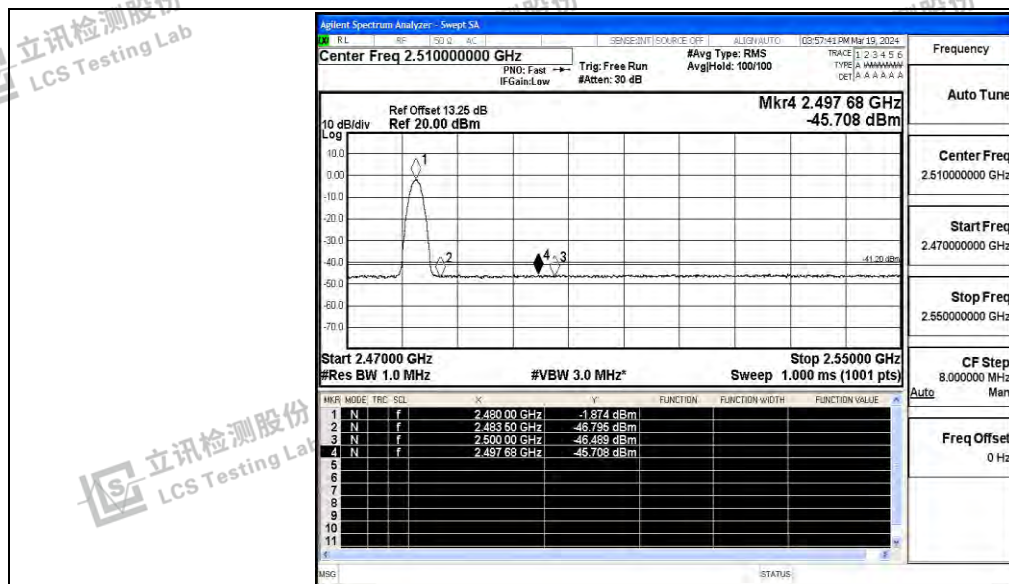
3DH5_Ant_High_2480_Peak
