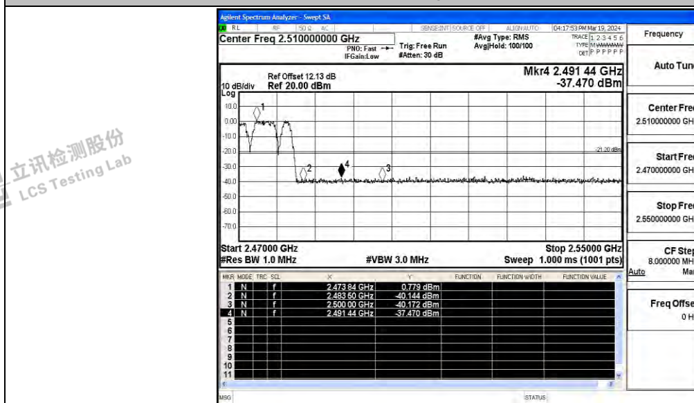
3DH5_Ant_High_Hop_2480_Peak
