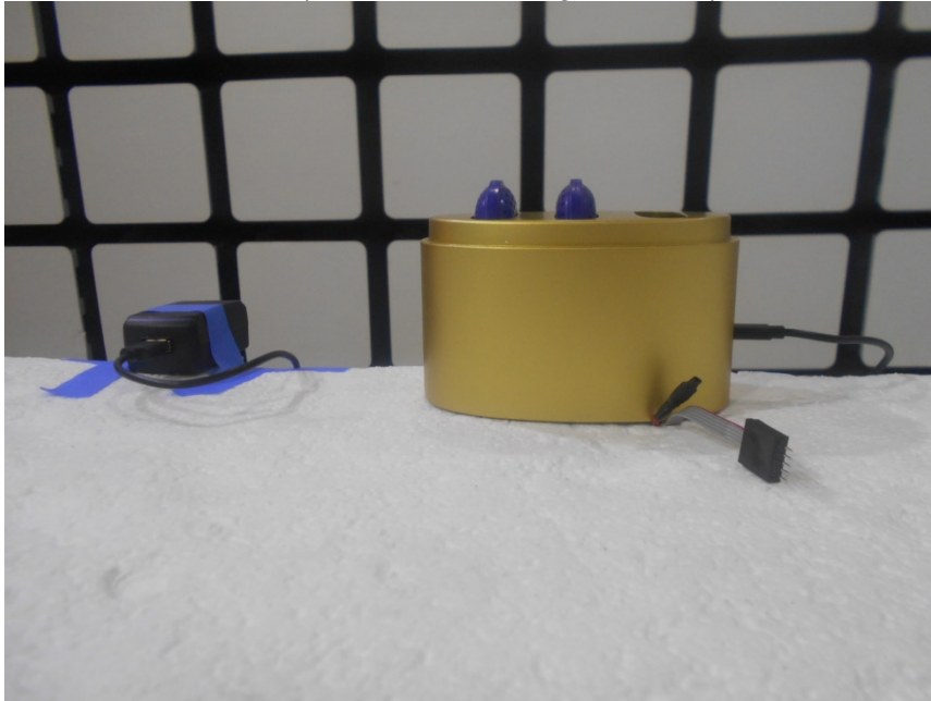
RADIATED PHOTO (<30MHz, With Tags, RFID 2)
