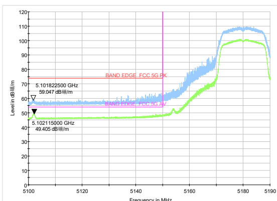
802.11n HT20 -Channel 36: Peak+ Average
