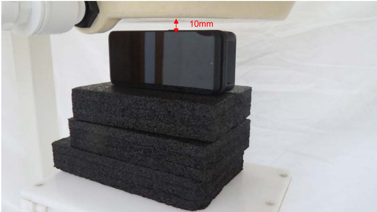
Picture 5: Left Edge, the distance from handset to the bottom of the Phantom is 10mm
