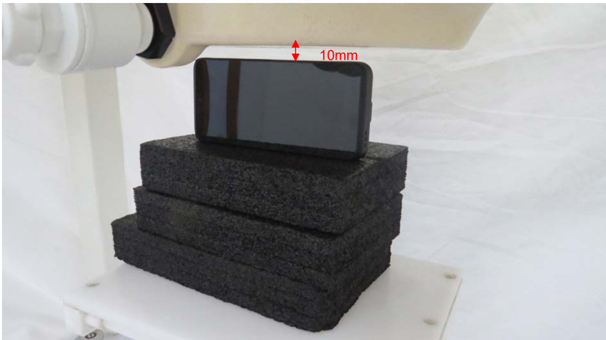
Picture 6: Right Edge, the distance from handset to the bottom of the Phantom is 10mm
