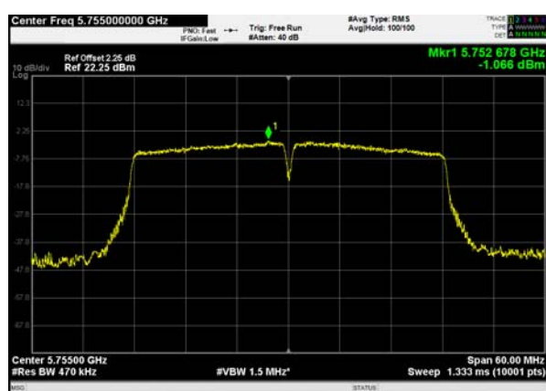
U-NII-3, 802.11n HT40, Channel No.: 151
