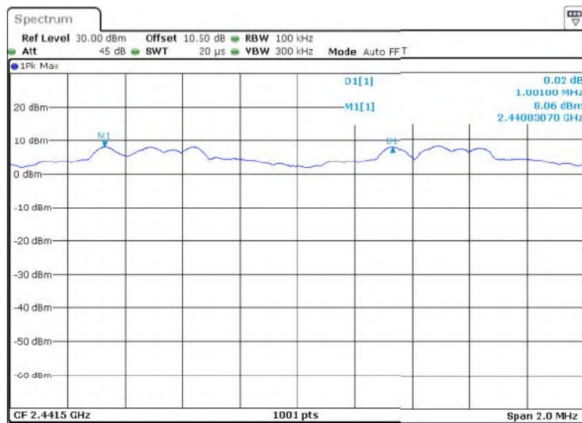
Test Mode: 8DPSK ---Middle
