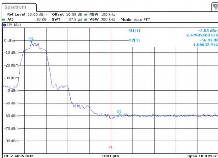
For 8DPSK Non-Hopping Mode (High)
