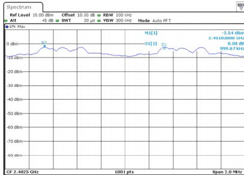
Test Mode: 8DPSK---Low
