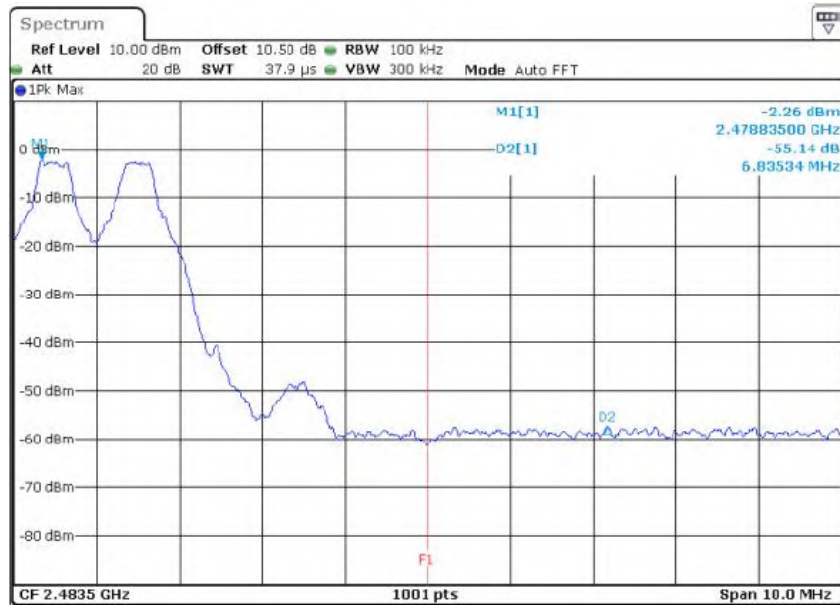
For GFSK Hopping Mode (High)
