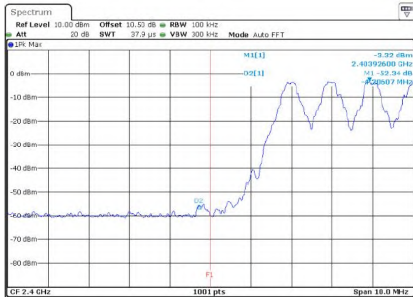
For GFSK Hopping Mode (Low)
