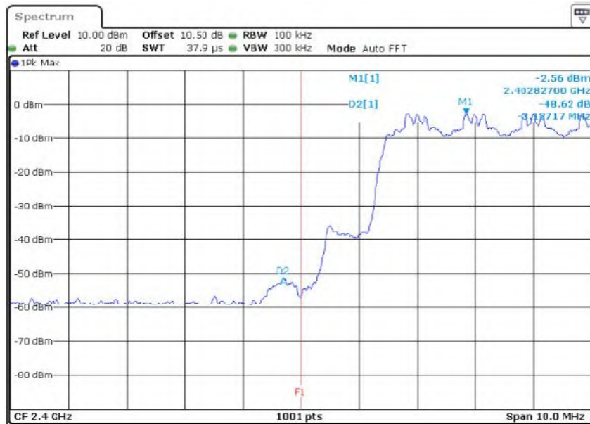
For 8DPSK Hopping Mode (Low)
