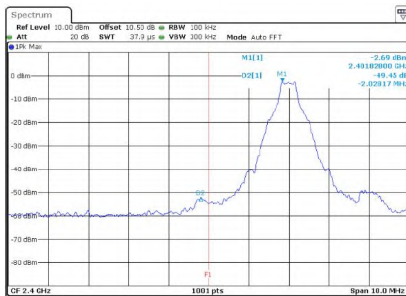
For GFSK Non-Hopping Mode (Low)
