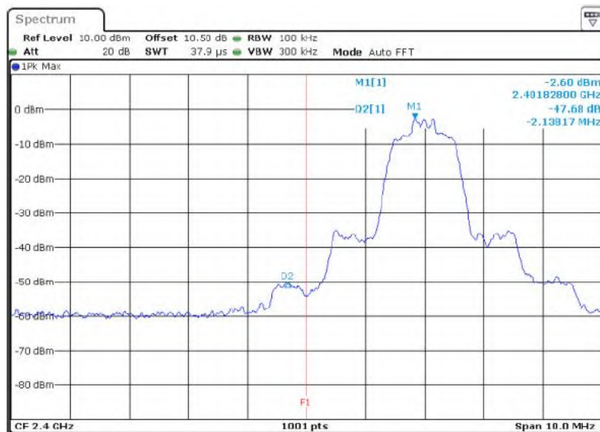
For 8DPSK NonHopping Mode (Low)
