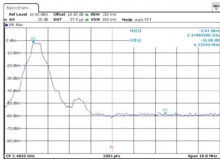
For GFSK Non-Hopping Mode (High)
