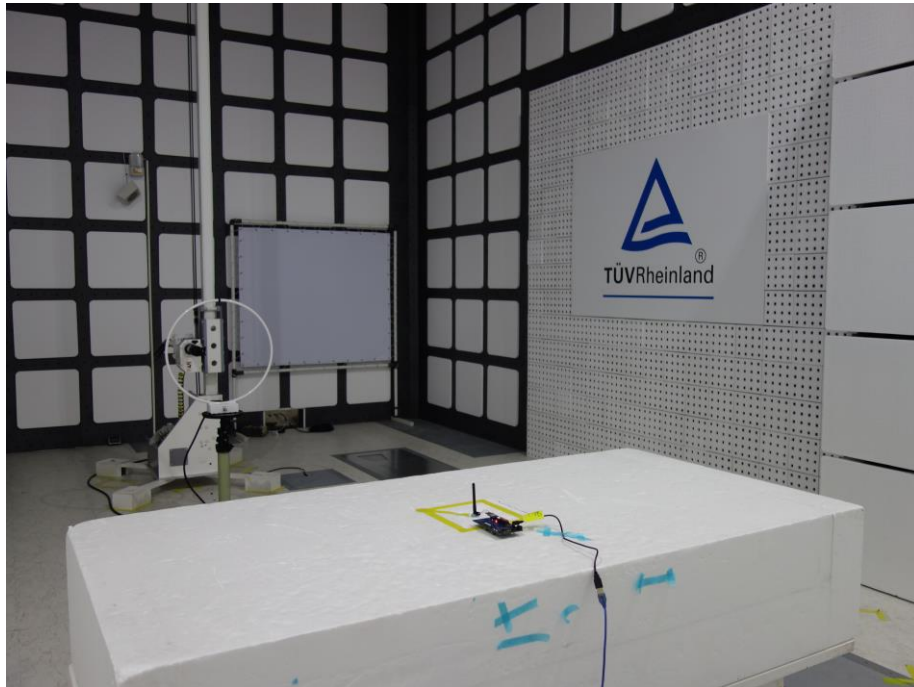
Photograph 19: Test Setup for Spurious Emissions (Back View 3, MSK32WT-M13, ZIGBEE)
