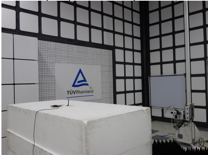
Photograph 14: Test Setup for Spurious Emissions (Back View 4, MSK32WT-M13, BLE)
