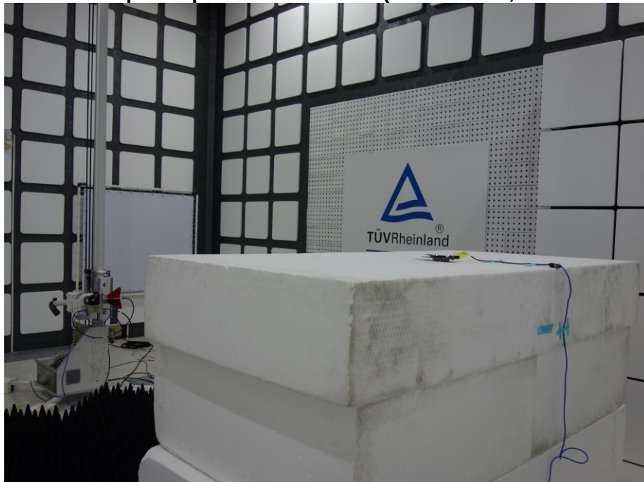
Photograph 4: Test Setup for Spurious Emissions (Back View 2, MSK32WT-M10)
