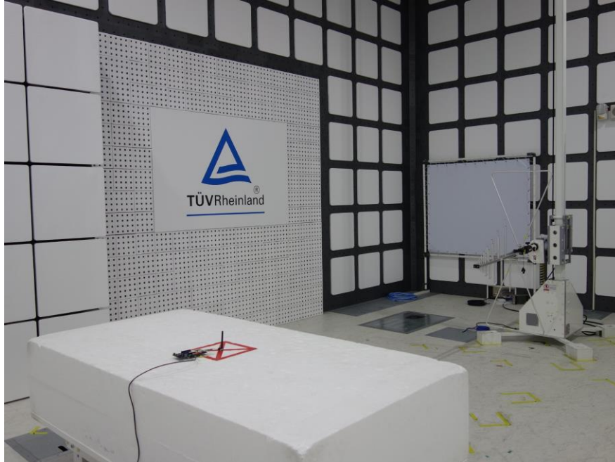
Photograph 11: Test Setup for Spurious Emissions (Back View 1, MSK32WT-M13, BLE)
