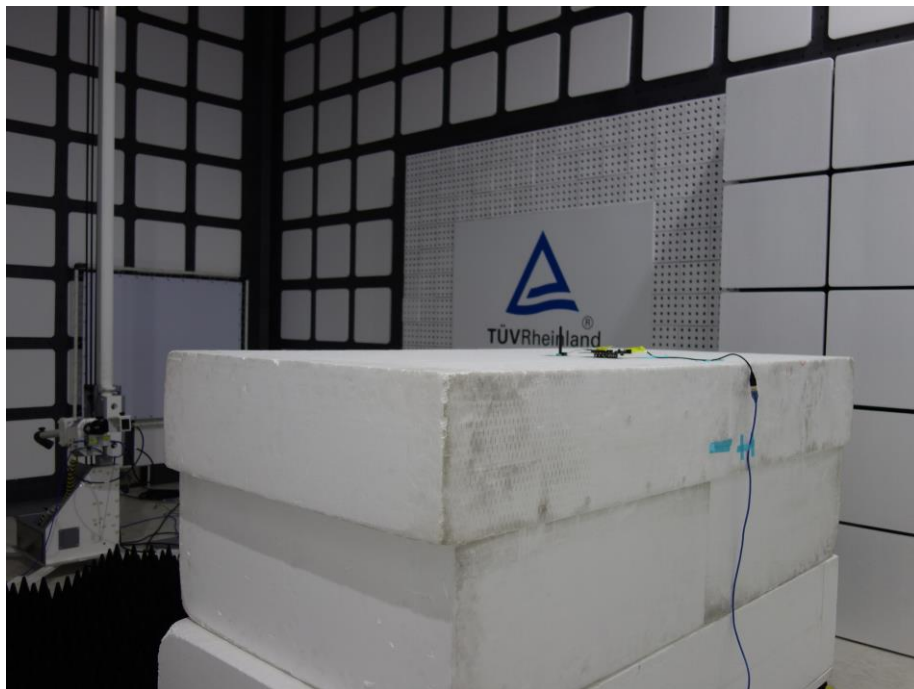
Photograph 18: Test Setup for Spurious Emissions (Back View 2, MSK32WT-M13, ZIGBEE)
