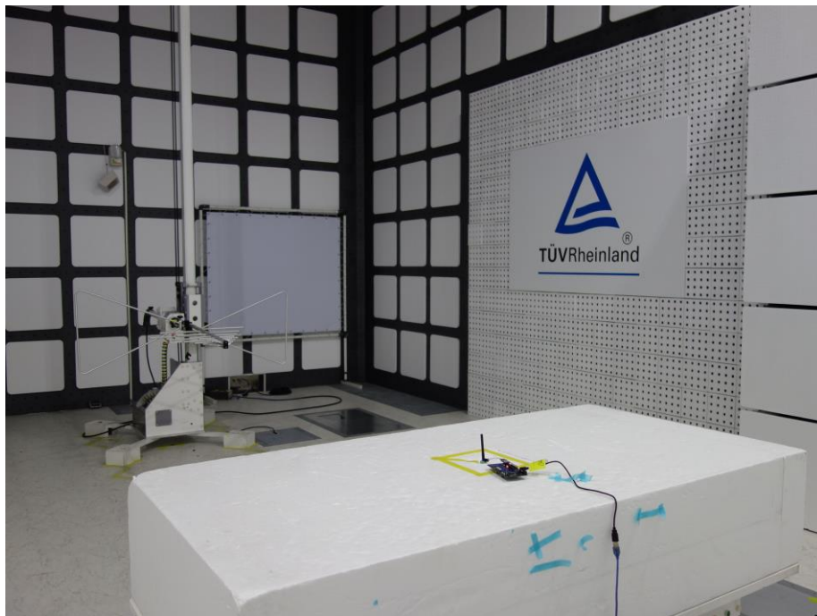
Photograph 20: Test Setup for Spurious Emissions (Back View 4, MSK32WT-M13, ZIGBEE)
