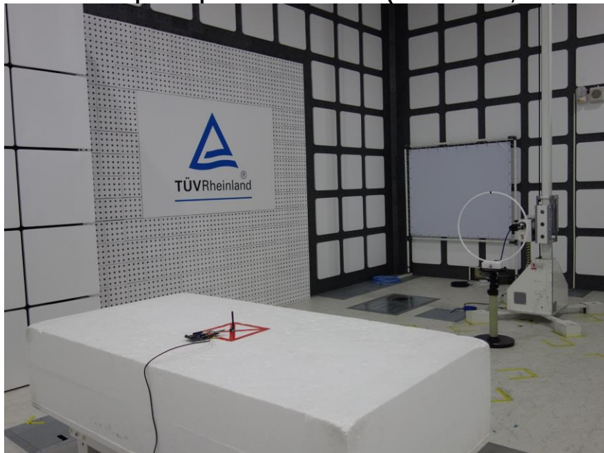
Photograph 12: Test Setup for Spurious Emissions (Back View 2, MSK32WT-M13, BLE)
