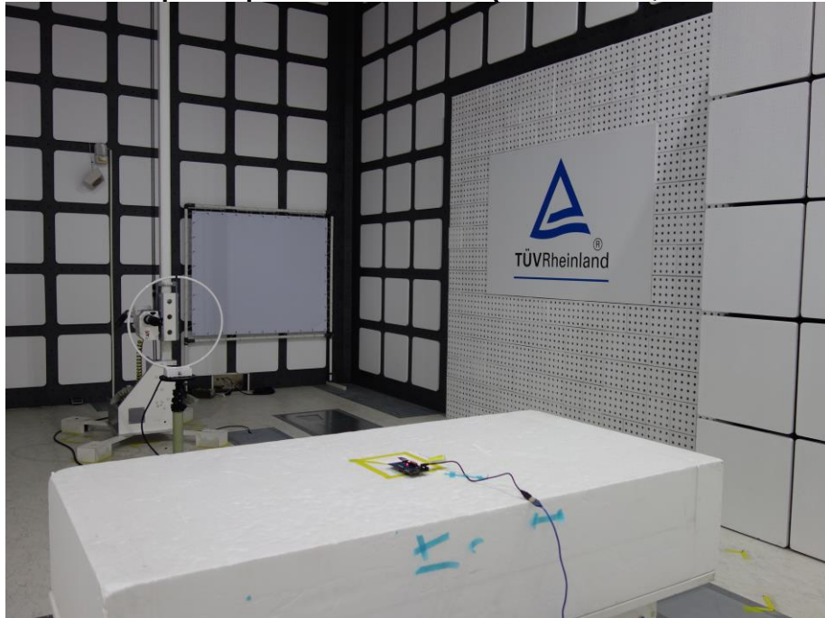
Photograph 6: Test Setup for Spurious Emissions (Back View 4, MSK32WT-M10)
