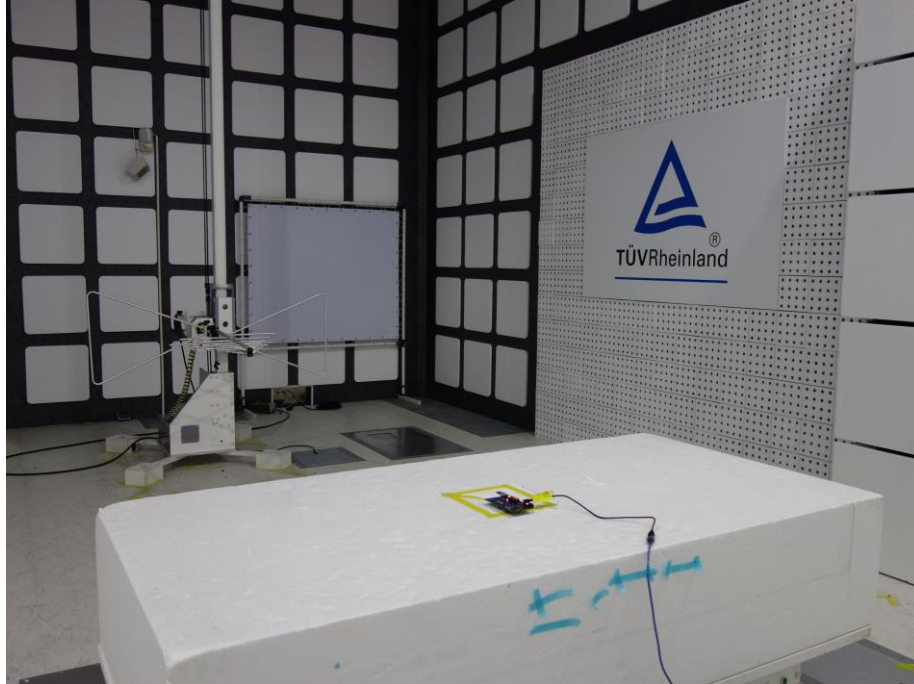
Photograph 5: Test Setup for Spurious Emissions (Back View 3, MSK32WT-M10)
