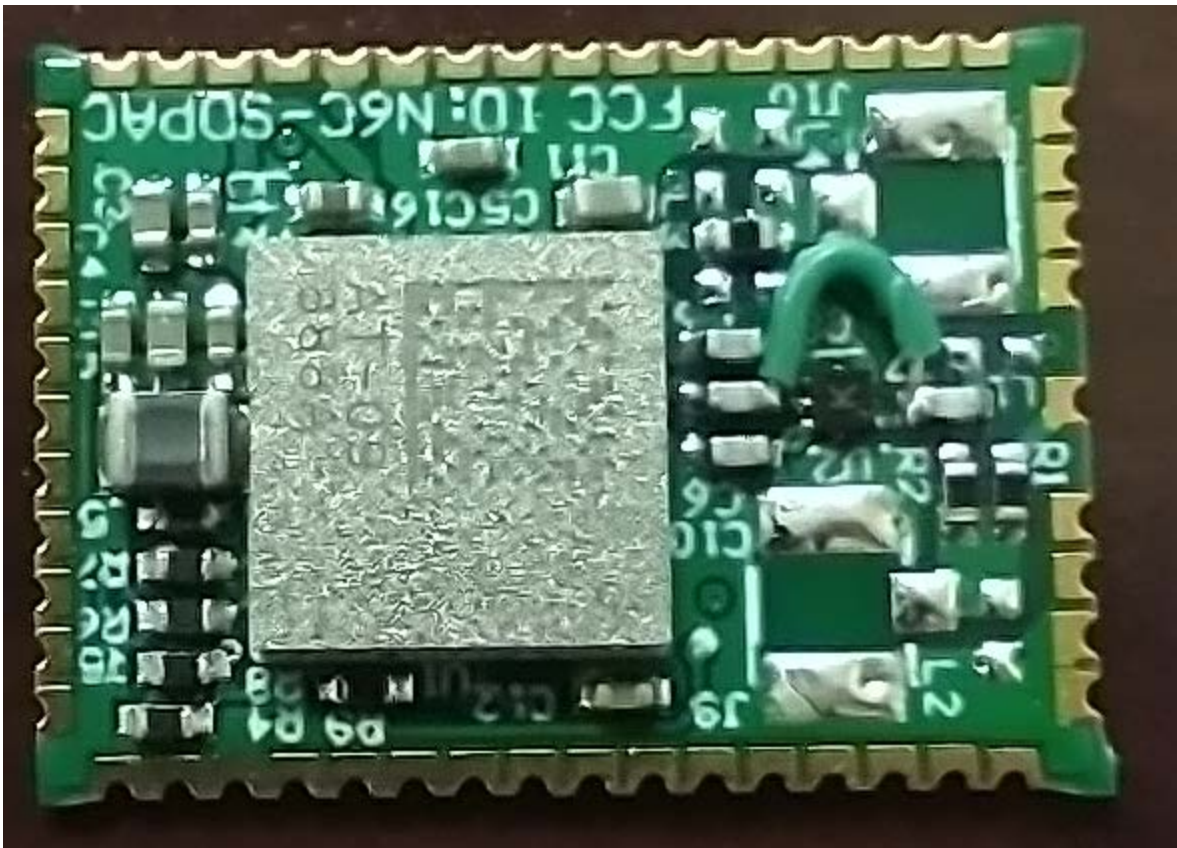
Figure 1: Front View
